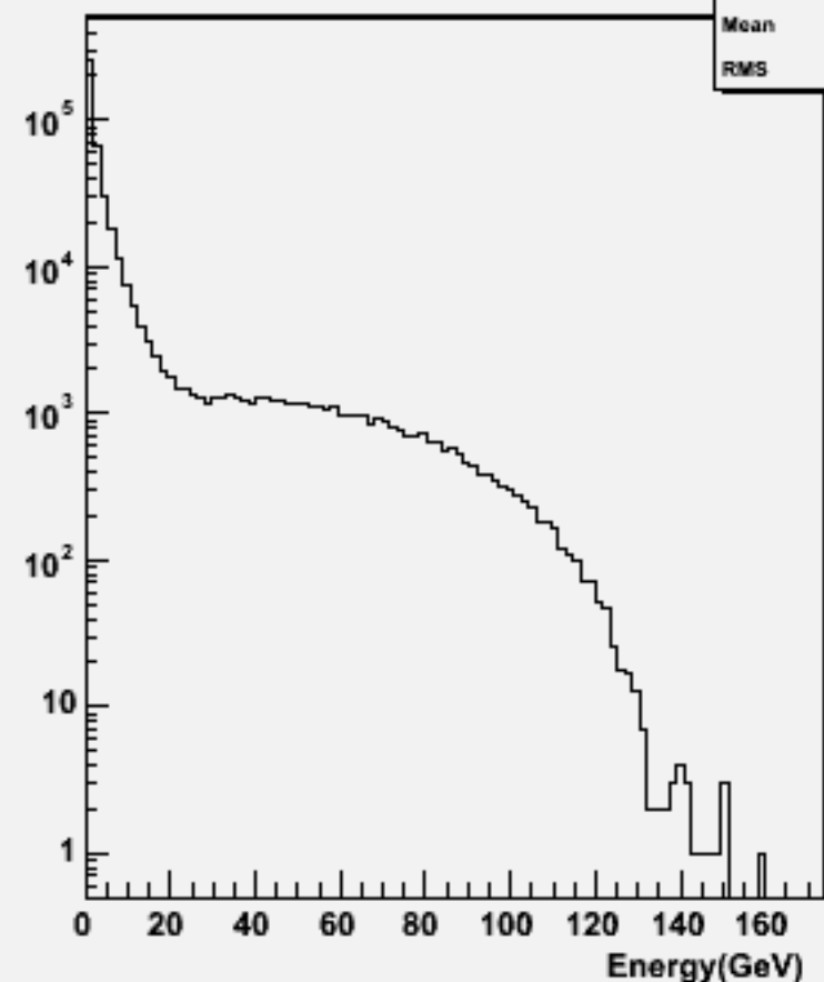
Start point R : w101309 n1n1n1e1du_o
