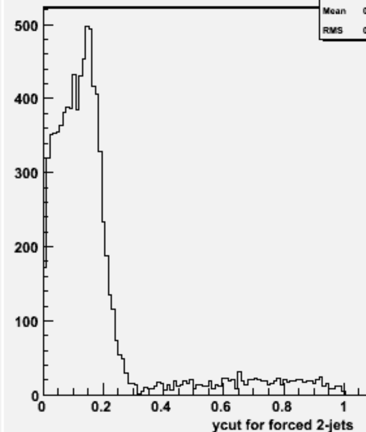
Ycut for 2-jets :w101309 n1n1n1e1du_o
