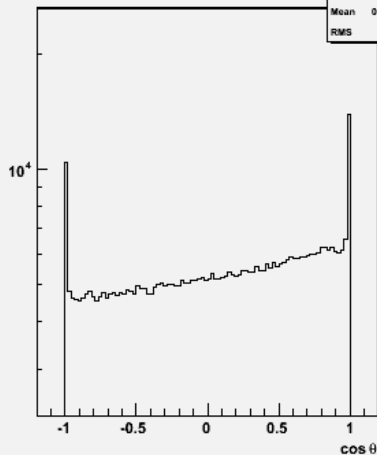
Particle cosθ : w101309 n1n1n1e1du_o
