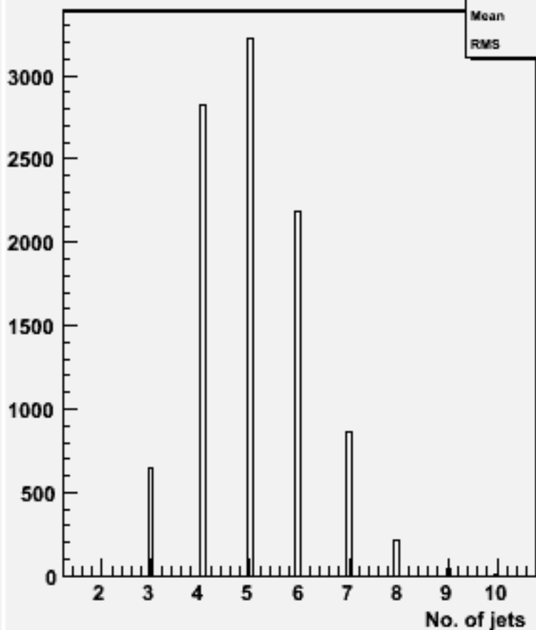
No. jets (ycut=0.001) : w101309 n1n1n1e1du_o
