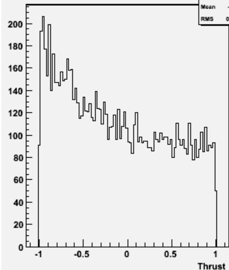
cos \Theta (thrust) w101309 n1n1n1e1du_o
