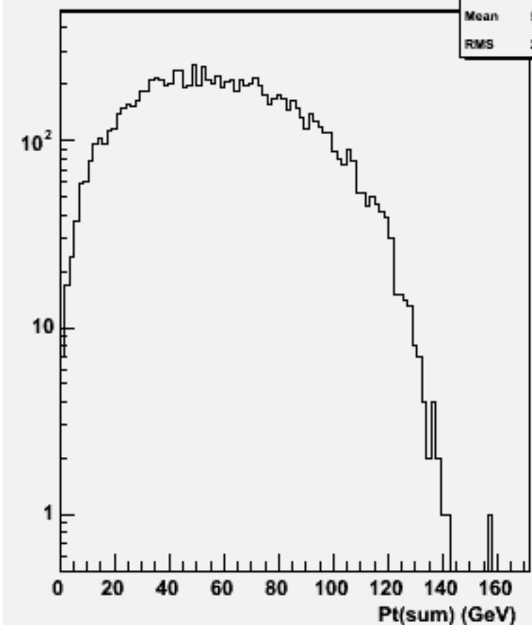
Pt Sum: w101309 n1n1n1e1du_o
