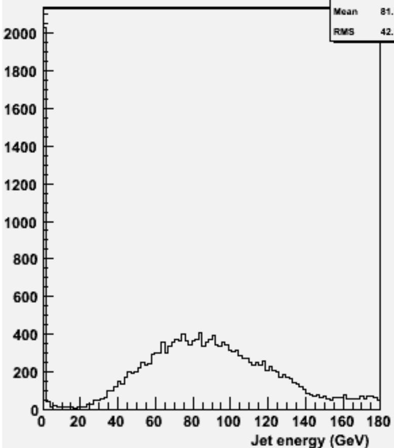
energy for 2-jets :w101309 n1n1n1e1du_o
