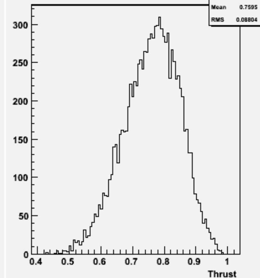
Thrust w101309 n1n1n1e1du_o
