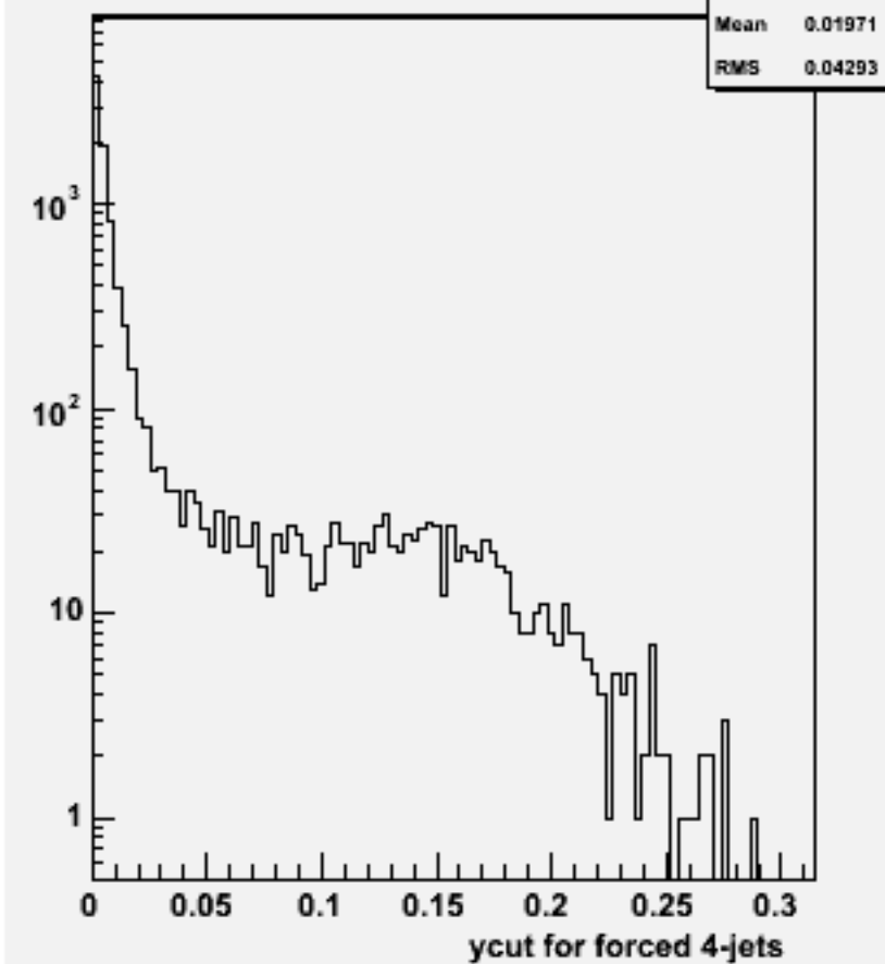
Ycut for 4-jets :w101309 n1n1n1e1du_o
