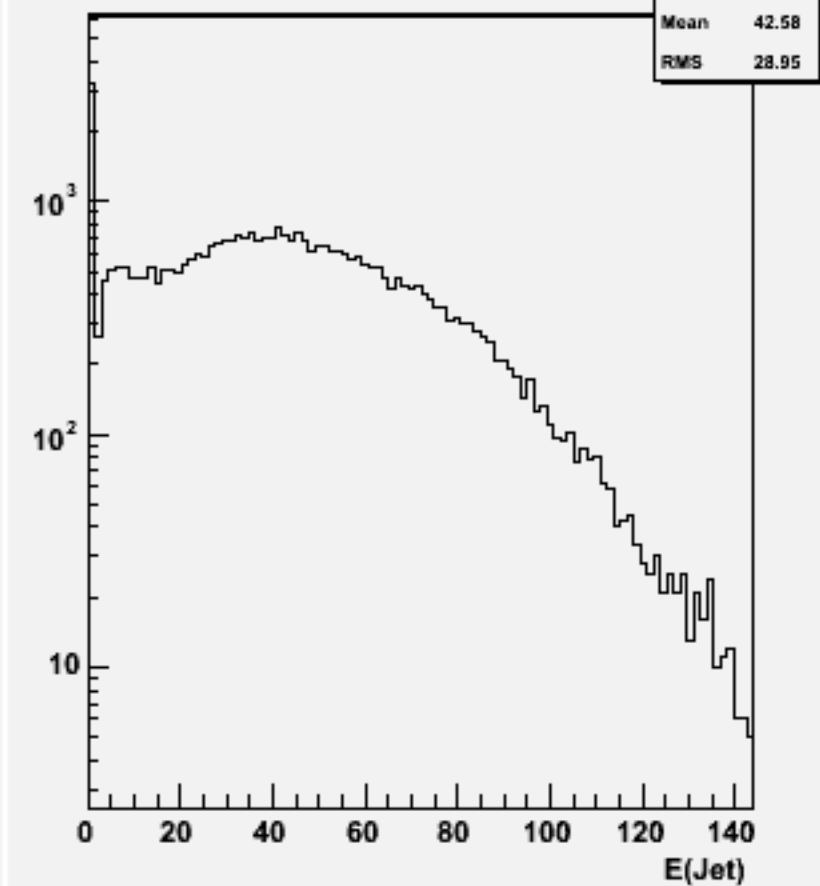
Jet energies(All jets)w101309 n1n1n1e1du_o
