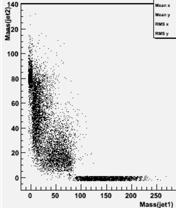
Jet mass for forced 2-jets : w101309 n1n1n1e1du_o
