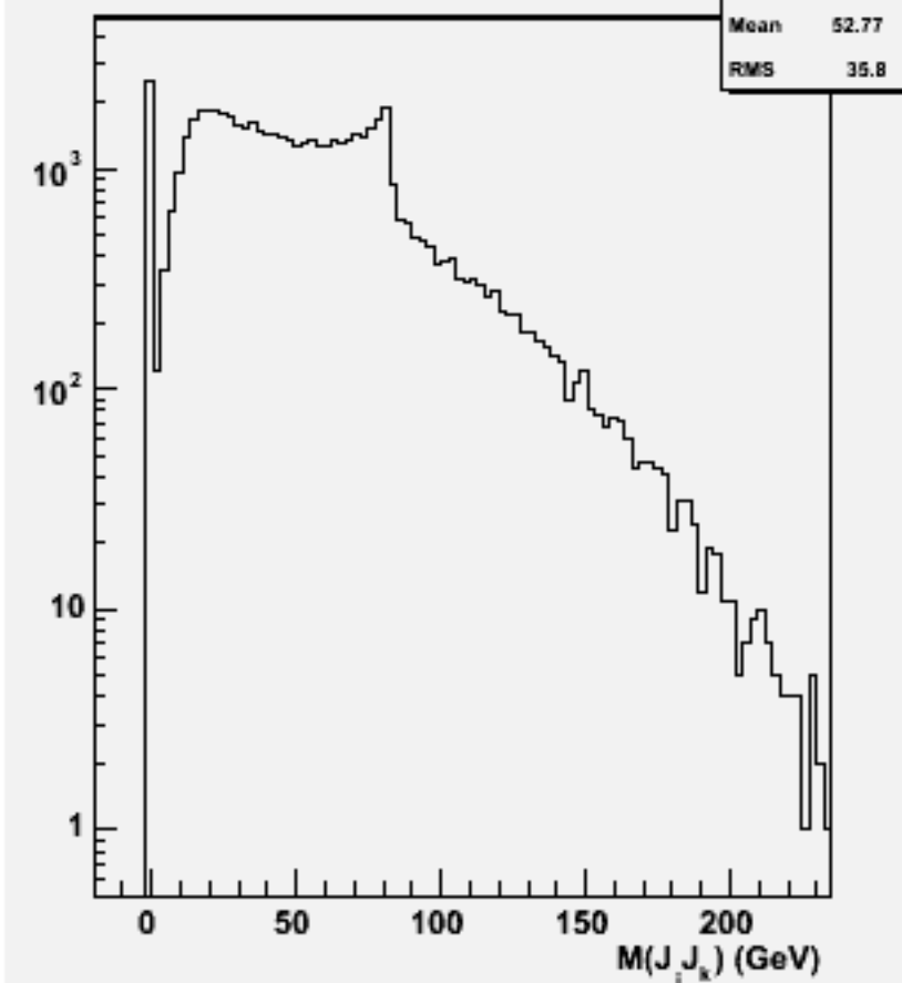
2jets mass(All comb)w101309 n1n1n1e1du_o
