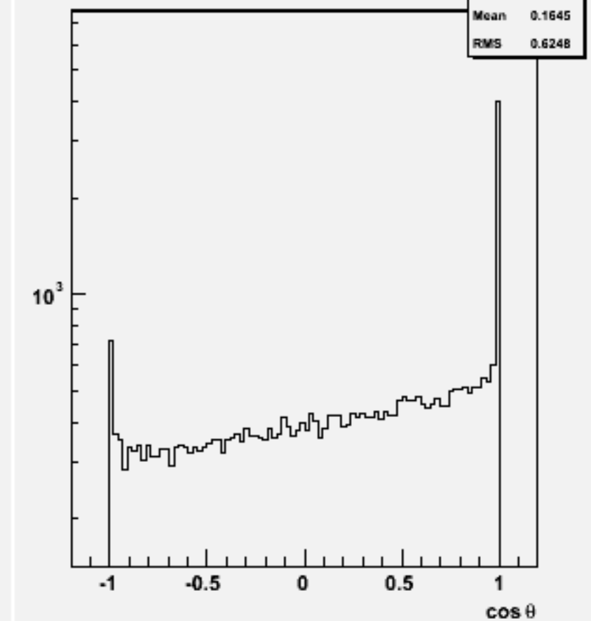
Jet cos \theta (All jets)w101309 n1n1n1e1du_o
