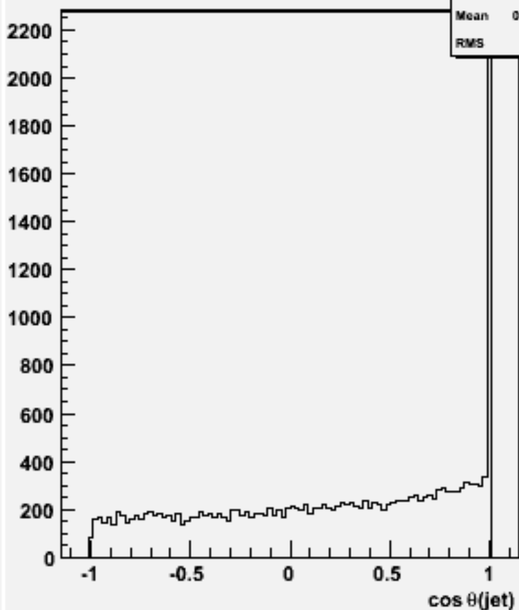
cos \Theta for 2-jets :w101309 n1n1n1e1du_o
