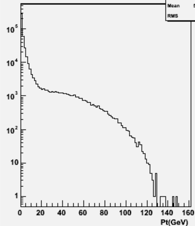
Start point Z : w101309 n1n1n1e1du_o
