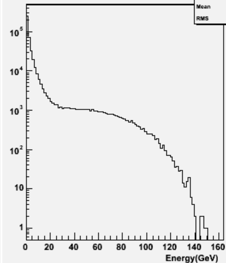
Particle Energy : w101308 n1n1n1e1du_o
