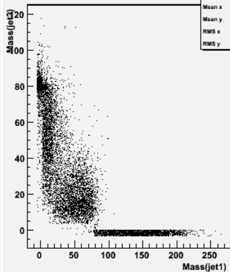
Jet mass for forced 2-jets : w101308 n1n1n1e1du_o
