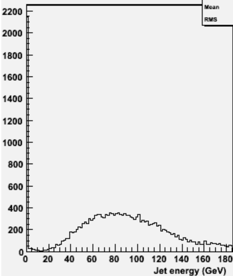
energy for 2-jets :w101308 n1n1n1e1du_o
