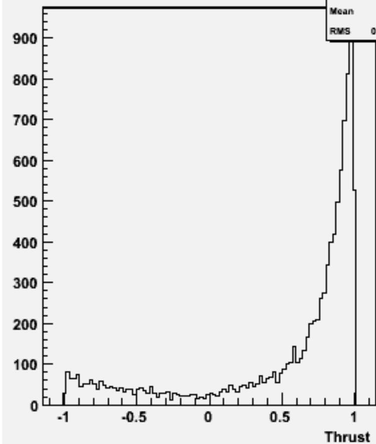
cos \Theta (thrust) w101308 n1n1n1e1du_o
