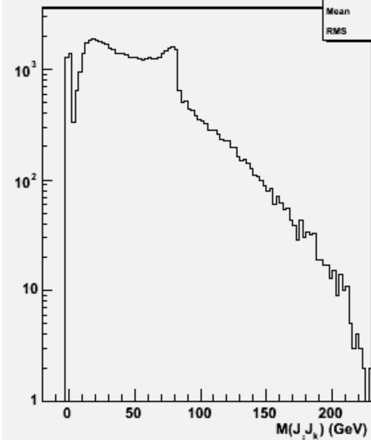
2jets mass(All comb)w101308 n1n1n1e1du_o
