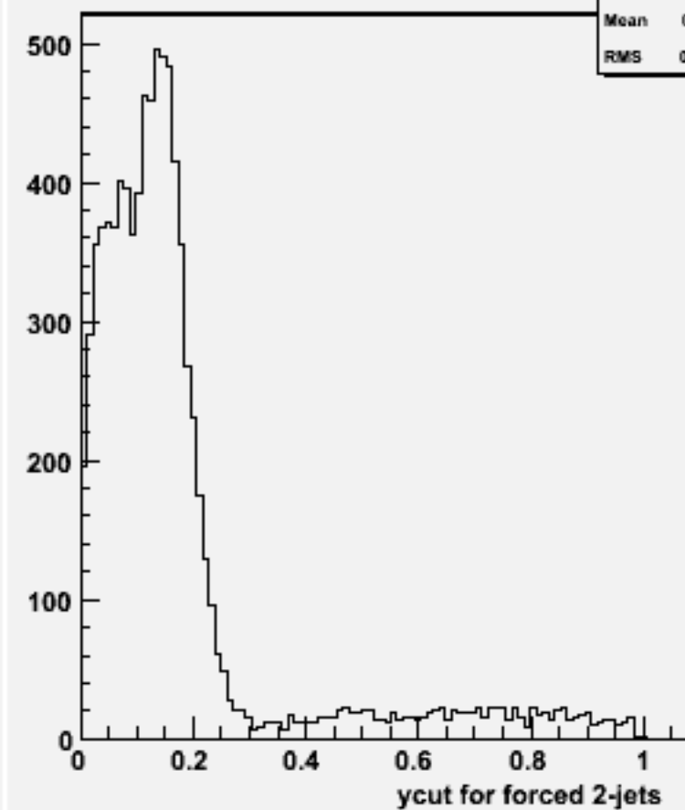
Ycut for 2-jets :w101308 n1n1n1e1du_o
