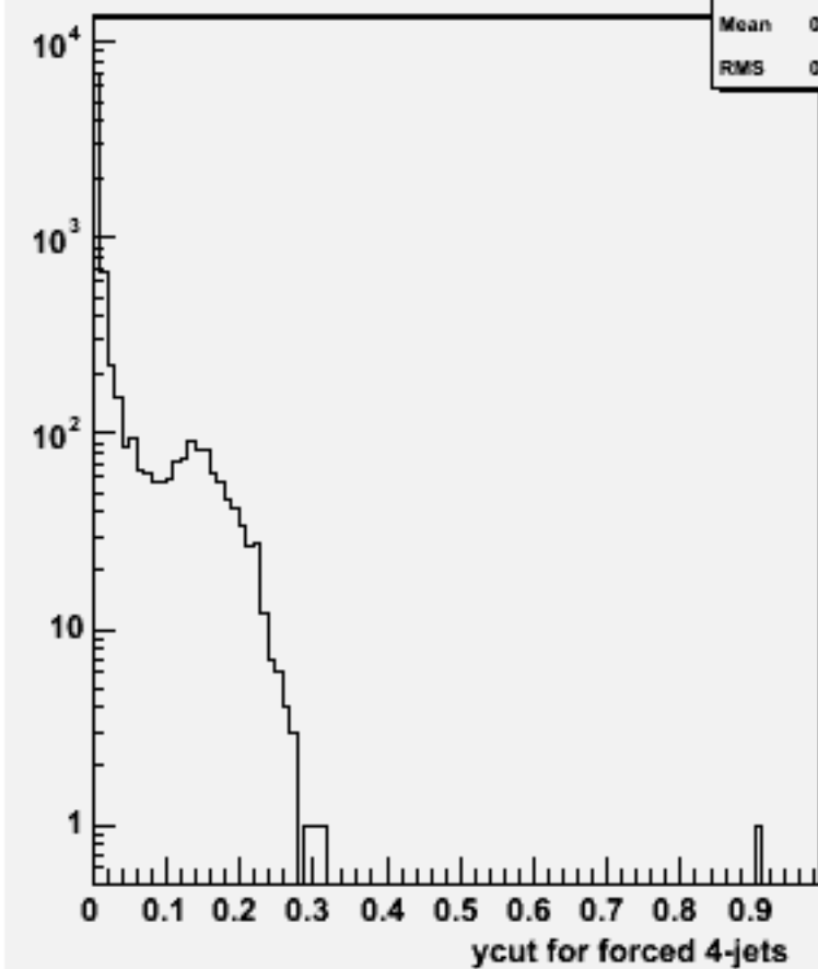
Ycut for 4-jets :w101308 n1n1n1e1du_o
