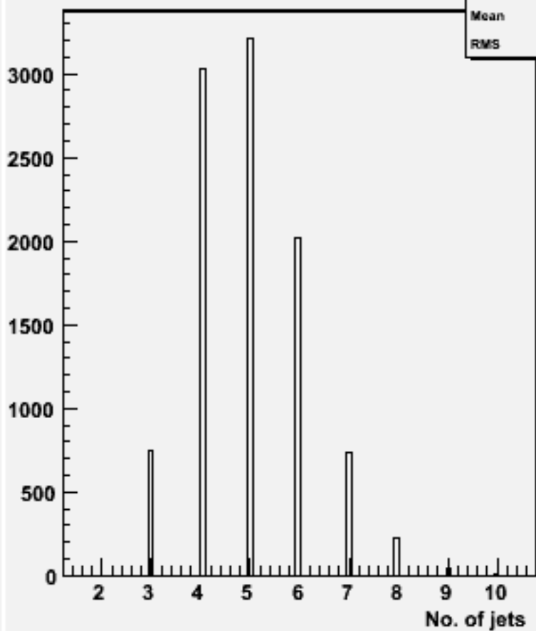
No. jets (ycut=0.001) : w101308 n1n1n1e1du_o
