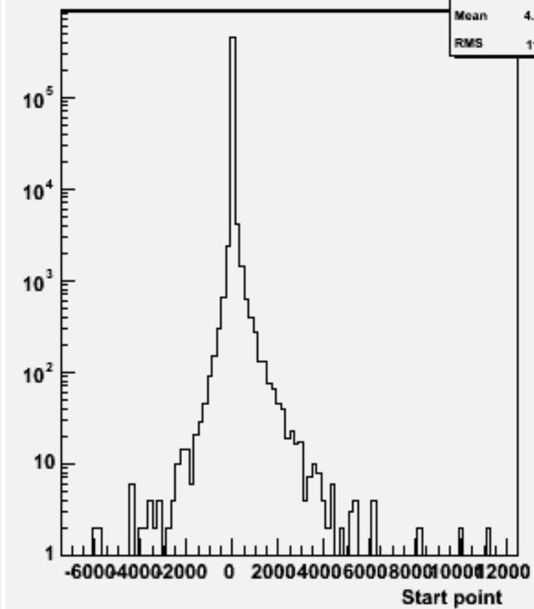
Start point Z : w101308 n1n1n1e1du_o
