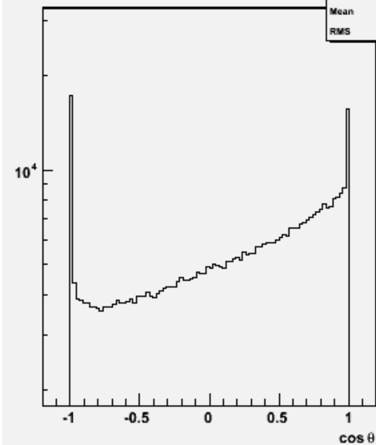
Particle cos \theta : w101308 n1n1n1e1du_o
