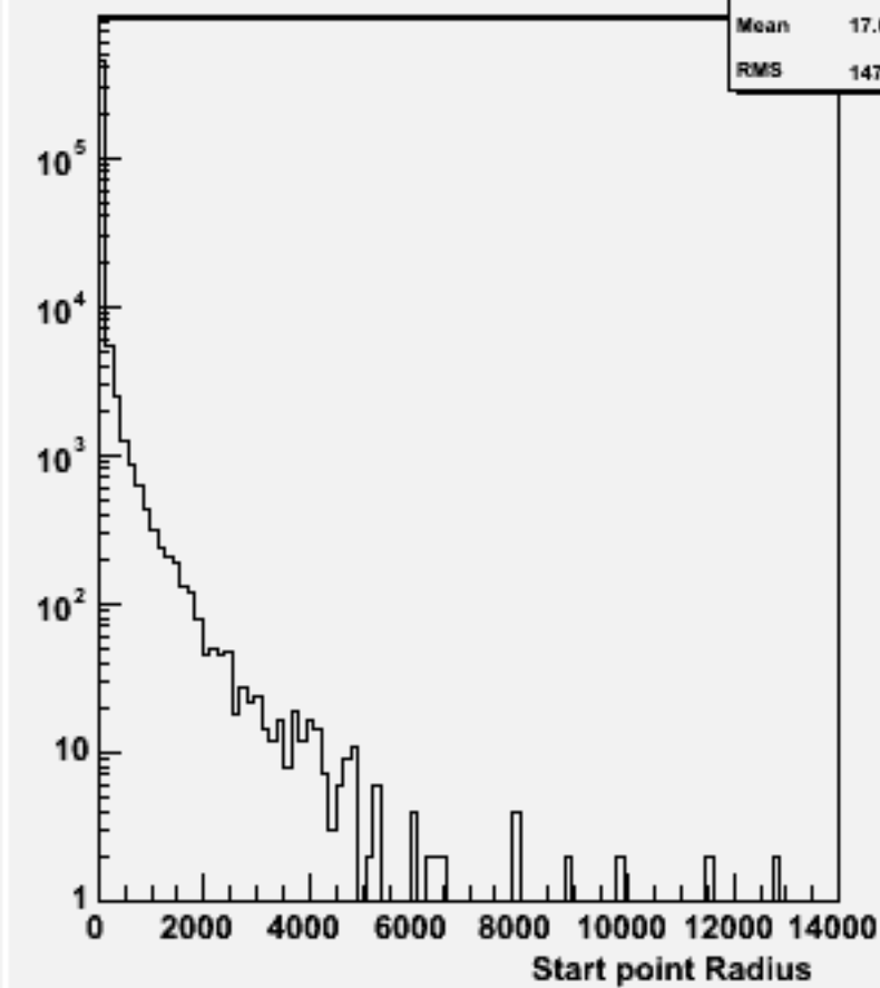
Start point R : w101308 n1n1n1e1du_o
