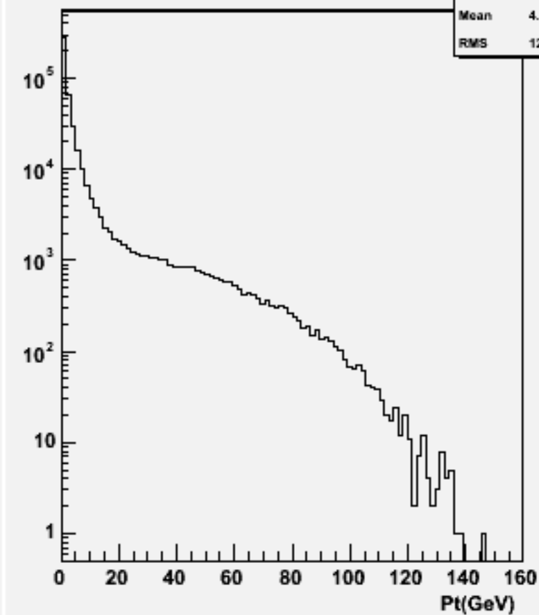
Particle Pt : w101308 n1n1n1e1du_o
