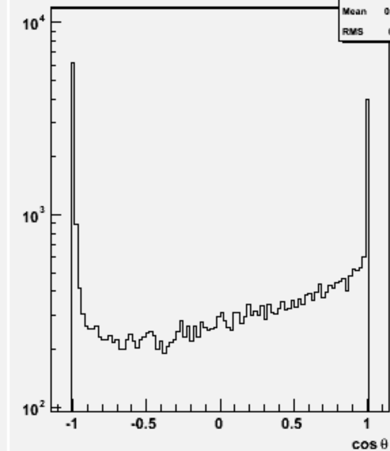
Jet cos \theta (All jets)w101308 n1n1n1e1du_o
