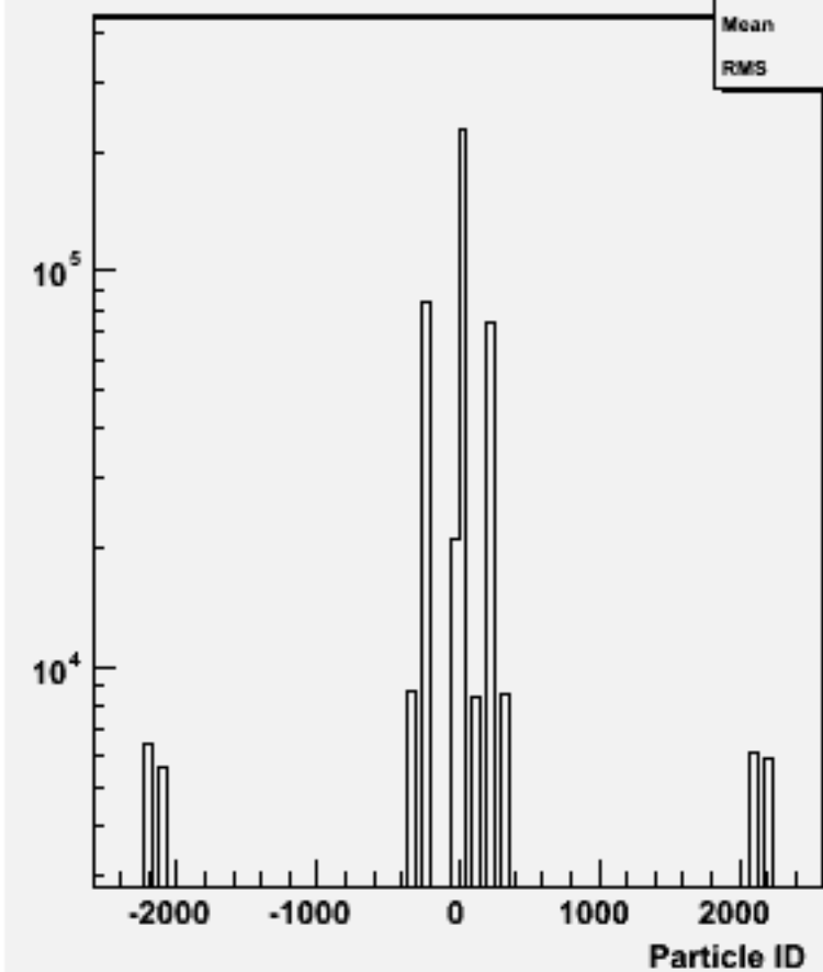
Particle ID : w101308 n1n1n1e1du_o
