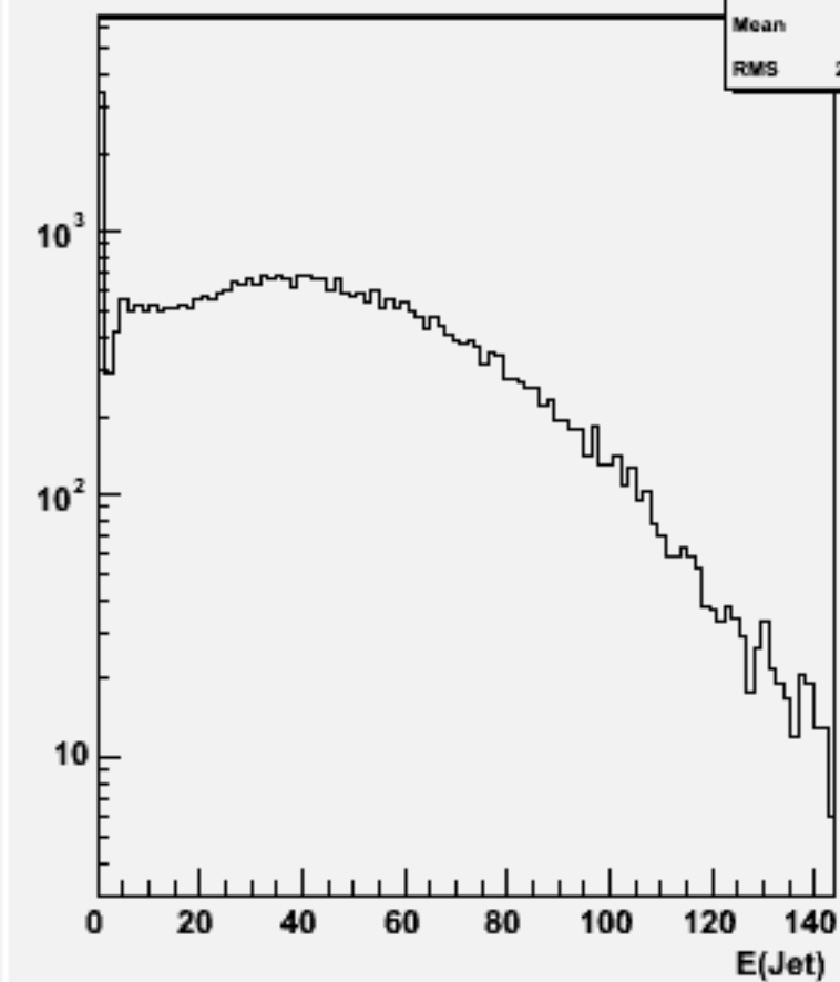
Jet energies(All jets)w101308 n1n1n1e1du_o
