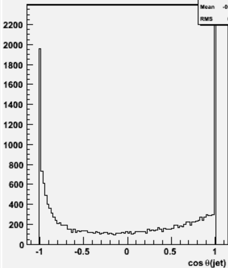
cos \theta for 2-jets :w101308 n1n1n1e1du_o
