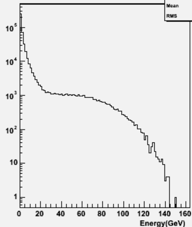
Start point R : w101307 n1n1n1e1du_o
