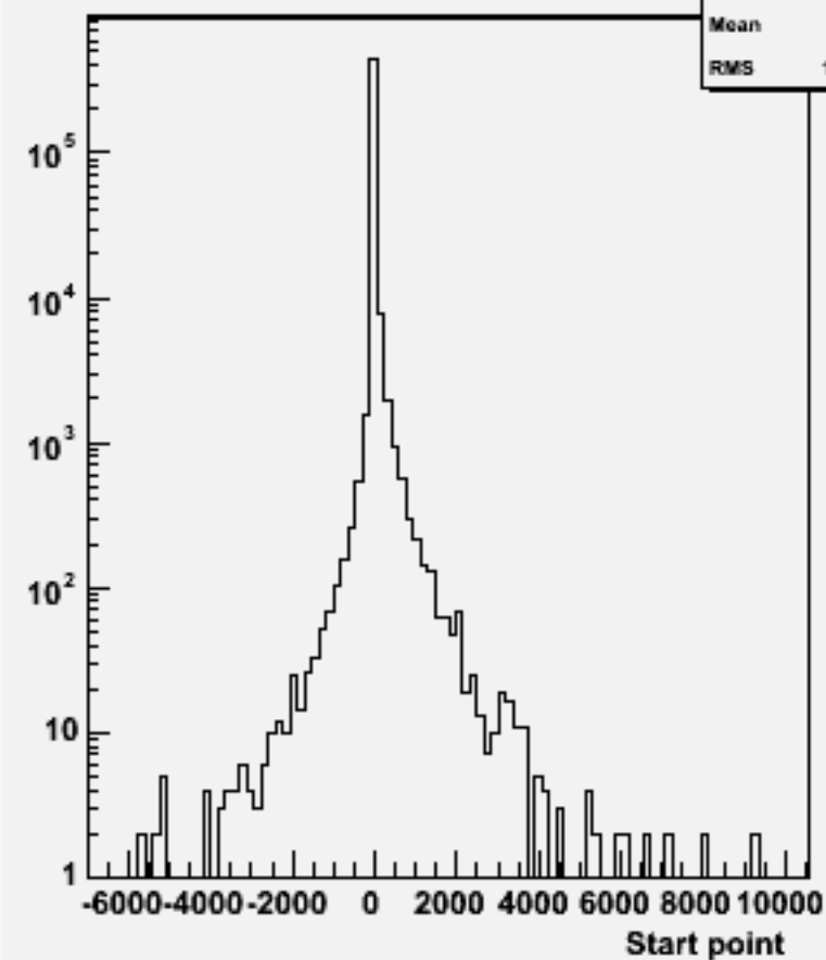
Start point Z : w101307 n1n1n1e1du_o
