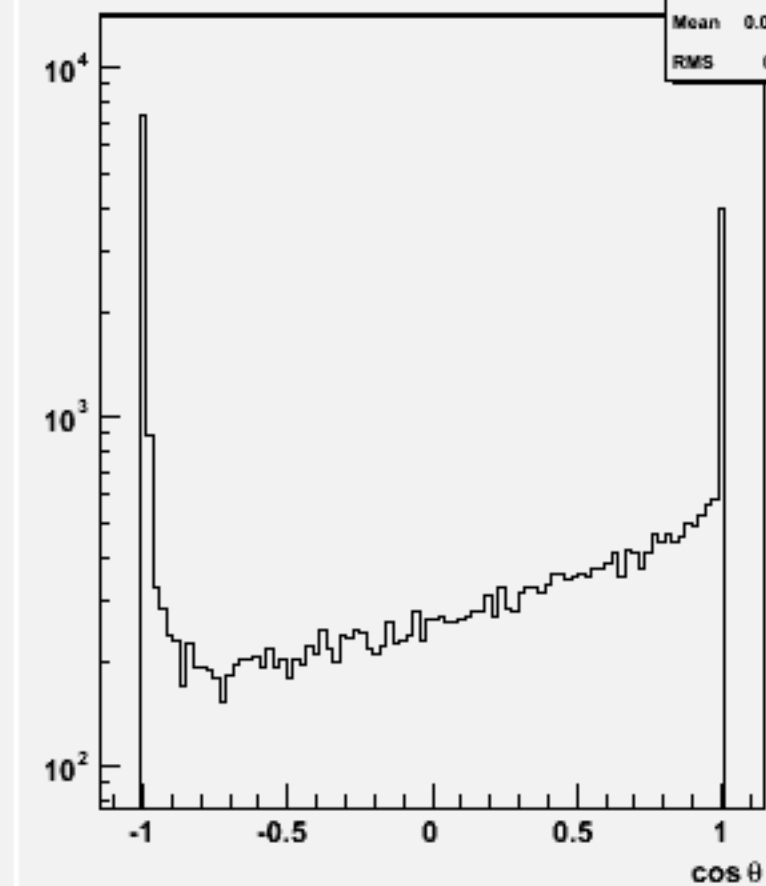
Jet cos \theta (All jets)w101307 n1n1n1e1du_o
