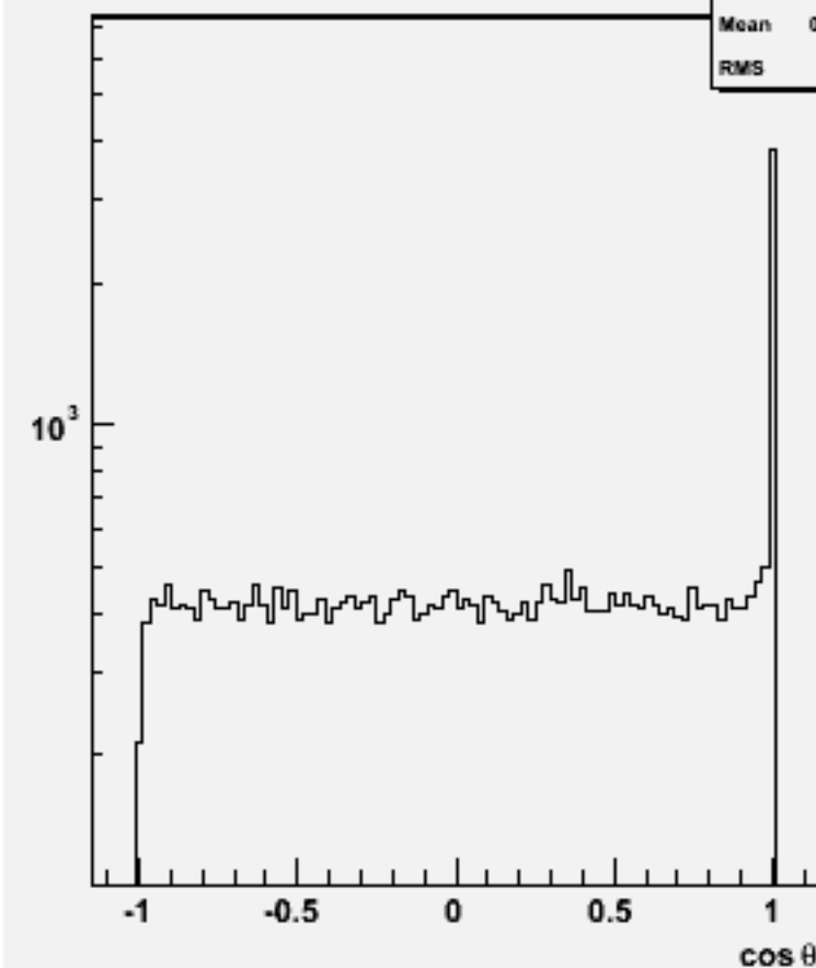
Jet cos \theta (All jets)w101293 bbcssc_o
