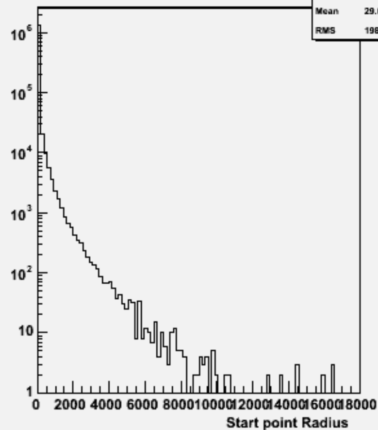
Start point R : w101293 bbcssc_o
