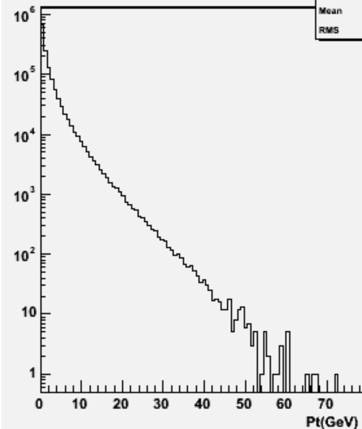
Particle Pt : w101293 bbcssc_o
