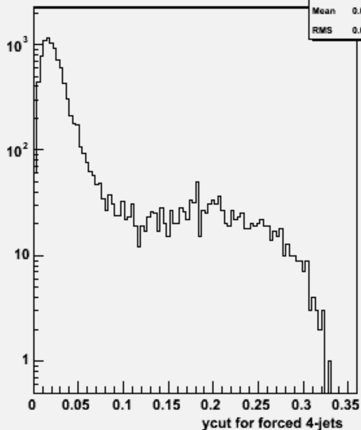
Ycut for 4-jets :w101293 bbcssc_o
