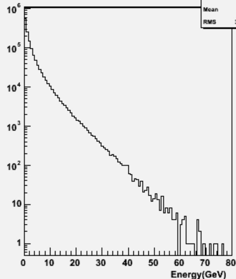
Particle Energy : w101293 bbcssc_o
