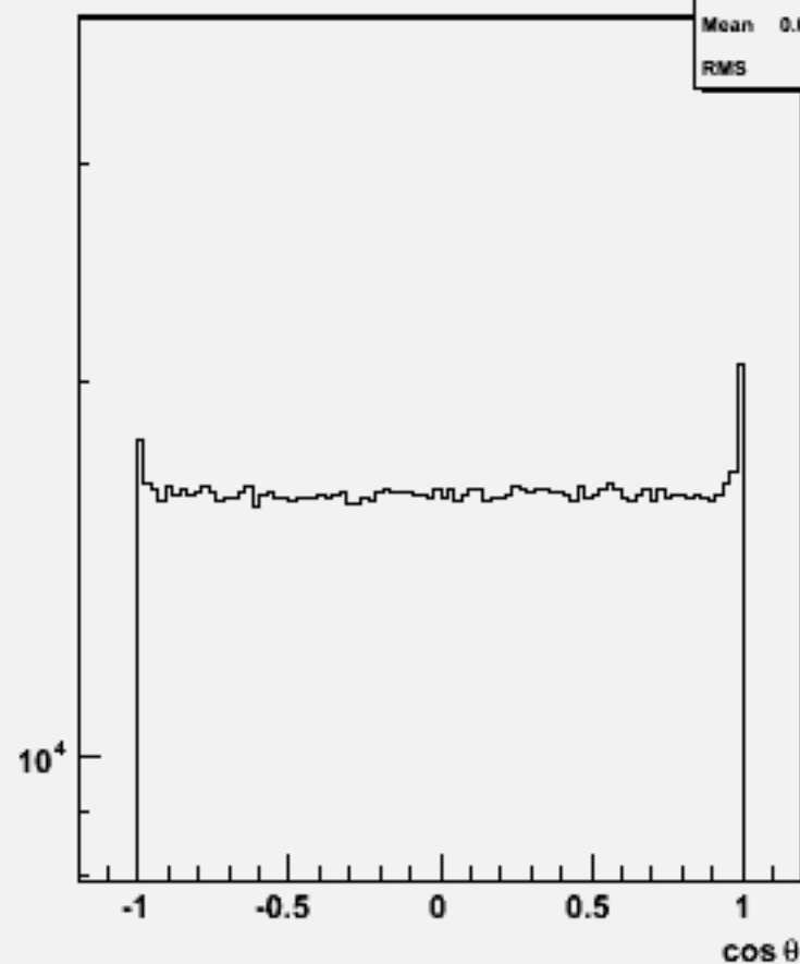
Particle cosθ : w101293 bbcssc_o
