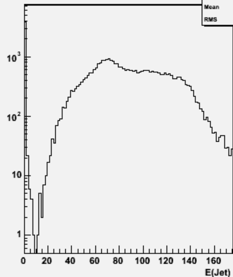
Jet energies(All jets)w101293 bbcssc_o
