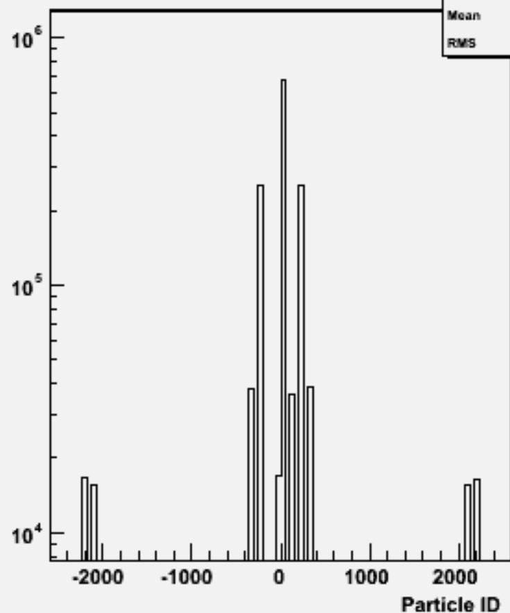
Particle ID : w101293 bbcssc_o
