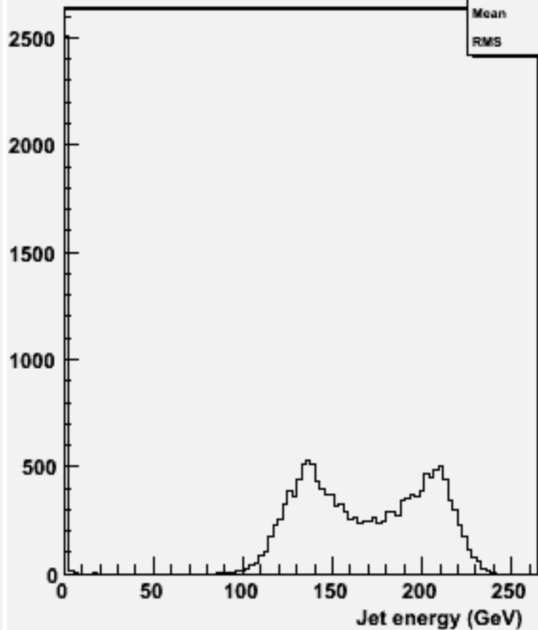
energy for 2-jets :w101293 bbcssc_o
