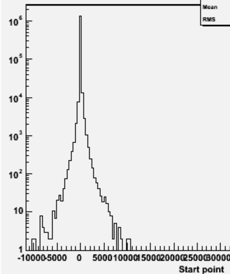
Start point Z : w101293 bbcssc_o
