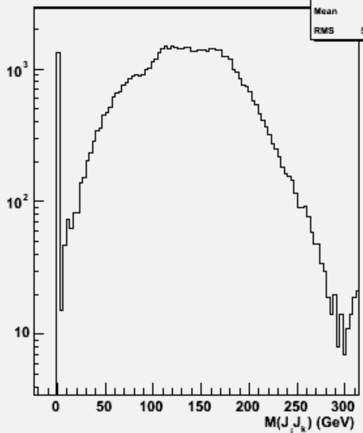
2jets mass(All comb)w101293 bbcssc_o
