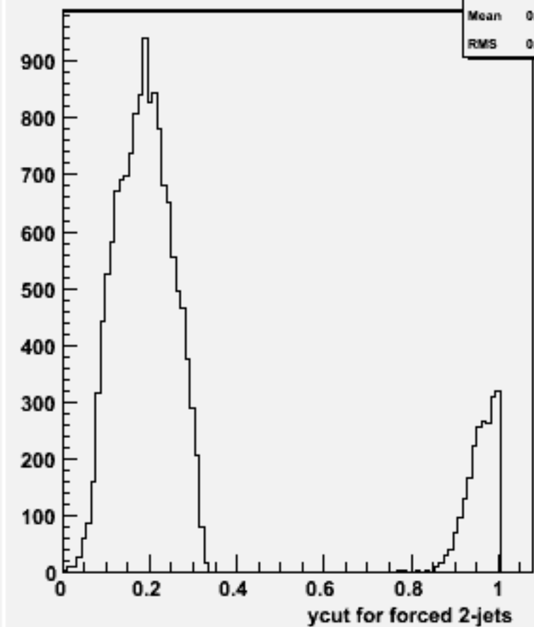
Ycut for 2-jets :w101292 bbcssc_o
