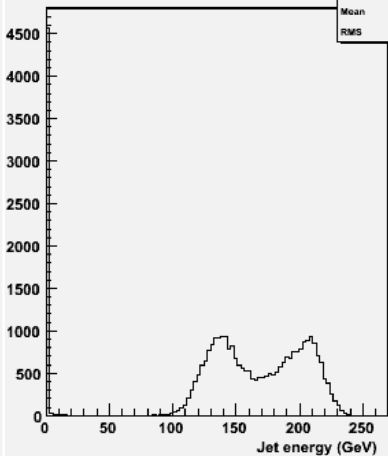
energy for 2-jets :w101292 bbcssc_o
