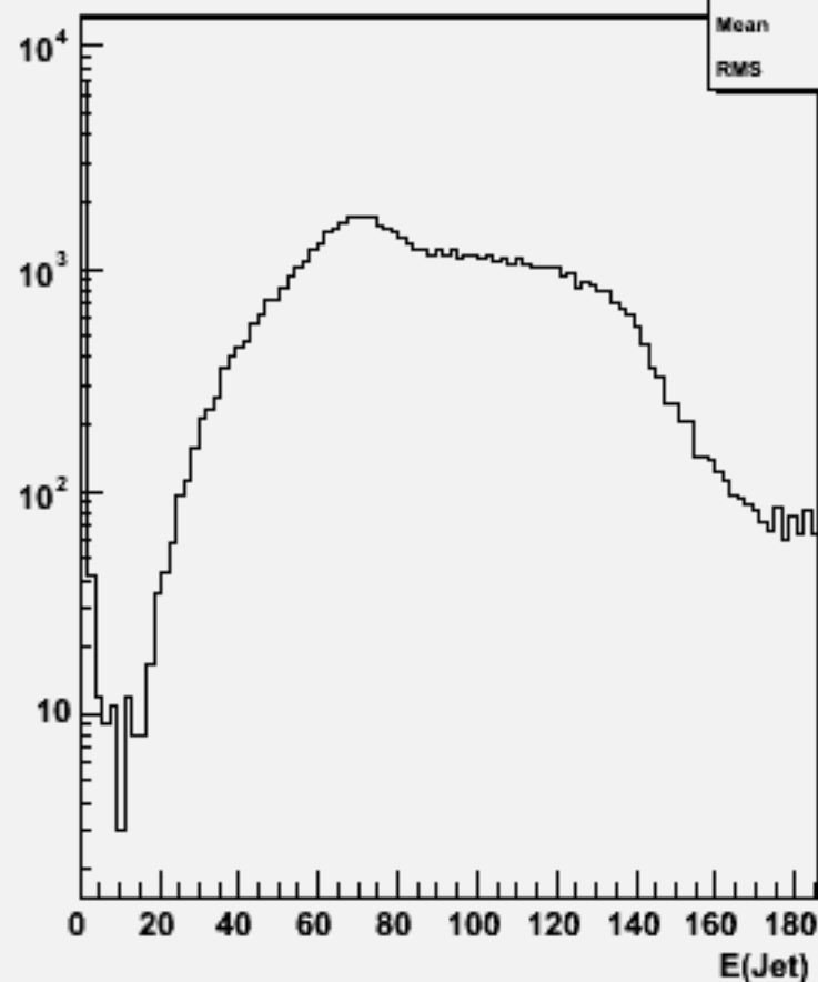
Jet energies(All jets)w101292 bbcssc_o
