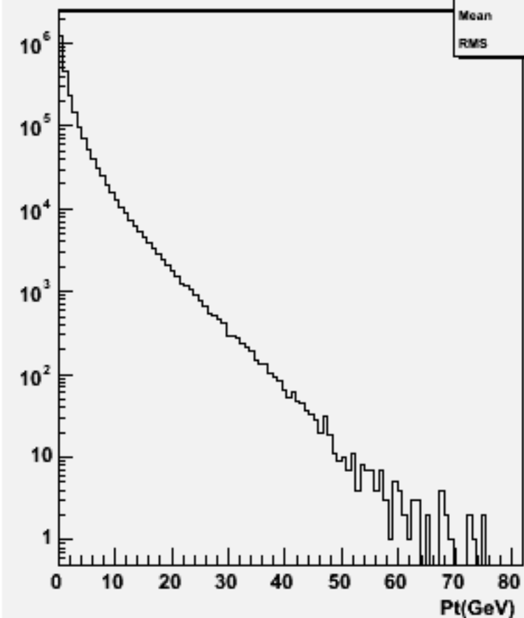
Particle Pt : w101292 bbcssc_o
