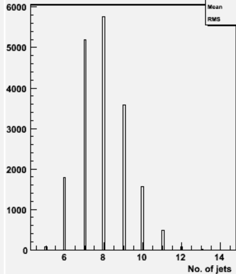
No. jets (ycut=0.001) : w101292 bbcssc_o
