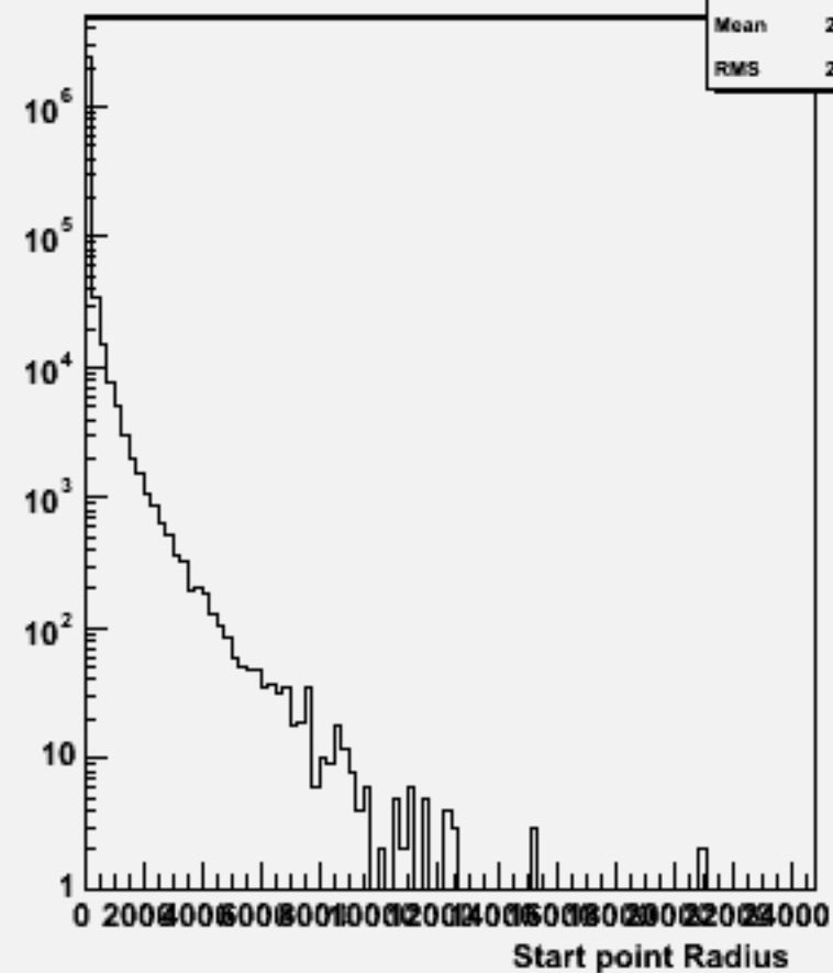
Start point R : w101292 bbcssc_o
