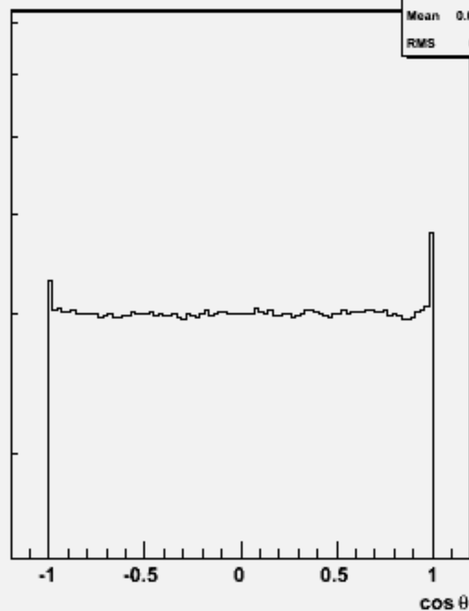
Particle cosθ : w101292 bbcssc_o
