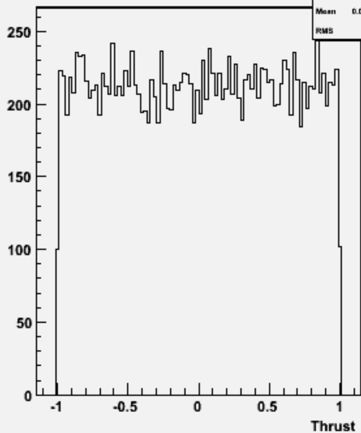
cos \Theta (thrust) w101292 bbcssc_o
