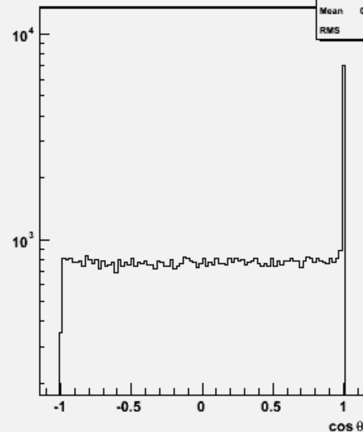
Jet cos \theta (All jets)w101292 bbcssc_o
