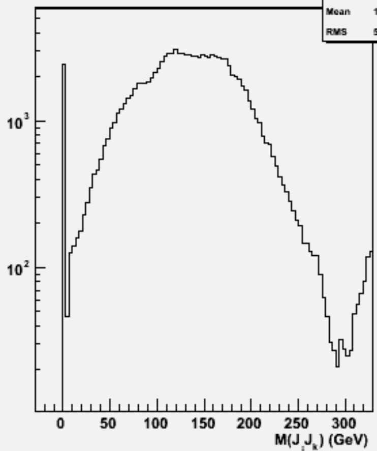
2jets mass(All comb)w101292 bbcssc_o
