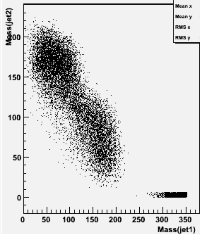
Jet mass for forced 2-jets : w101292 bbcssc_o
