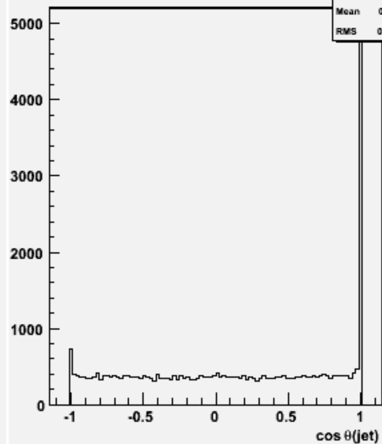
cos \theta for 2-jets :w101292 bbcssc_o
