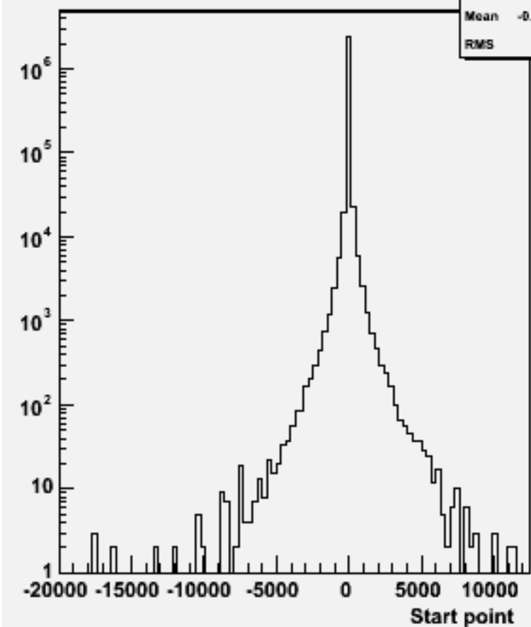
Start point Z : w101292 bbcssc_o
