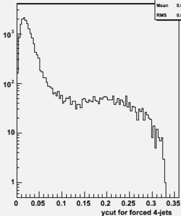
Ycut for 4-jets :w101292 bbcssc_o
