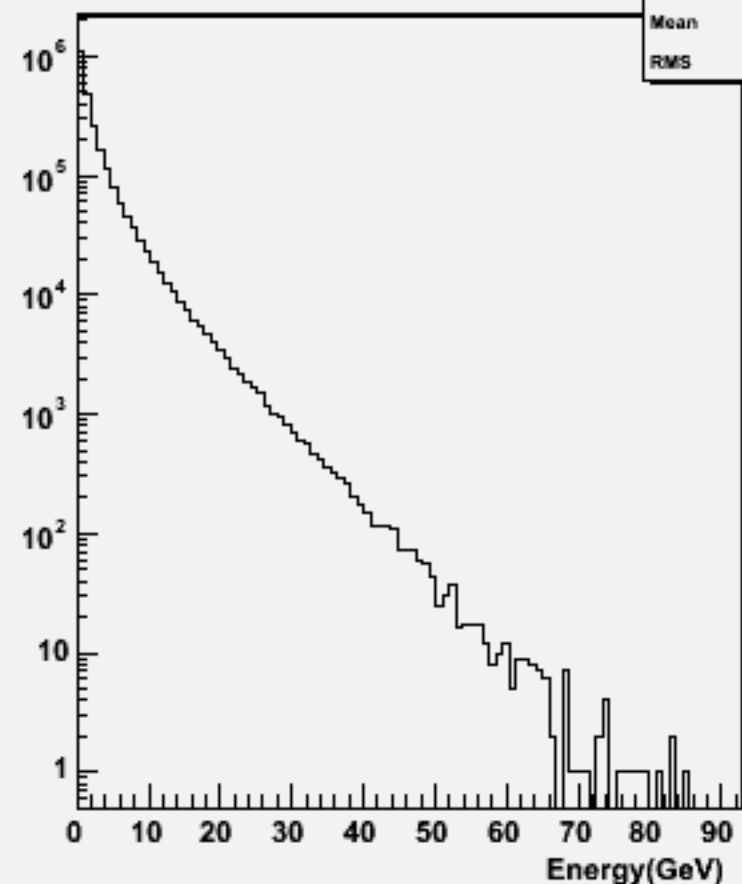
Particle Energy : w101292 bbcssc_o
