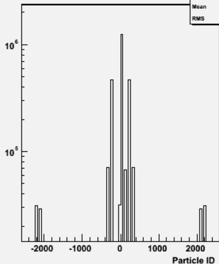
Particle ID : w101292 bbcssc_o
