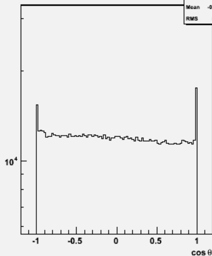
Particle cos \theta : w101284 bbcse3n3_o
