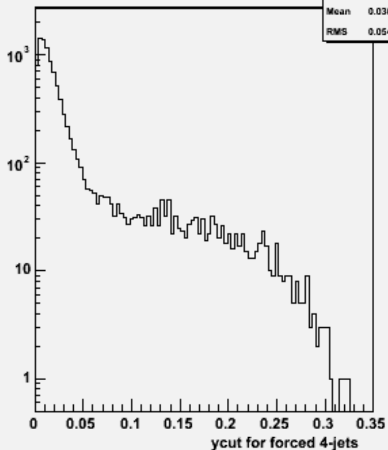
Ycut for 4-jets :w101284 bbcse3n3_o
