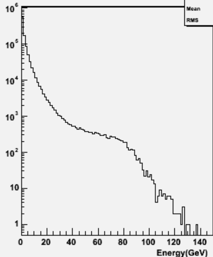
Particle Energy : w101284 bbcse3n3_o
