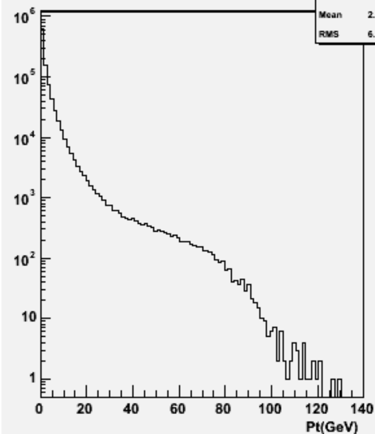
Particle Pt : w101284 bbcse3n3_o
