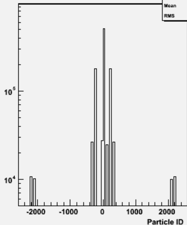
Particle ID : w101284 bbcse3n3_o
