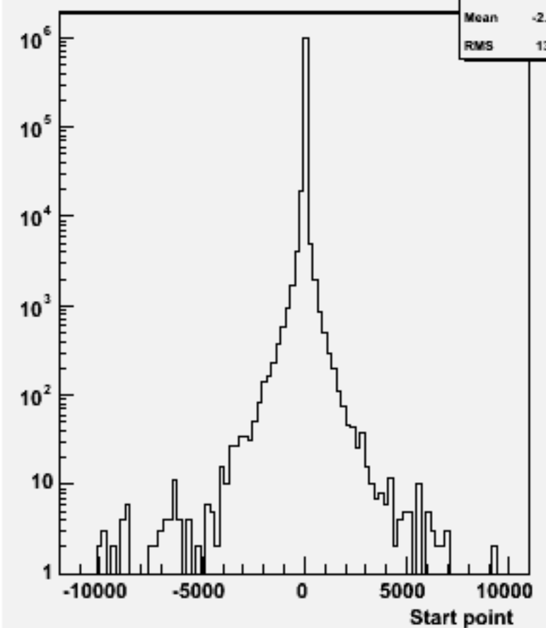
Start point Z : w101284 bbcse3n3_o
