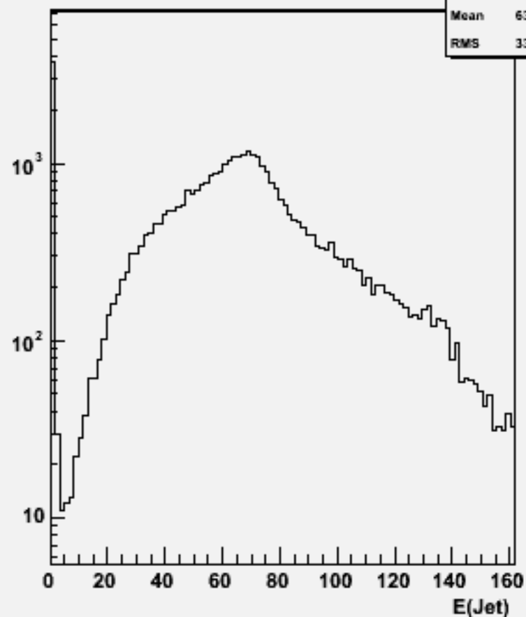
Jet energies(All jets)w101284 bbcse3n3_o
