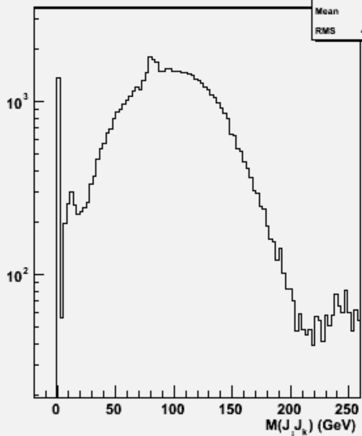
2jets mass(All comb)w101284 bbcse3n3_o
