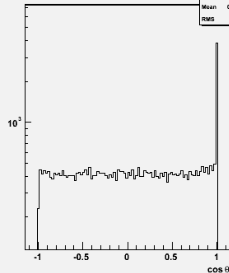
Jet cos \theta (All jets)w101284 bbcse3n3_o
