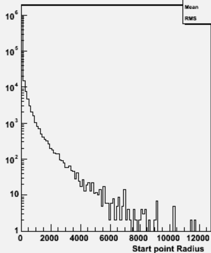
Start point R : w101284 bbcse3n3_o
