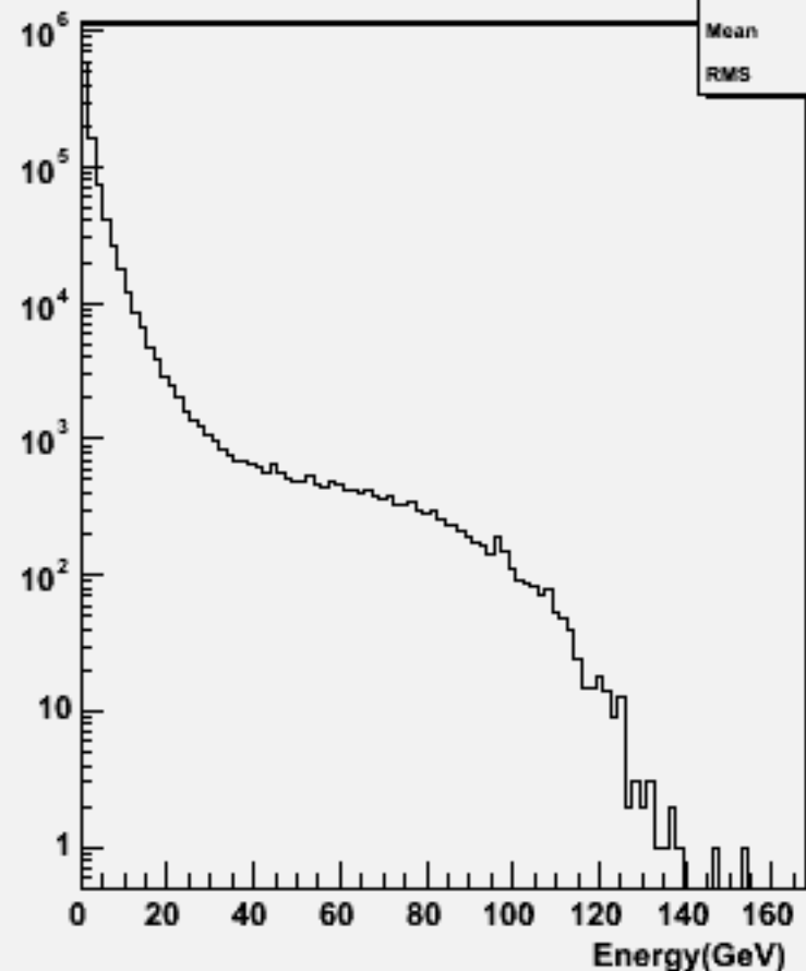
Particle Energy : w101278 bbcse1n1_o
