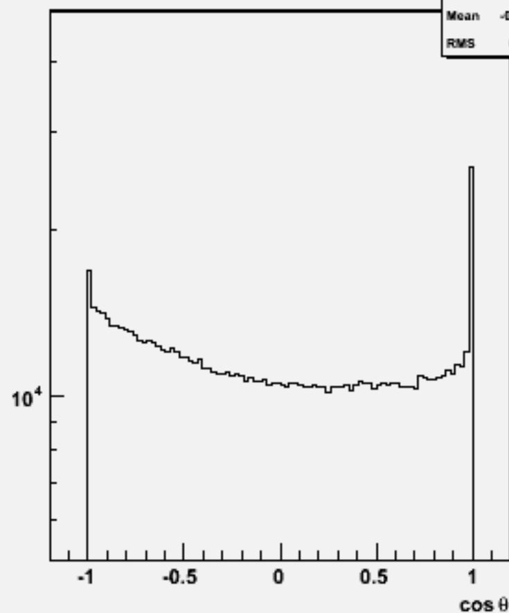
Particle cos \theta : w101278 bbcse1n1_o
