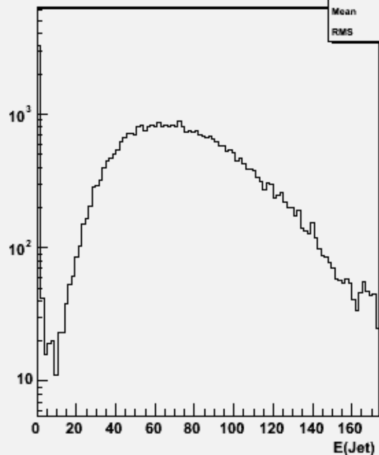
Jet energies(All jets)w101278 bbcse1n1_o
