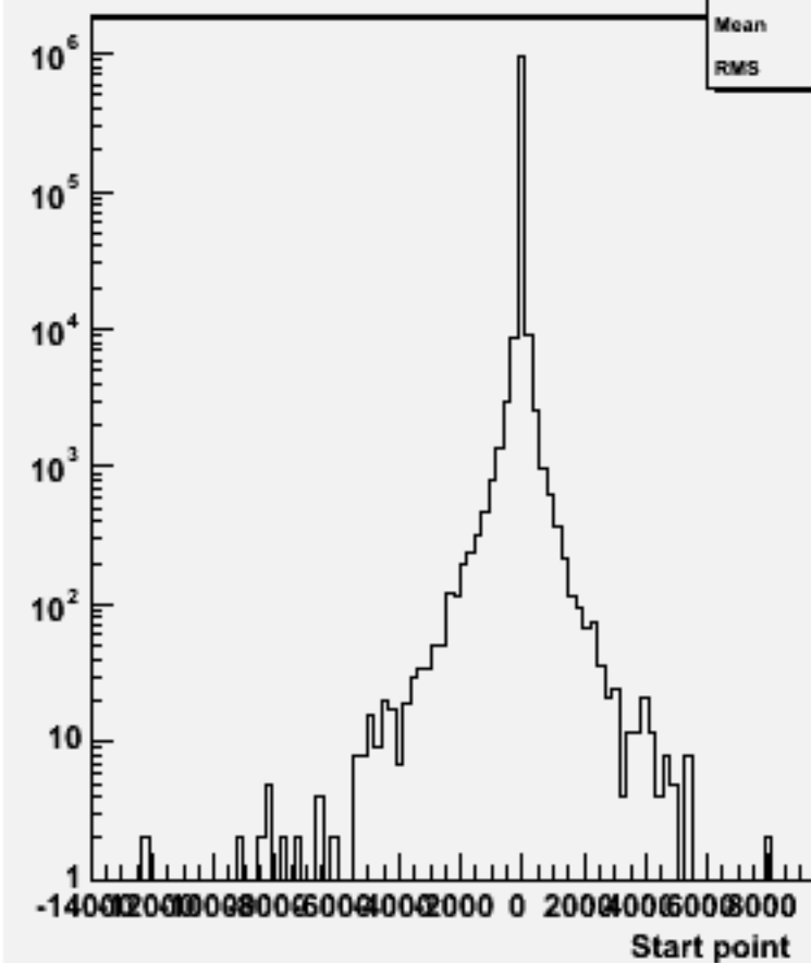
Start point Z : w101278 bbcse1n1_o
