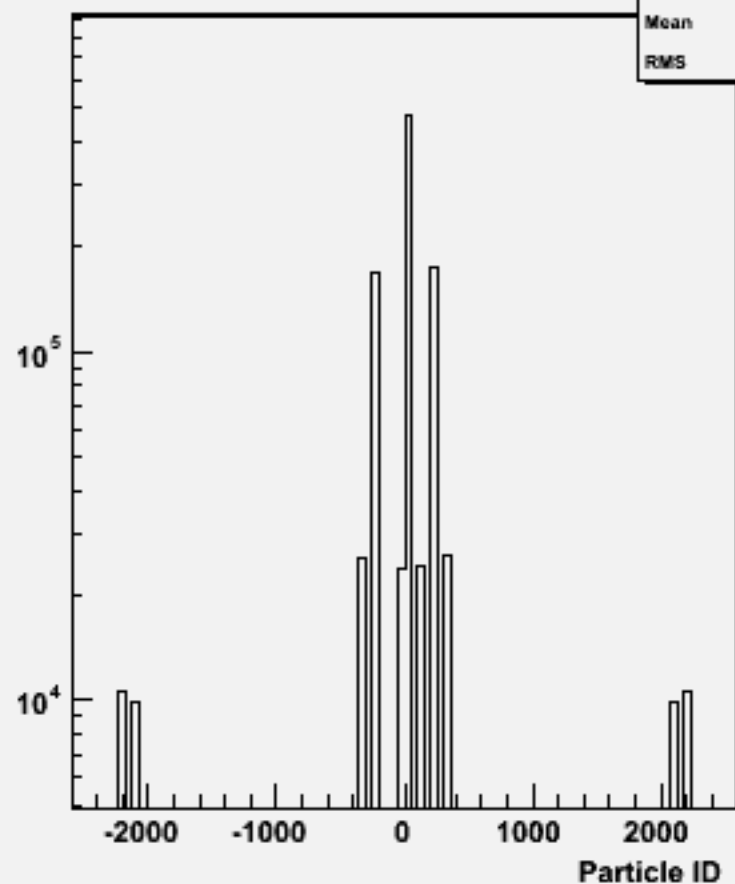
Particle ID : w101278 bbcse1n1_o
