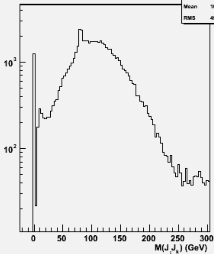
2jets mass(All comb)w101278 bbcse1n1_o
