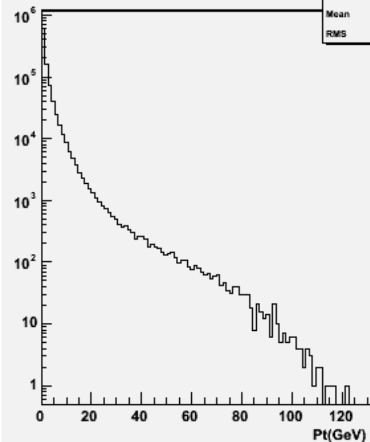
Particle Pt : w101278 bbcse1n1_o
