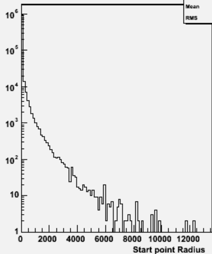
Start point R : w101278 bbcse1n1_o
