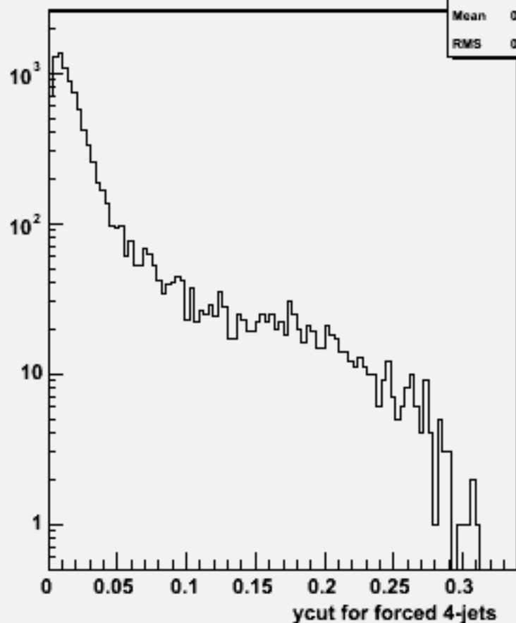
Ycut for 4-jets :w101278 bbcse1n1_o
