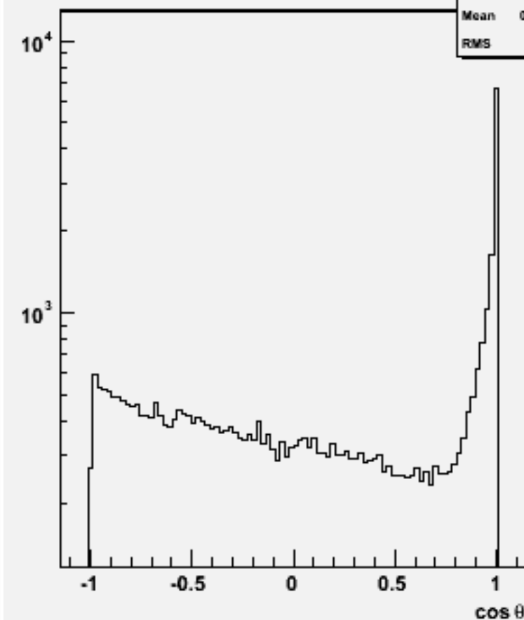
Jet cos \theta (All jets)w101278 bbcse1n1_o
