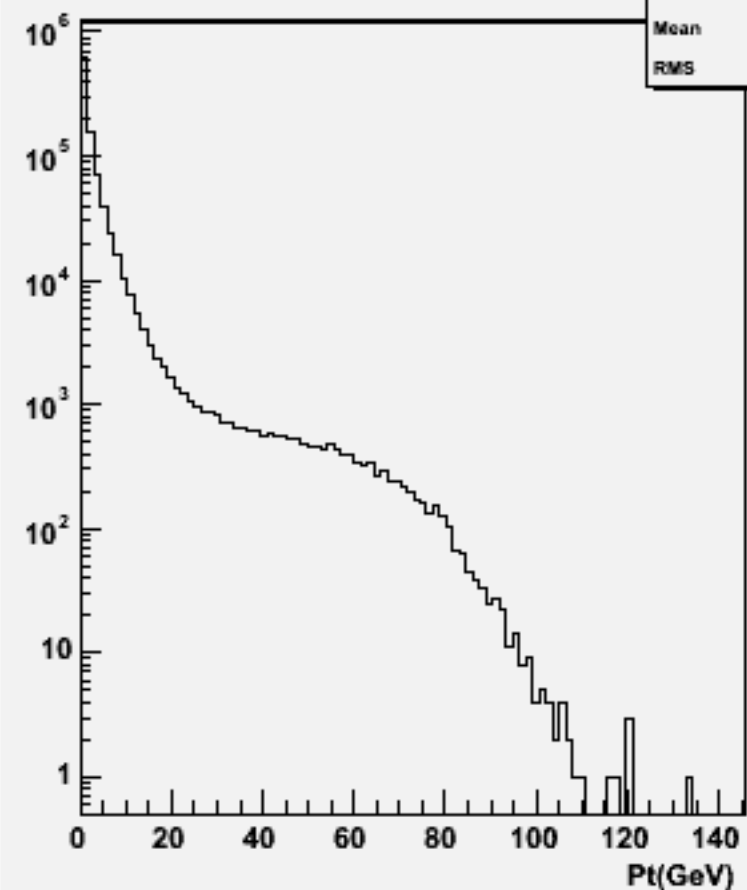
Particle Pt : w101277 bbcse1n1_o
