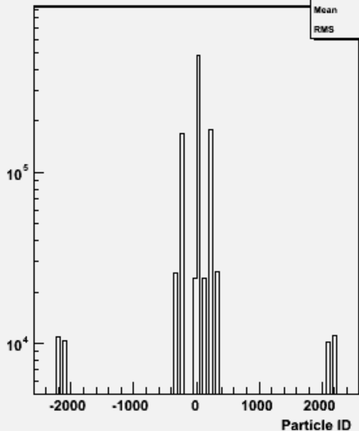
Particle ID : w101277 bbcse1n1_o
