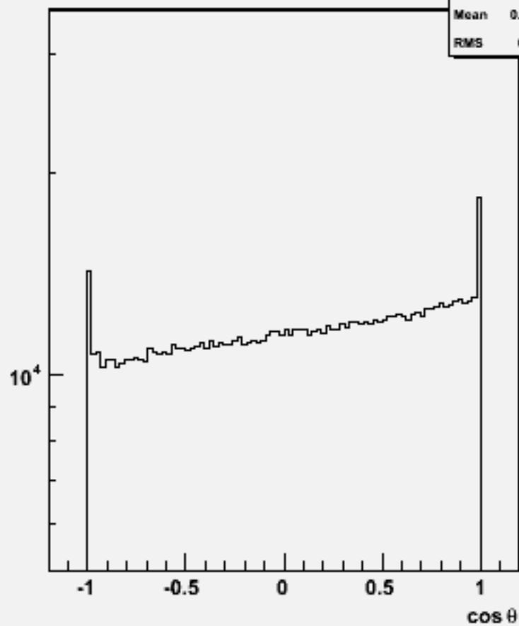
Particle \cos \theta : w101277 bbcse1n1_o
