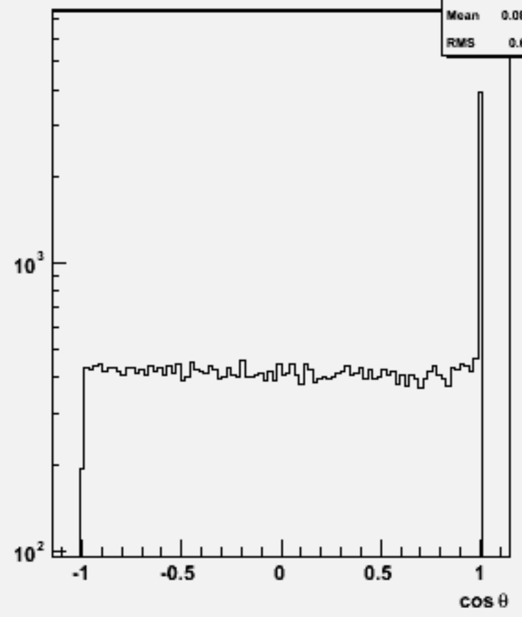
Jet cosθ (All jets)w101277 bbcse1n1_o
