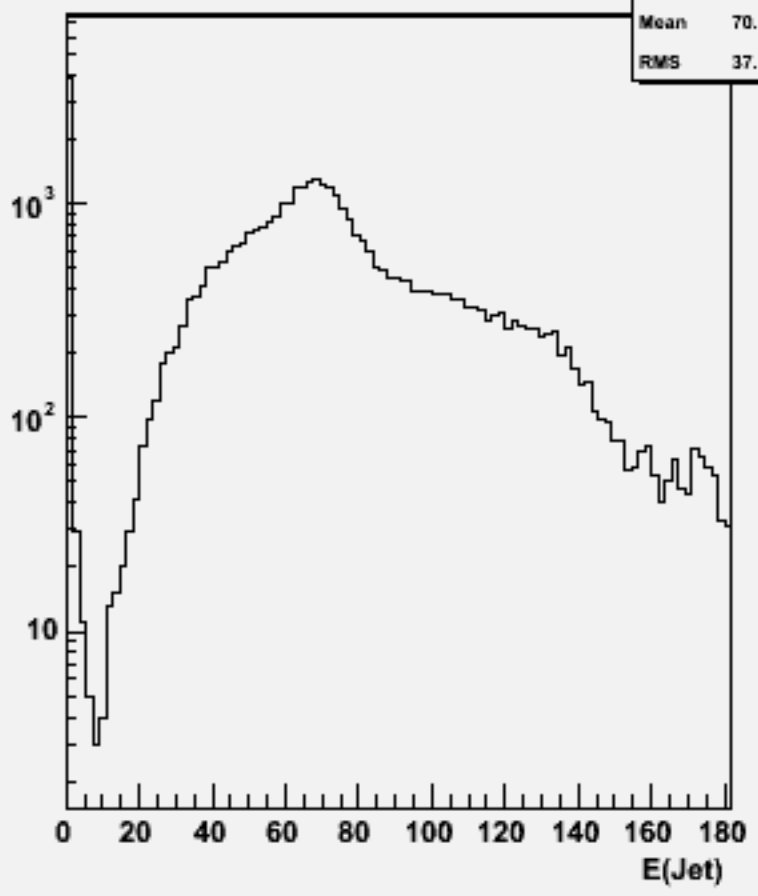
Jet energies(All jets)w101277 bbcse1n1_o
