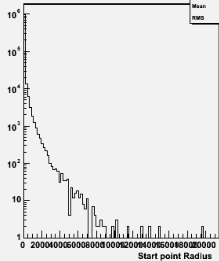
Start point R : w101277 bbcse1n1_o
