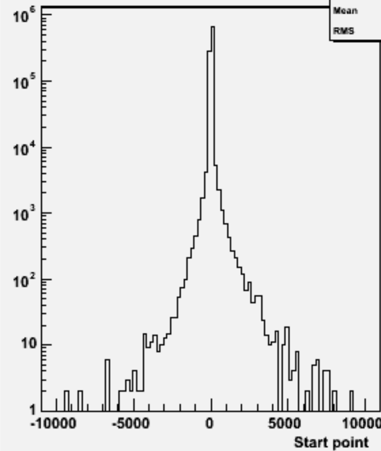
Start point Z : w101277 bbcse1n1_o
