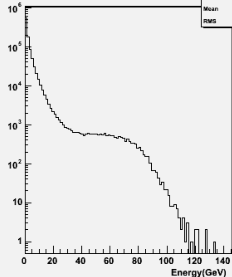
Particle Energy : w101277 bbcse1n1_o
