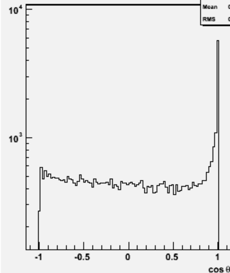
Jet cosθ (All jets)w101276 bbcse1n1_o
