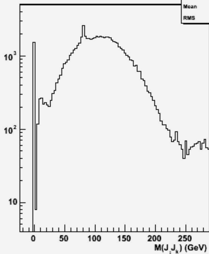
2jets mass(All comb)w101276 bbcse1n1_o
