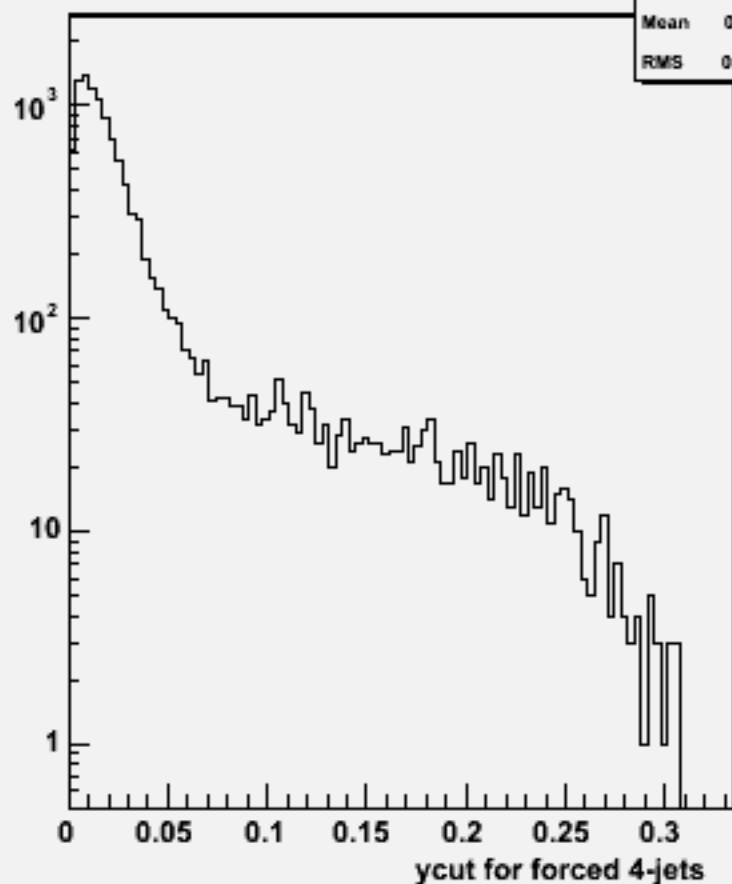
Ycut for 4-jets :w101276 bbcse1n1_o
