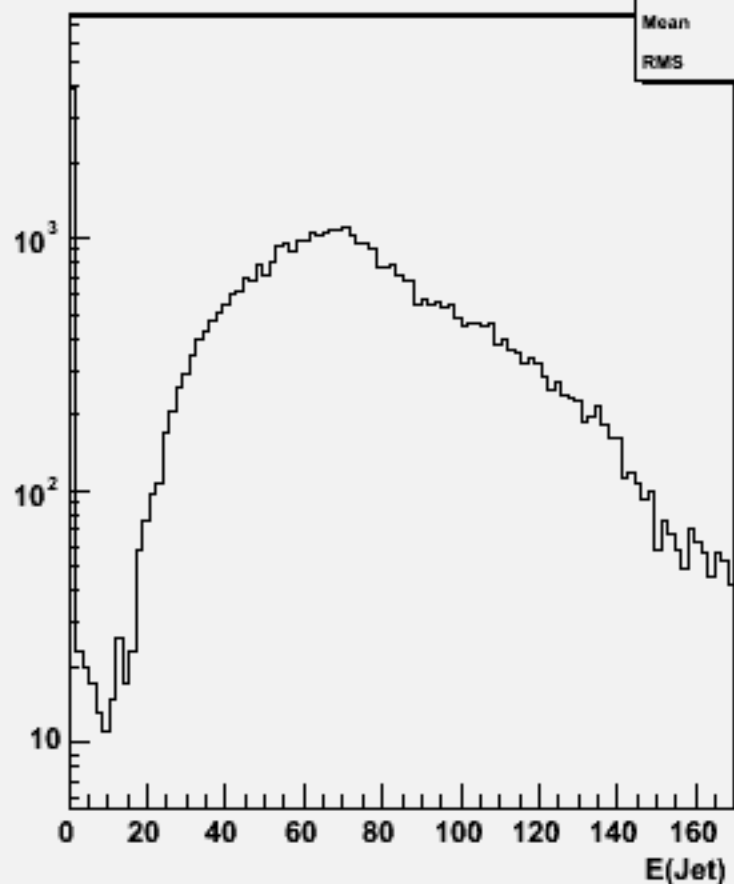
Jet energies(All jets)w101276 bbcse1n1_o
