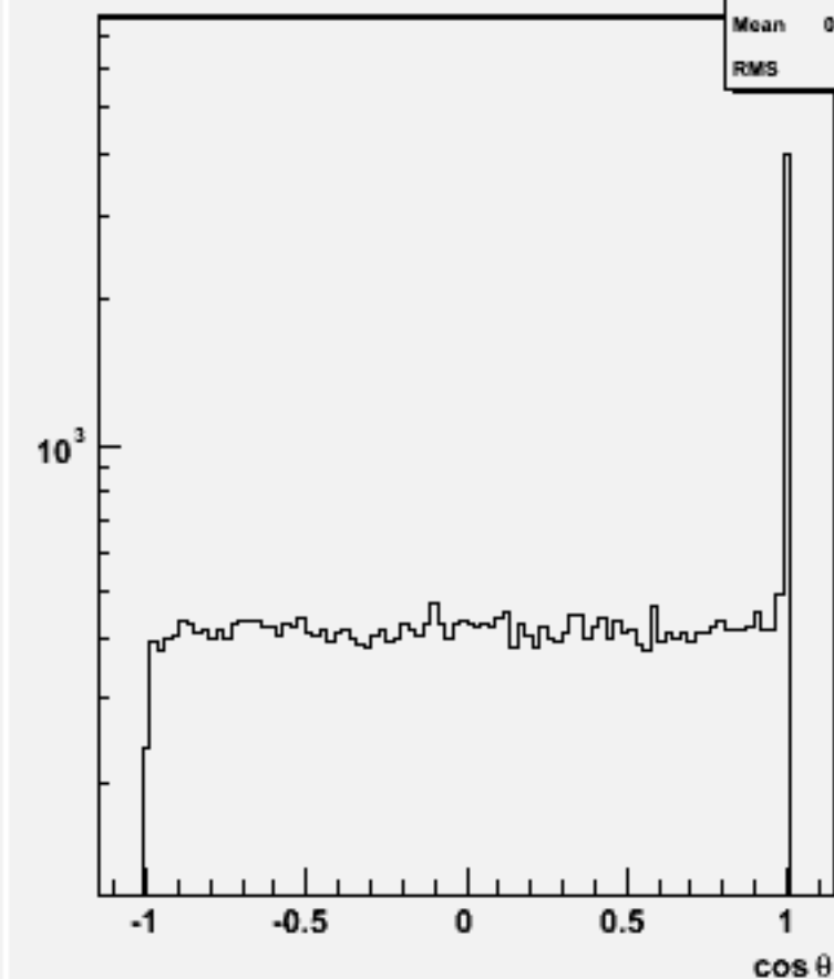
Jet cos \theta (All jets)w101273 bbudsc_o
