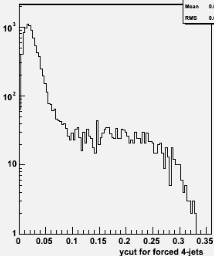
Ycut for 4-jets :w101273 bbudsc_o
