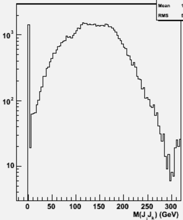
2jets mass(All comb)w101273 bbudsc_o
