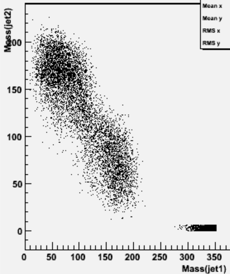
Jet mass for forced 2-jets : w101273 bbudsc_o
