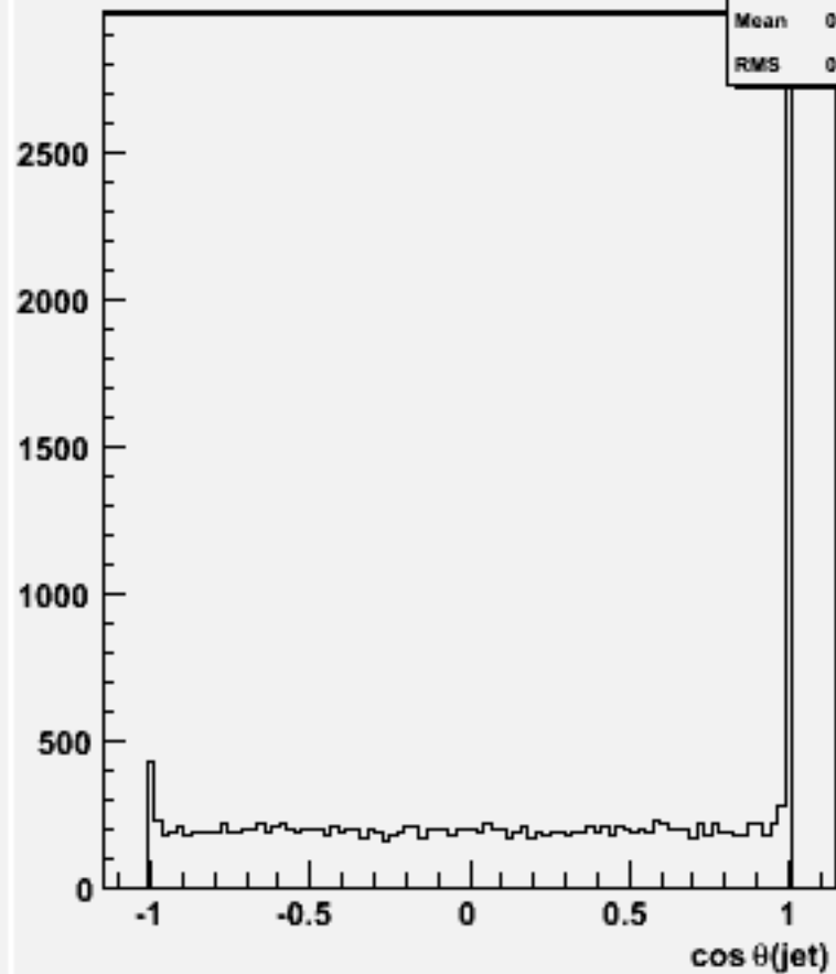
cos \Theta for 2-jets :w101273 bbudsc_o
