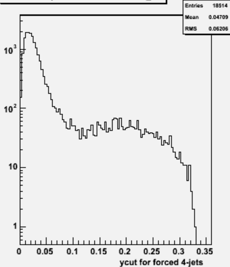
Ycut for 4-jets :w101272 bbudsc_o
