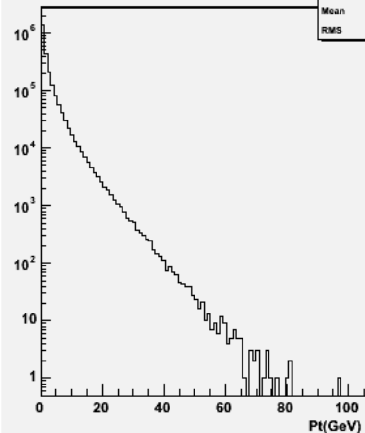
Start point Z : w101272 bbudsc_o
