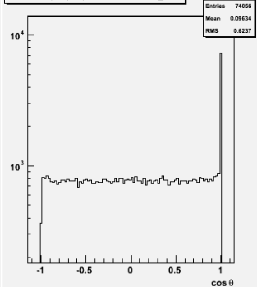
Jet cos \theta (All jets)w101272 bbudsc_o
