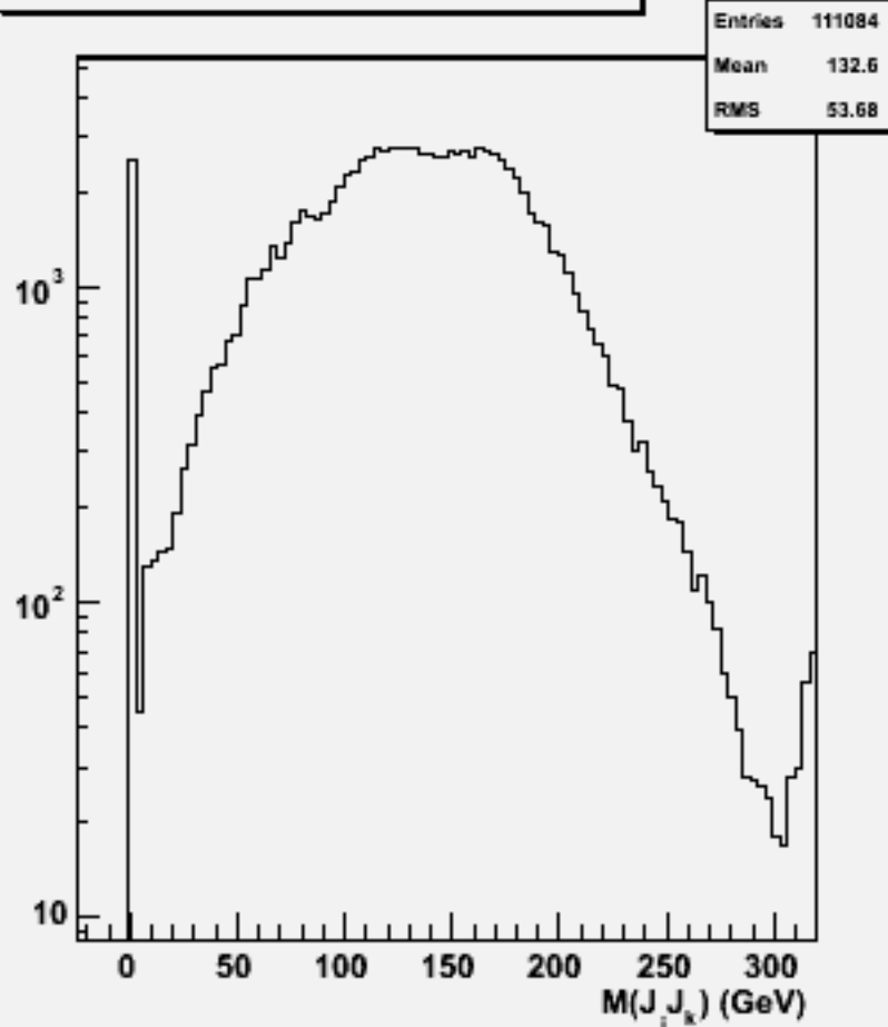
2jets mass(All comb)w101272 bbudsc_o
