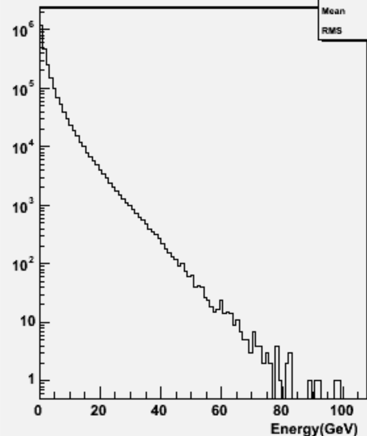
Start point R : w101272 bbudsc_o
