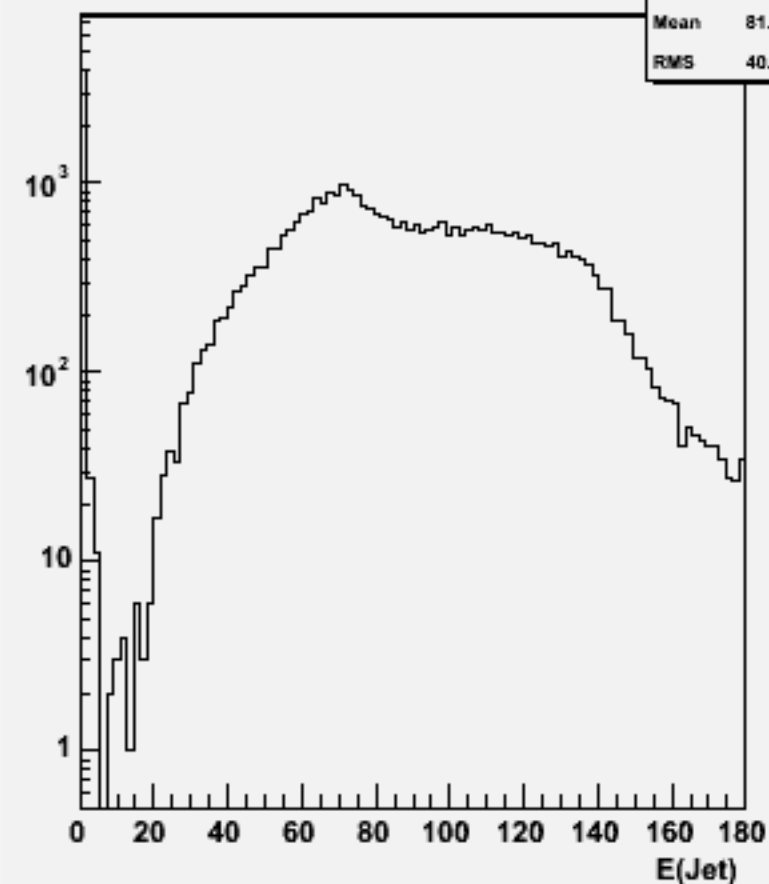
Jet energies(All jets)w101269 bbuddu_o
