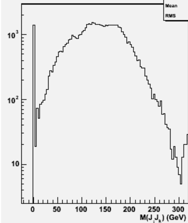
2jets mass(All comb)w101269 bbuddu_o
