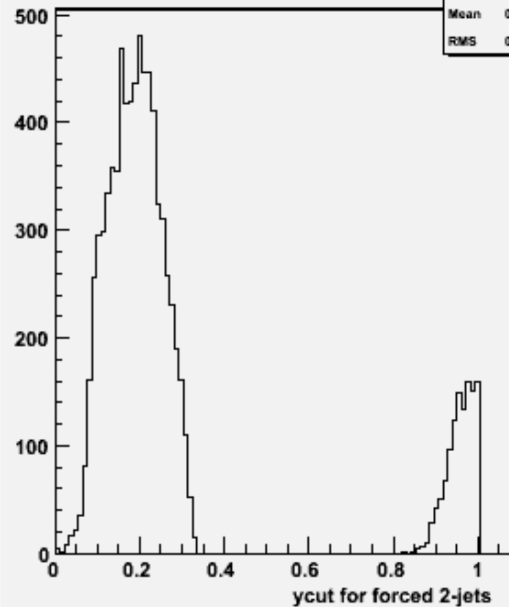
Ycut for 2-jets :w101269 bbuddu_o
