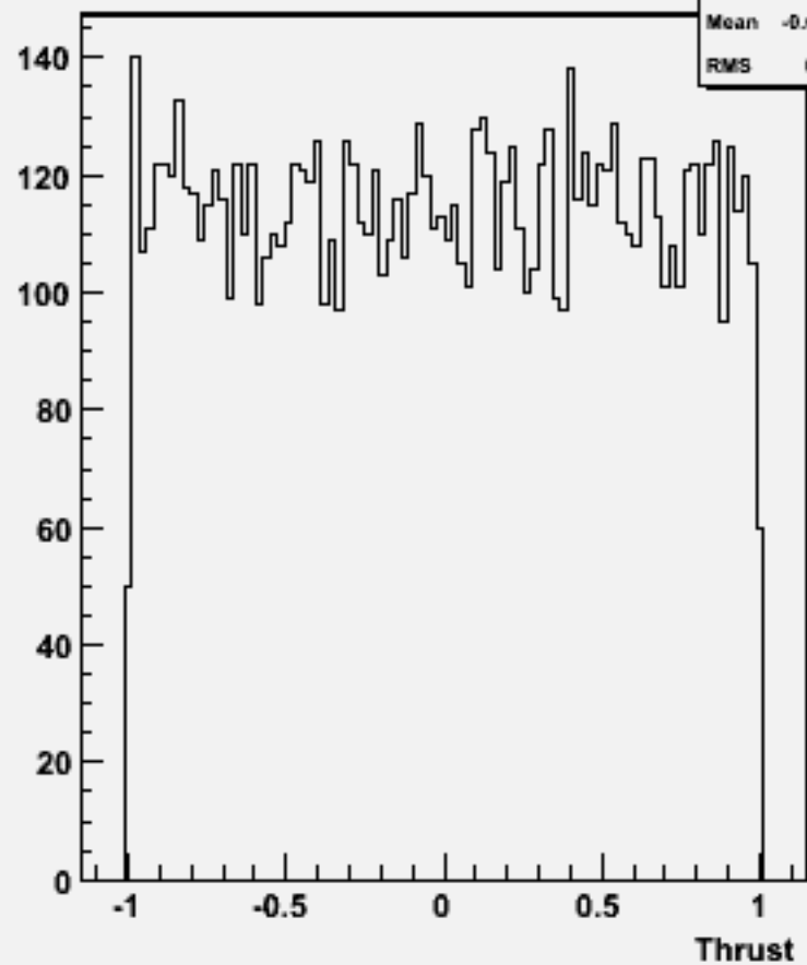
cos \Theta (thrust) w101269 bbuddu_o
