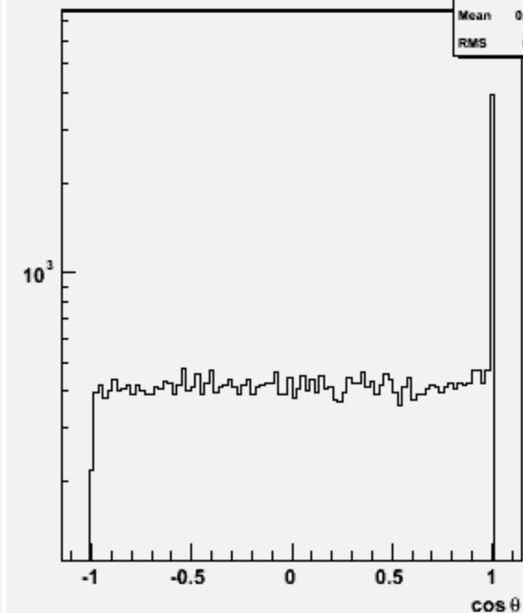
Jet cos \theta (All jets)w101269 bbuddu_o
