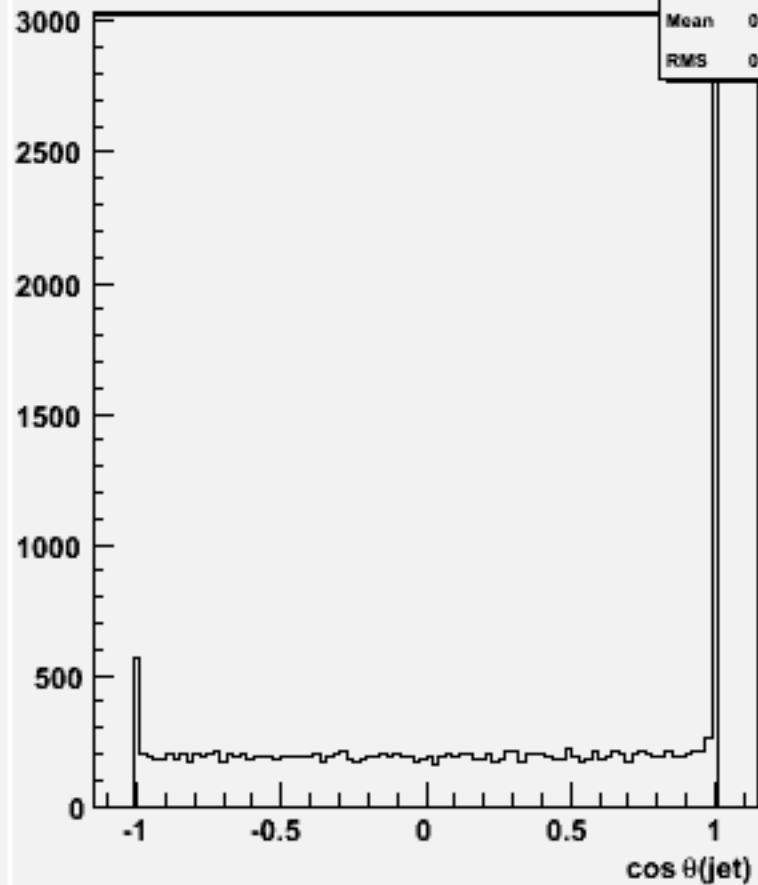
cos \Theta for 2-jets :w101269 bbuddu_o
