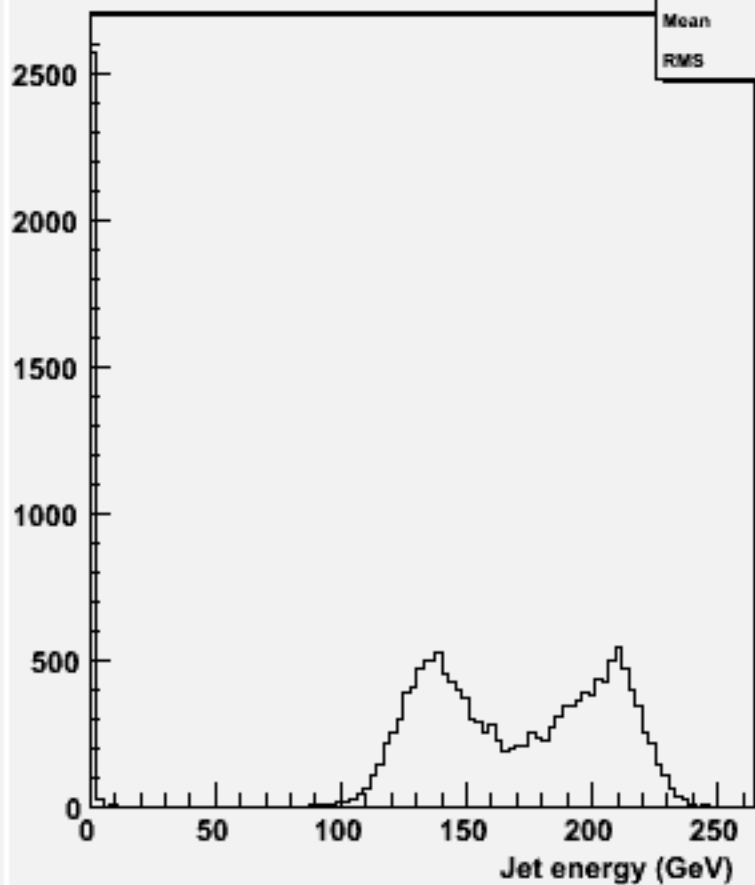
energy for 2-jets :w101269 bbuddu_o
