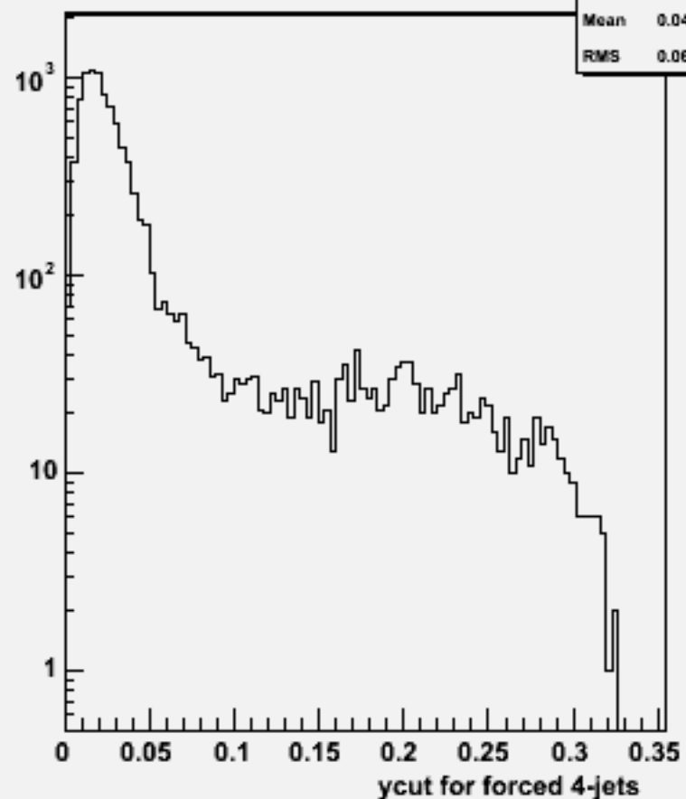
Ycut for 4-jets :w101269 bbuddu_o
