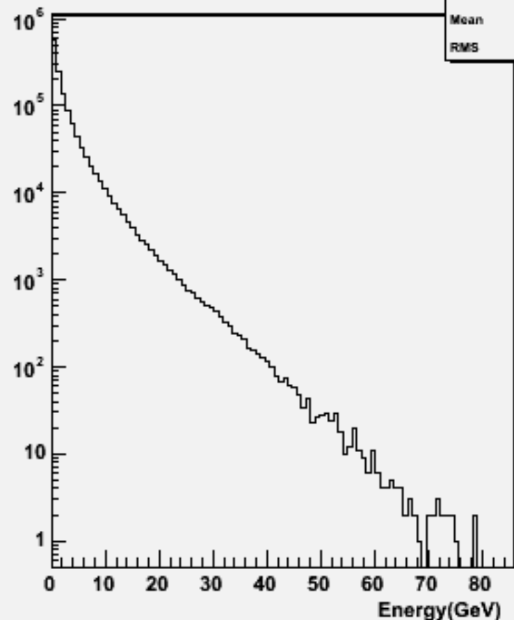
Particle Energy : w101269 bbuddu_o
