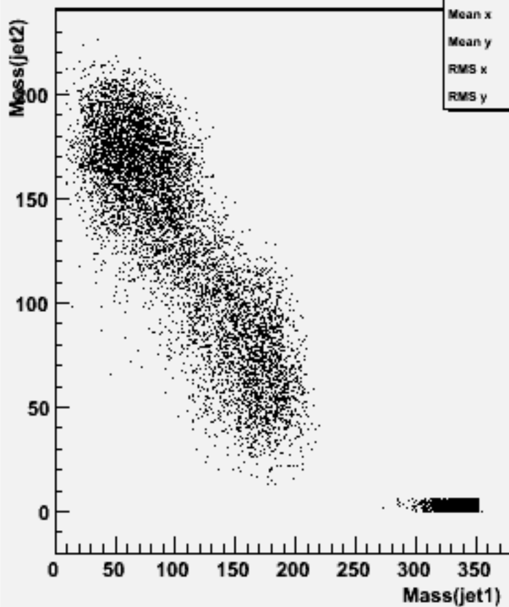
Jet mass for forced 2-jets : w101269 bbuddu_o
