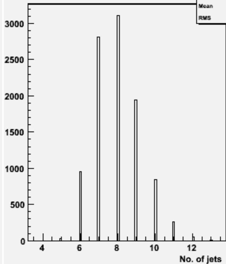
No. jets (ycut=0.001) : w101269 bbuddu_o
