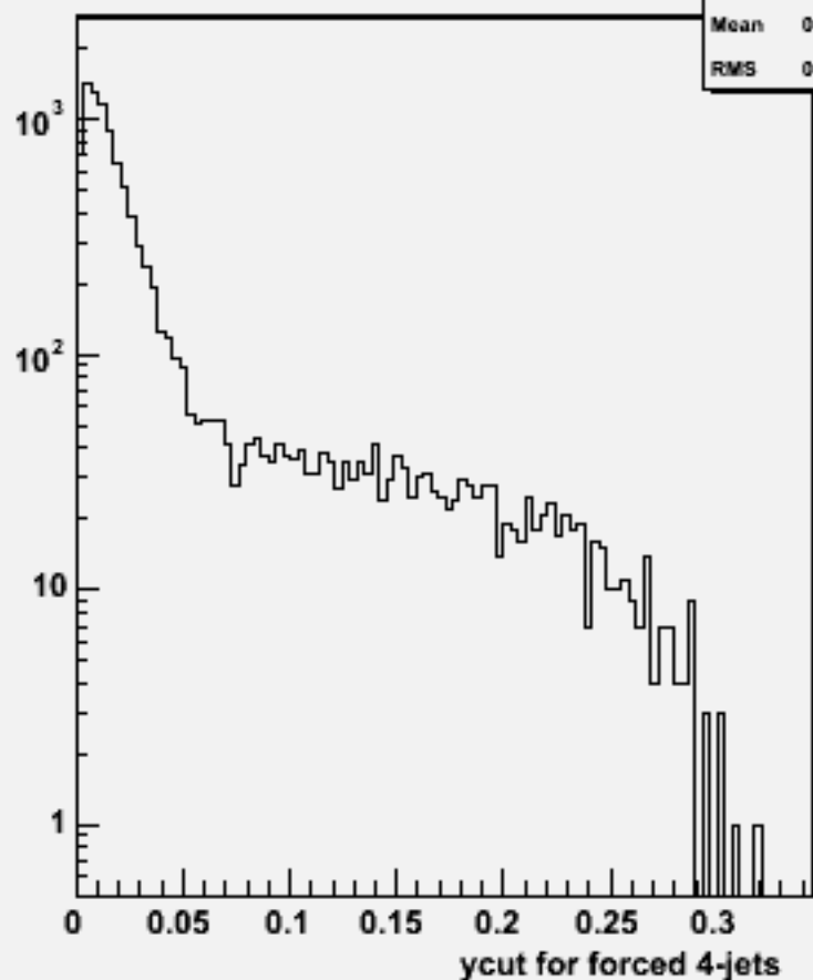
Ycut for 4-jets :w101265 bbude3n3_o
