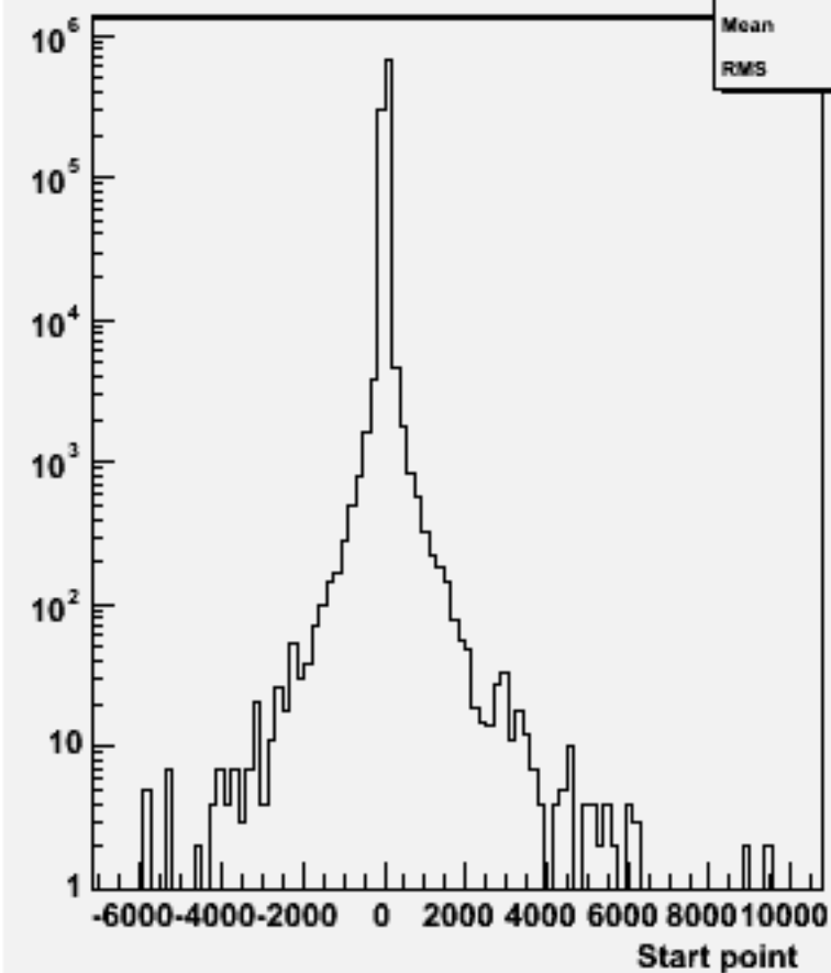
Start point Z : w101265 bbude3n3_o
