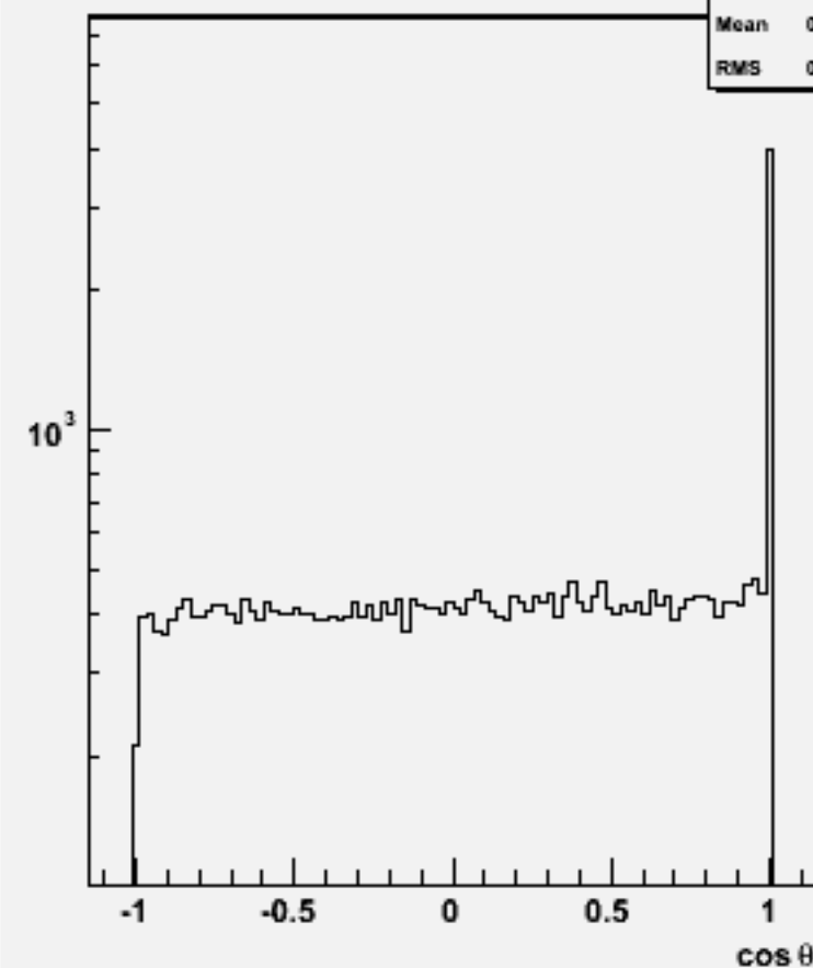
Jet cos \theta (All jets)w101265 bbude3n3_o
