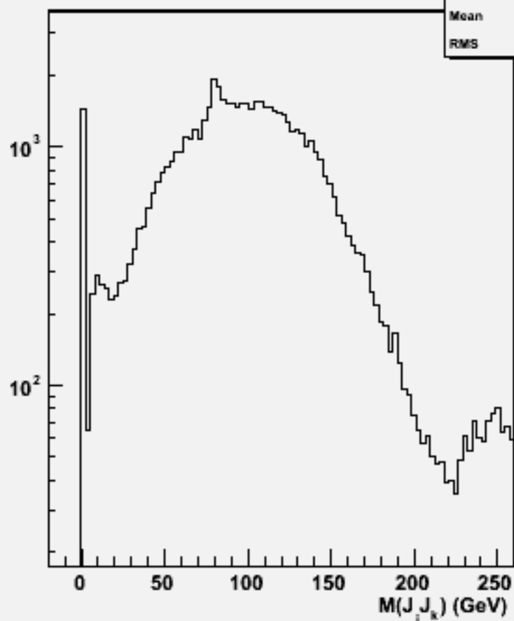
2jets mass(All comb)w101265 bbude3n3_o
