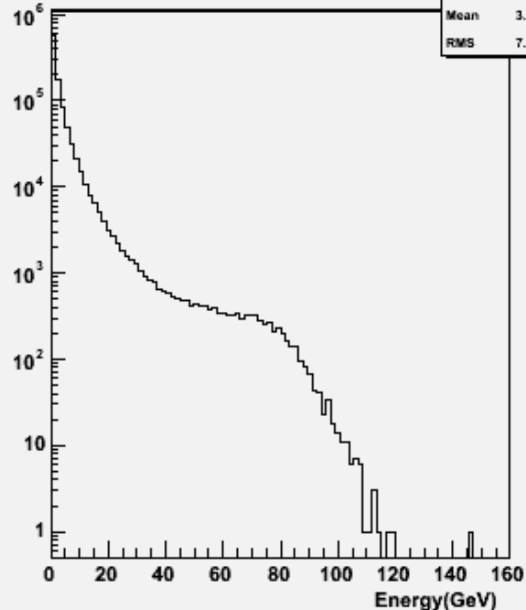
Particle Energy : w101265 bbude3n3_o
