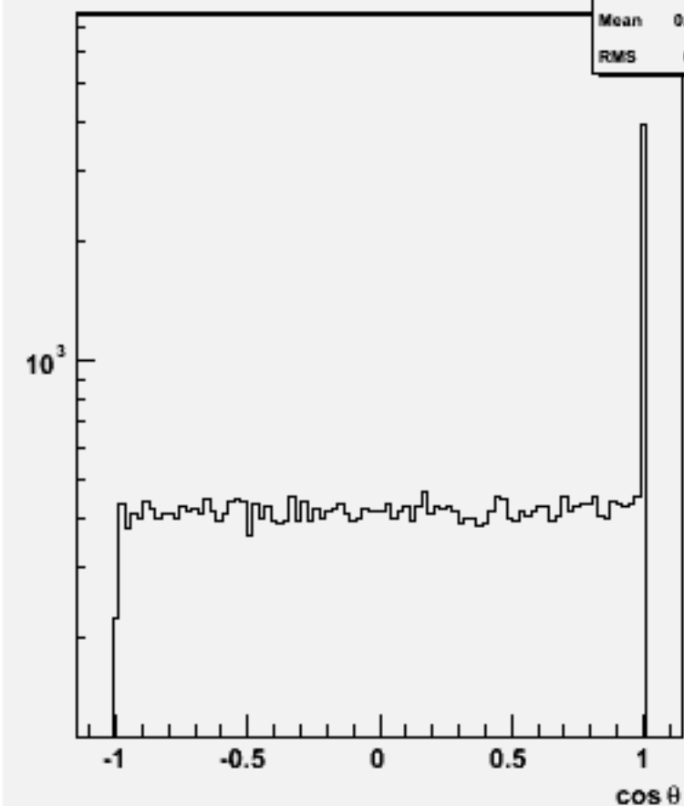
Jet cos \theta (All jets)w101264 bbude3n3_o
