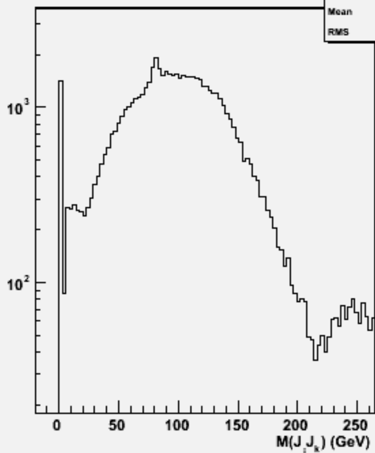
2jets mass(All comb)w101264 bbude3n3_o
