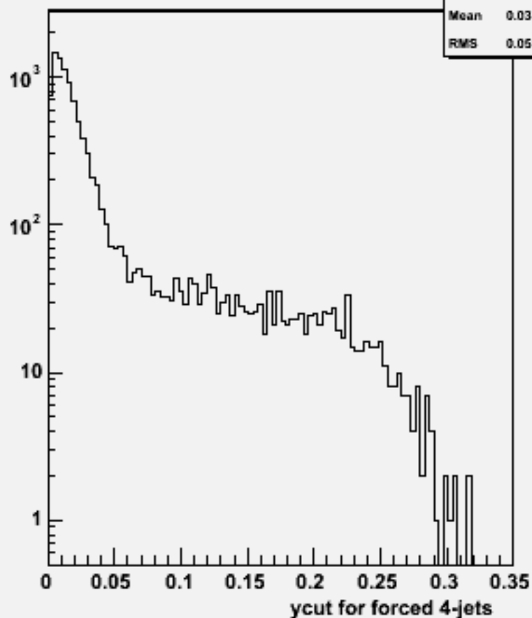
Ycut for 4-jets :w101264 bbude3n3_o
