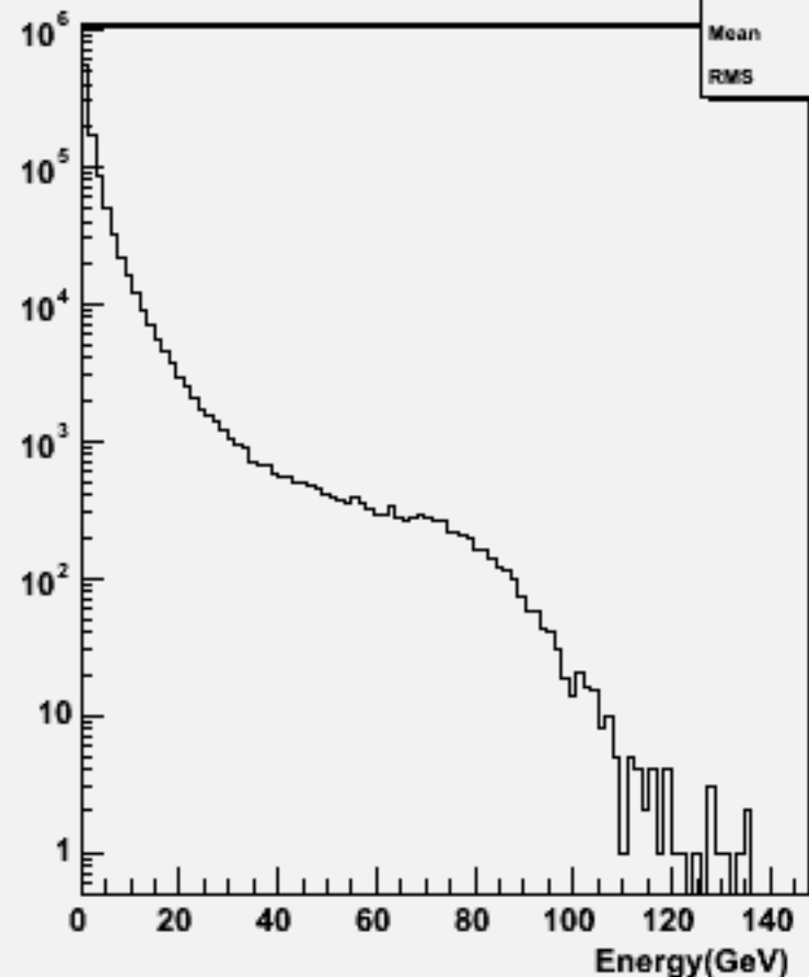
Particle Energy : w101264 bbude3n3_o
