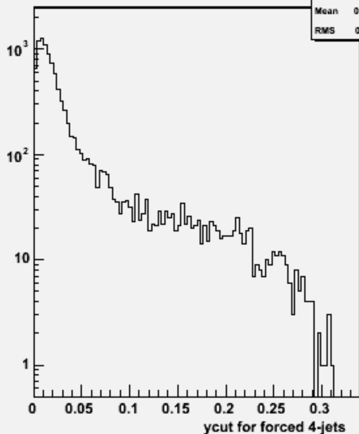
Ycut for 4-jets :w101258 bbude1n1_o
