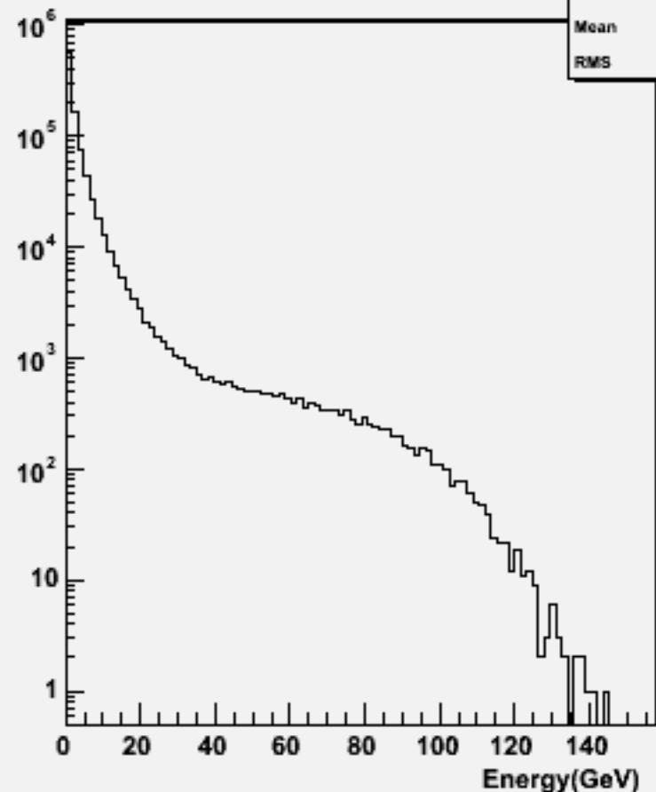
Particle Energy : w101258 bbude1n1_o
