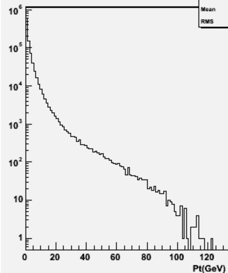
Particle Pt : w101258 bbude1n1_o
