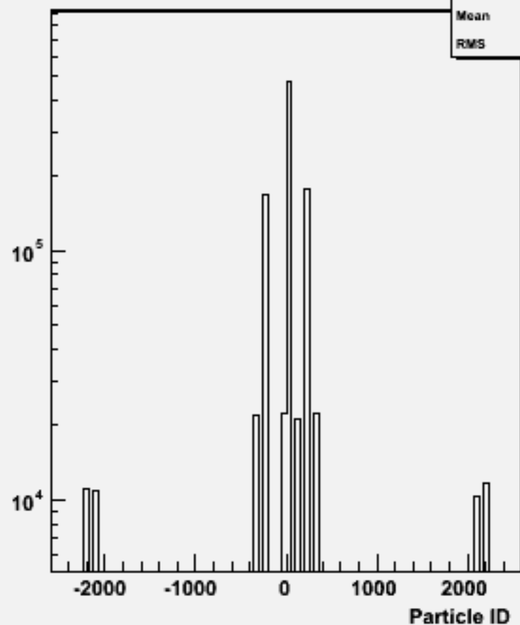
Particle ID : w101258 bbude1n1_o
