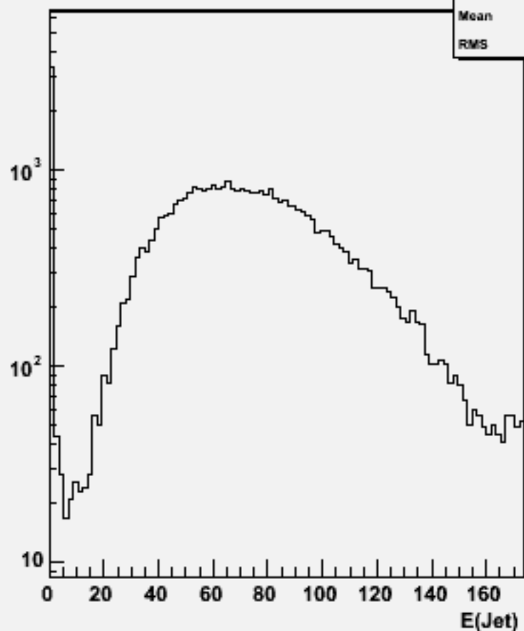
Jet energies(All jets)w101258 bbude1n1_o
