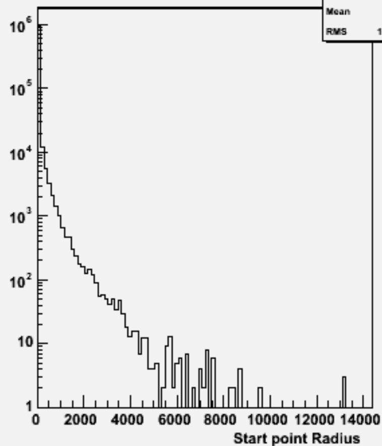
Start point R : w101258 bbude1n1_o
