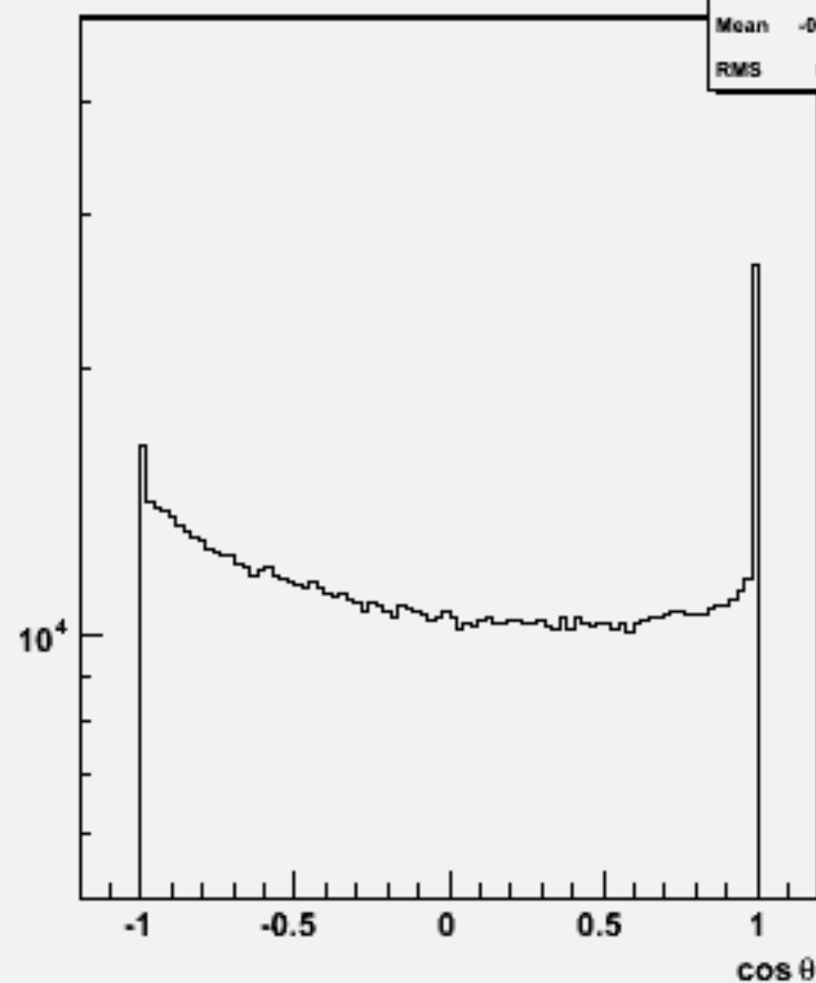
Particle cos \theta : w101258 bbude1n1_o
