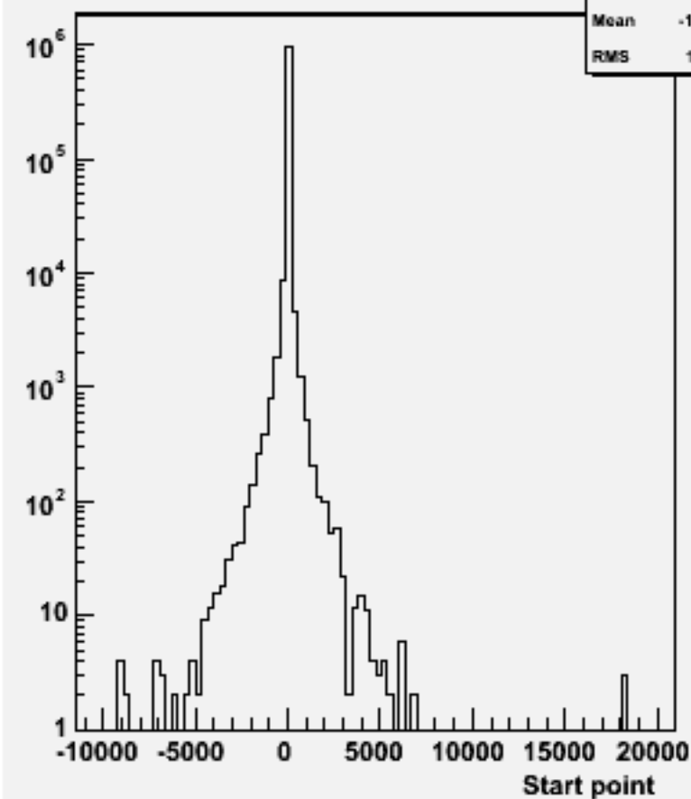
Start point Z : w101258 bbude1n1_o
