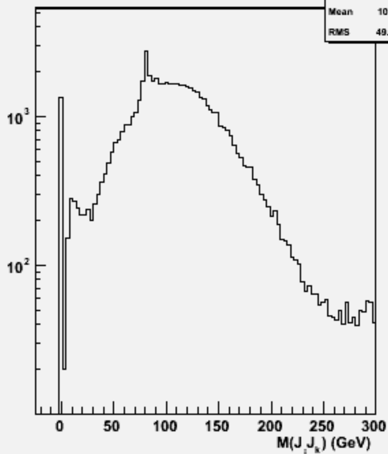
2jets mass(All comb)w101258 bbude1n1_o
