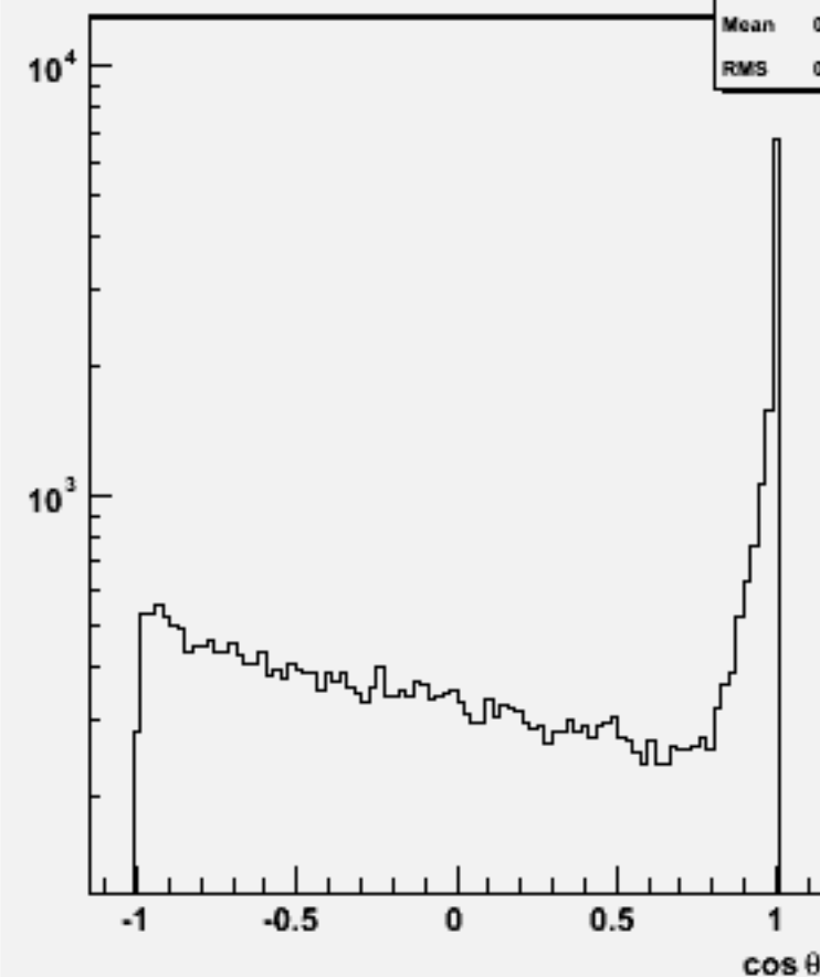
Jet cos \theta (All jets)w101258 bbude1n1_o
