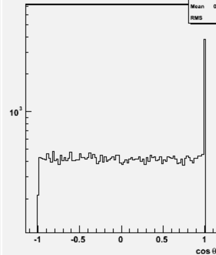
Jet cos \theta (All jets)w101257 bbude1n1_o
