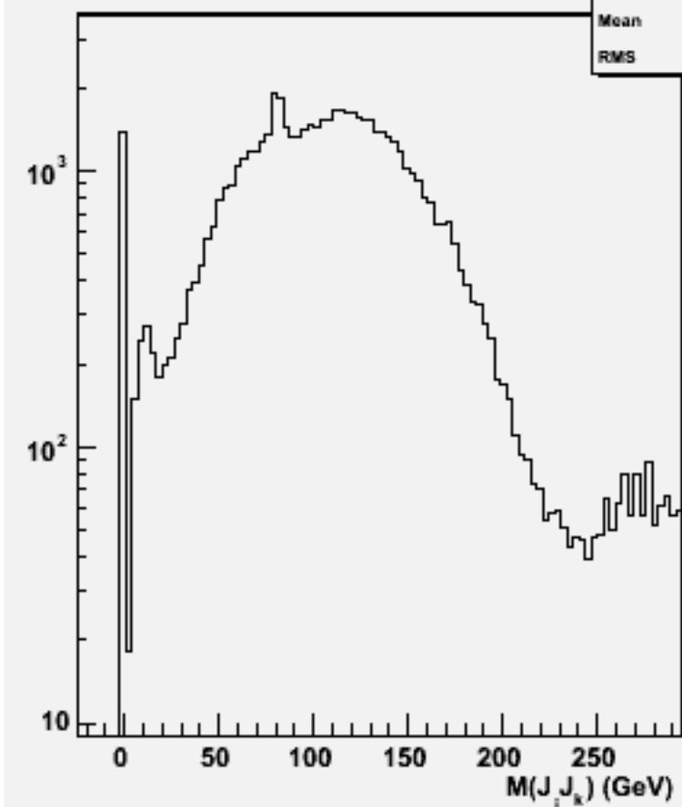
2jets mass(All comb)w101257 bbude1n1_o
