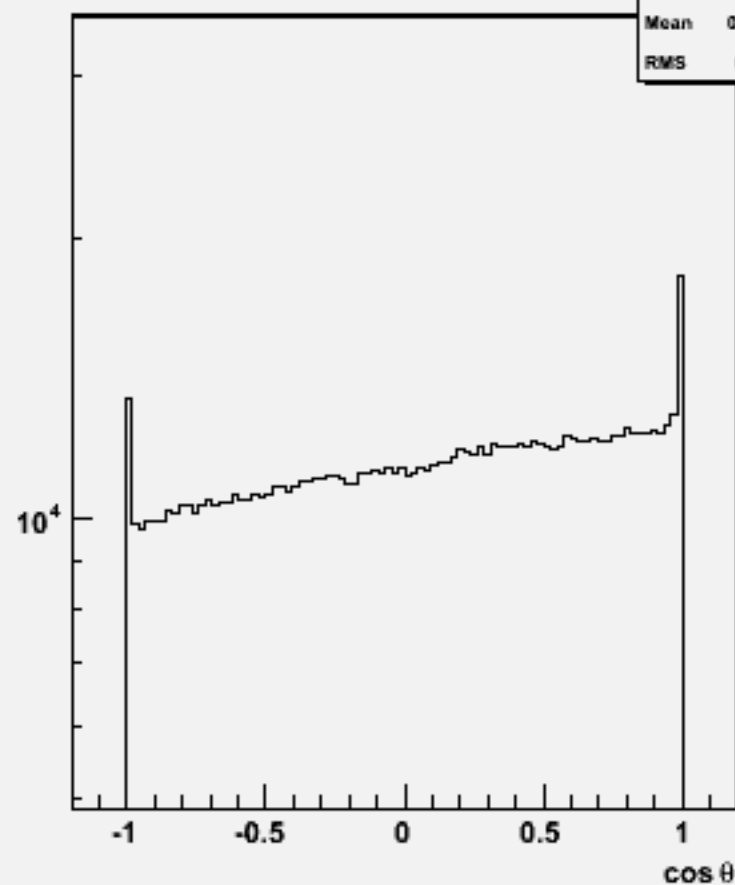
Particle cos \theta : w101257 bbude1n1_o
