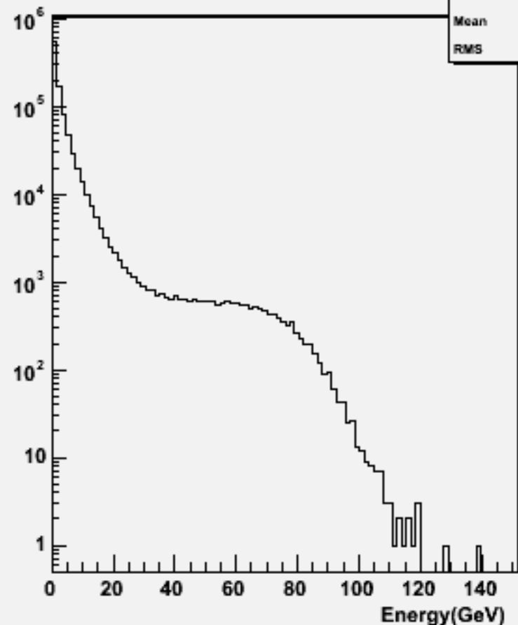
Particle Energy : w101257 bbude1n1_o
