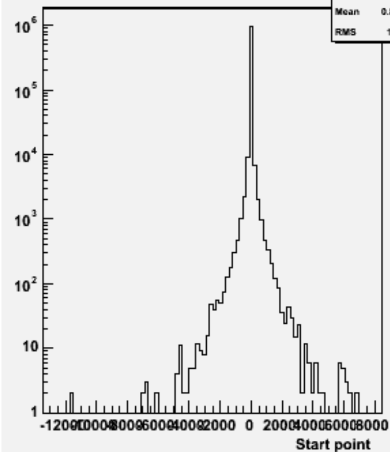
Start point Z : w101257 bbude1n1_o
