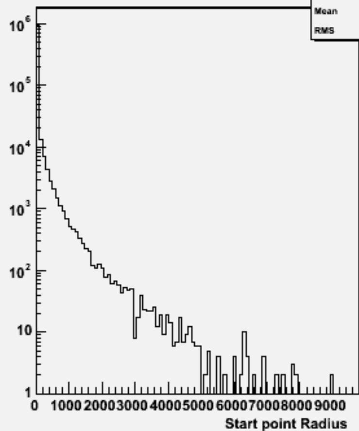
Start point R : w101257 bbude1n1_o
