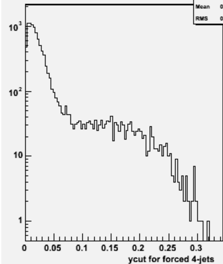
Ycut for 4-jets :w101257 bbude1n1_o
