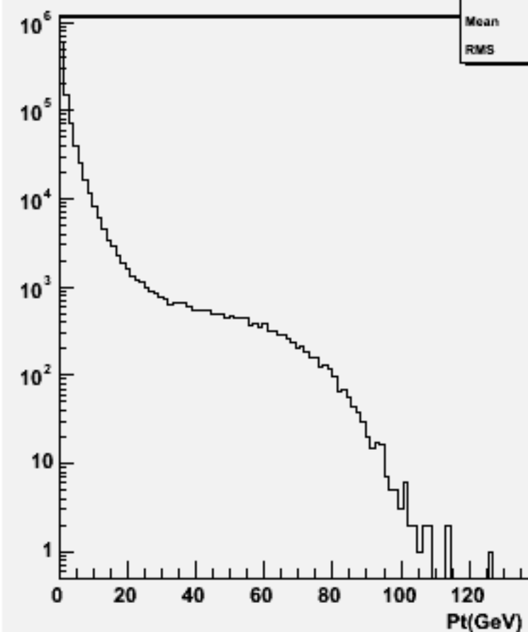
Particle Pt : w101257 bbude1n1_o
