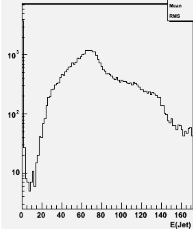
Jet energies(All jets)w101257 bbude1n1_o
