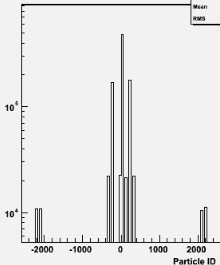
Particle ID : w101257 bbude1n1_o
