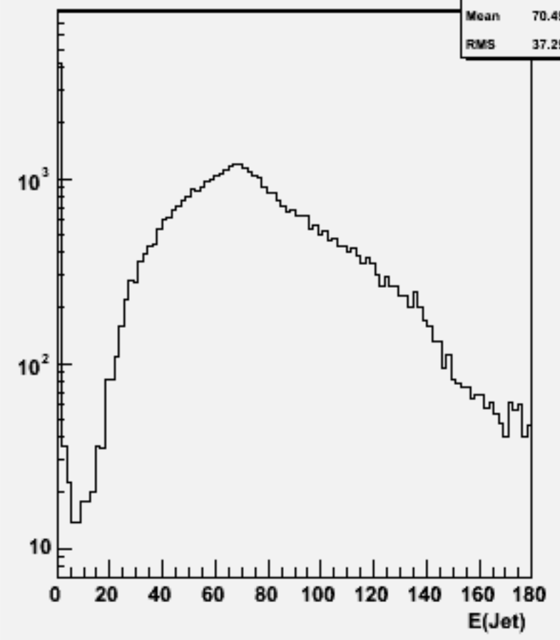
Jet energies(All jets)w101256 bbude1n1_o
