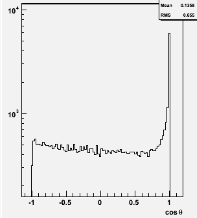
Jet cosθ (All jets)w101256 bbude1n1_o
