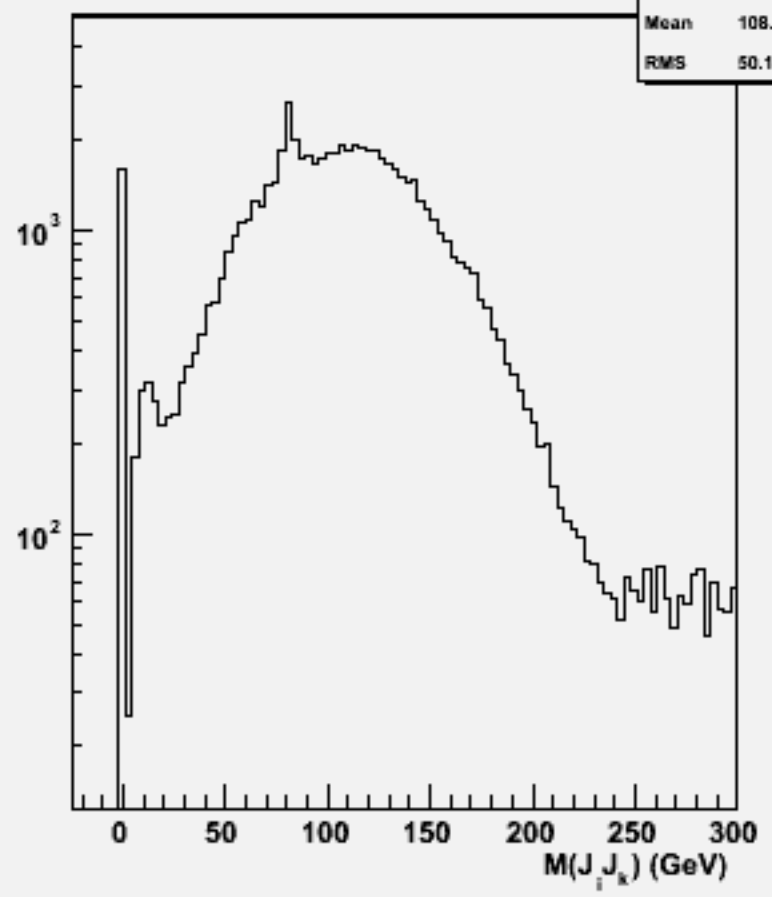
2jets mass(All comb)w101256 bbude1n1_o
