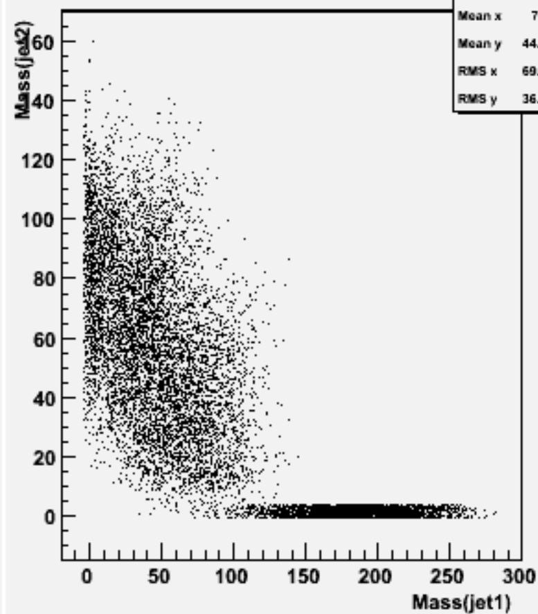
Jet mass for forced 2-jets : w101241 bbn3e3e2n2_o
