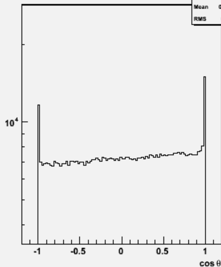
Particle cos \theta : w101241 bbn3e3e2n2_o
