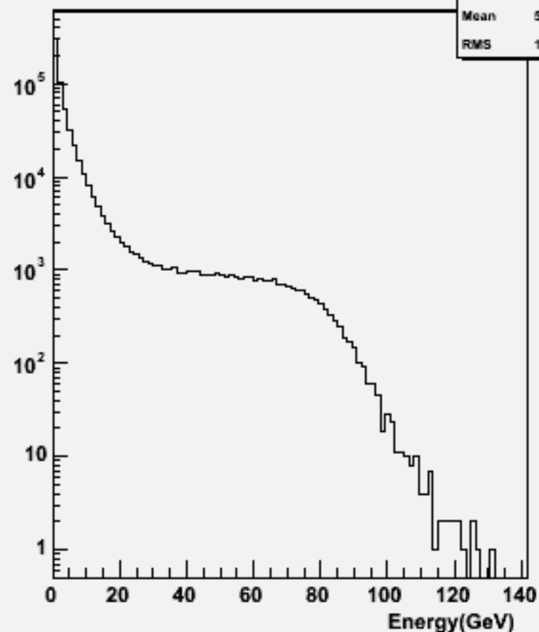
Particle Energy : w101241 bbn3e3e2n2_o
