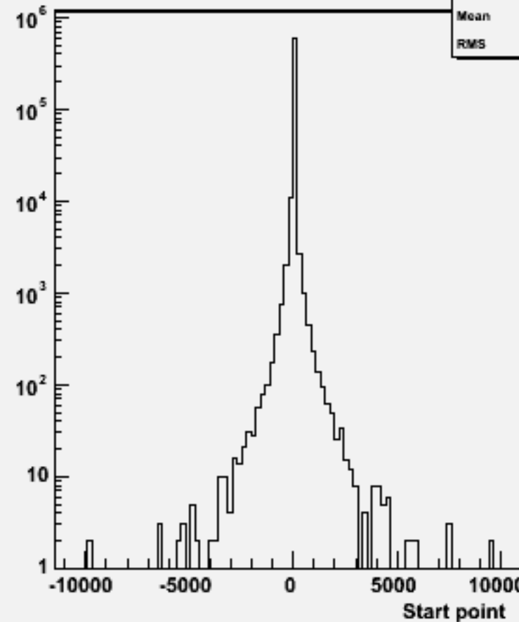
Start point Z : w101241 bbn3e3e2n2_o
