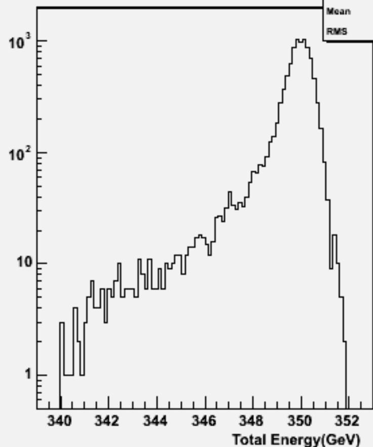
Pz Sum: w101241 bbn3e3e2n2_o
