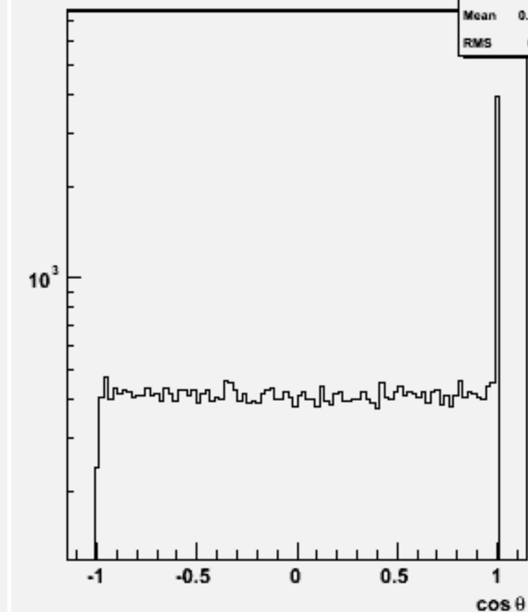
Jet cos \theta (All jets)w101241 bbn3e3e2n2_o
