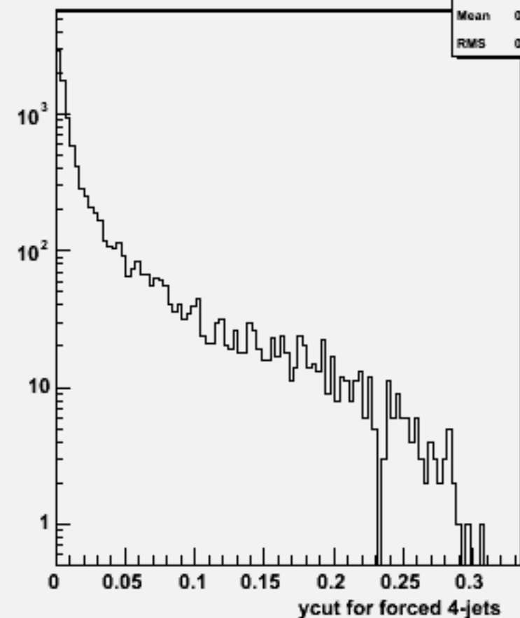
Ycut for 4-jets :w101241 bbn3e3e2n2_o
