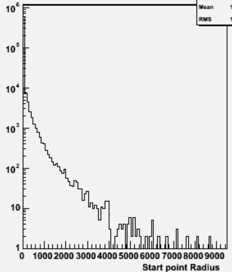
Start point R : w101241 bbn3e3e2n2_o
