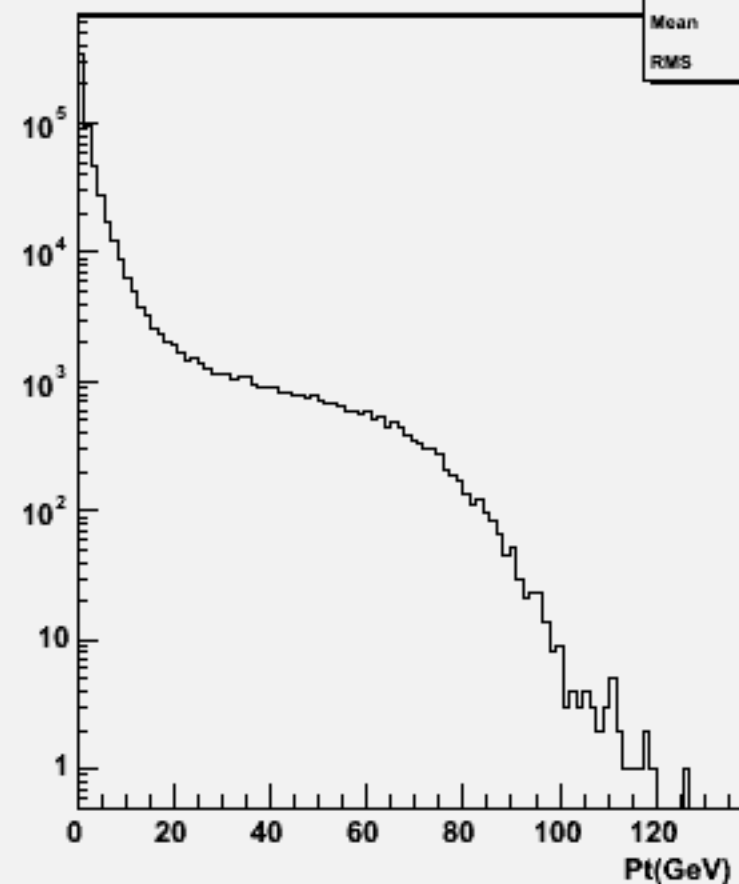
Particle Pt : w101241 bbn3e3e2n2_o
