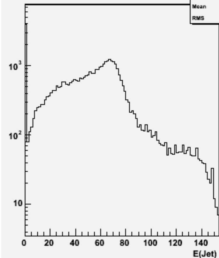
Jet energies(All jets)w101241 bbn3e3e2n2_o
