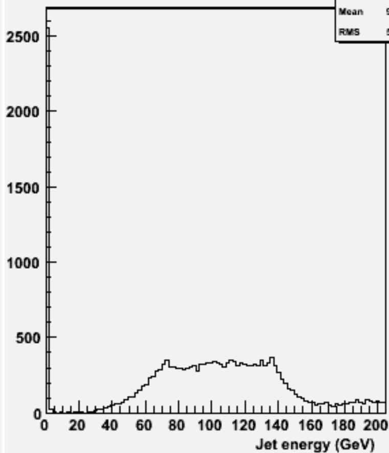
energy for 2-jets :w101241 bbn3e3e2n2_o
