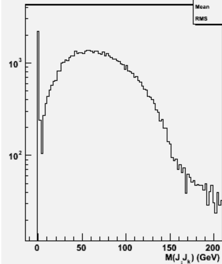
2jets mass(All comb)w101241 bbn3e3e2n2_o
