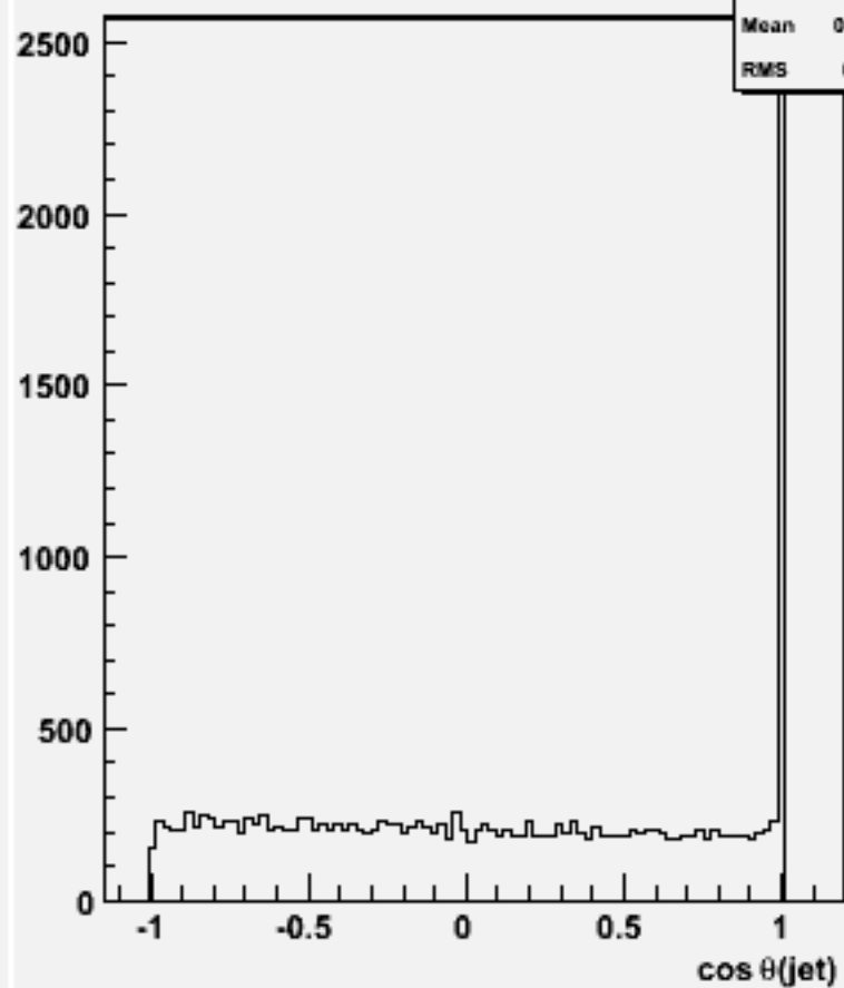
cos \theta for 2-jets :w101241 bbn3e3e2n2_o
