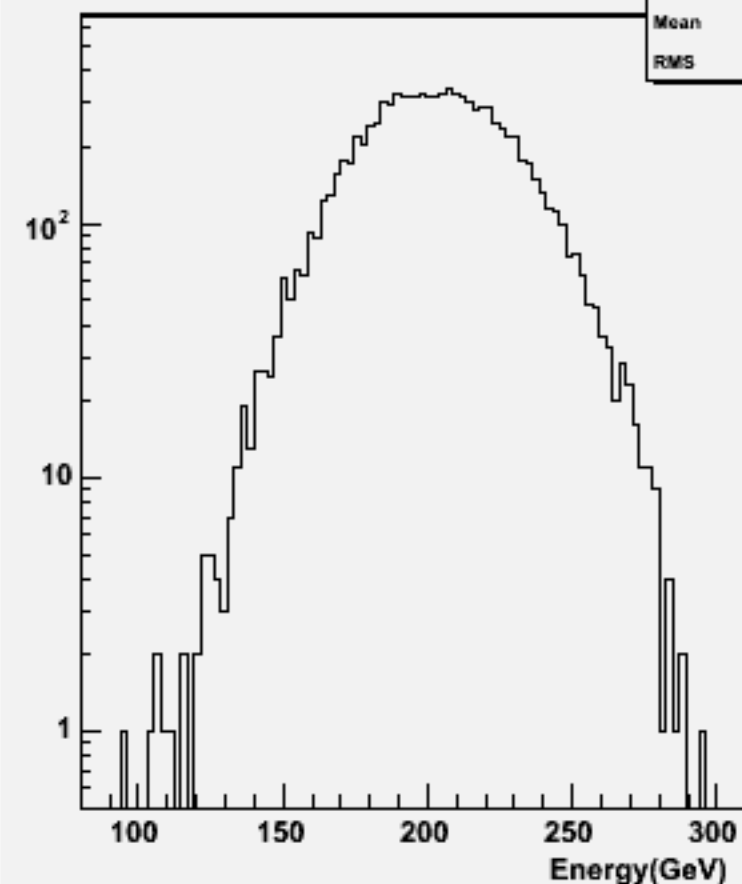
Thrust w101241 bbn3e3e2n2_o
