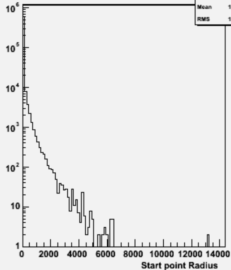
Start point R : w101240 bbn3e3e2n2_o
