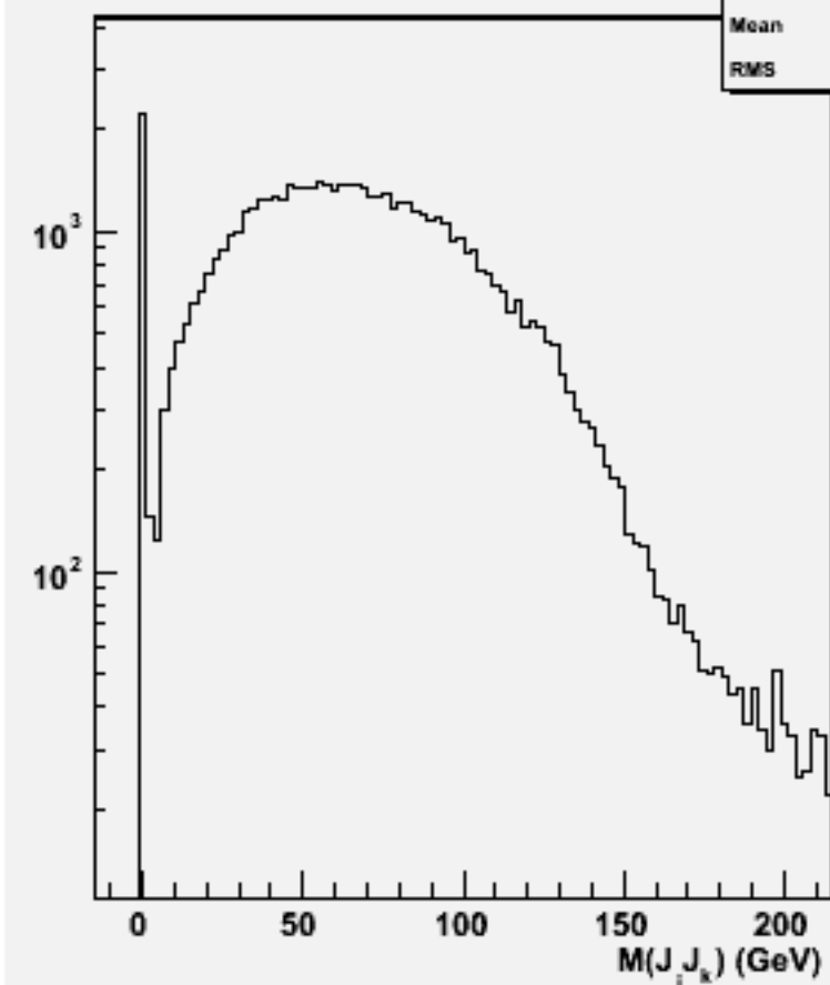
2jets mass(All comb)w101240 bbn3e3e2n2_o
