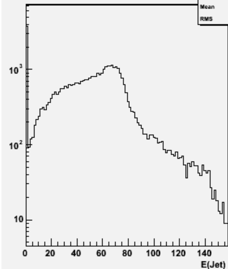
Jet energies(All jets)w101240 bbn3e3e2n2_o
