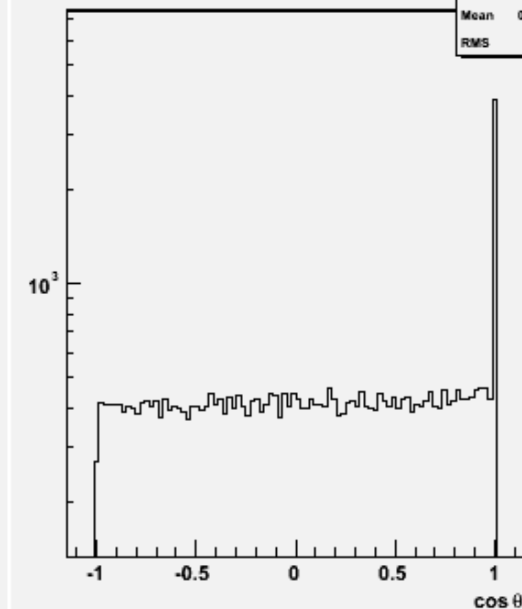
Jet cos \theta (All jets)w101240 bbn3e3e2n2_o
