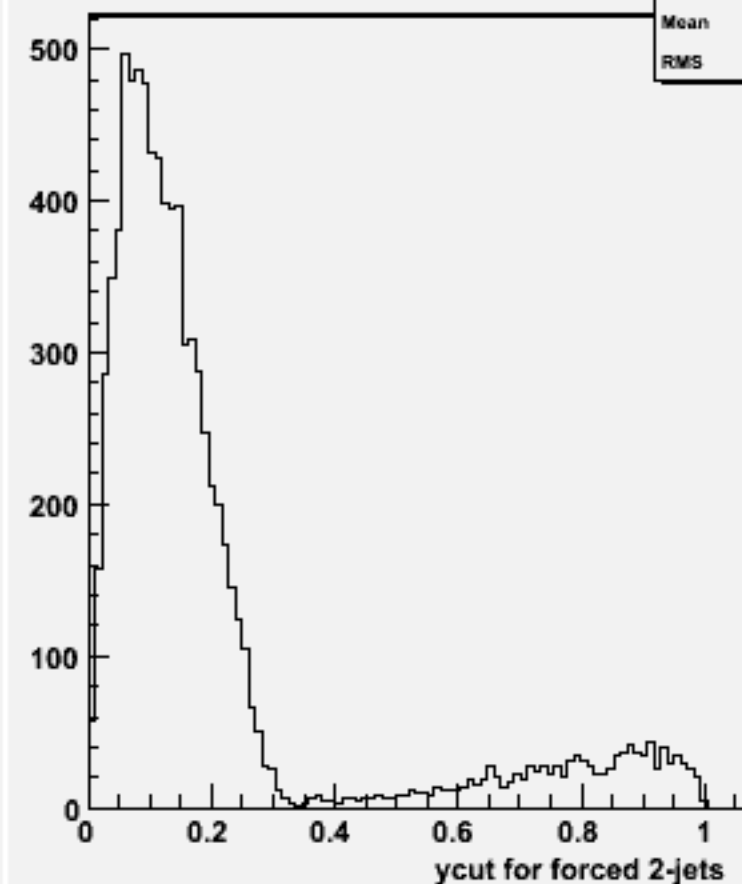
Ycut for 2-jets :w101240 bbn3e3e2n2_o
