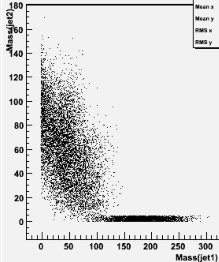
Jet mass for forced 2-jets : w101240 bbn3e3e2n2_o
