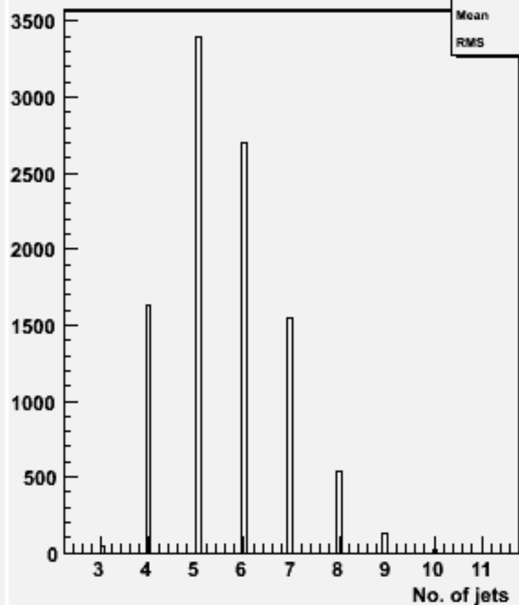
No. jets (ycut=0.001) : w101240 bbn3e3e2n2_o
