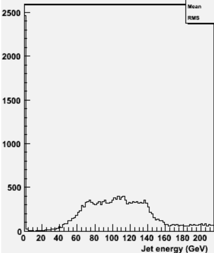
energy for 2-jets :w101240 bbn3e3e2n2_o
