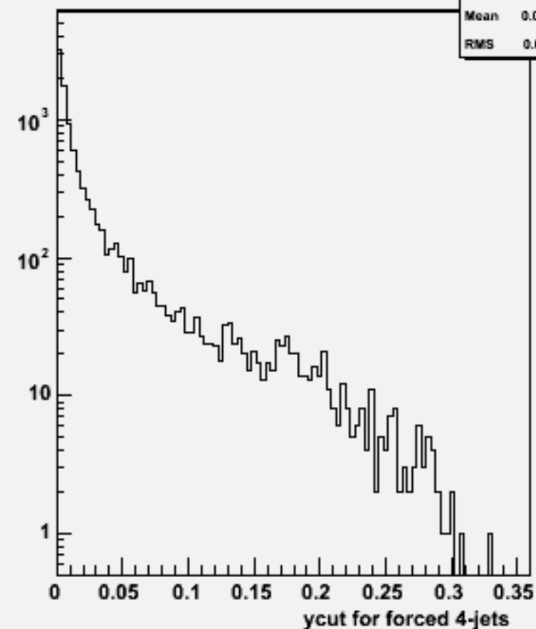
Ycut for 4-jets :w101240 bbn3e3e2n2_o
