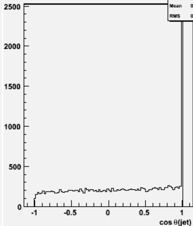
cos \theta for 2-jets :w101240 bbn3e3e2n2_o
