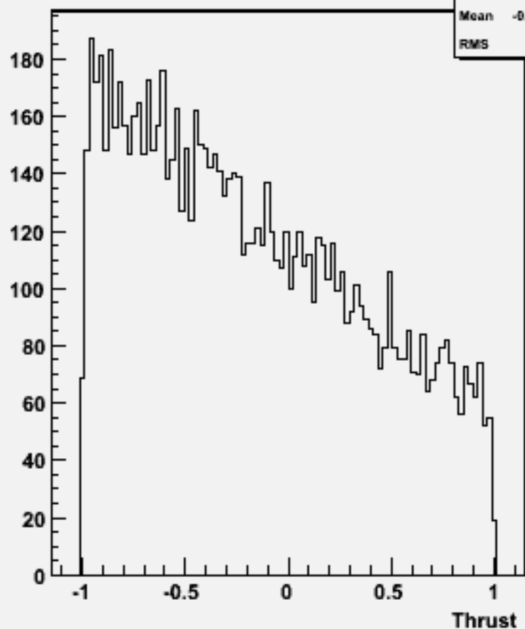
cos \Theta (thrust) w101240 bbn3e3e2n2_o
