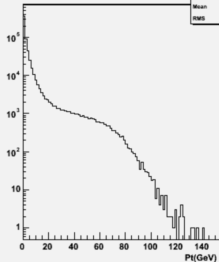
Particle Pt : w101240 bbn3e3e2n2_o
