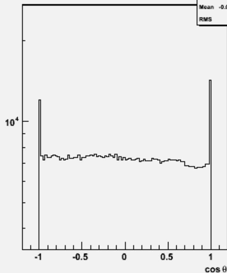
Particle cosθ : w101240 bbn3e3e2n2_o
