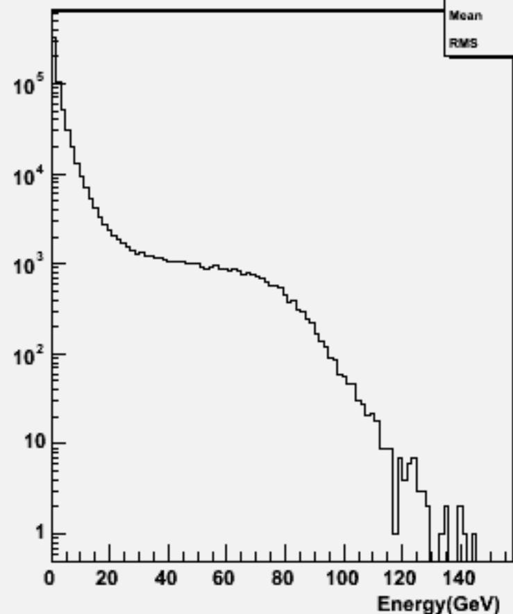
Particle Energy : w101240 bbn3e3e2n2_o
