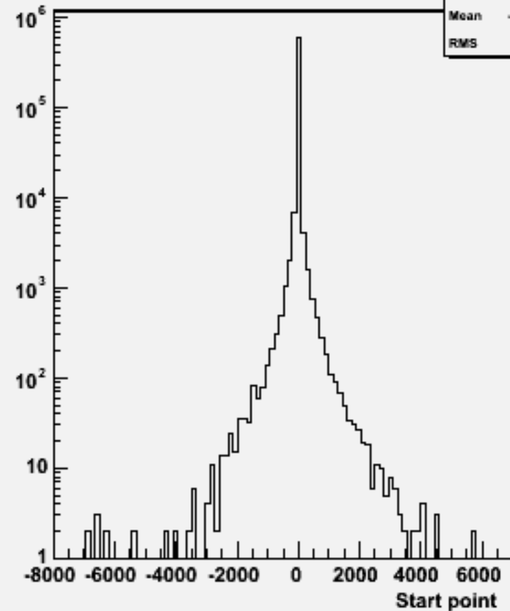
Start point Z : w101240 bbn3e3e2n2_o
