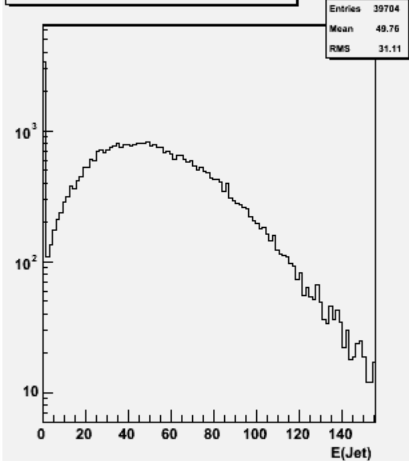
Jet energies(All jets)w101238 bbn3e3e1n1_o
