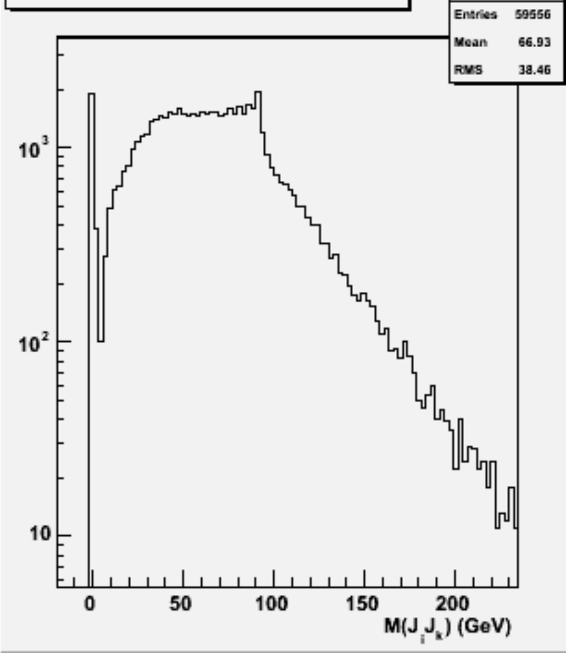
2jets mass(All comb)w101238 bbn3e3e1n1_o
