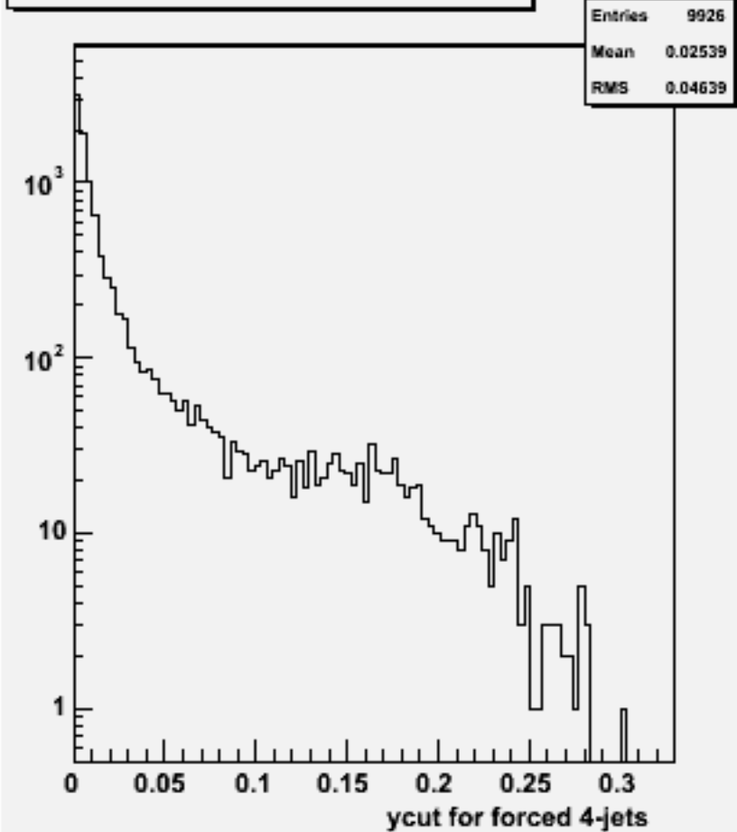
Ycut for 4-jets :w101238 bbn3e3e1n1_o
