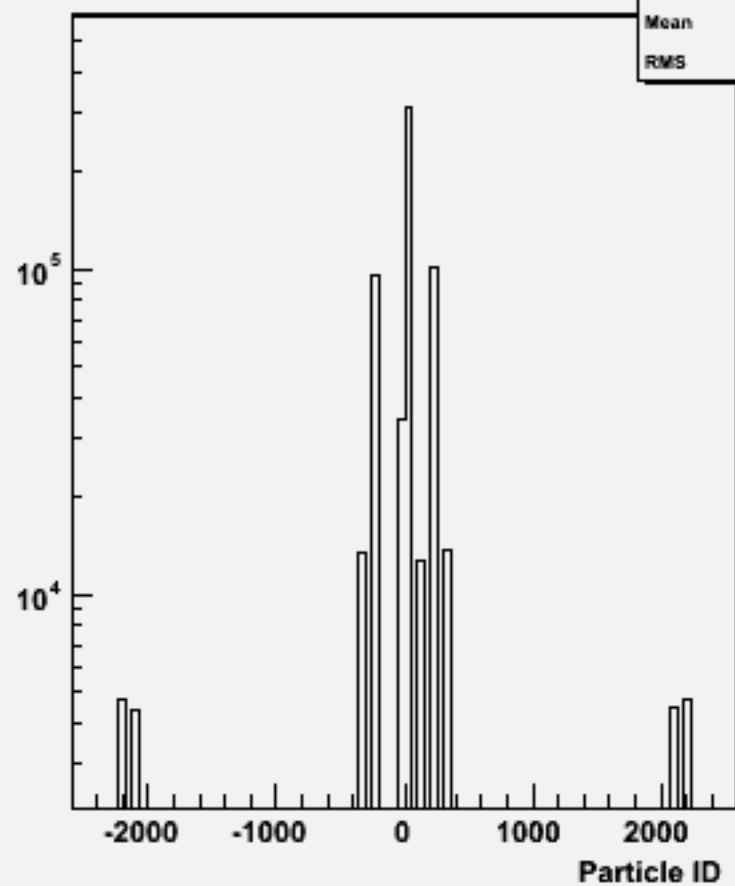
Particle ID : w101238 bbn3e3e1n1_o
