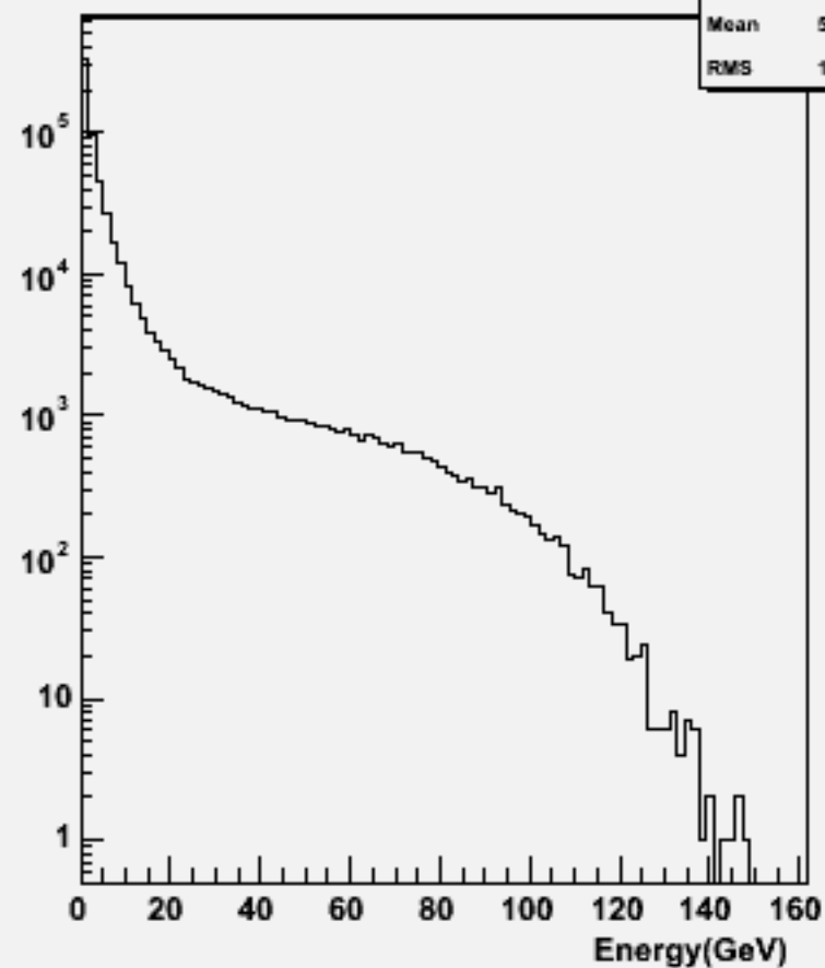
Particle Energy : w101238 bbn3e3e1n1_o
