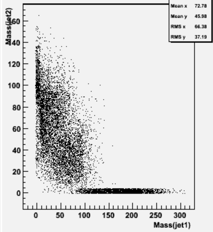
Jet mass for forced 2-jets : w101238 bbn3e3e1n1_o
