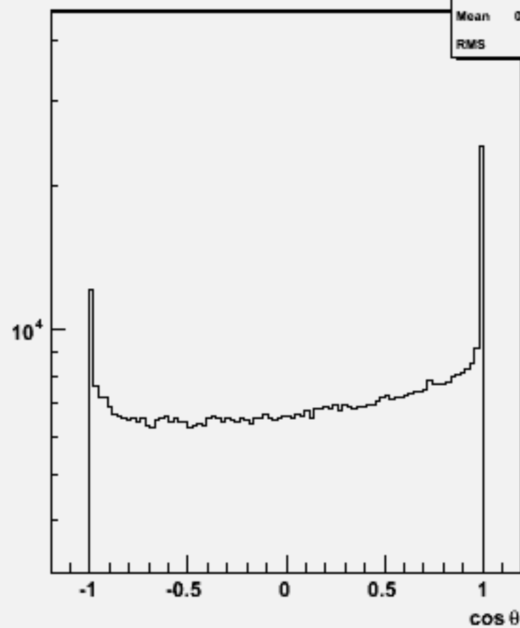
Particle \cos\theta : w101238 bbn3e3e1n1_o
