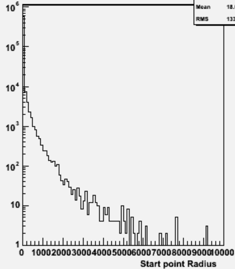
Start point R : w101238 bbn3e3e1n1_o
