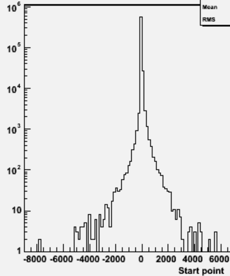
Start point Z : w101238 bbn3e3e1n1_o
