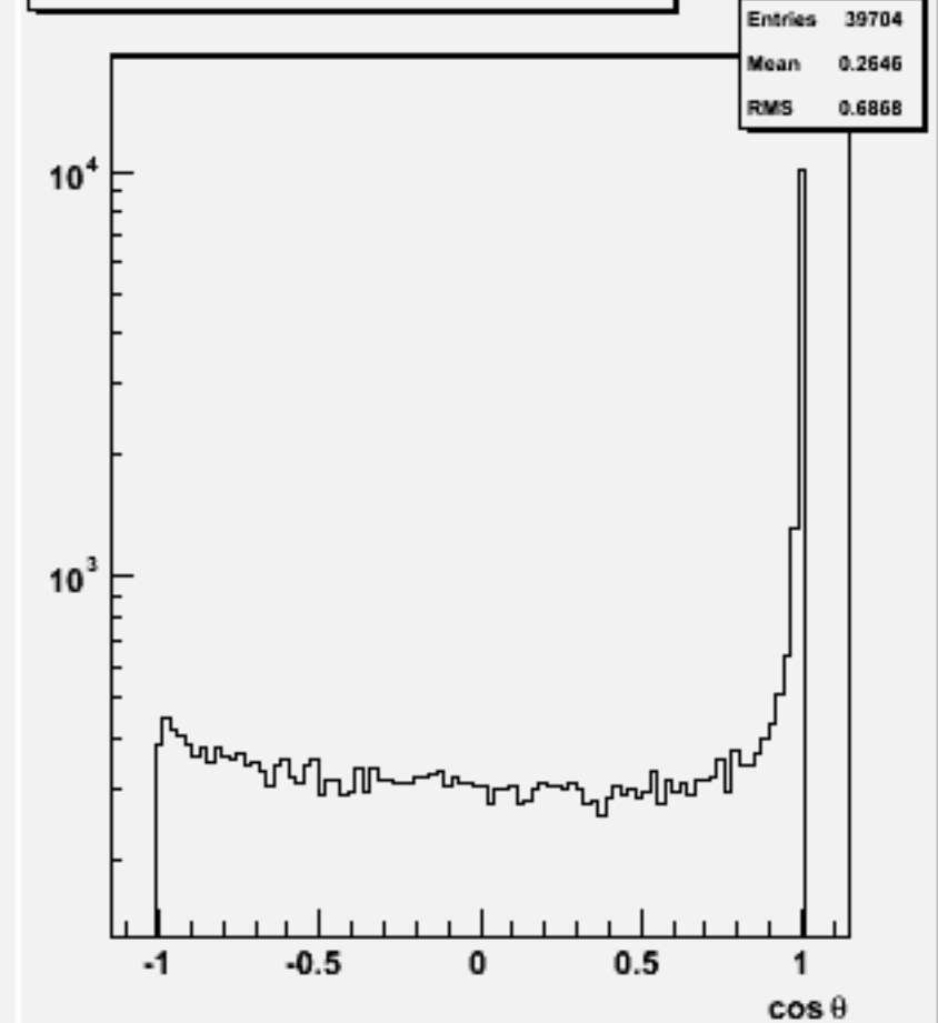
Jet cos \theta (All jets)w101238 bbn3e3e1n1_o
