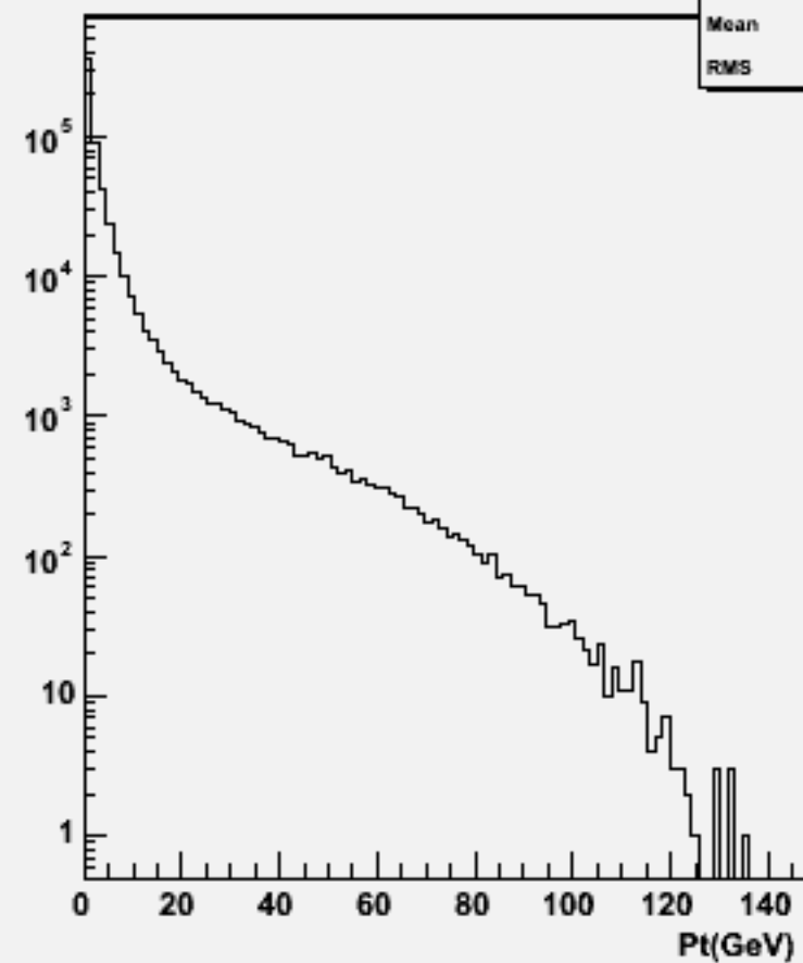
Particle Pt : w101238 bbn3e3e1n1_o
