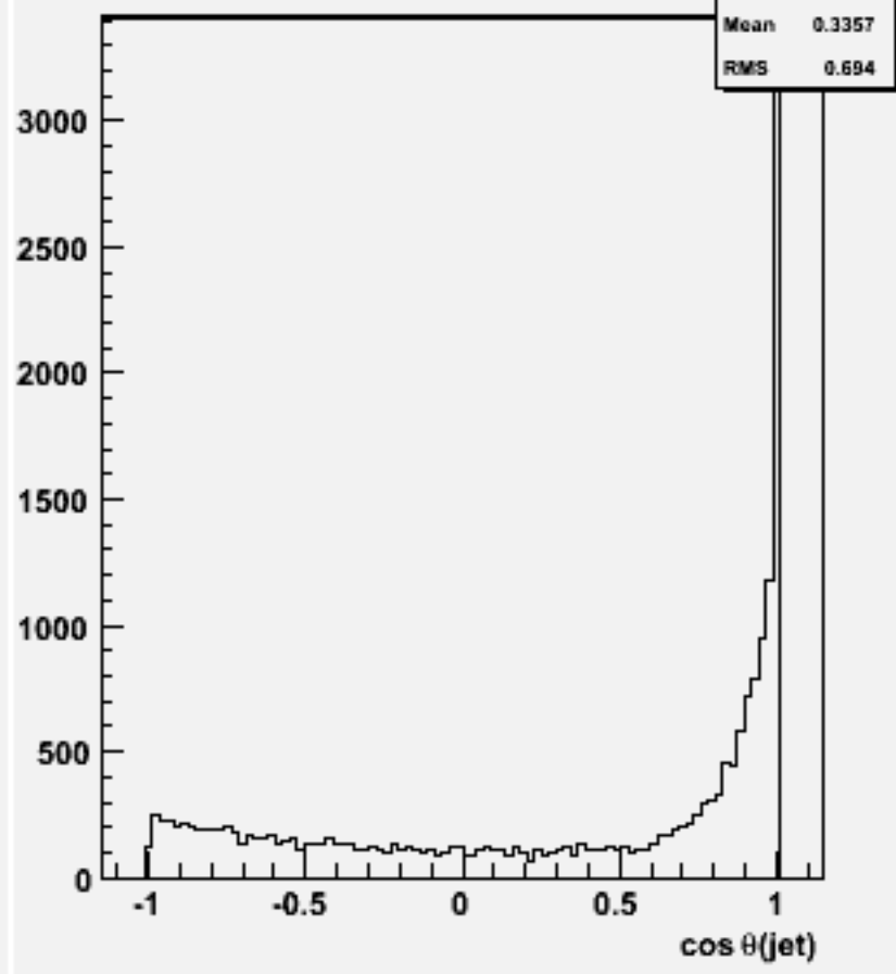
cos \theta for 2-jets :w101238 bbn3e3e1n1_o
