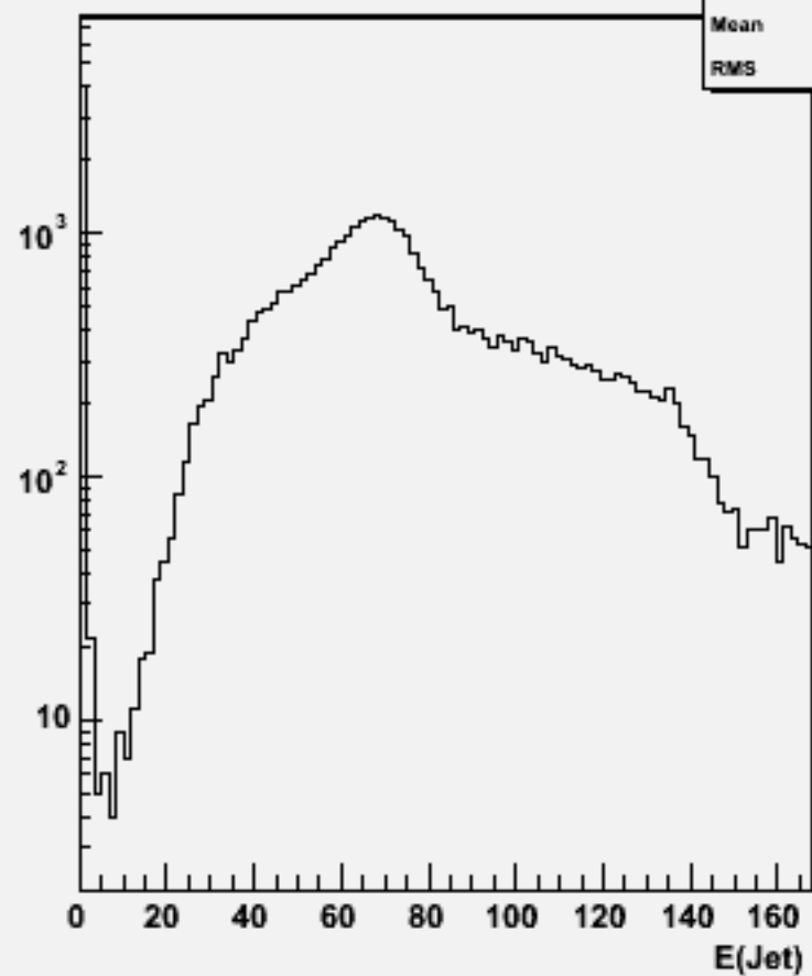
Jet energies(All jets)w101233 bbn2e2sc_o
