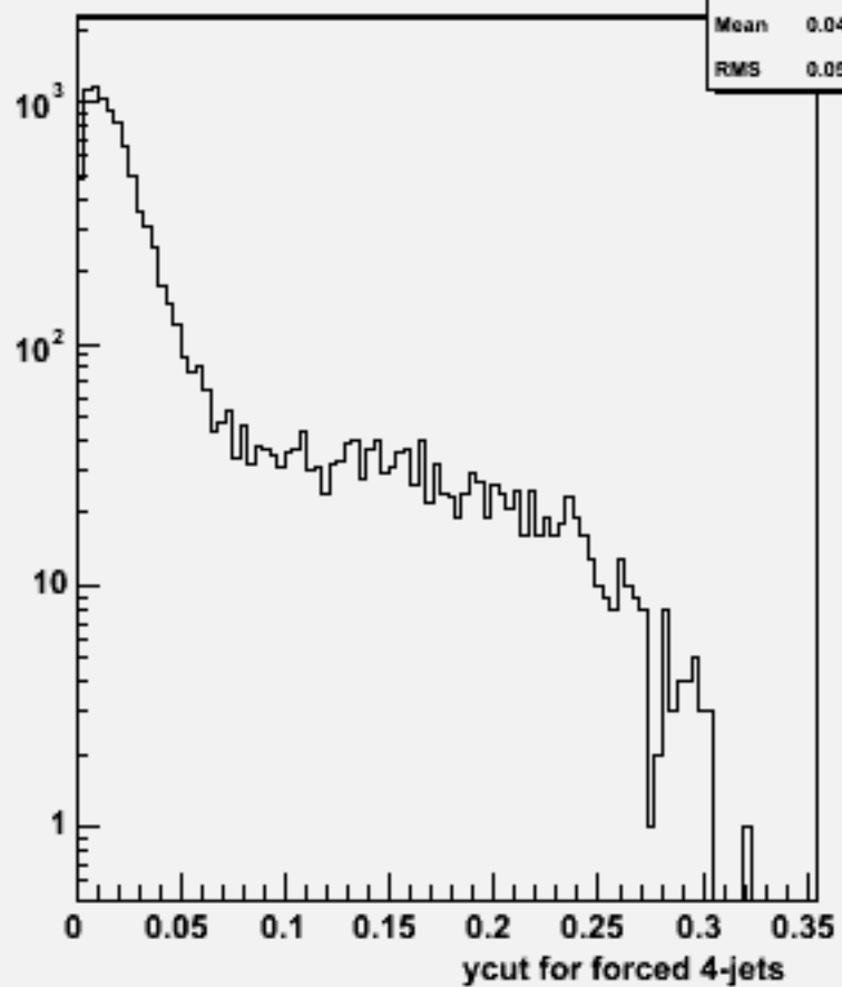
Ycut for 4-jets :w101233 bbn2e2sc_o
