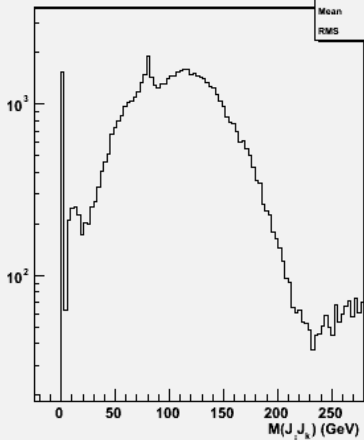
2jets mass(All comb)w101233 bbn2e2sc_o
