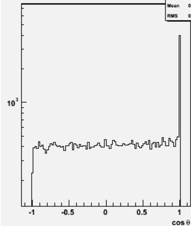
Jet cos \theta (All jets)w101233 bbn2e2sc_o
