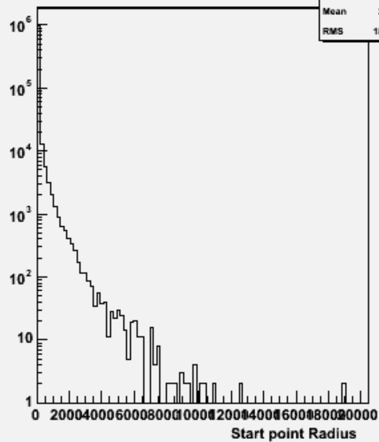
Start point R : w101233 bbn2e2sc_o
