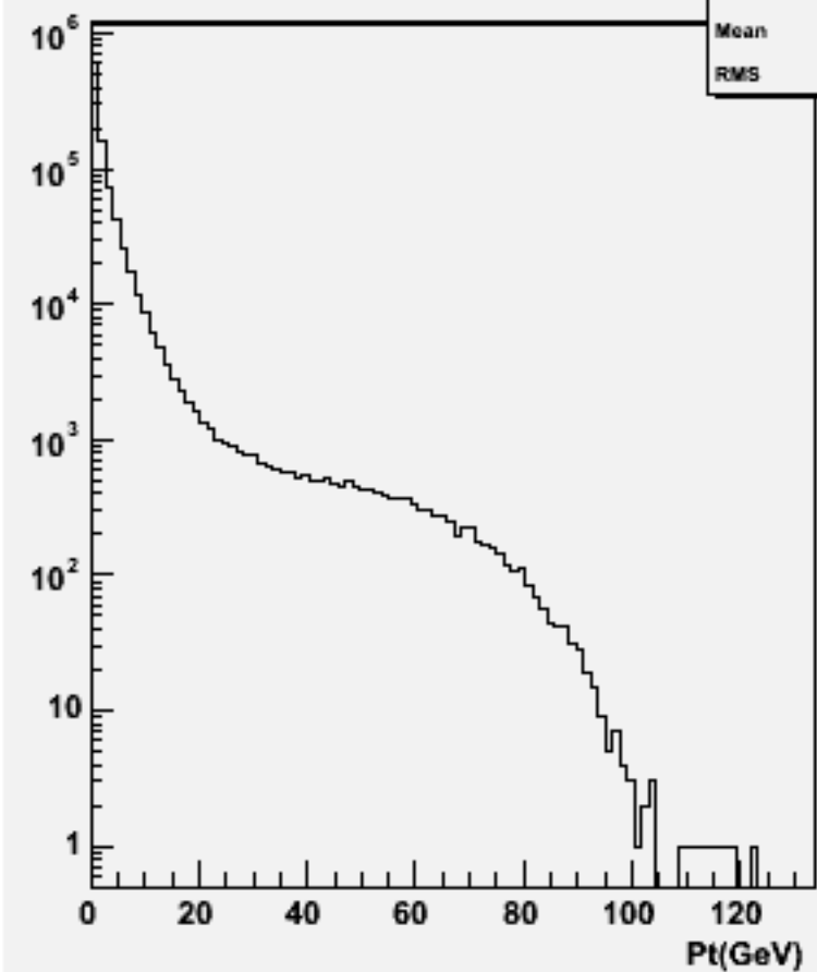
Particle Pt : w101233 bbn2e2sc_o
