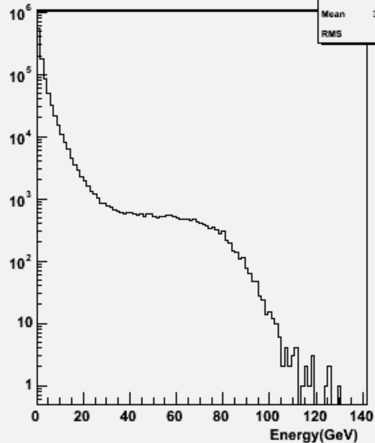
Particle Energy : w101233 bbn2e2sc_o
