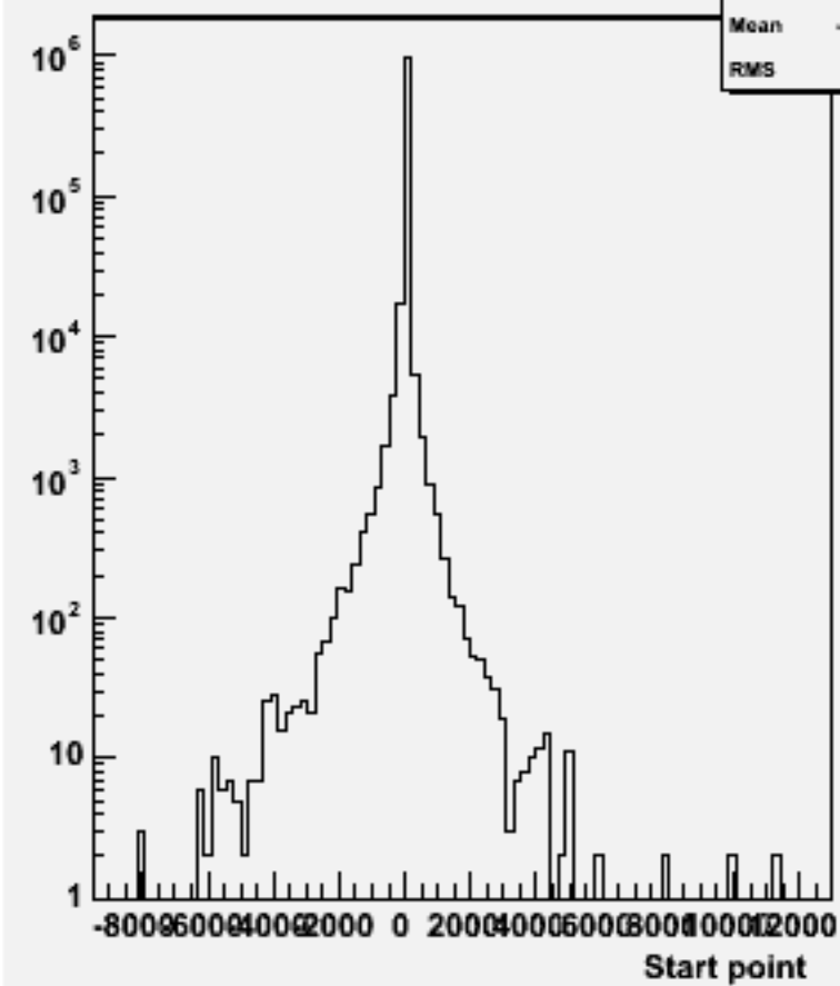
Start point Z : w101233 bbn2e2sc_o
