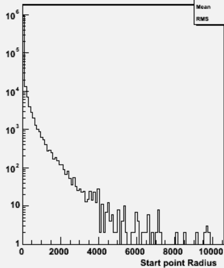
Start point R : w101228 bbn2e2du_o
