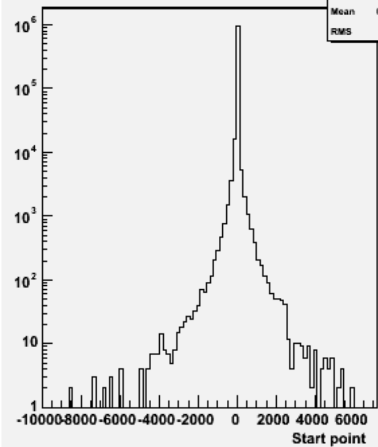
Start point Z : w101228 bbn2e2du_o
