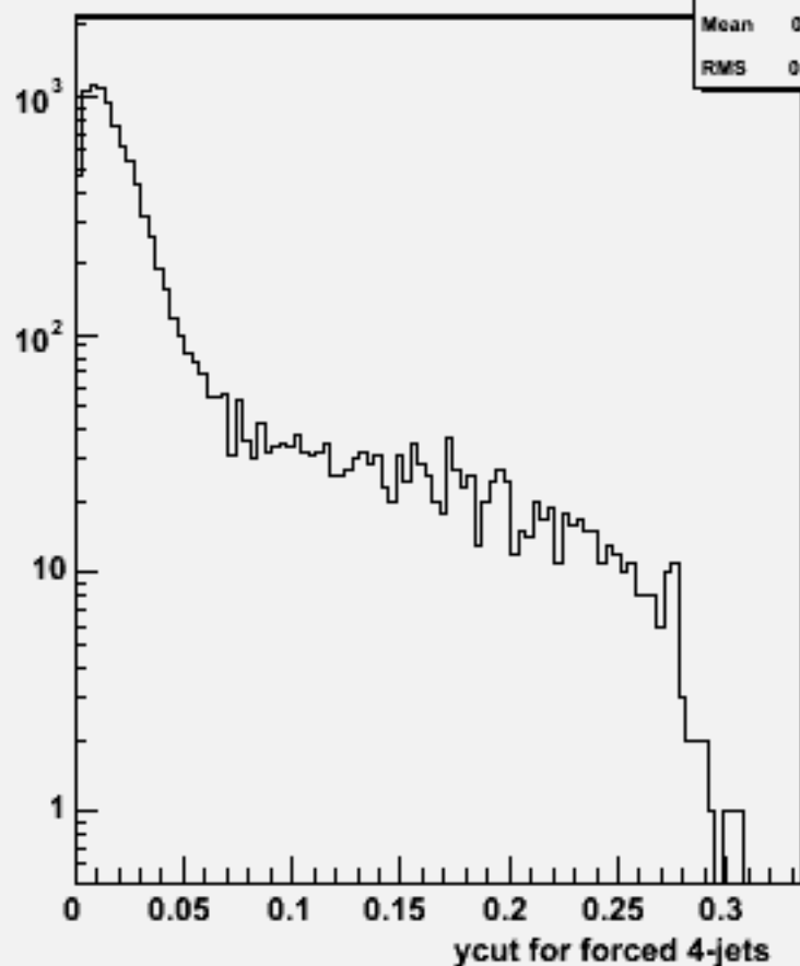
Ycut for 4-jets :w101228 bbn2e2du_o
