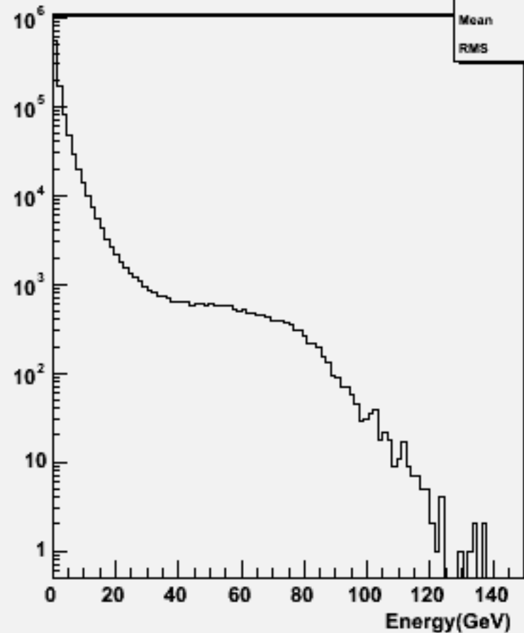
Particle Energy : w101228 bbn2e2du_o
