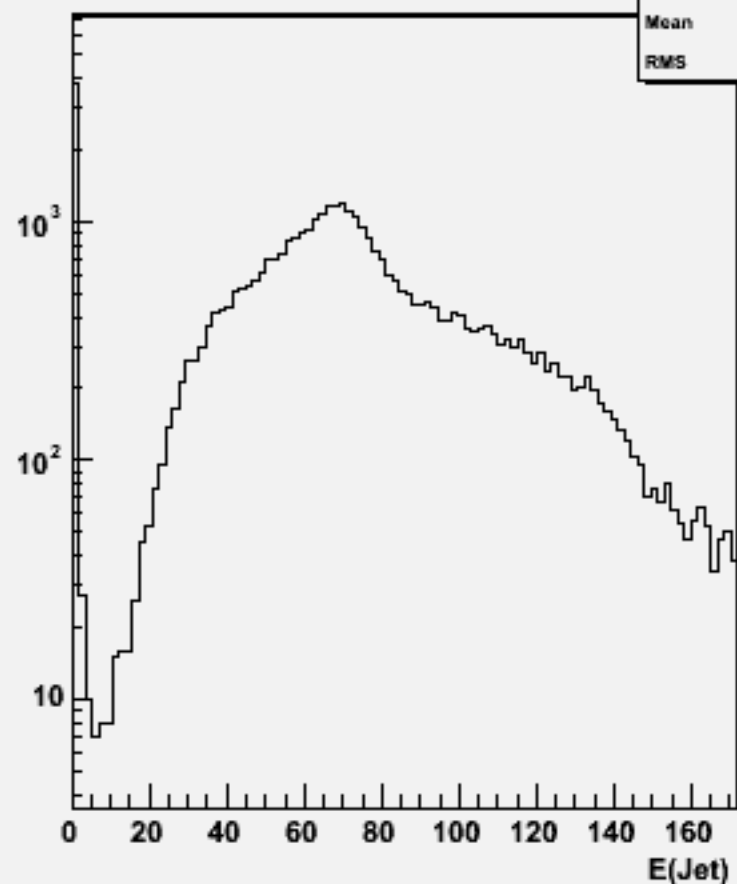
Jet energies(All jets)w101228 bbn2e2du_o
