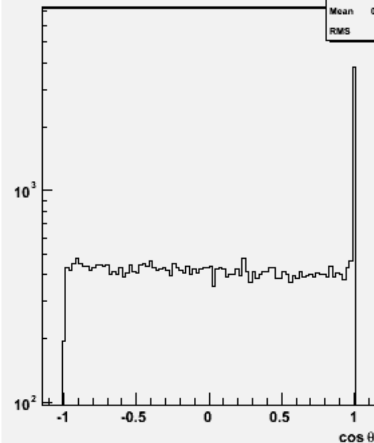
Jet cos \theta (All jets)w101228 bbn2e2du_o
