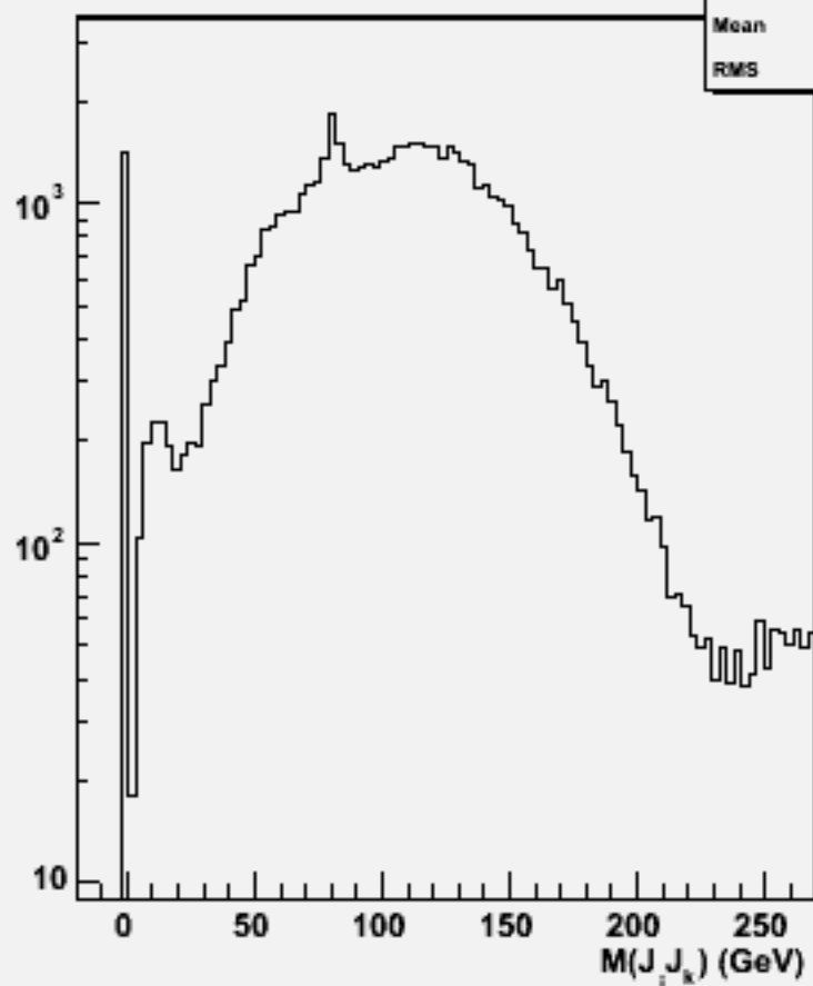
2jets mass(All comb)w101228 bbn2e2du_o
