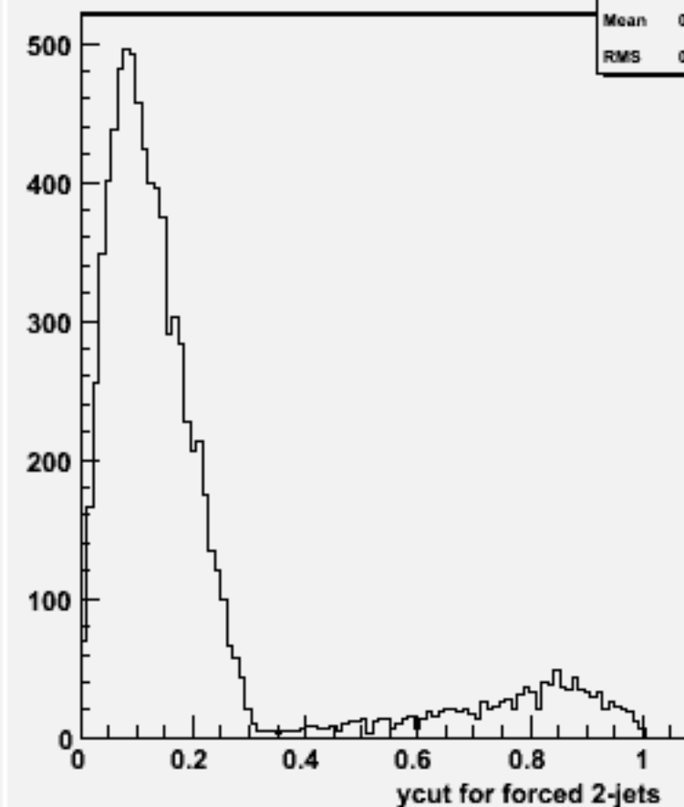
Ycut for 2-jets :w101225 bbn2e2e3n3_o
