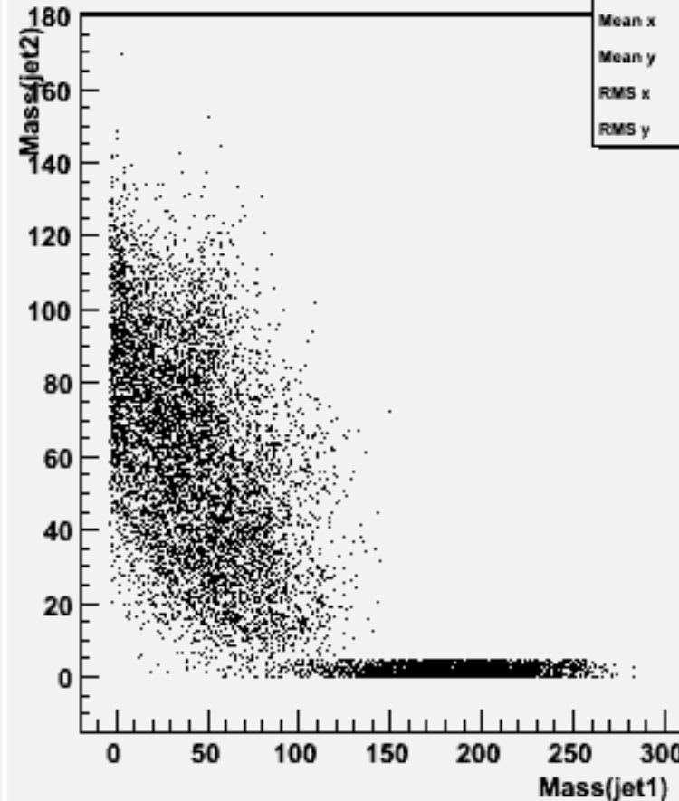
Jet mass for forced 2-jets : w101225 bbn2e2e3n3_o
