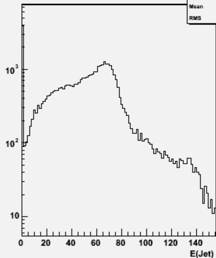
Jet energies(All jets)w101225 bbn2e2e3n3_o
