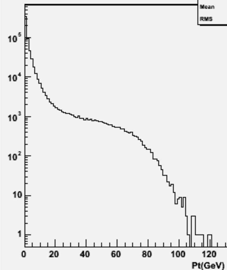
Start point Z : w101225 bbn2e2e3n3_o
