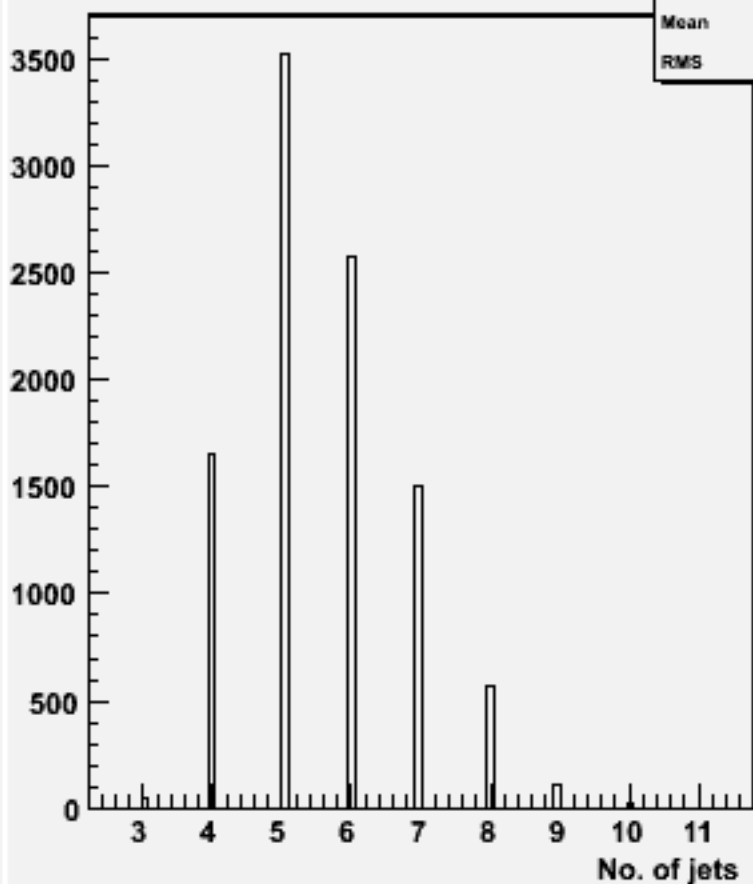
No. jets (ycut=0.001) : w101225 bbn2e2e3n3_o
