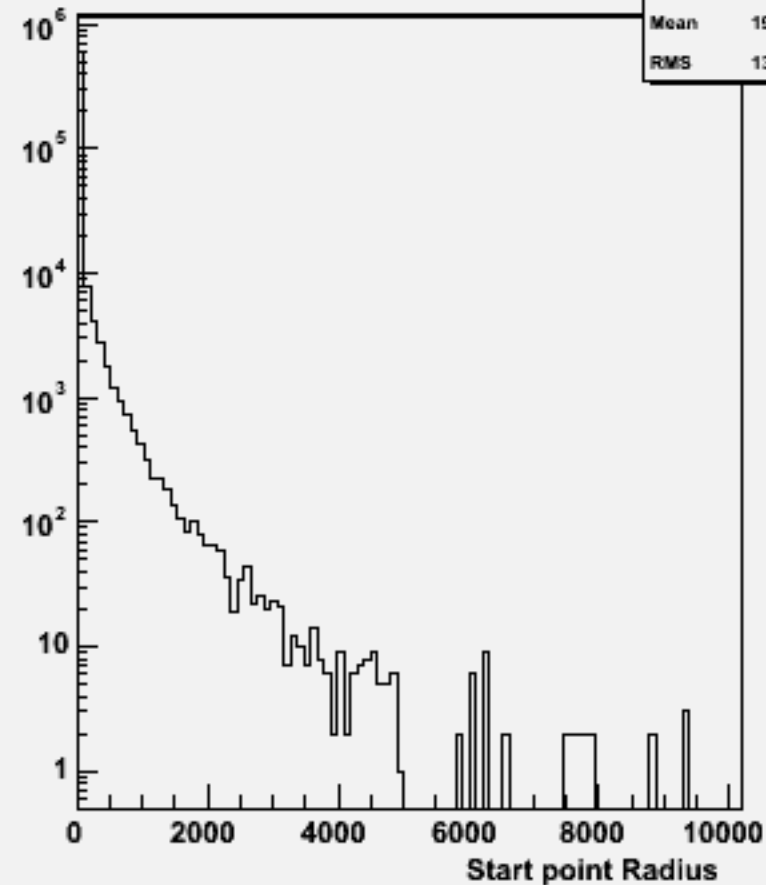
Start point R : w101225 bbn2e2e3n3_o
