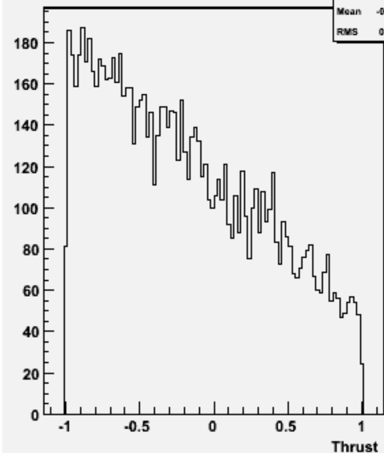
cos \Theta (thrust) w101225 bbn2e2e3n3_o
