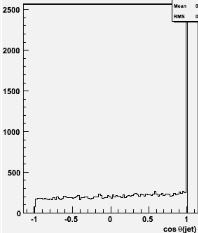
cos \theta for 2-jets :w101225 bbn2e2e3n3_o
