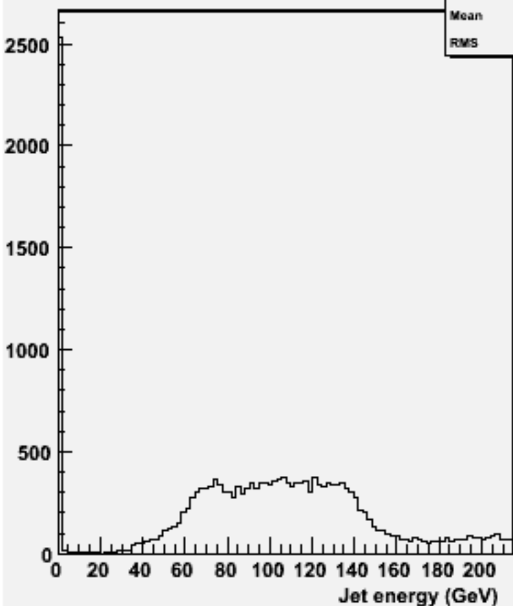
energy for 2-jets :w101225 bbn2e2e3n3_o
