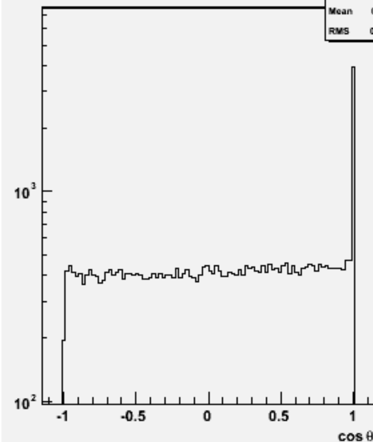
Jet cos \theta (All jets)w101225 bbn2e2e3n3_o
