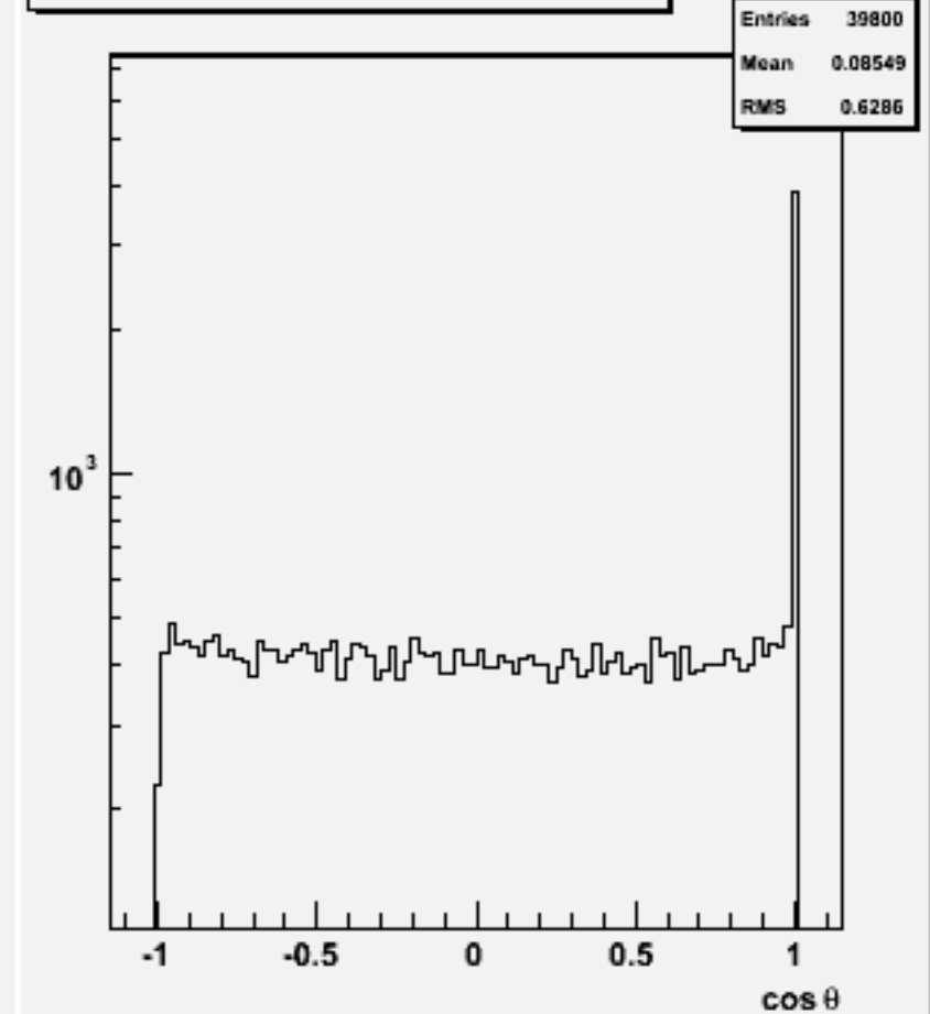
Jet cos \theta (All jets)w101224 bbn2e2e3n3_o
