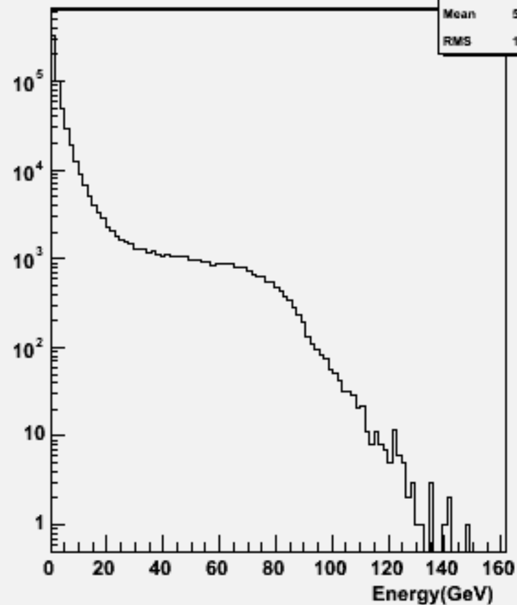
Start point R : w101224 bbn2e2e3n3_o
