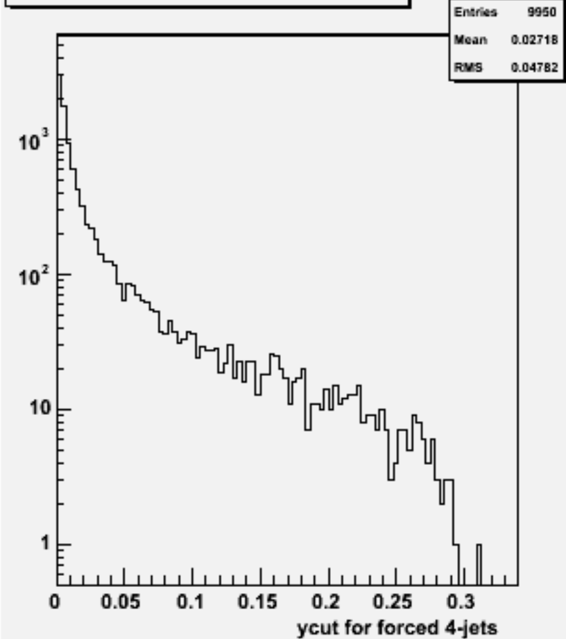
Ycut for 4-jets :w101224 bbn2e2e3n3_o
