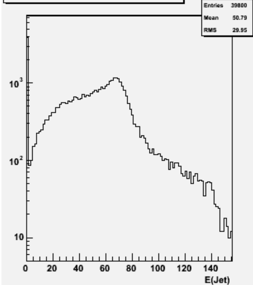
Jet energies(All jets)w101224 bbn2e2e3n3_o
