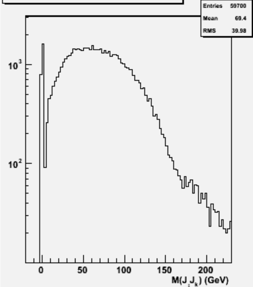
2jets mass(All comb)w101224 bbn2e2e3n3_o
