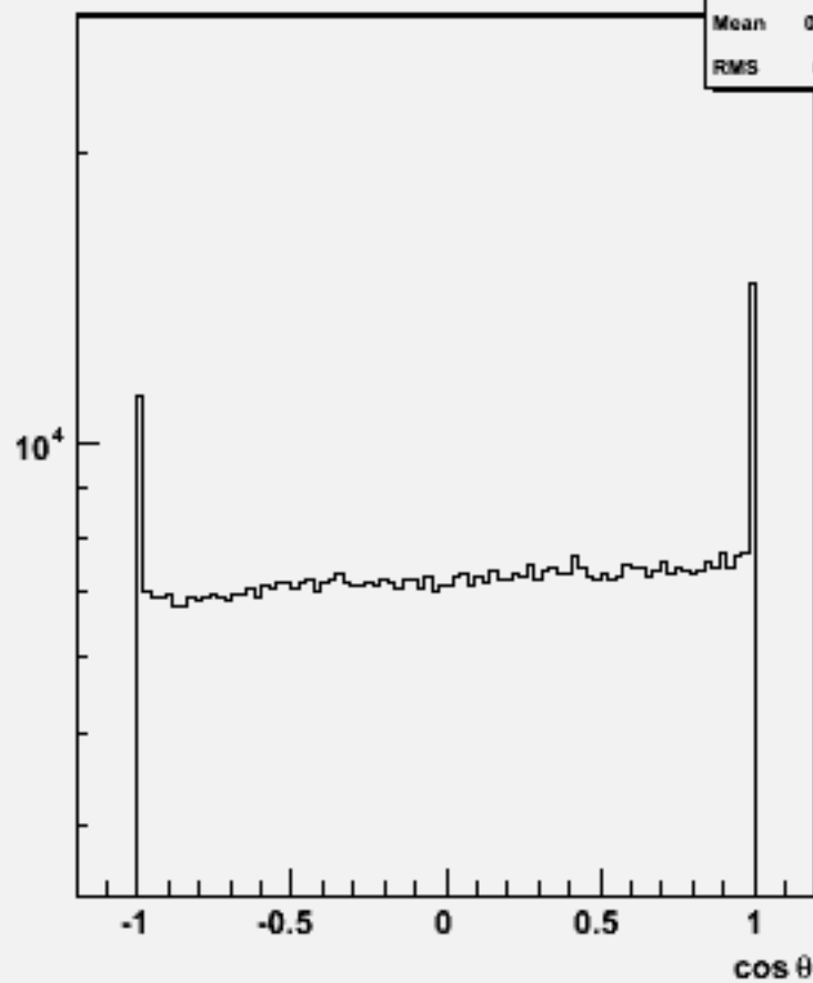
Particle \cos\theta : w101224 bbn2e2e3n3_o
