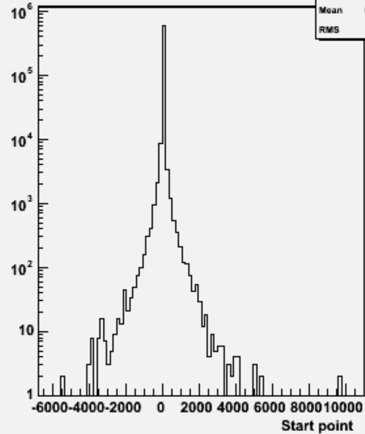
Start point Z : w101224 bbn2e2e3n3_o
