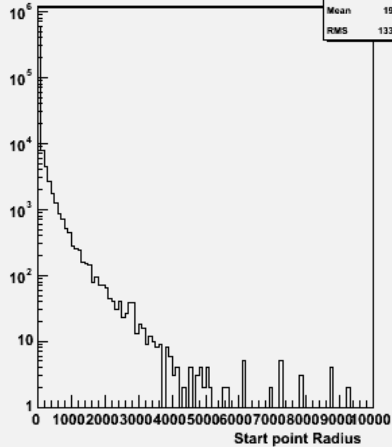
Start point R : w101224 bbn2e2e3n3_o
