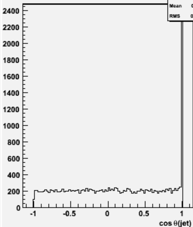
cos \theta for 2-jets :w101221 bbn2e2e2n2_o
