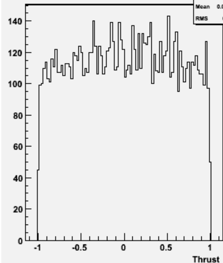
cos \Theta (thrust) w101221 bbn2e2e2n2_o
