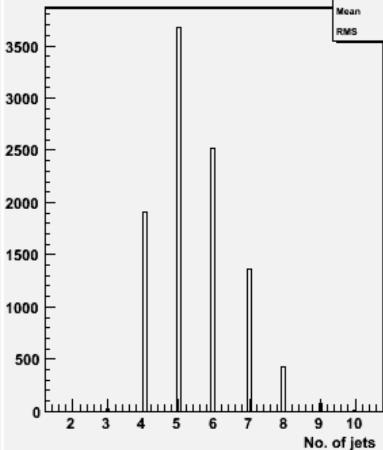
No. jets (ycut=0.001) : w101221 bbn2e2e2n2_o
