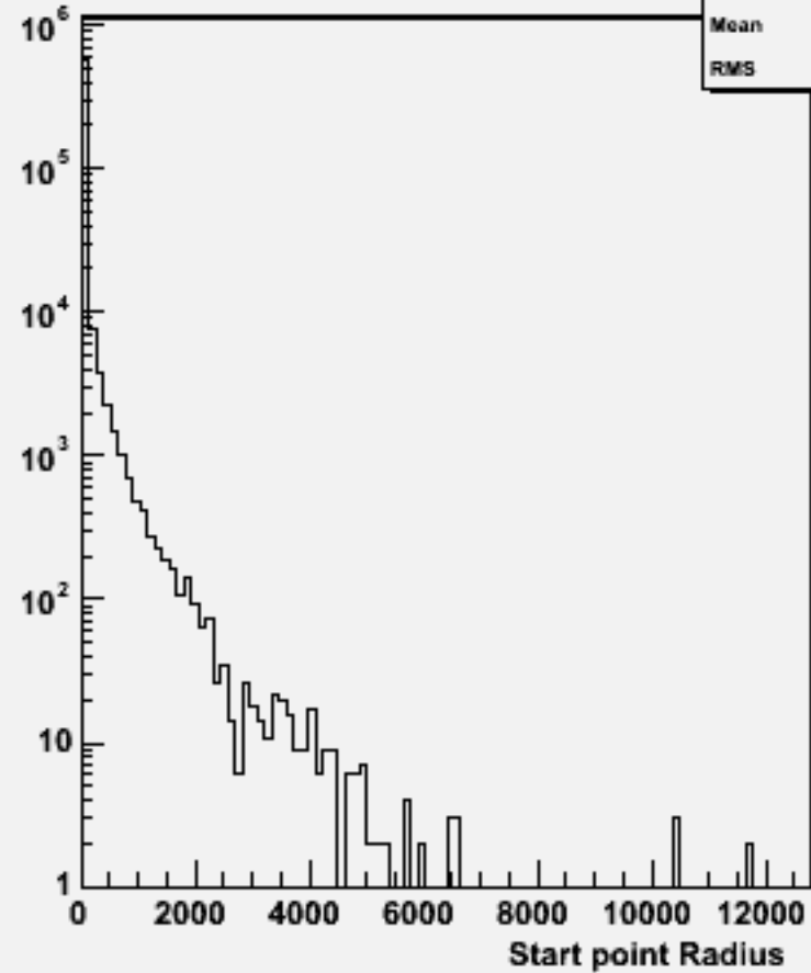
Start point R : w101221 bbn2e2e2n2_o
