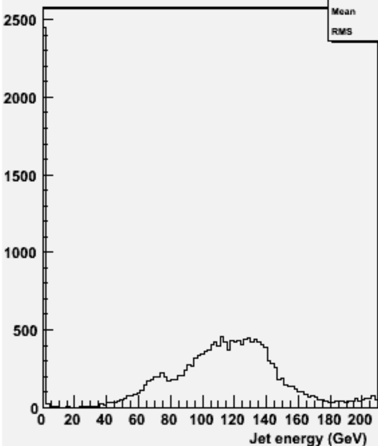
energy for 2-jets :w101221 bbn2e2e2n2_o
