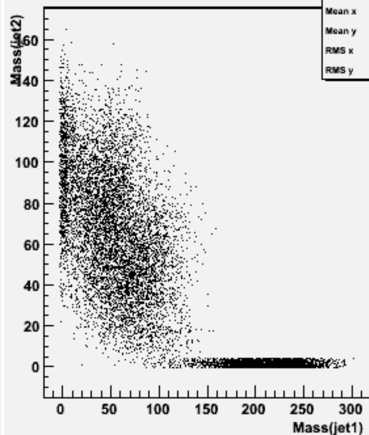
Jet mass for forced 2-jets : w101221 bbn2e2e2n2_o
