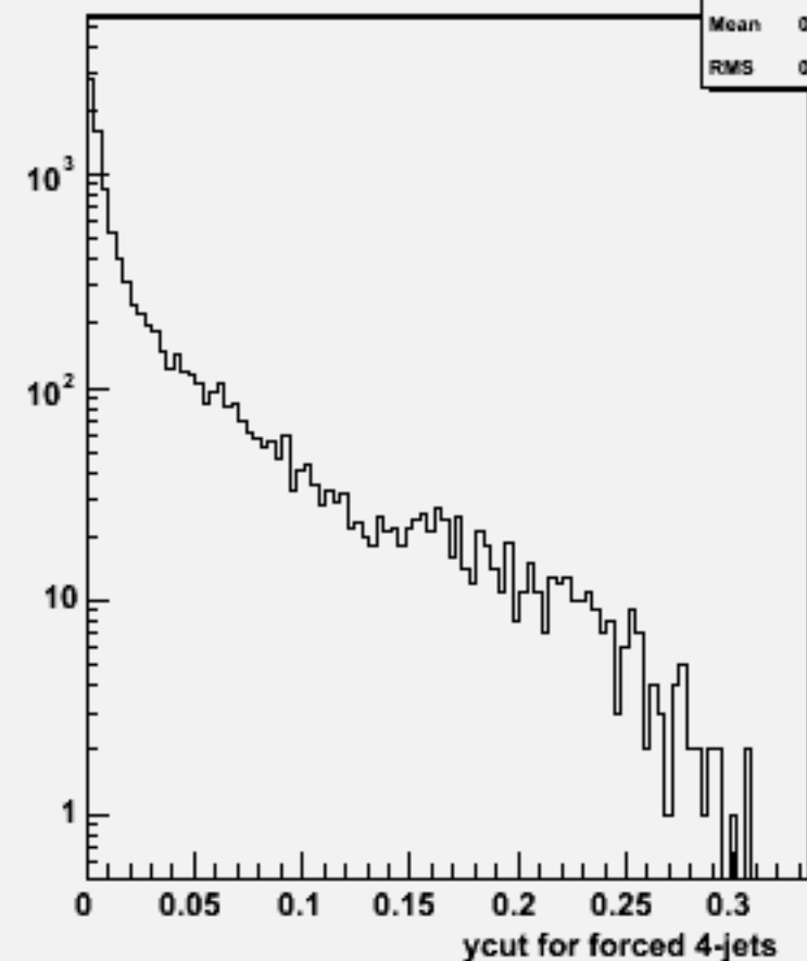
Ycut for 4-jets :w101221 bbn2e2e2n2_o
