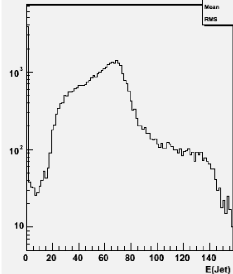
Jet energies(All jets)w101221 bbn2e2e2n2_o
