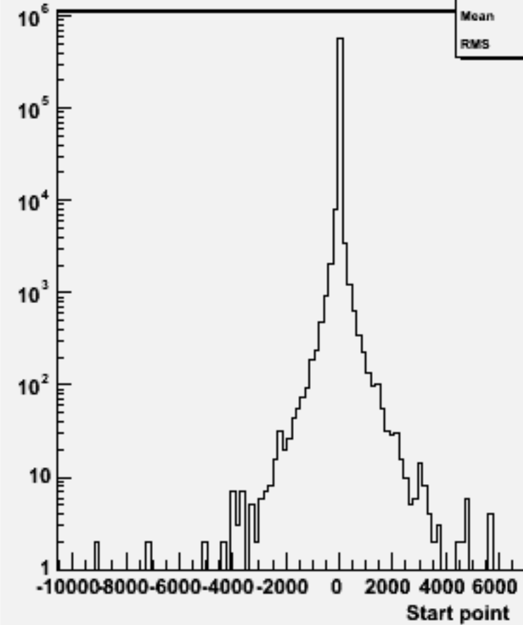
Start point Z : w101221 bbn2e2e2n2_o
