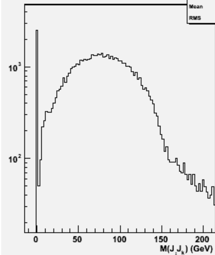
2jets mass(All comb)w101221 bbn2e2e2n2_o
