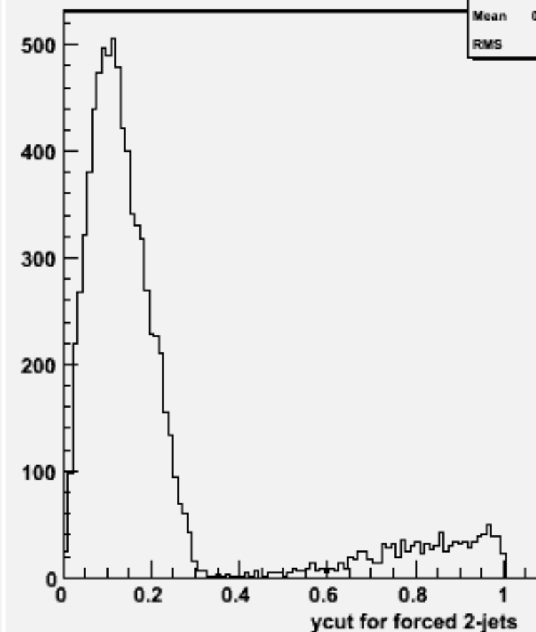
Ycut for 2-jets :w101221 bbn2e2e2n2_o
