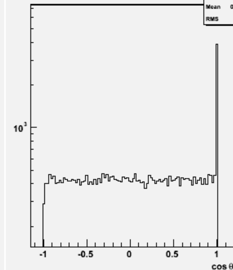
Jet cos \theta (All jets)w101221 bbn2e2e2n2_o
