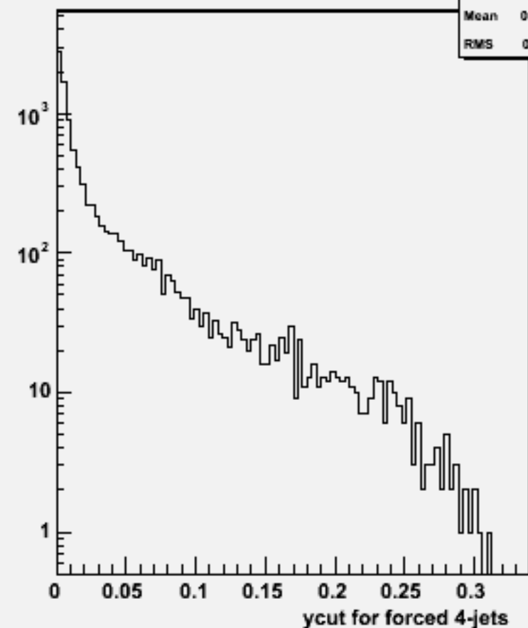
Ycut for 4-jets :w101220 bbn2e2e2n2_o
