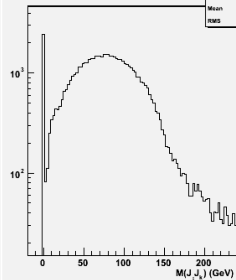
2jets mass(All comb)w101220 bbn2e2e2n2_o
