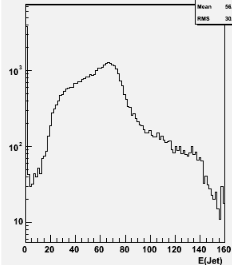
Jet energies(All jets)w101220 bbn2e2e2n2_o
