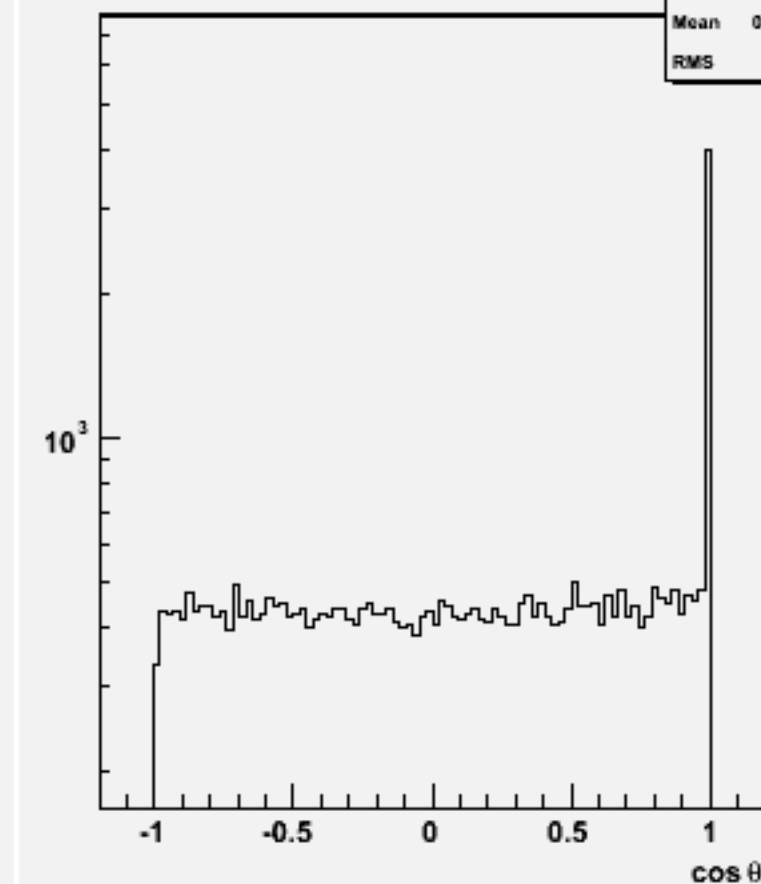
Jet cos \theta (All jets)w101220 bbn2e2e2n2_o
