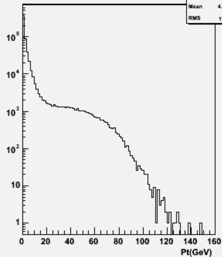
Start point Z : w101220 bbn2e2e2n2_o
