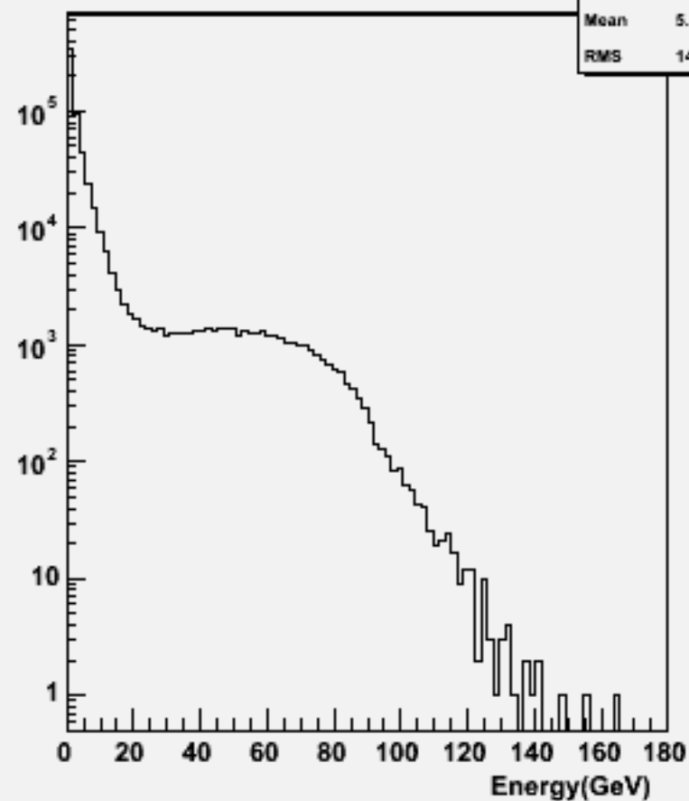
Start point R : w101220 bbn2e2e2n2_o
