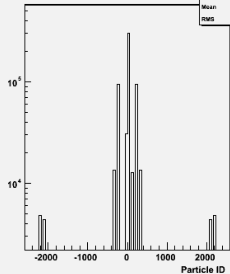
Particle ID : w101218 bbn2e2e1n1_o
