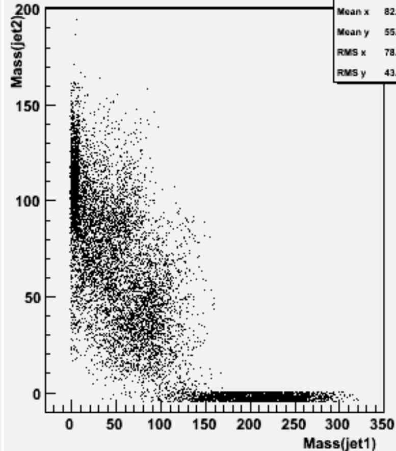
Jet mass for forced 2-jets : w101218 bbn2e2e1n1_o
