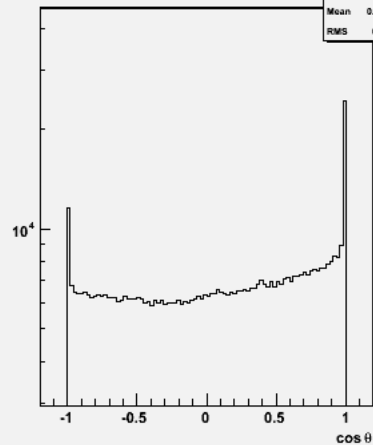
Particle cos \theta : w101218 bbn2e2e1n1_o
