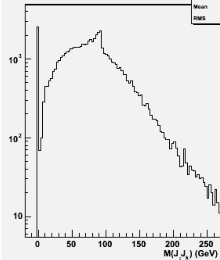
2jets mass(All comb)w101218 bbn2e2e1n1_o
