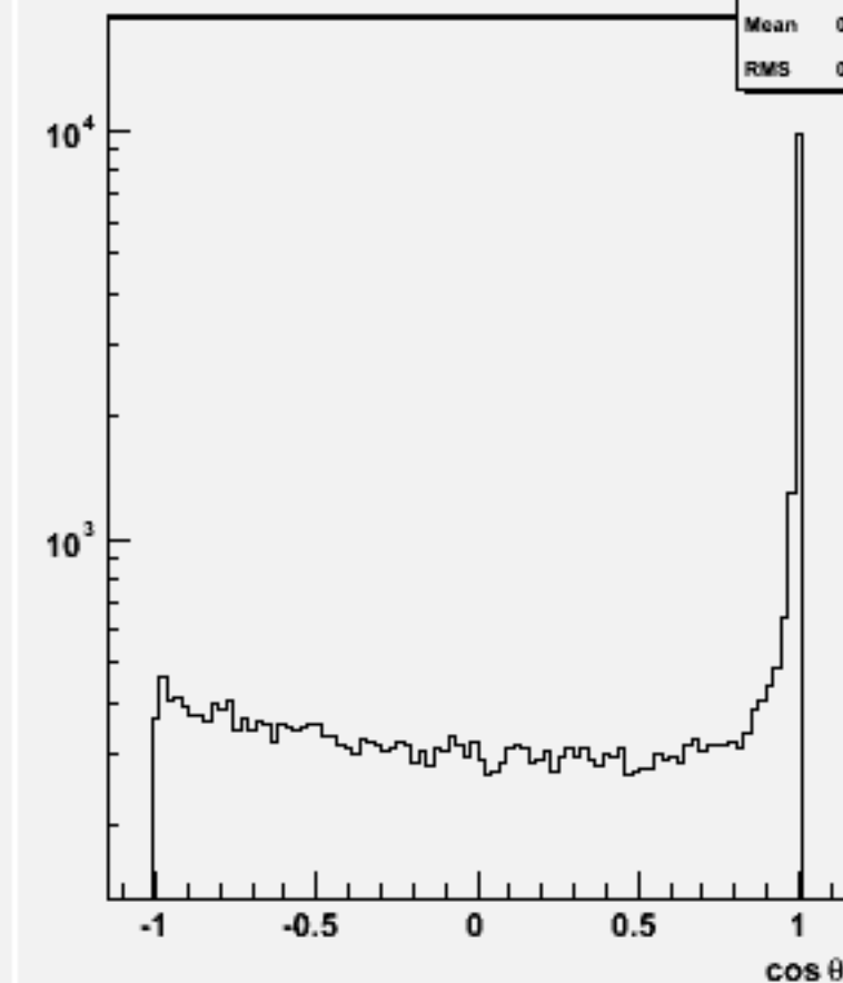
Jet cos \theta (All jets)w101218 bbn2e2e1n1_o
