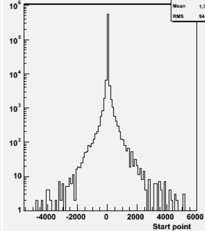
Start point Z : w101218 bbn2e2e1n1_o
