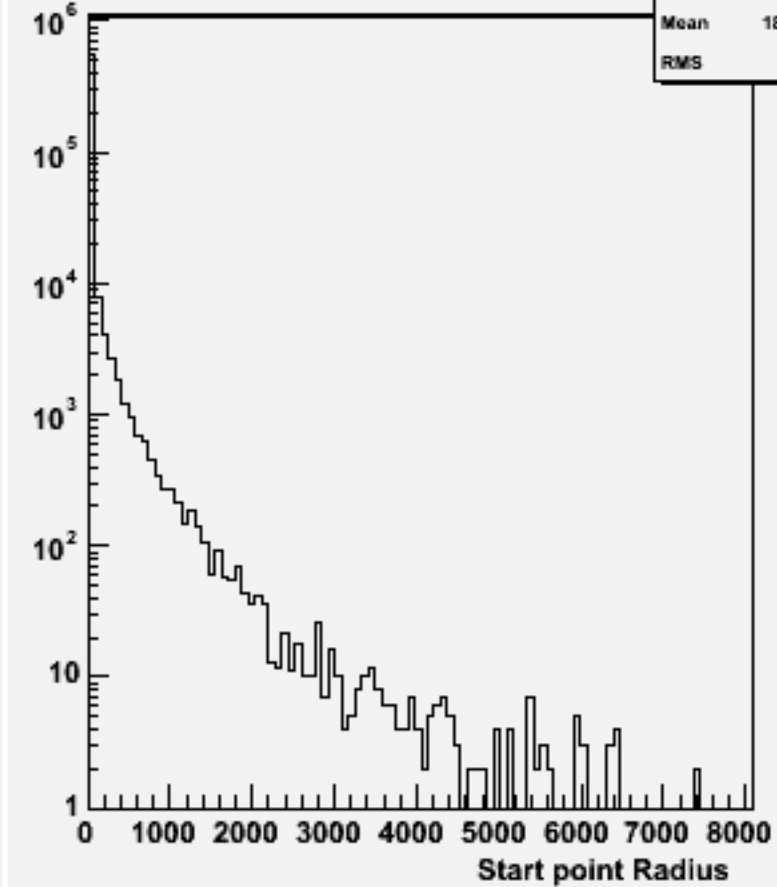
Start point R : w101218 bbn2e2e1n1_o
