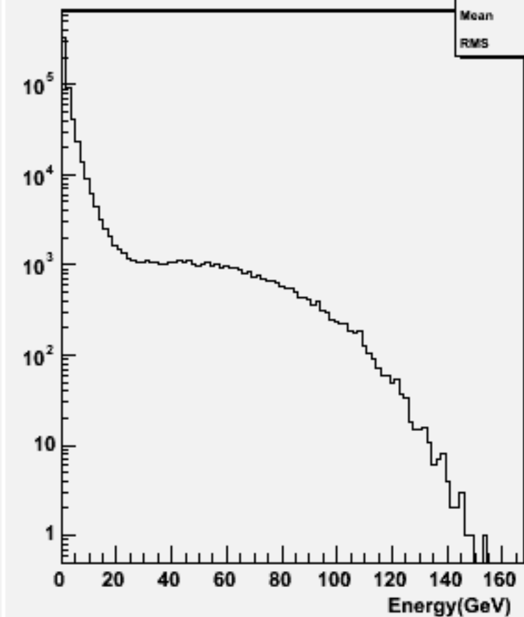
Particle Energy : w101218 bbn2e2e1n1_o
