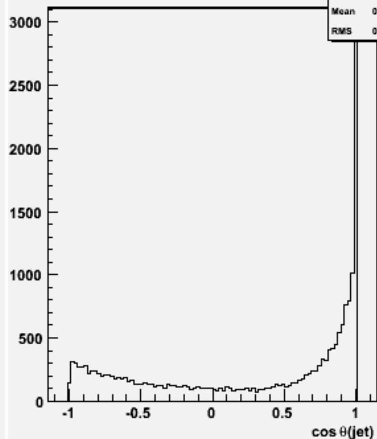
cos \theta for 2-jets :w101218 bbn2e2e1n1_o
