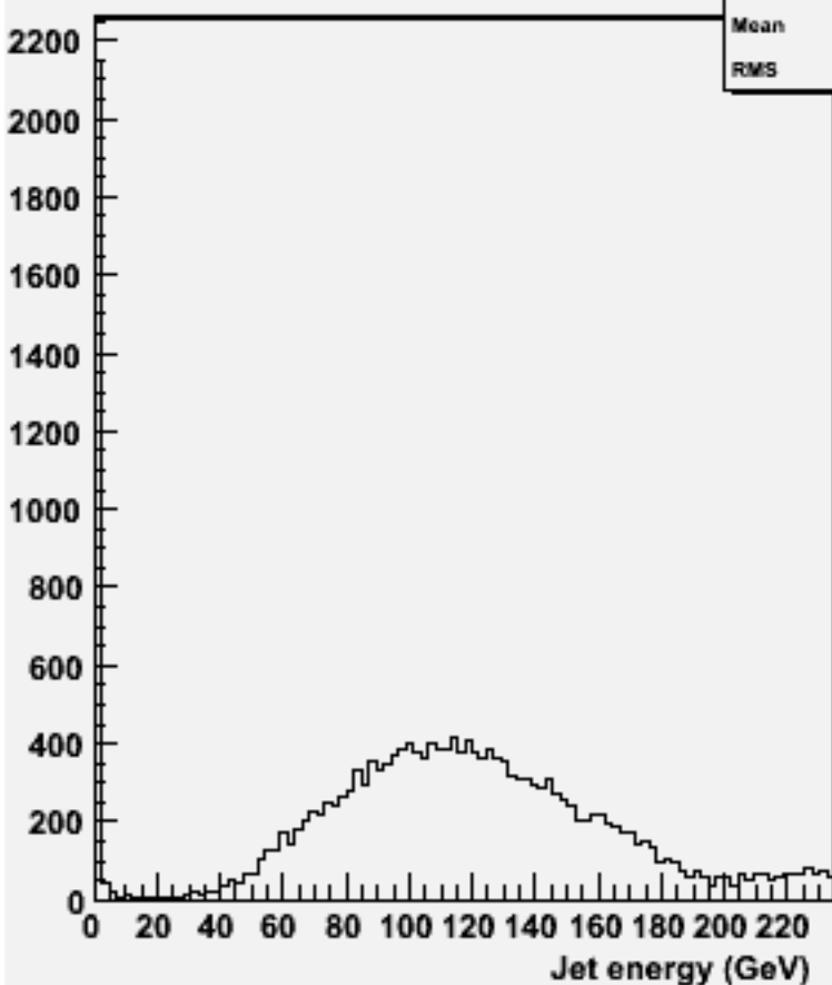
energy for 2-jets :w101218 bbn2e2e1n1_o
