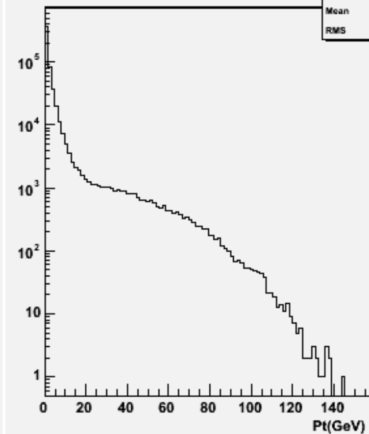
Particle Pt : w101218 bbn2e2e1n1_o
