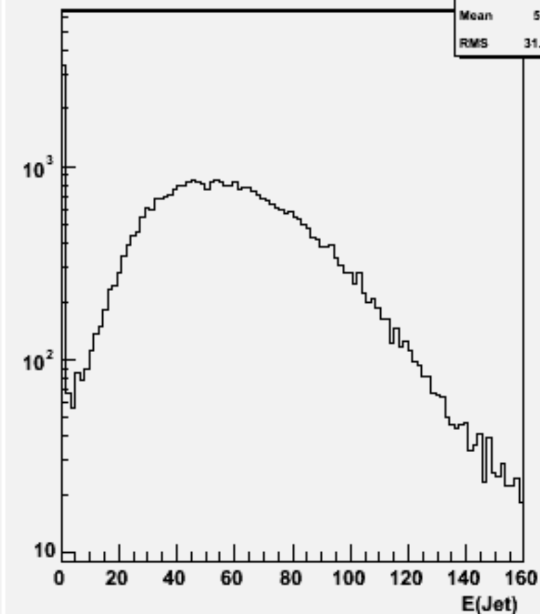
Jet energies(All jets)w101218 bbn2e2e1n1_o
