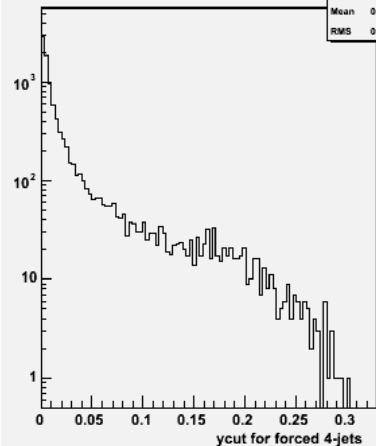
Ycut for 4-jets :w101218 bbn2e2e1n1_o
