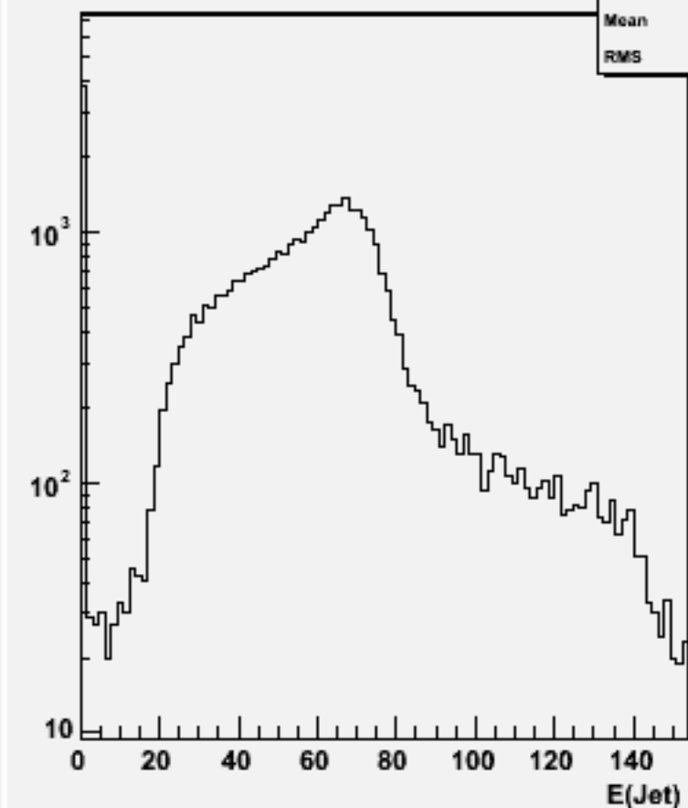
Jet energies(All jets)w101217 bbn2e2e1n1_o
