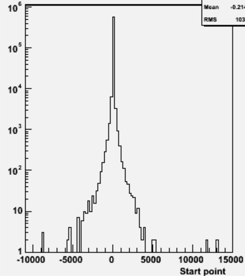
Start point Z : w101217 bbn2e2e1n1_o
