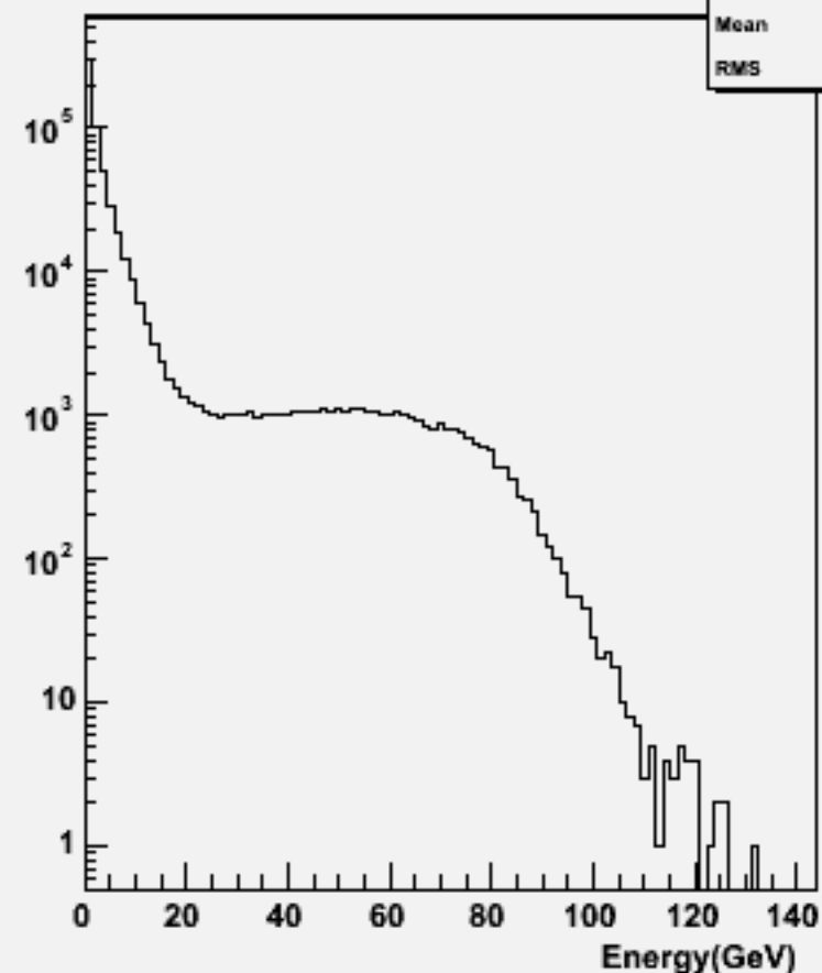
Start point R : w101217 bbn2e2e1n1_o
