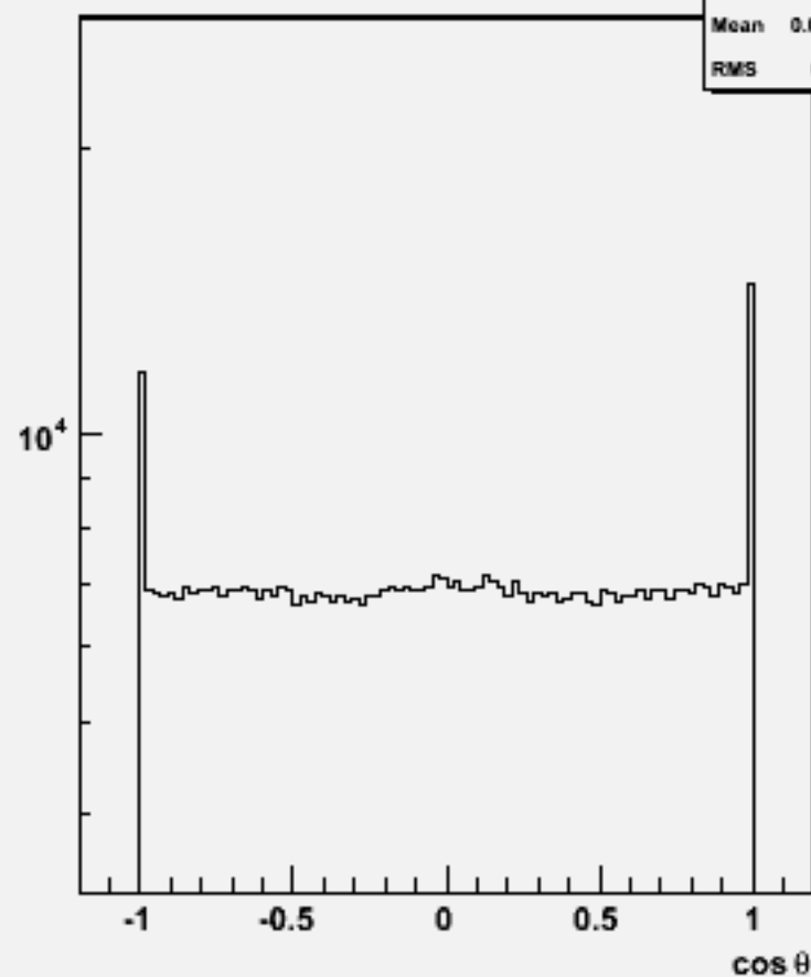
Particle cosθ : w101217 bbn2e2e1n1_o
