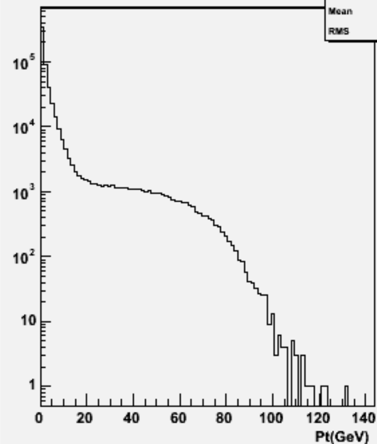
Start point Z : w101217 bbn2e2e1n1_o
