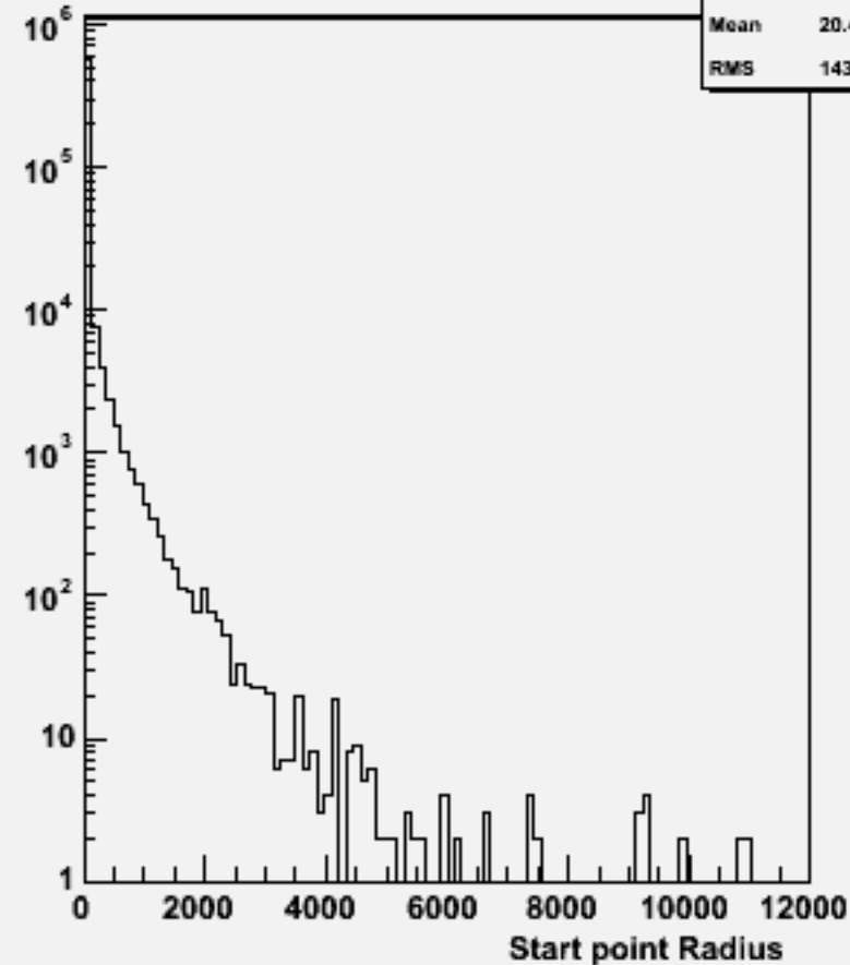
Start point R : w101217 bbn2e2e1n1_o
