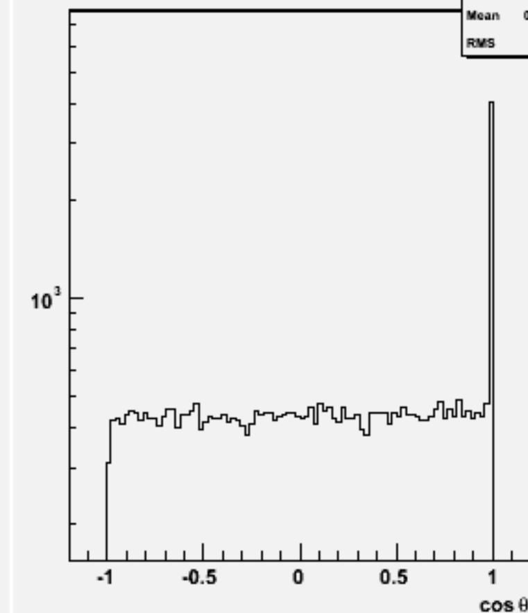
Jet cos \theta (All jets)w101217 bbn2e2e1n1_o
