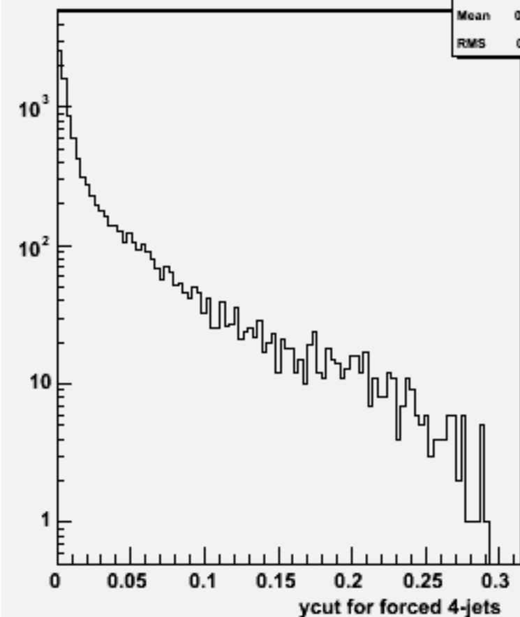
Ycut for 4-jets :w101217 bbn2e2e1n1_o
