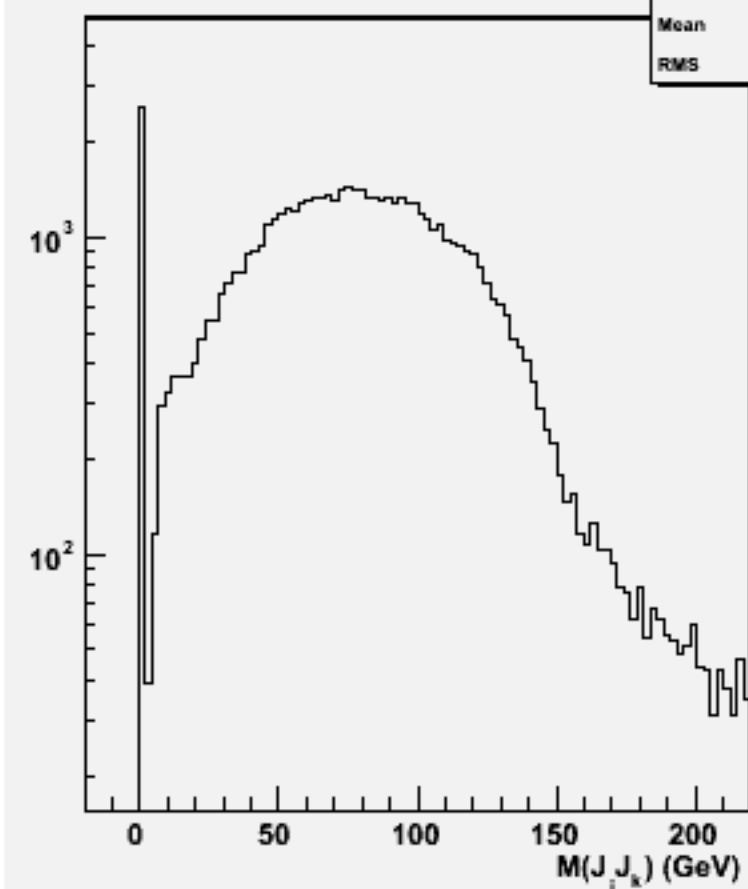
2jets mass(All comb)w101217 bbn2e2e1n1_o
