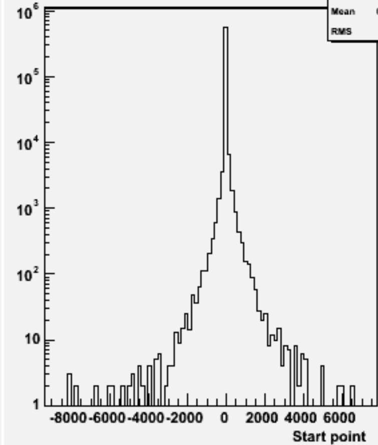
Start point Z : w101216 bbn2e2e1n1_o
