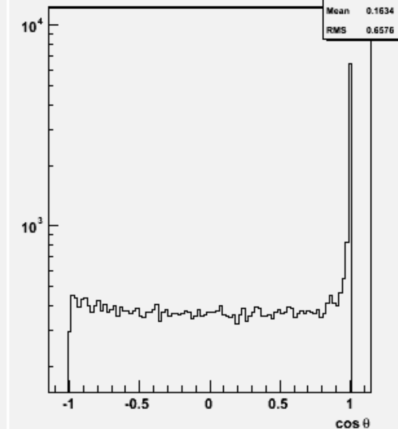
Jet cos \theta (All jets)w101216 bbn2e2e1n1_o
