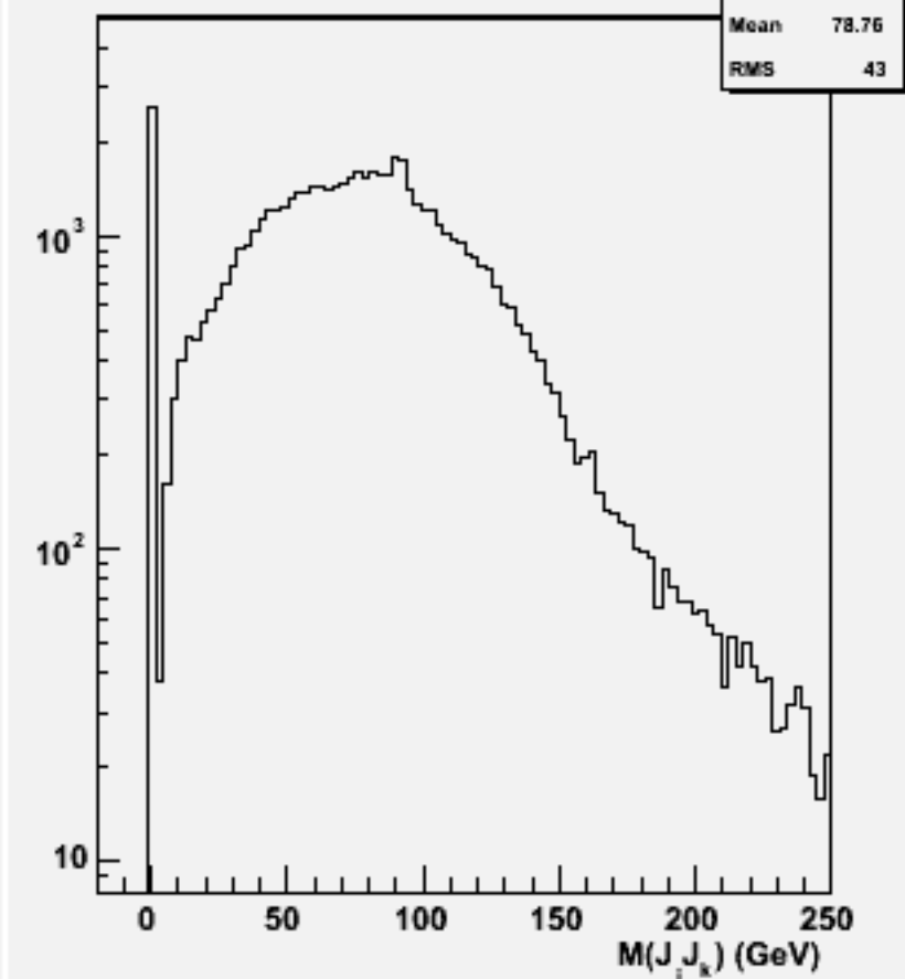
2jets mass(All comb)w101216 bbn2e2e1n1_o
