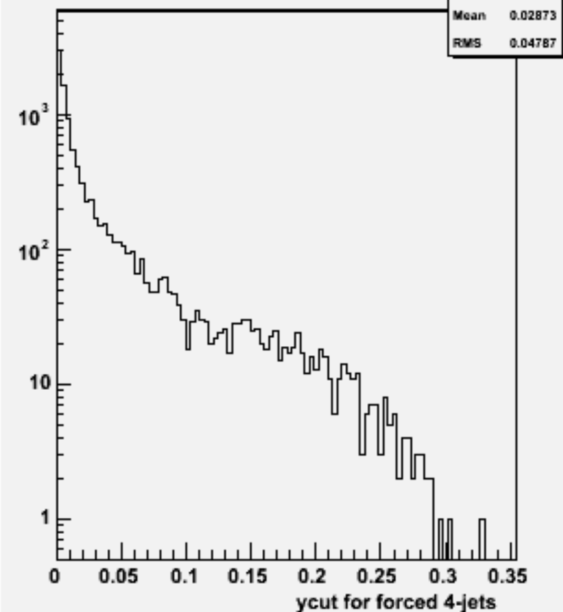
Ycut for 4-jets :w101216 bbn2e2e1n1_o
