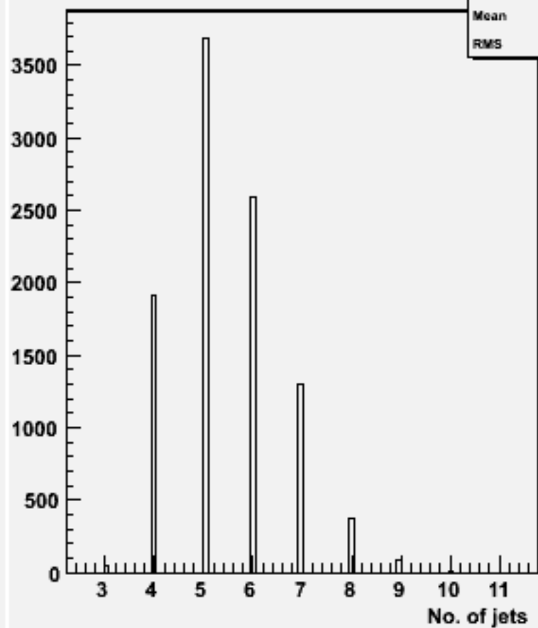
No. jets (ycut=0.001) : w101216 bbn2e2e1n1_o
