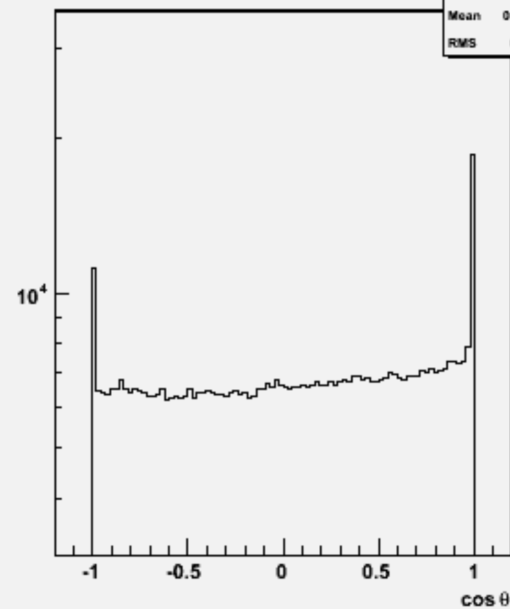
Particle cosθ : w101216 bbn2e2e1n1_o
