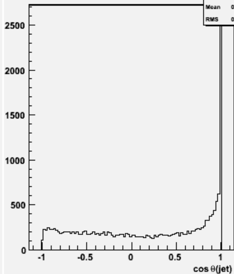
cos \theta for 2-jets :w101216 bbn2e2e1n1_o
