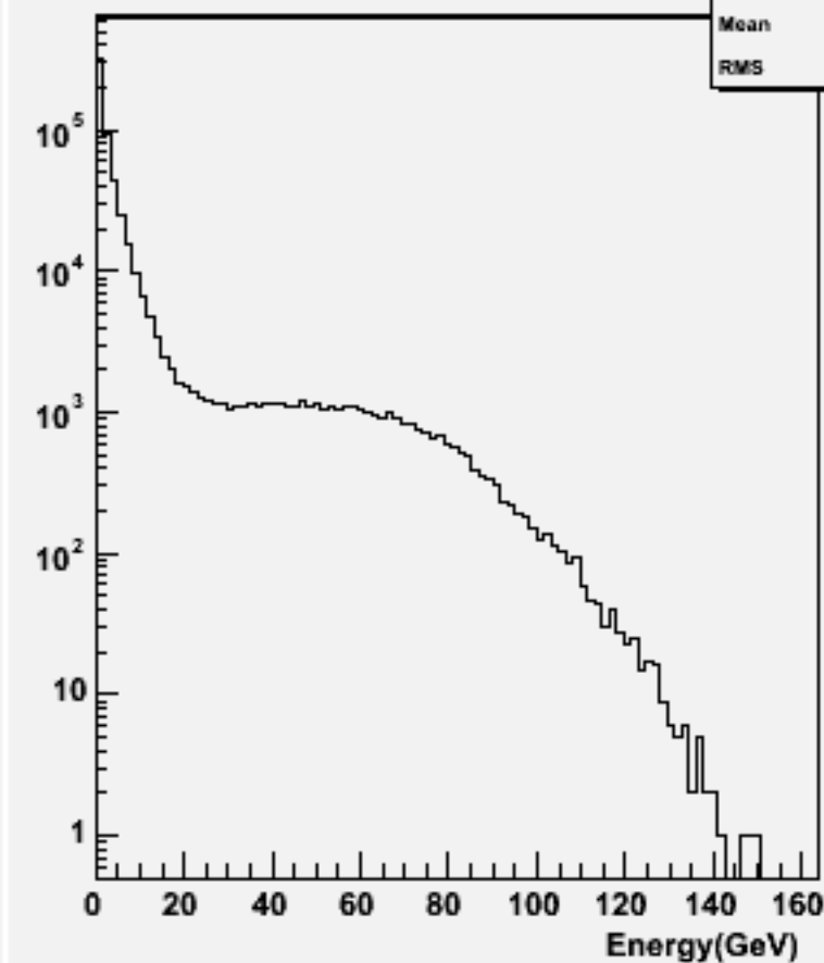
Start point R : w101216 bbn2e2e1n1_o
