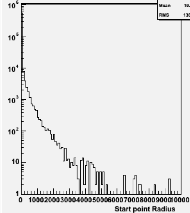
Start point R : w101216 bbn2e2e1n1_o
