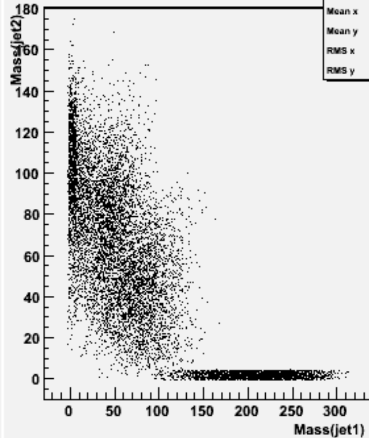
Jet mass for forced 2-jets : w101216 bbn2e2e1n1_o
