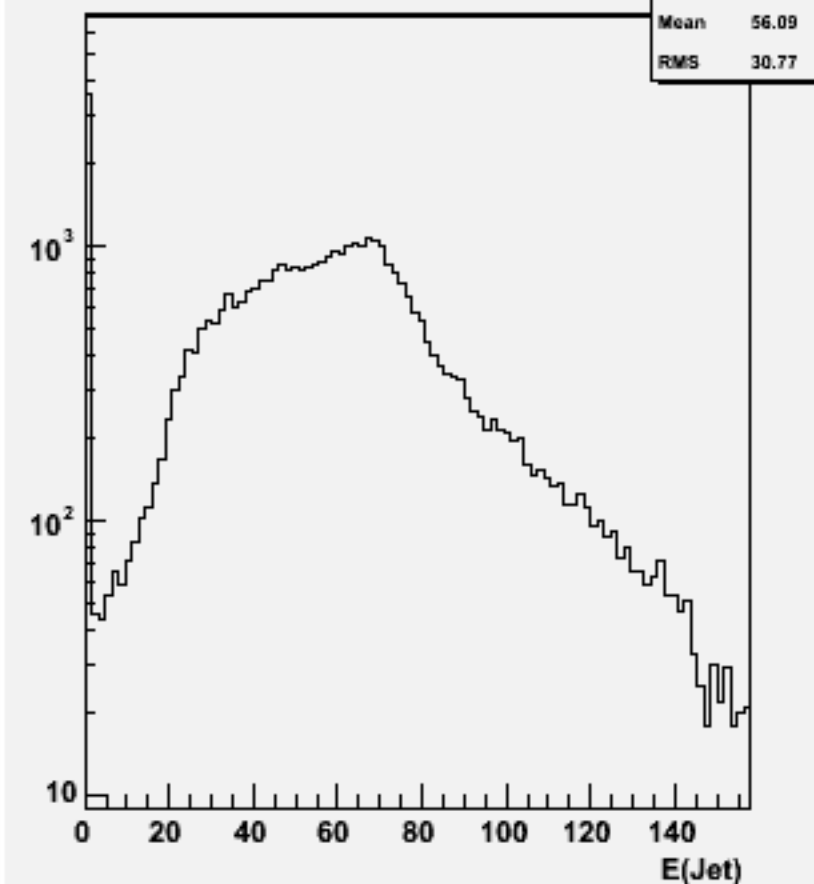
Jet energies(All jets)w101216 bbn2e2e1n1_o
