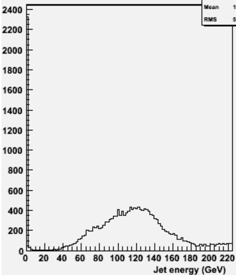
energy for 2-jets :w101216 bbn2e2e1n1_o
