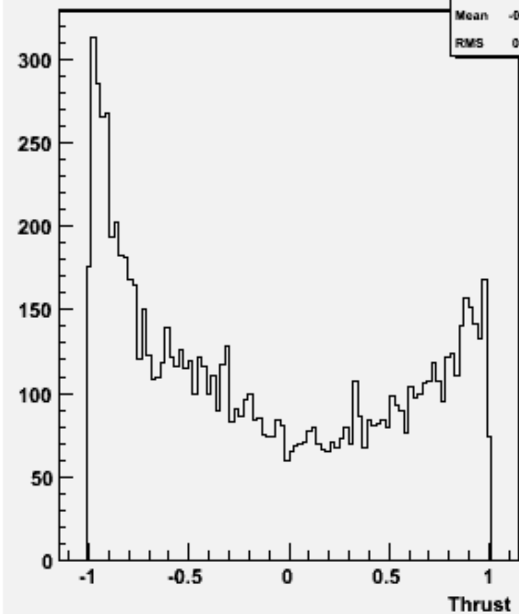
cos \Theta (thrust) w101216 bbn2e2e1n1_o
