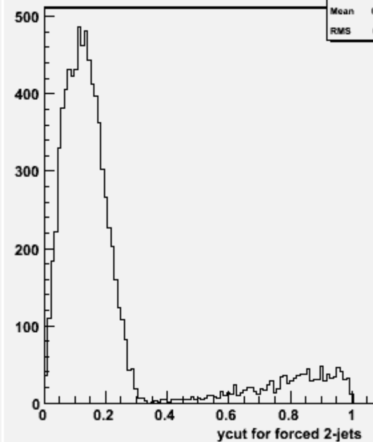
Ycut for 2-jets :w101216 bbn2e2e1n1_o
