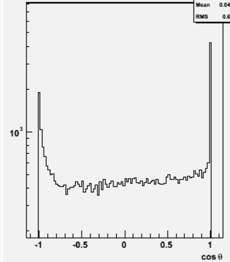
Jet cos \theta (All jets)w101212 bbn1e1sc_o
