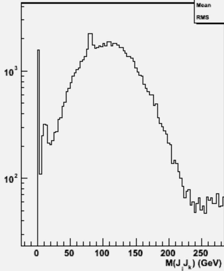
2jets mass(All comb)w101212 bbn1e1sc_o
