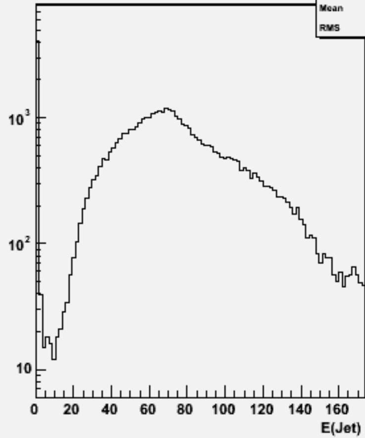
Jet energies(All jets)w101212 bbn1e1sc_o
