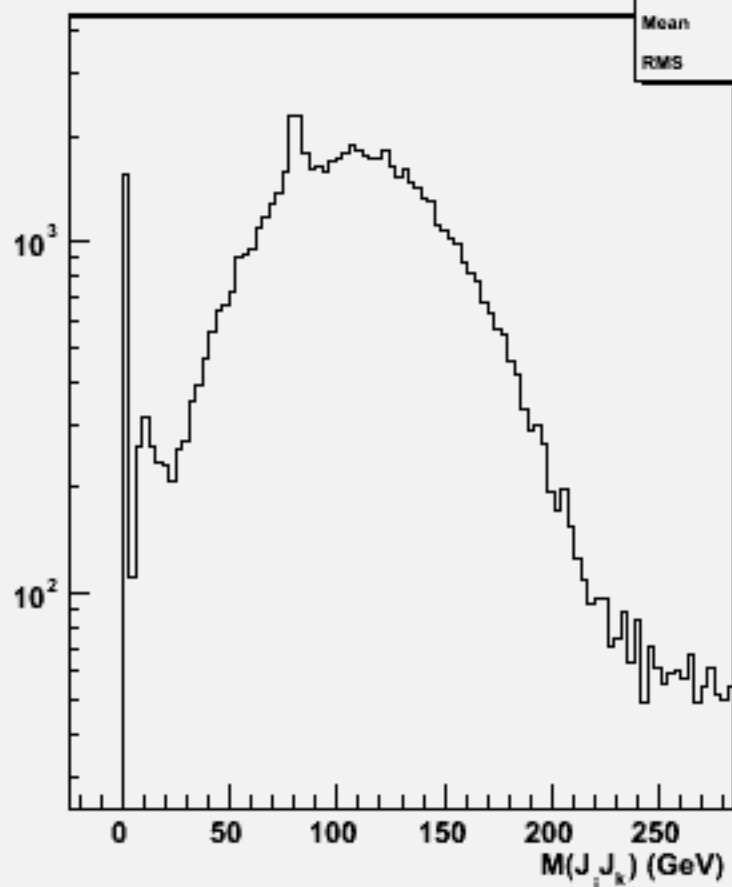
2jets mass(All comb)w101208 bbn1e1du_o
