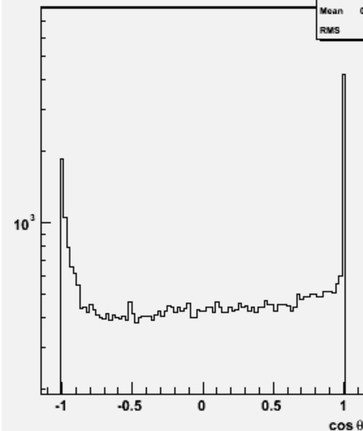
Jet cos \theta (All jets)w101208 bbn1e1du_o
