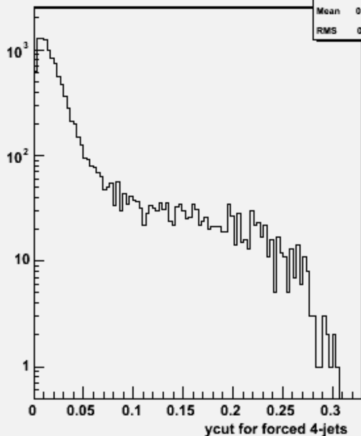
Ycut for 4-jets :w101208 bbn1e1du_o
