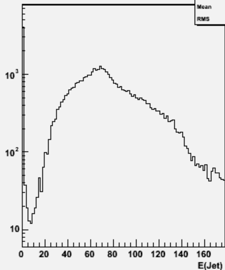
Jet energies(All jets)w101208 bbn1e1du_o
