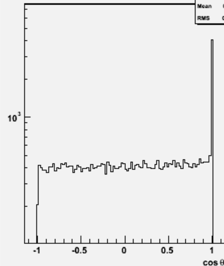
Jet cos \theta (All jets)w101205 bbn1e1e3n3_o
