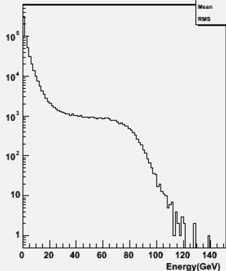
Particle Energy : w101205 bbn1e1e3n3_o
