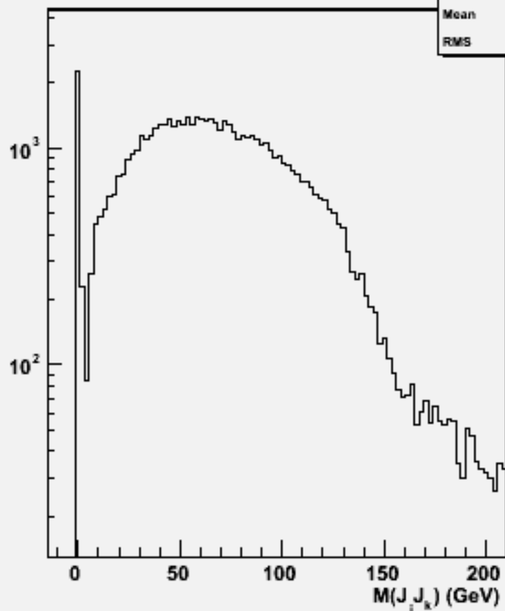
2jets mass(All comb)w101205 bbn1e1e3n3_o
