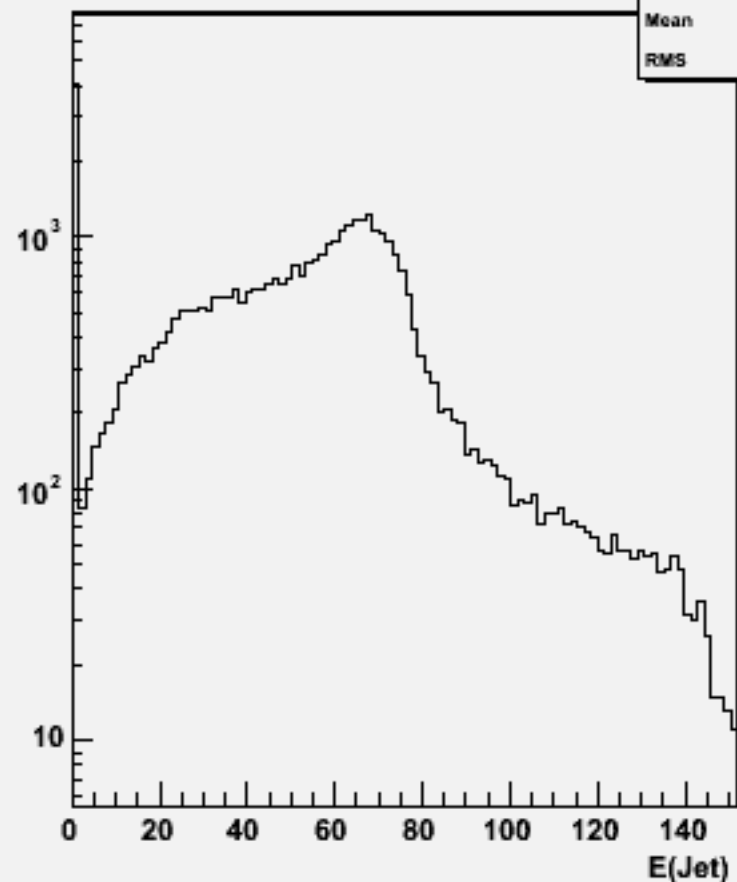
Jet energies(All jets)w101205 bbn1e1e3n3_o
