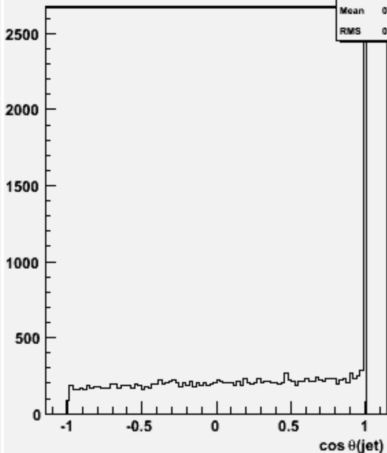
cos \theta for 2-jets :w101205 bbn1e1e3n3_o
