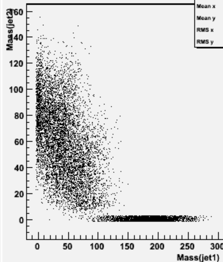
Jet mass for forced 2-jets : w101205 bbn1e1e3n3_o
