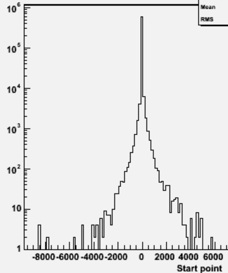
Start point Z : w101205 bbn1e1e3n3_o
