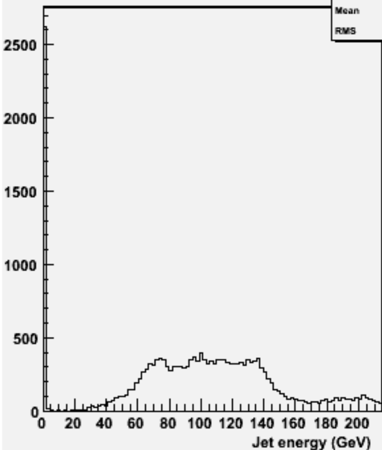
energy for 2-jets :w101205 bbn1e1e3n3_o
