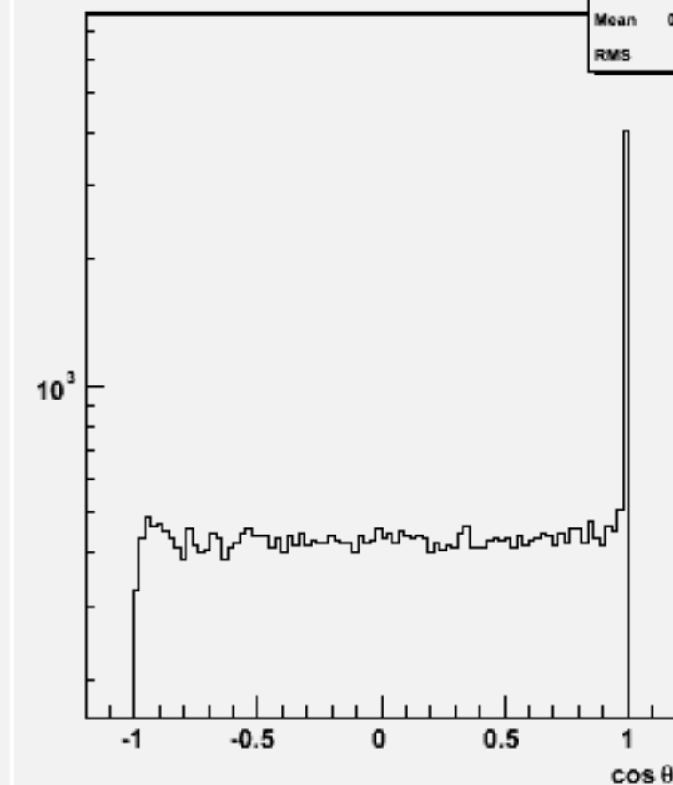
Jet cos \theta (All jets)w101201 bbn1e1e2n2_o
