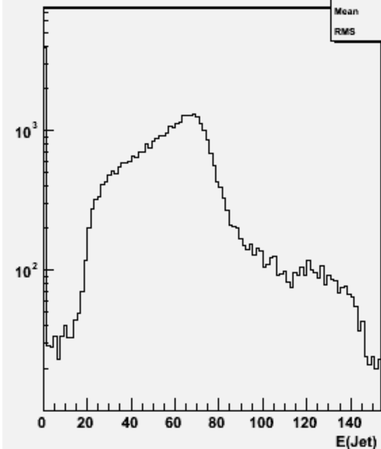
Jet energies(All jets)w101201 bbn1e1e2n2_o
