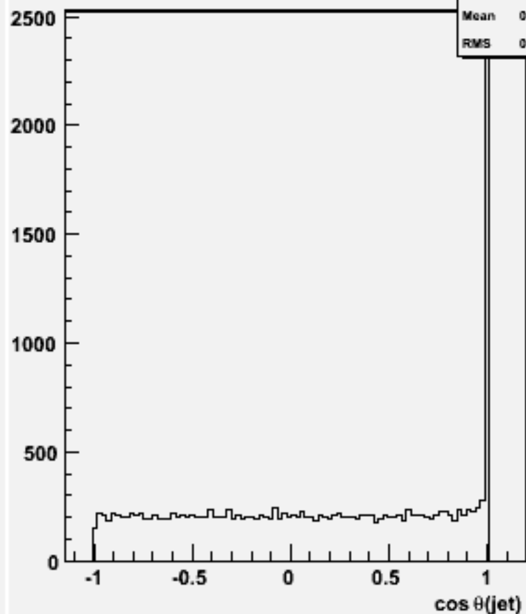
cos \theta for 2-jets :w101201 bbn1e1e2n2_o
