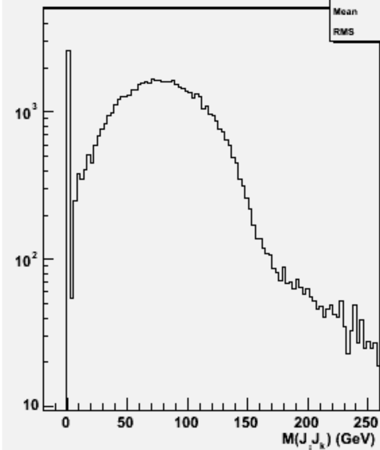
2jets mass(All comb)w101201 bbn1e1e2n2_o
