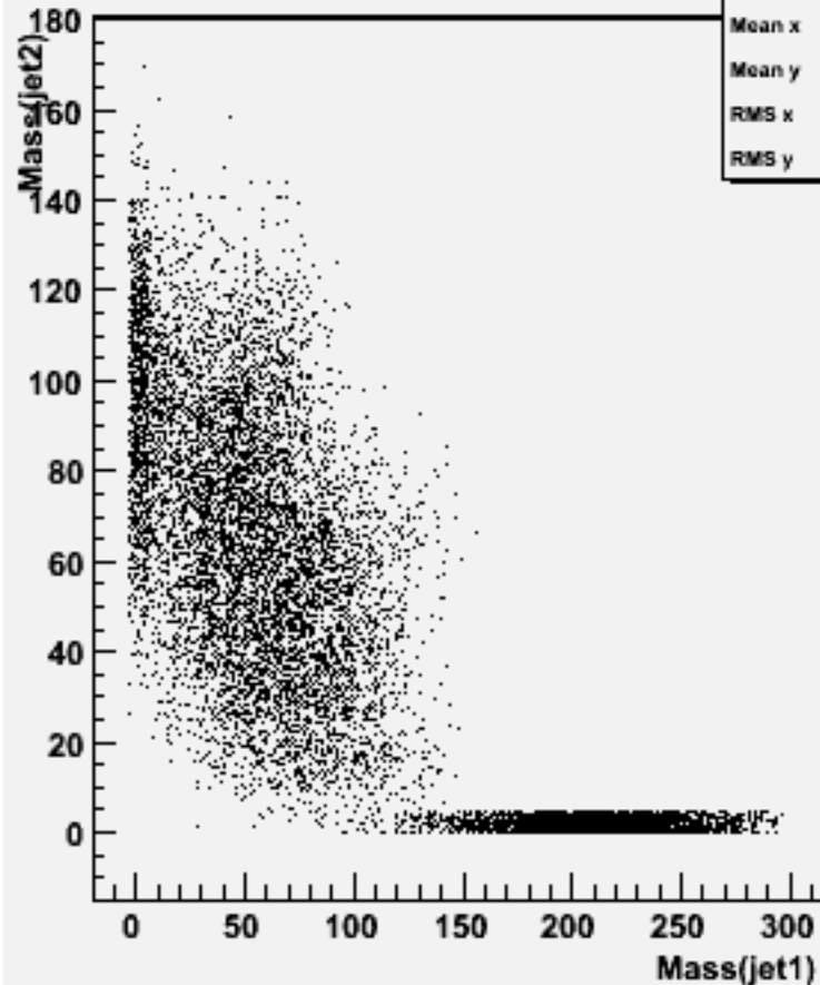
Jet mass for forced 2-jets : w101201 bbn1e1e2n2_o
