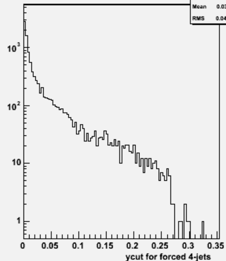
Ycut for 4-jets :w101201 bbn1e1e2n2_o
