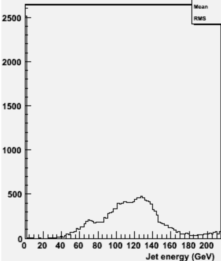
energy for 2-jets :w101201 bbn1e1e2n2_o
