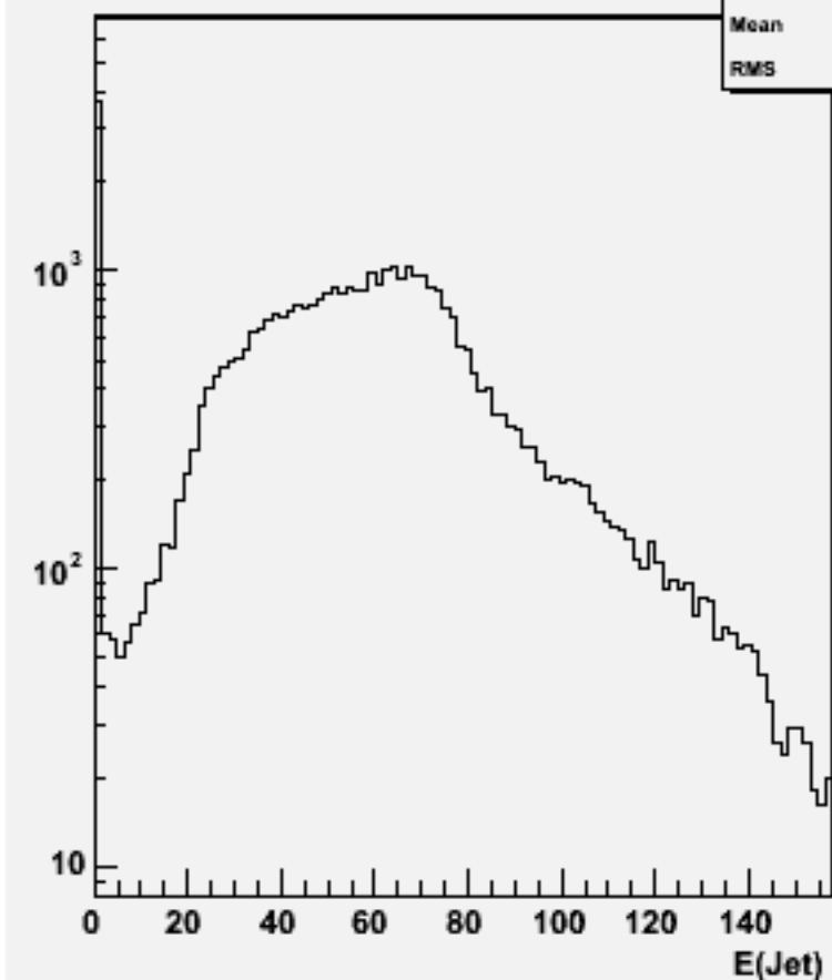
Jet energies(All jets)w101200 bbn1e1e2n2_o
