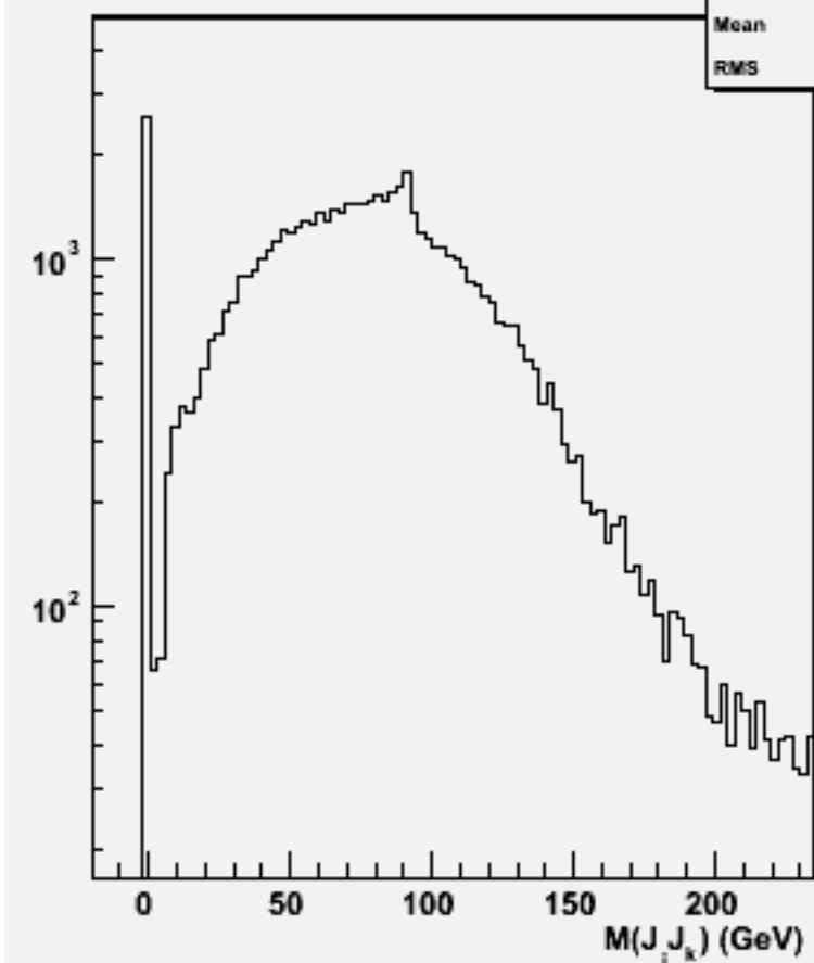
2jets mass(All comb)w101200 bbn1e1e2n2_o
