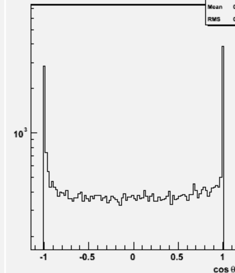
Jet cos \theta (All jets)w101200 bbn1e1e2n2_o
