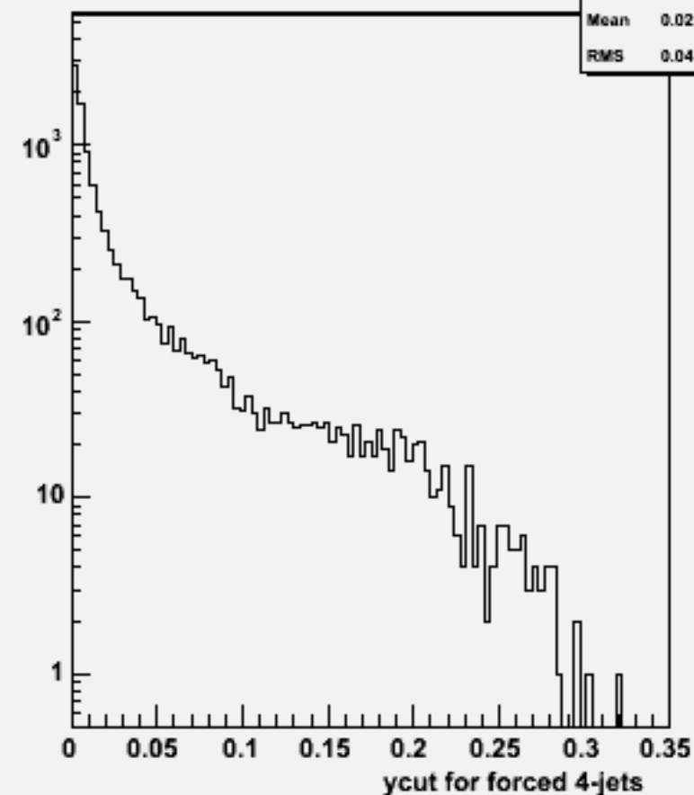
Ycut for 4-jets :w101200 bbn1e1e2n2_o
