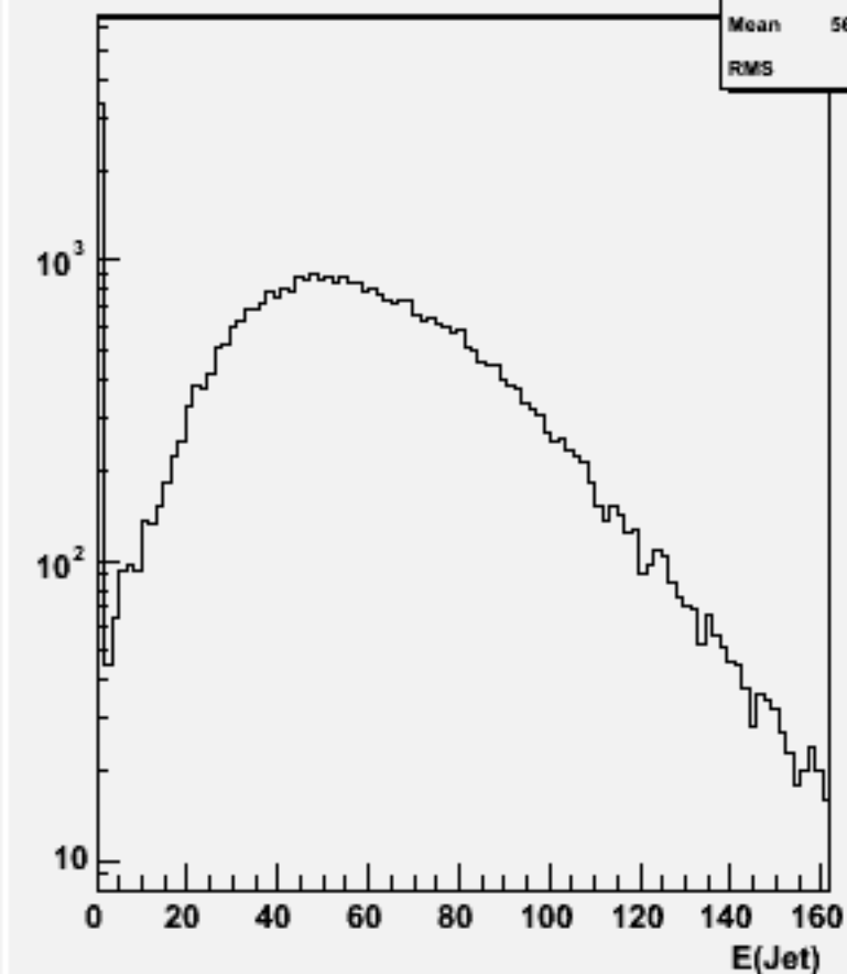
Jet energies(All jets)w101199 bbn1e1e2n2_o
