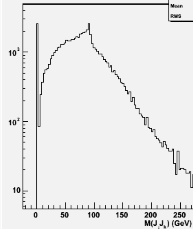
2jets mass(All comb)w101199 bbn1e1e2n2_o
