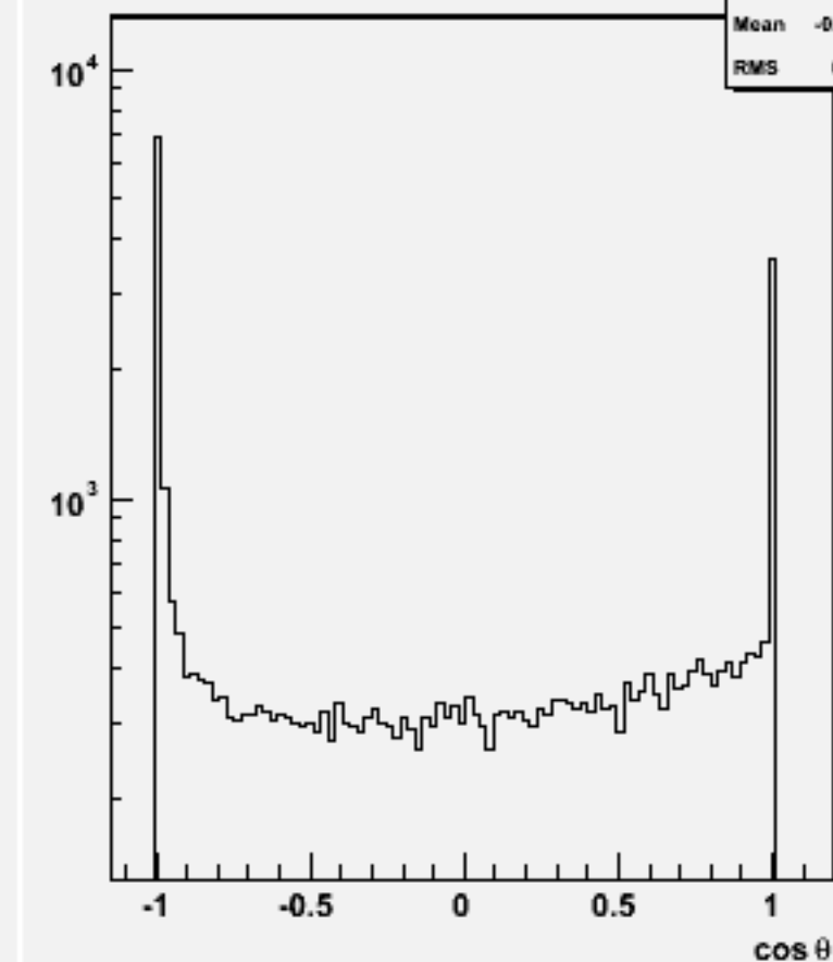
Jet cos \theta (All jets)w101199 bbn1e1e2n2_o
