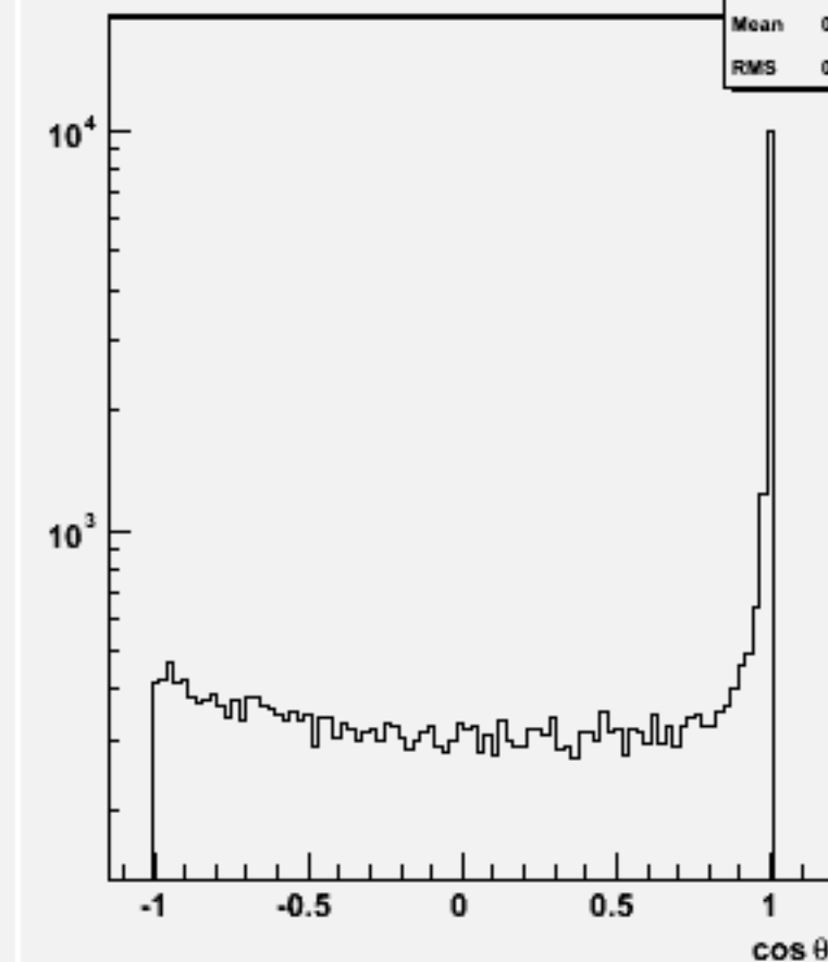
Jet cos \theta (All jets)w101198 bbn1e1e1n1_o
