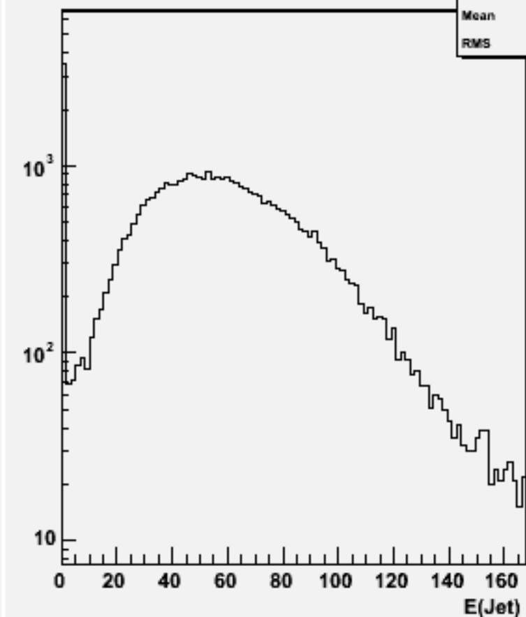
Jet energies(All jets)w101198 bbn1e1e1n1_o
