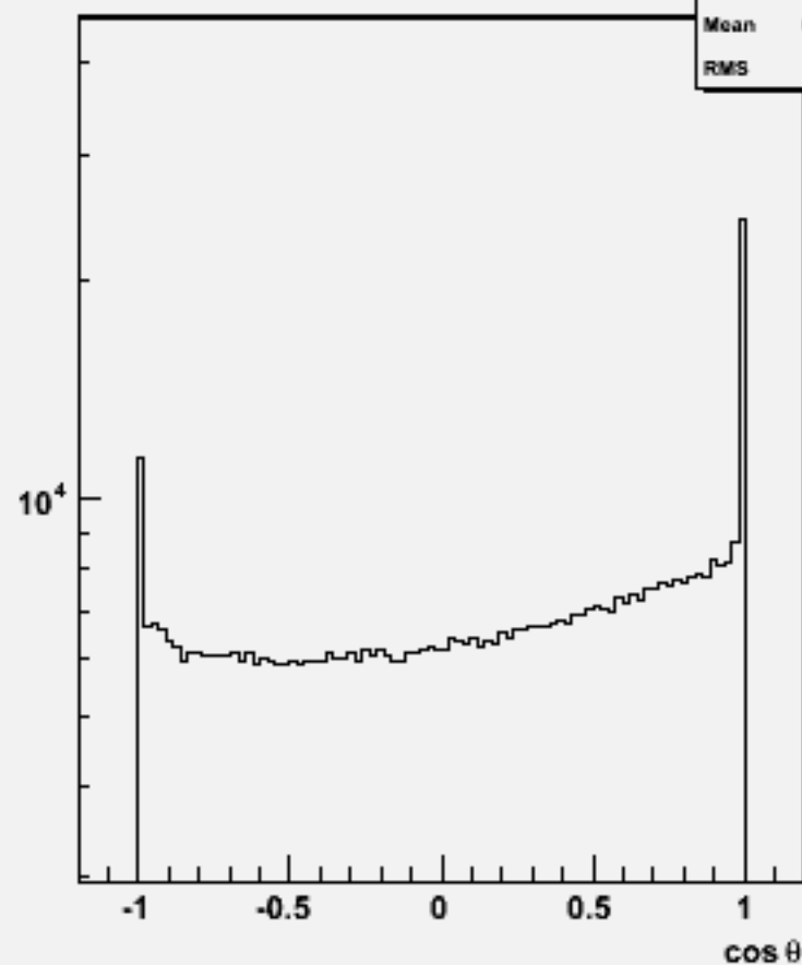
Particle cosθ : w101198 bbn1e1e1n1_o
