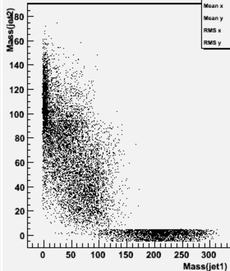
Jet mass for forced 2-jets : w101198 bbn1e1e1n1_o
