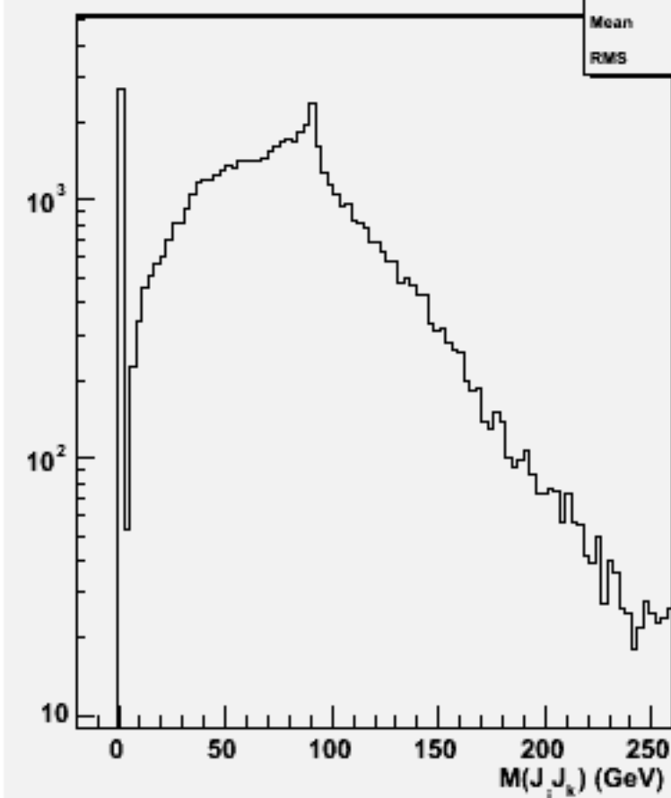
2jets mass(All comb)w101198 bbn1e1e1n1_o
