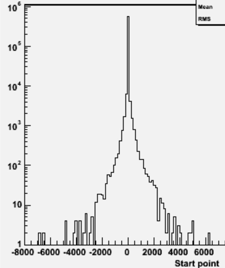
Start point Z : w101198 bbn1e1e1n1_o
