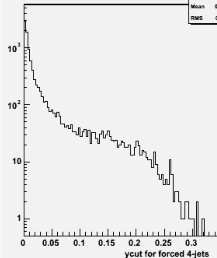
Ycut for 4-jets :w101198 bbn1e1e1n1_o
