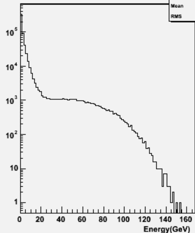
Particle Energy : w101198 bbn1e1e1n1_o
