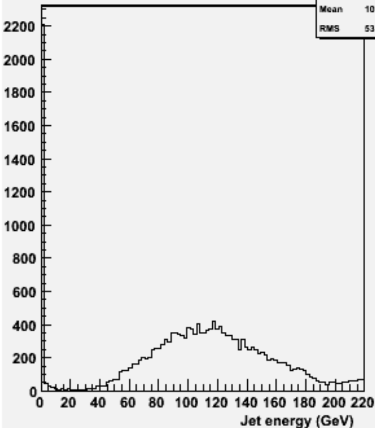
energy for 2-jets :w101198 bbn1e1e1n1_o
