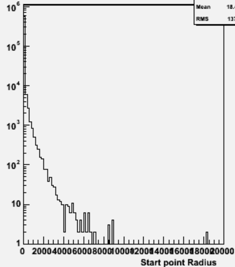
Start point R : w101198 bbn1e1e1n1_o
