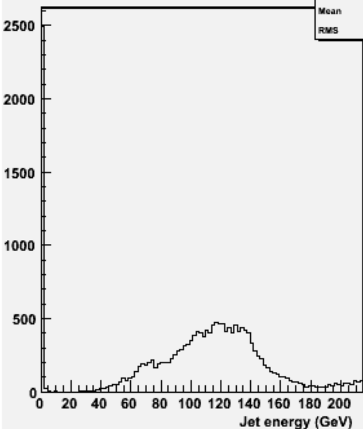
energy for 2-jets :w101197 bbn1e1e1n1_o
