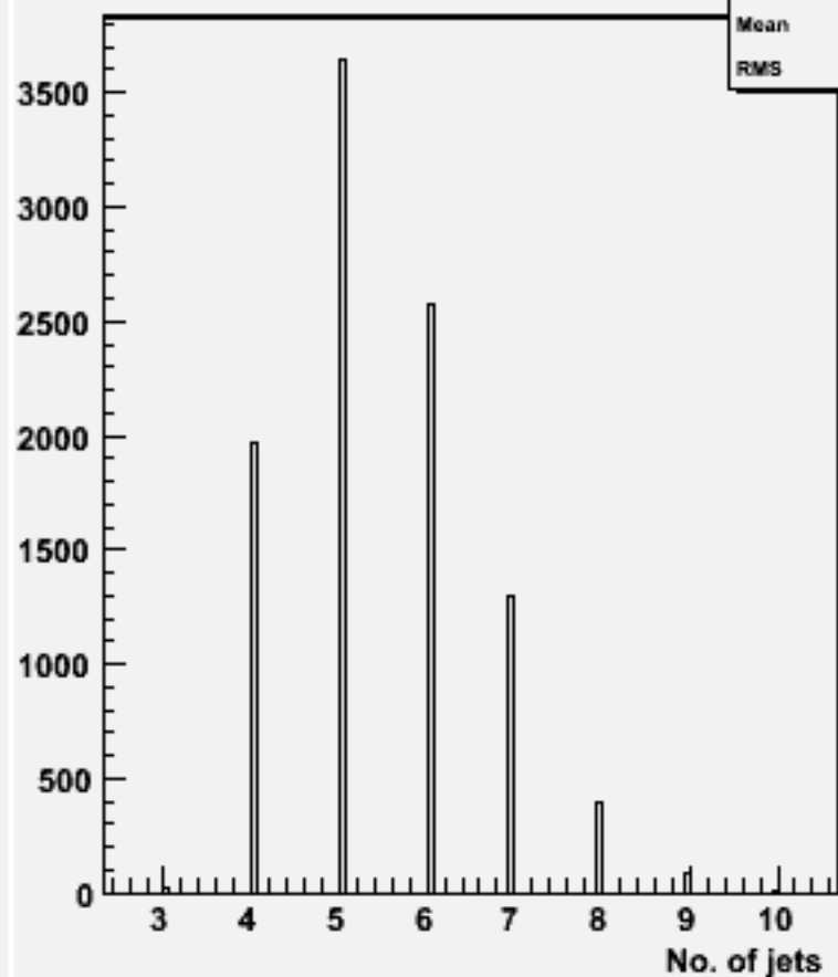
No. jets (ycut=0.001) : w101197 bbn1e1e1n1_o
