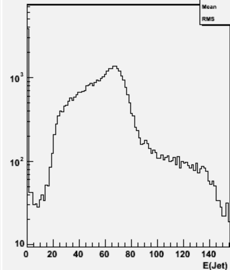
Jet energies(All jets)w101197 bbn1e1e1n1_o
