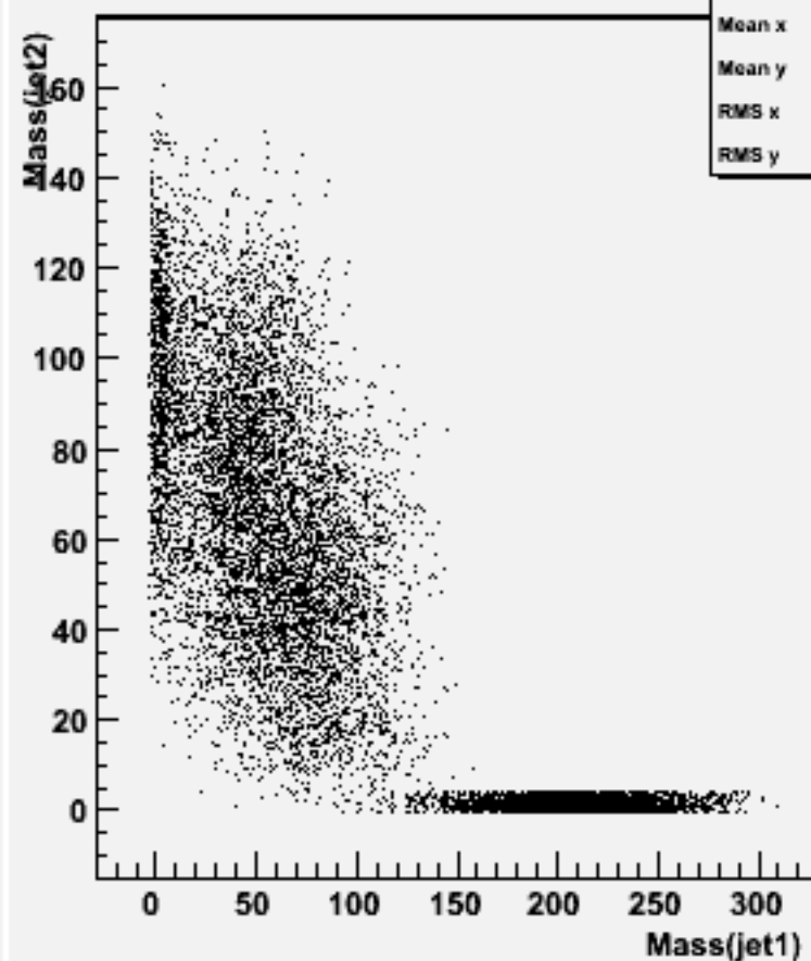
Jet mass for forced 2-jets : w101197 bbn1e1e1n1_o
