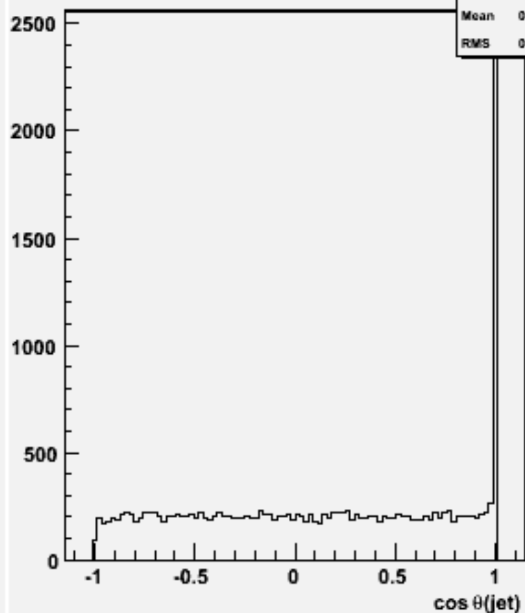
cos \Theta for 2-jets :w101197 bbn1e1e1n1_o
