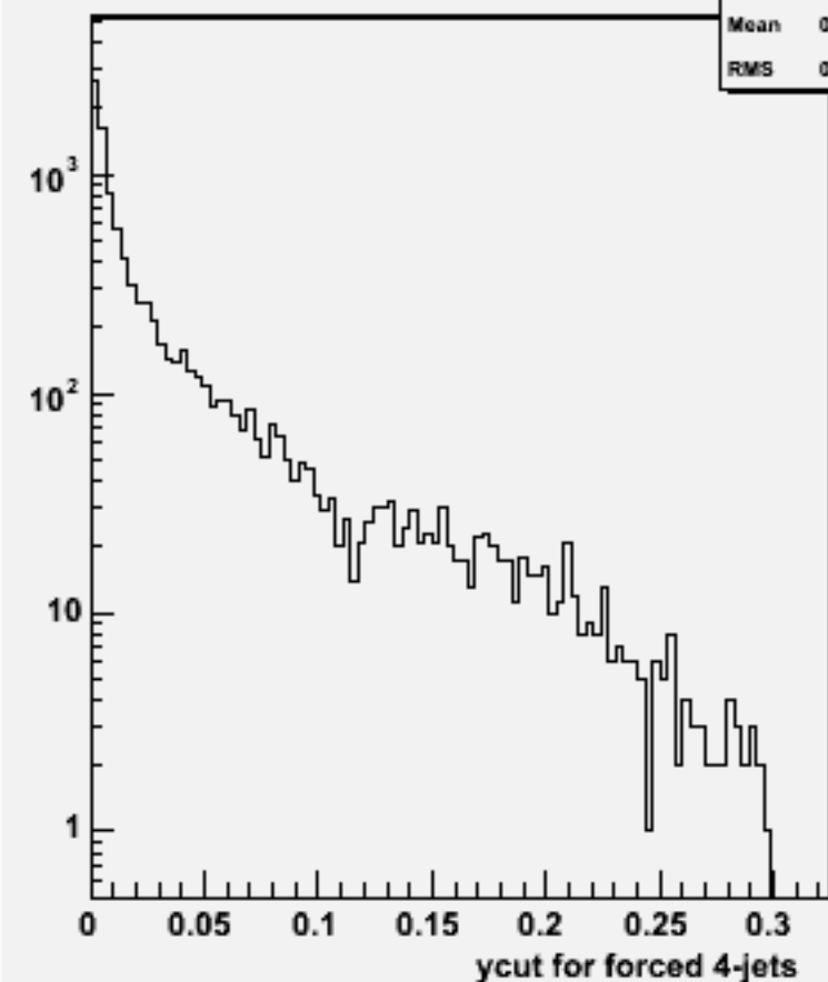
Ycut for 4-jets :w101197 bbn1e1e1n1_o
