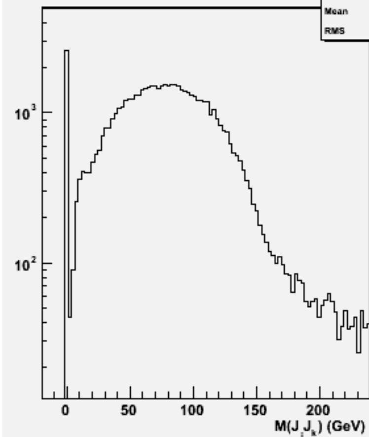
2jets mass(All comb)w101197 bbn1e1e1n1_o
