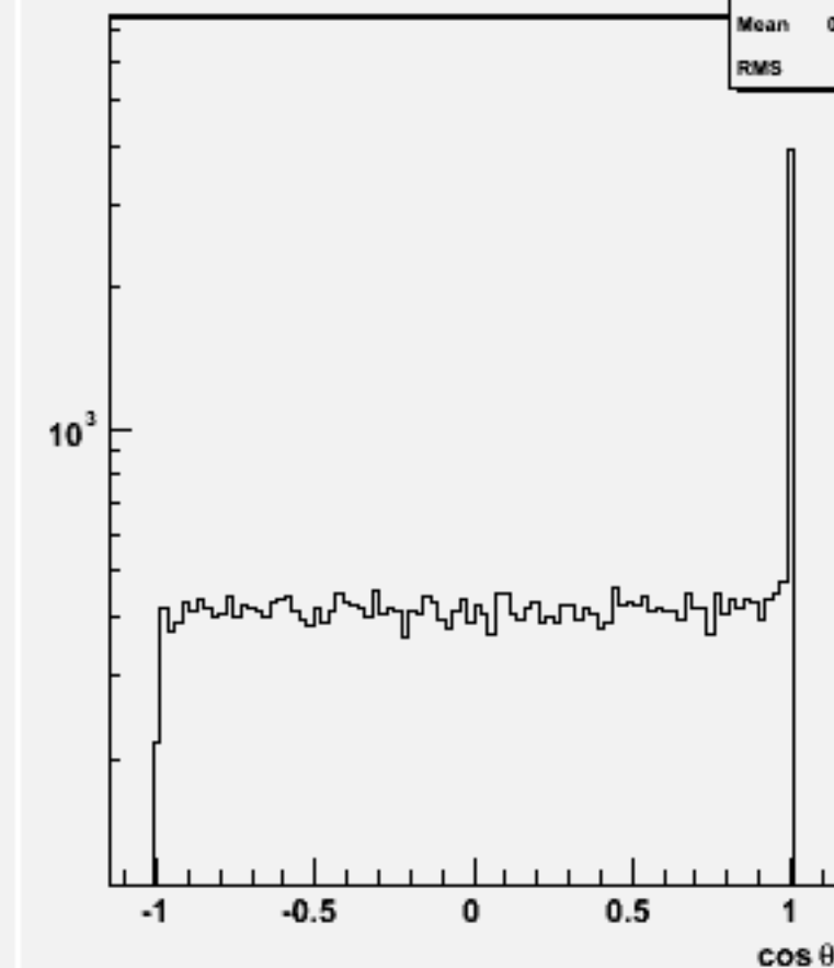
Jet cos \theta (All jets)w101197 bbn1e1e1n1_o
