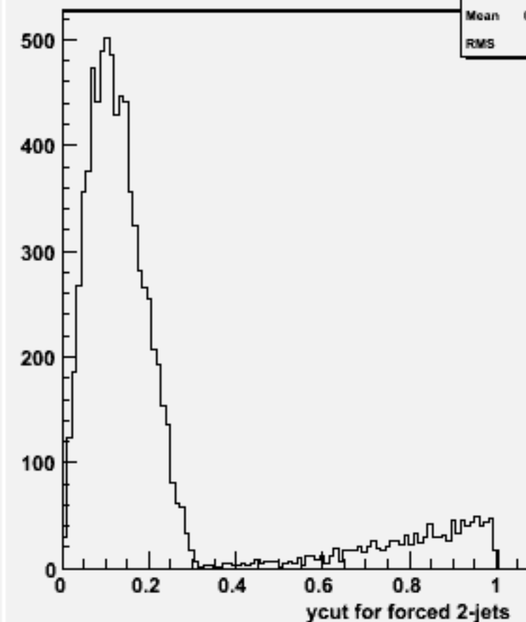
Ycut for 2-jets :w101197 bbn1e1e1n1_o
