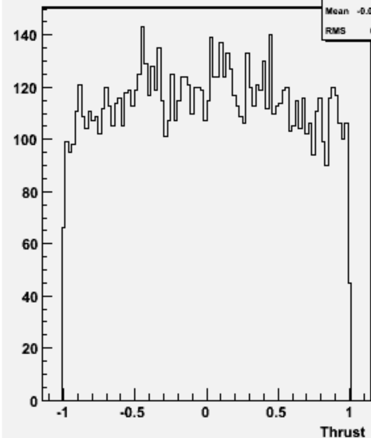
cos \Theta (thrust) w101197 bbn1e1e1n1_o
