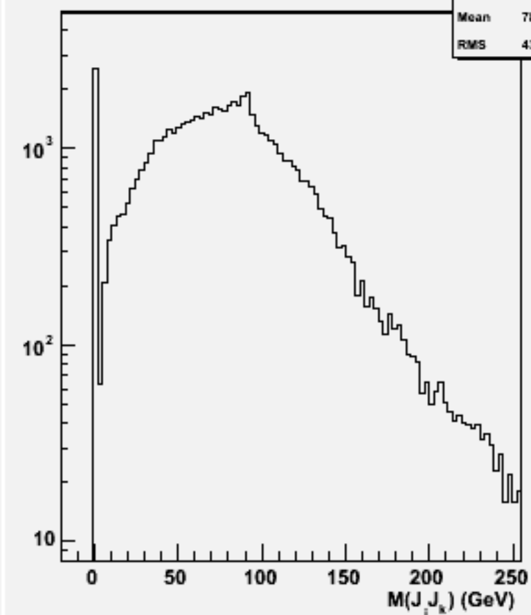
2jets mass(All comb)w101196 bbn1e1e1n1_o
