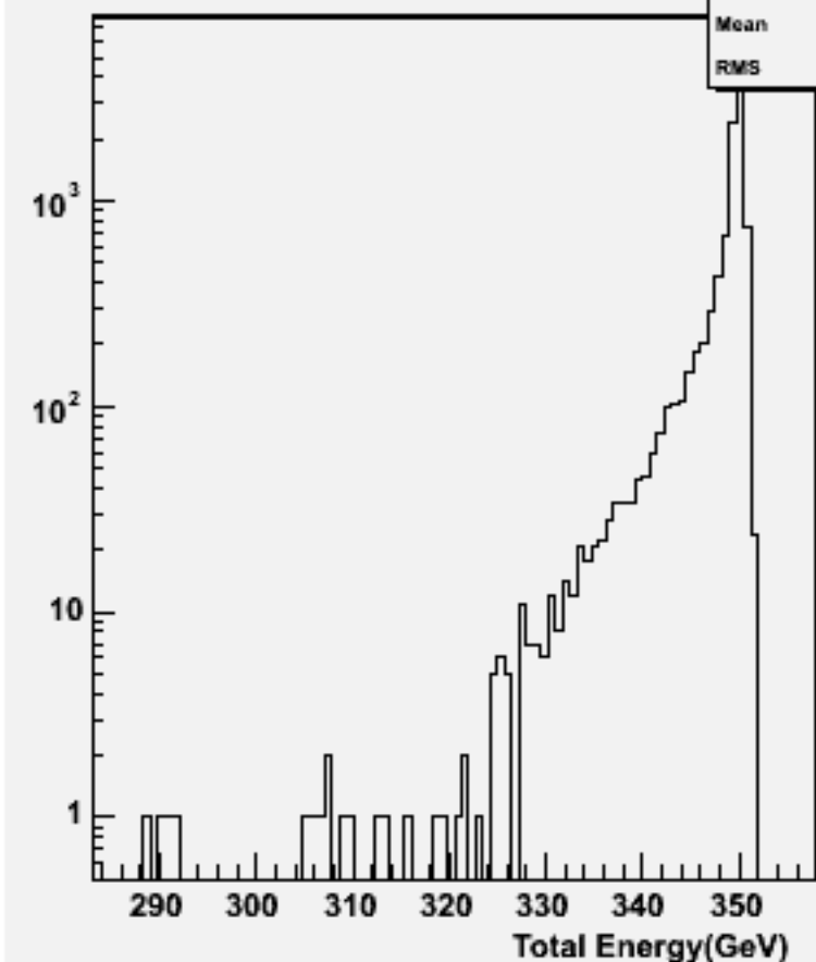
Pt Sum: w101196 bbn1e1e1n1_o
