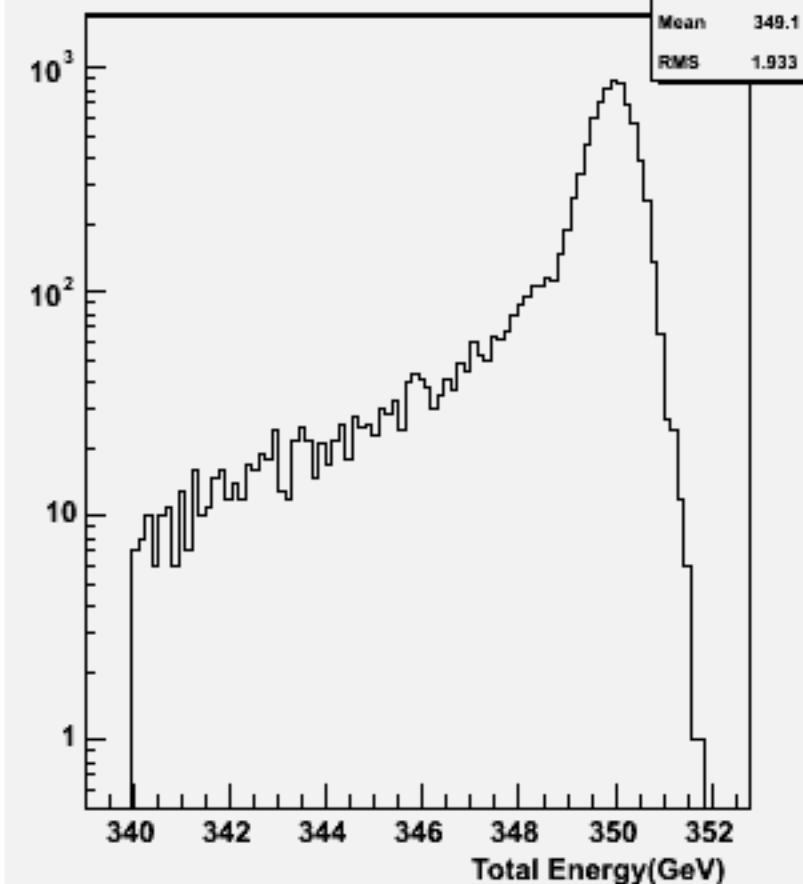
Pz Sum: w101196 bbn1e1e1n1_o
