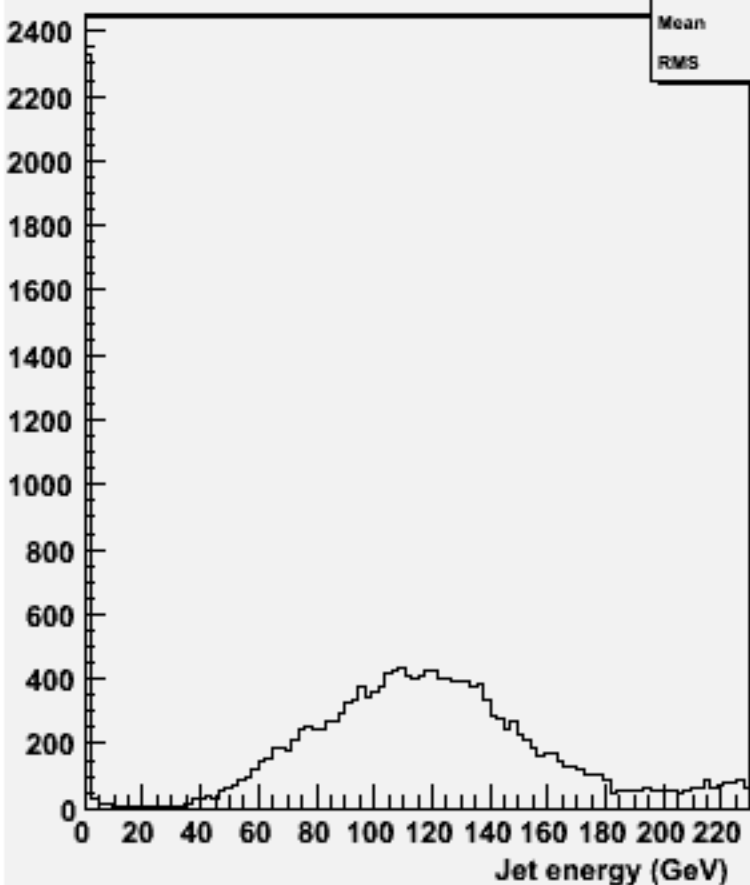
energy for 2-jets :w101196 bbn1e1e1n1_o
