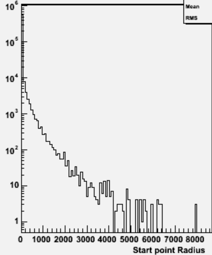
Start point R : w101196 bbn1e1e1n1_o
