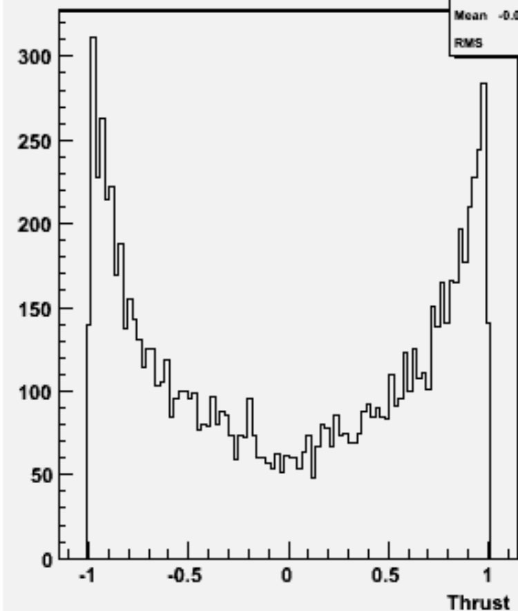
cos \Theta (thrust) w101196 bbn1e1e1n1_o
