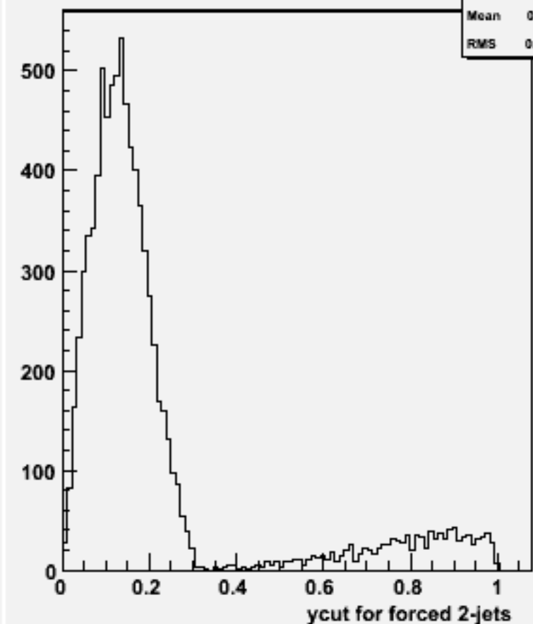
Ycut for 2-jets :w101196 bbn1e1e1n1_o
