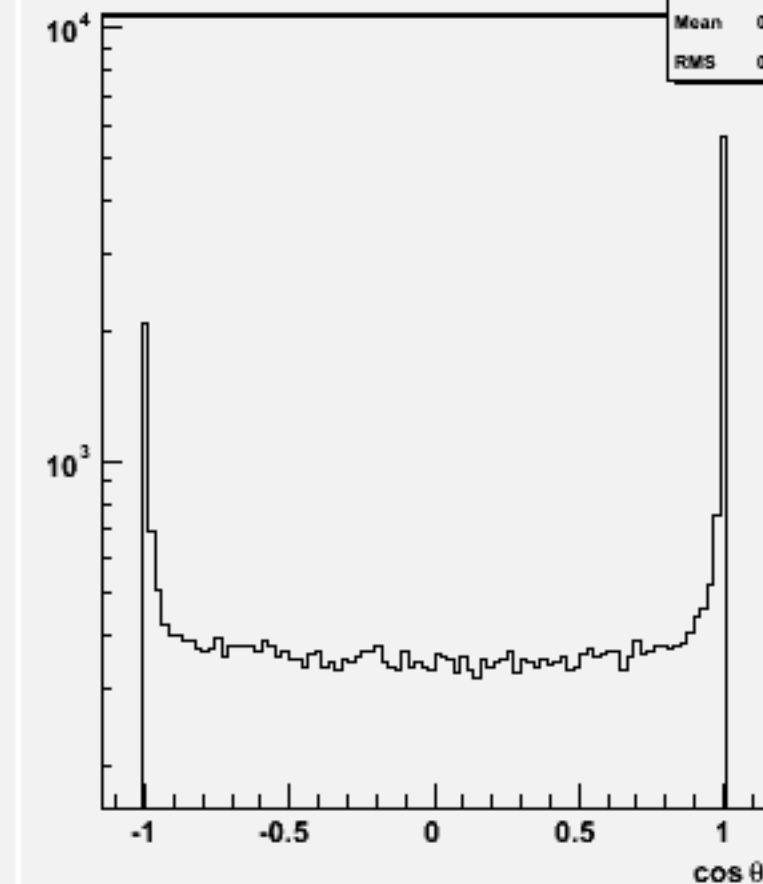
Jet cos \theta (All jets)w101196 bbn1e1e1n1_o
