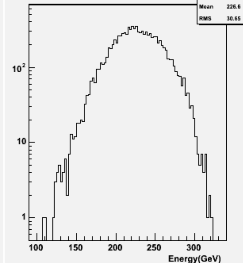
Thrust w101196 bbn1e1e1n1_o
