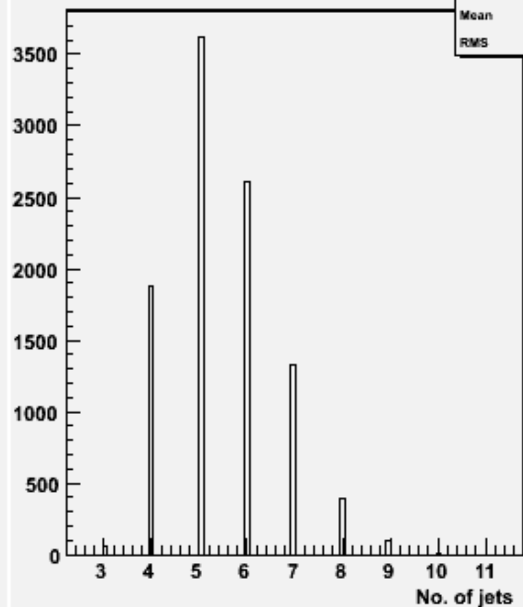
No. jets (ycut=0.001) : w101196 bbn1e1e1n1_o
