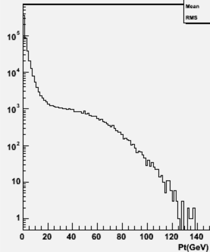
Start point Z : w101196 bbn1e1e1n1_o
