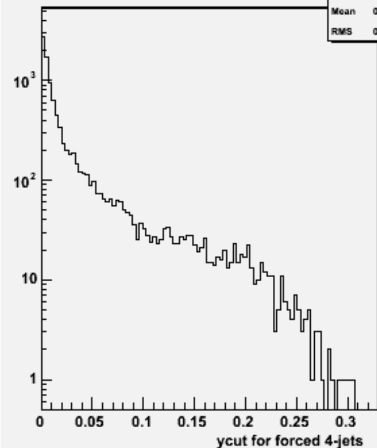
Ycut for 4-jets :w101196 bbn1e1e1n1_o
