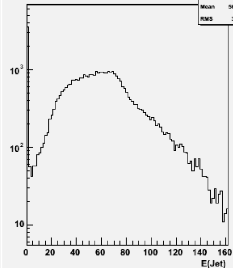
Jet energies(All jets)w101196 bbn1e1e1n1_o
