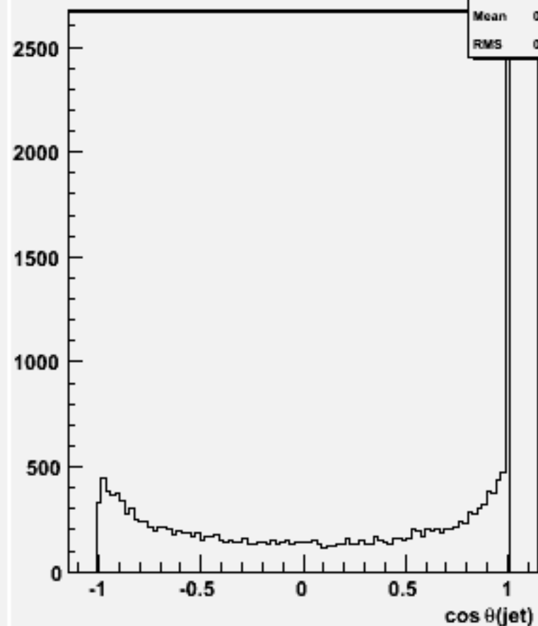
cos \theta for 2-jets :w101196 bbn1e1e1n1_o
