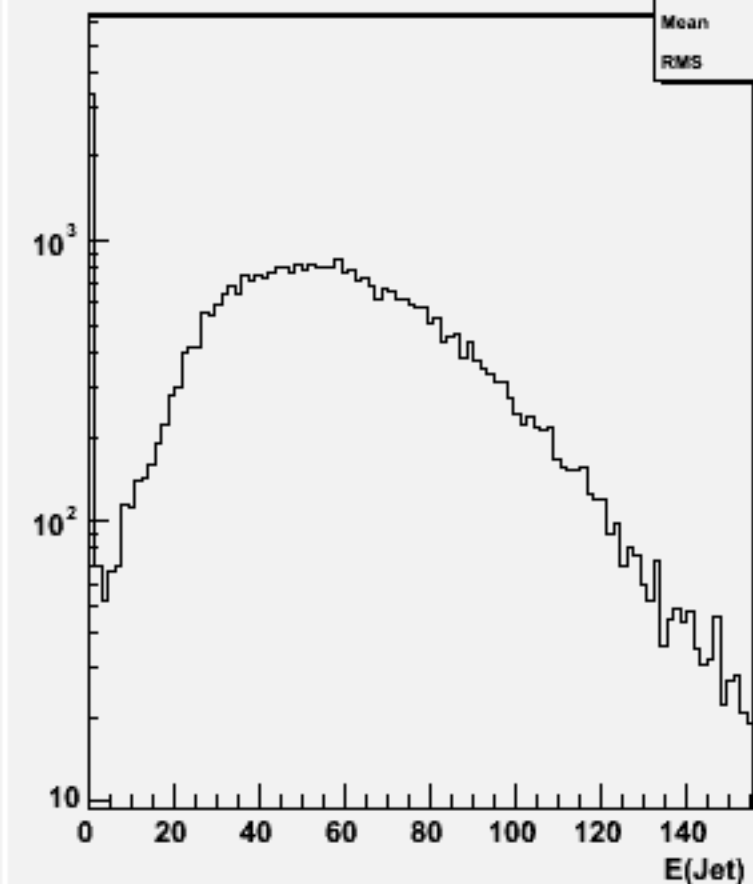
Jet energies(All jets)w101195 bbn1e1e1n1_o
