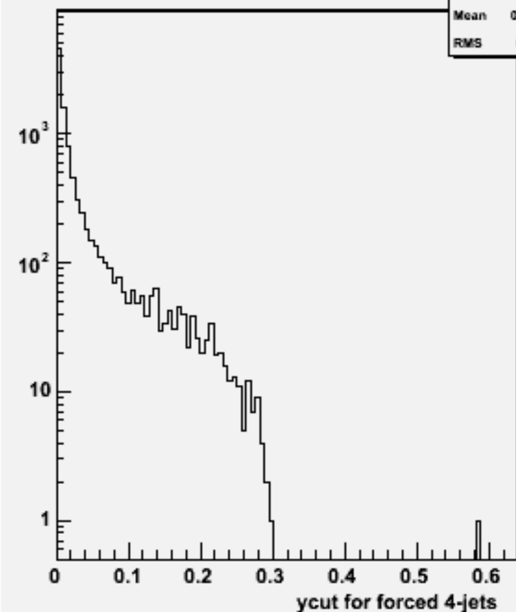
Ycut for 4-jets :w101195 bbn1e1e1n1_o
