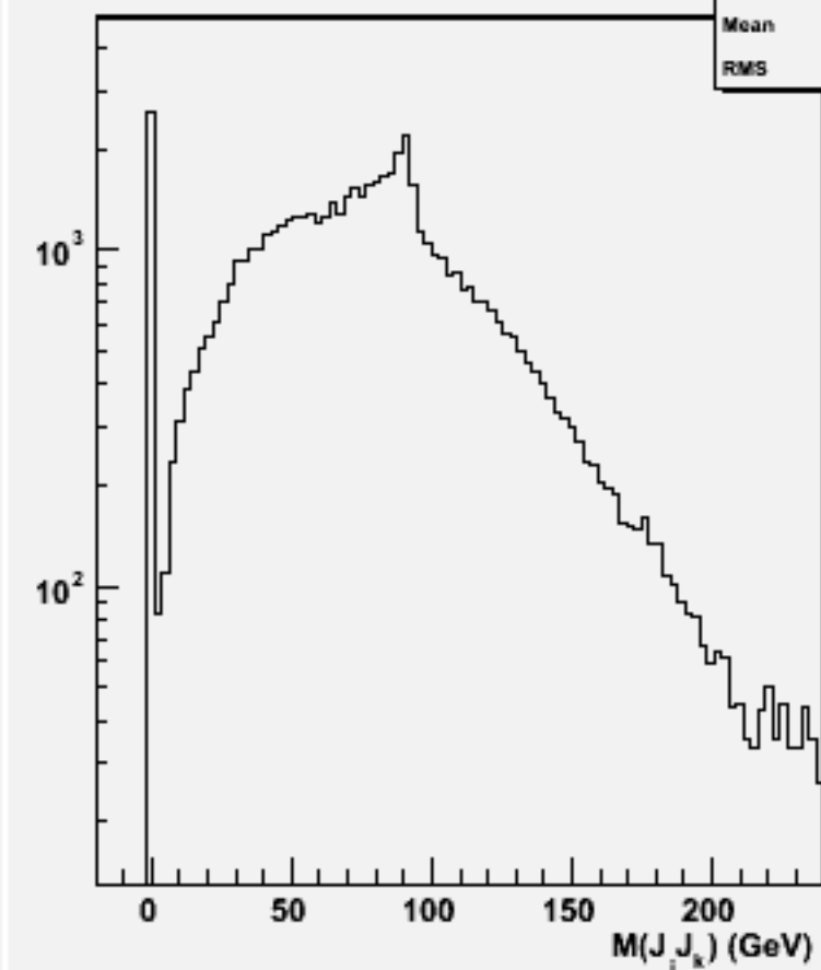
2jets mass(All comb)w101195 bbn1e1e1n1_o
