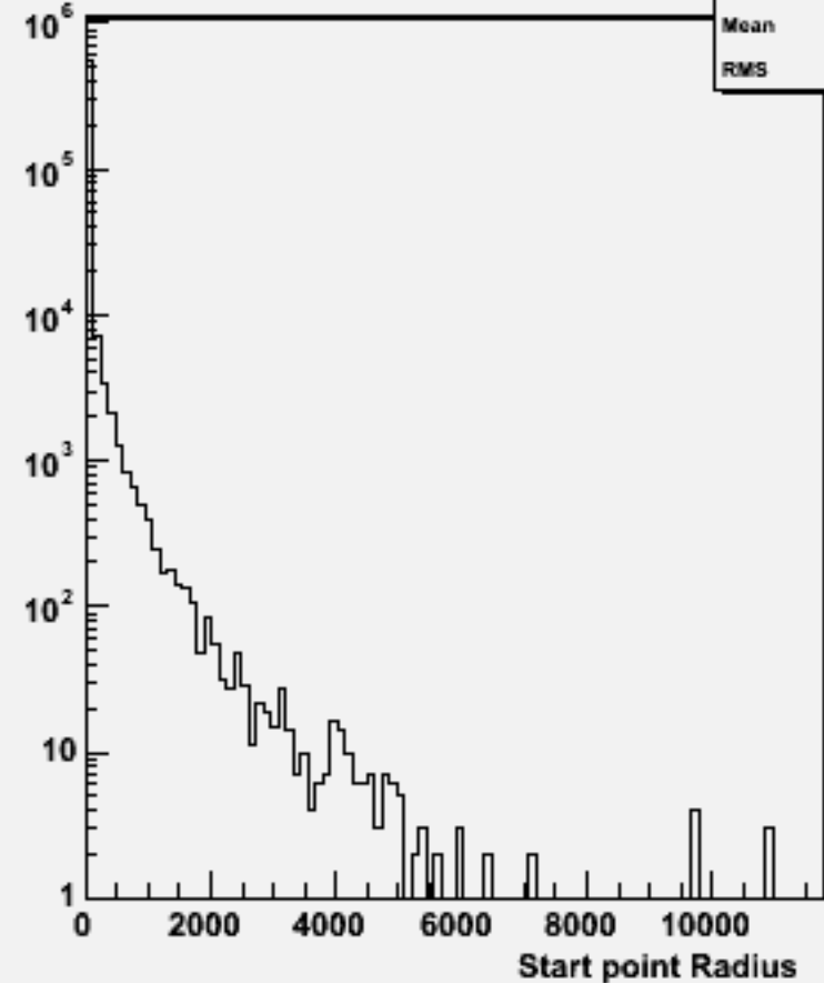
Start point R : w101195 bbn1e1e1n1_o
