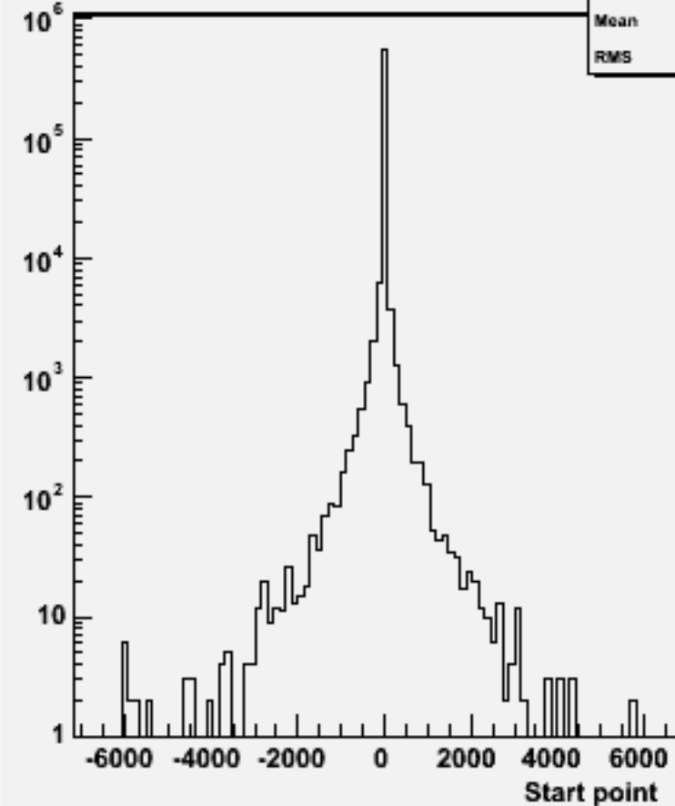
Start point Z : w101195 bbn1e1e1n1_o
