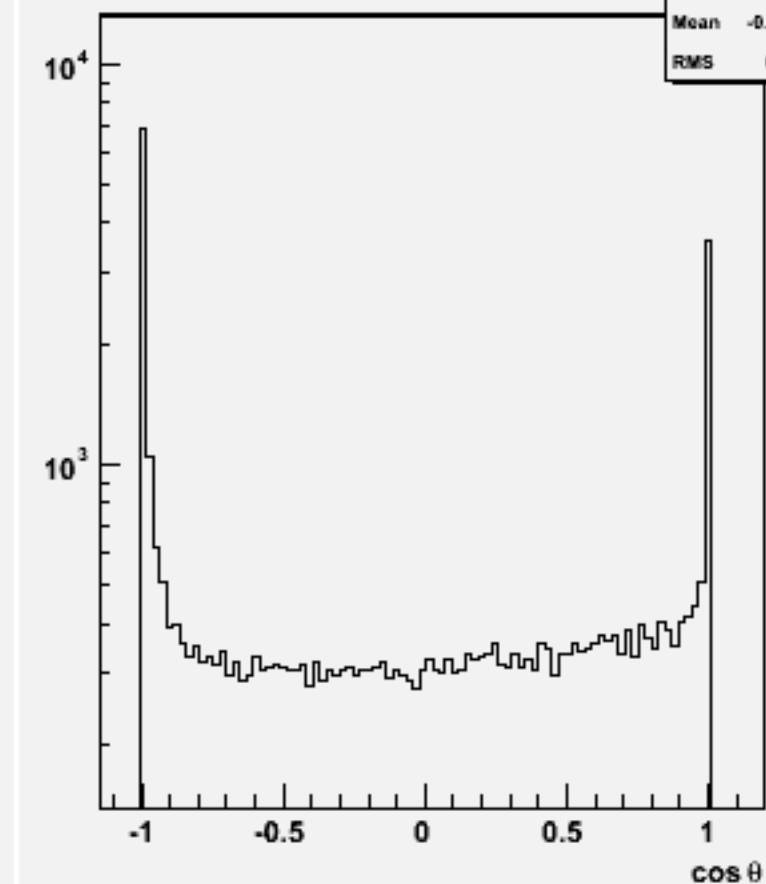
Jet cos \theta (All jets)w101195 bbn1e1e1n1_o
