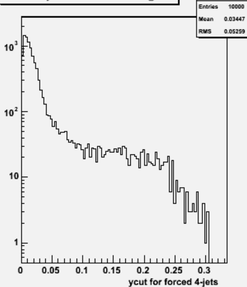
Ycut for 4-jets :w101185 sscse3n3_o
