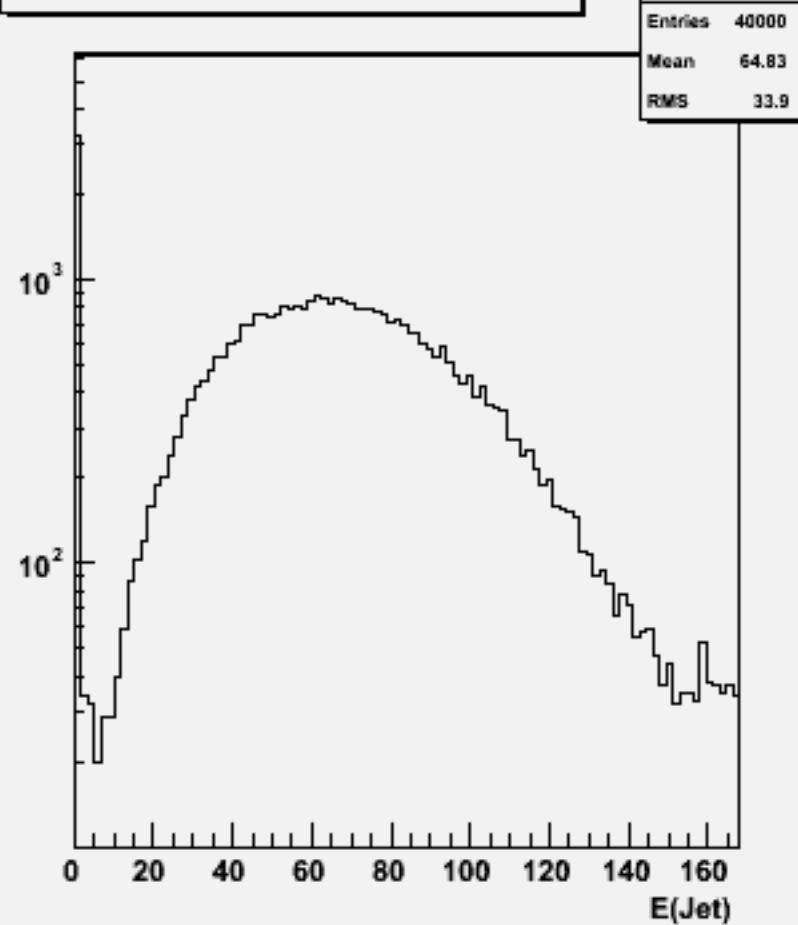
Jet energies(All jets)w101185 sscse3n3_o
