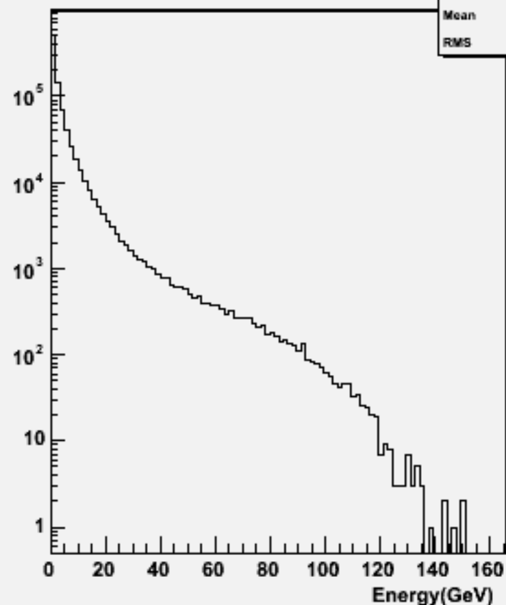
Particle Energy : w101185 sscse3n3_o
