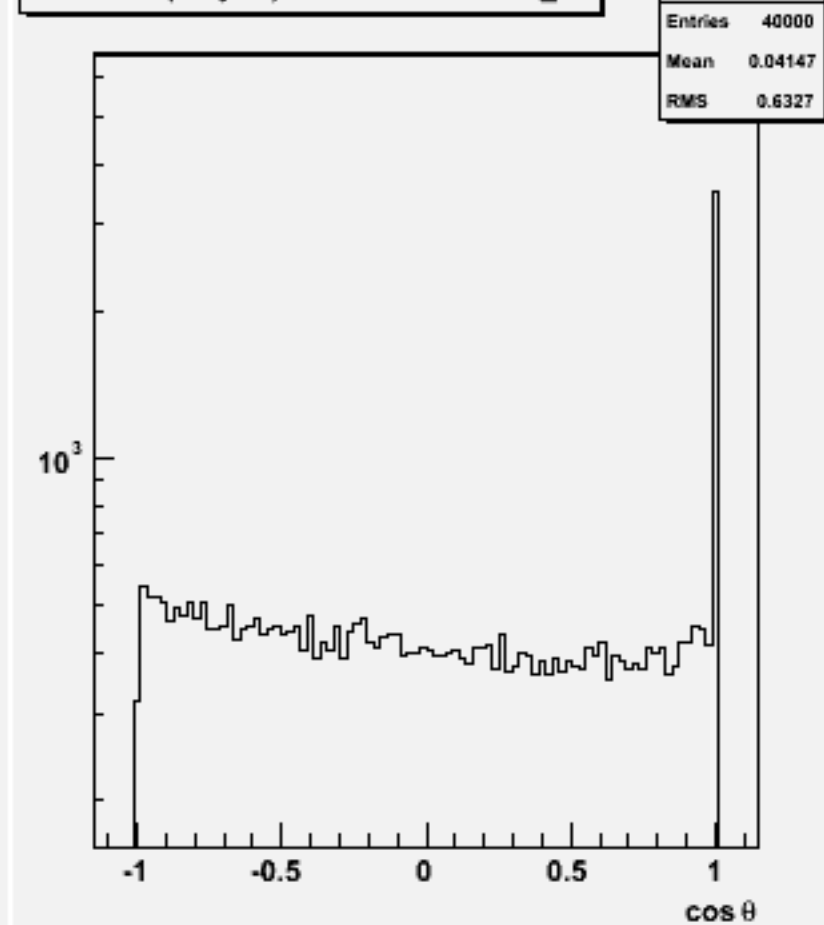
Jet cosθ (All jets)w101185 sscse3n3_o
