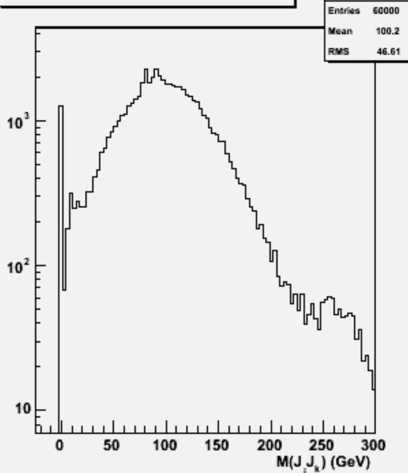
2jets mass(All comb)w101185 sscse3n3_o
