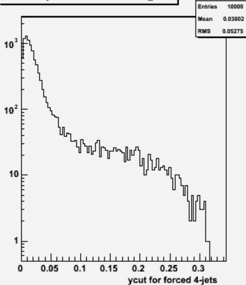
Ycut for 4-jets :w101180 sscse2n2_o
