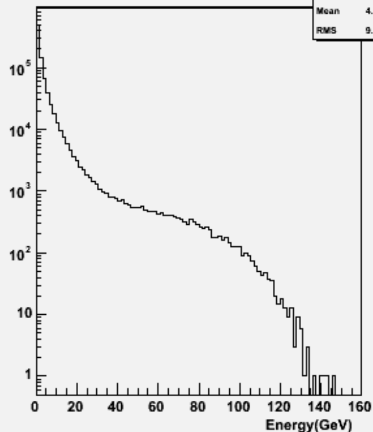
Particle Energy : w101176 sscse1n1_o
