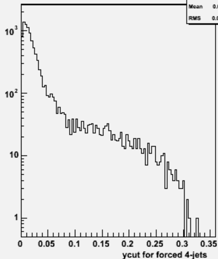
Ycut for 4-jets :w101176 sscse1n1_o
