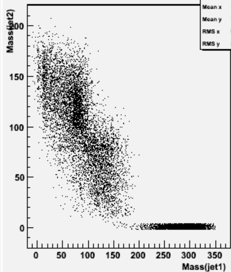
Jet mass for forced 2-jets : w101176 sscse1n1_o
