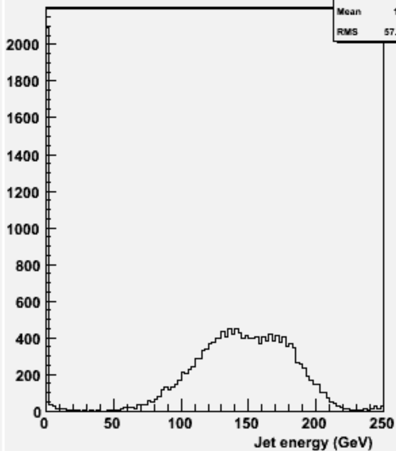
energy for 2-jets :w101176 sscse1n1_o
