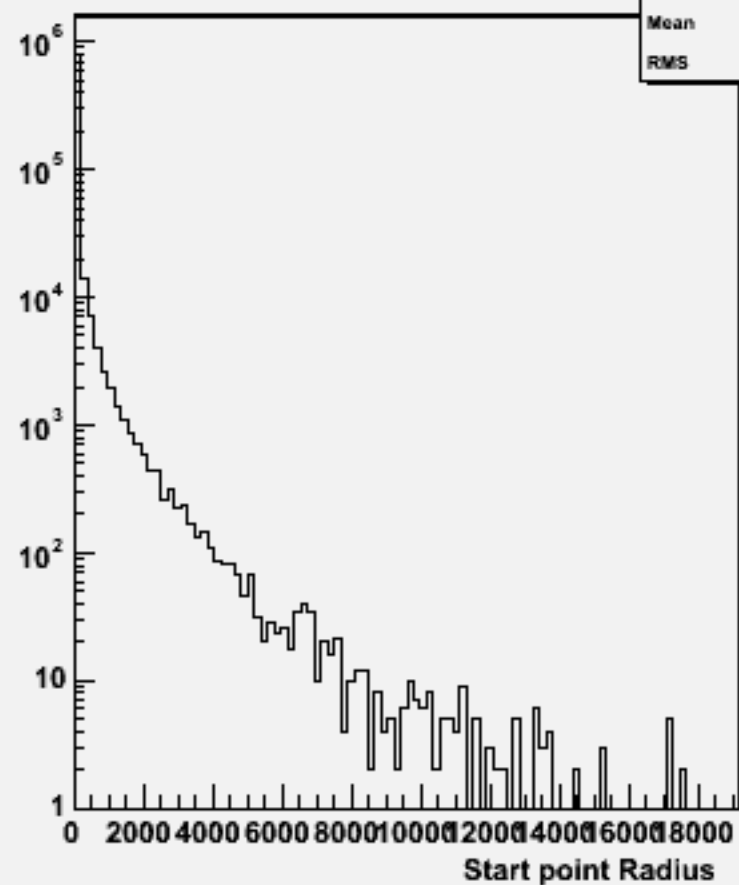
Start point R : w101176 sscse1n1_o
