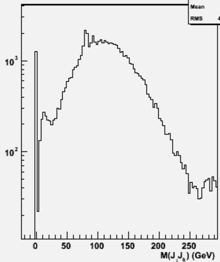
2jets mass(All comb)w101176 sscse1n1_o
