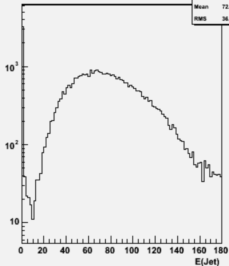
Jet energies(All jets)w101176 sscse1n1_o
