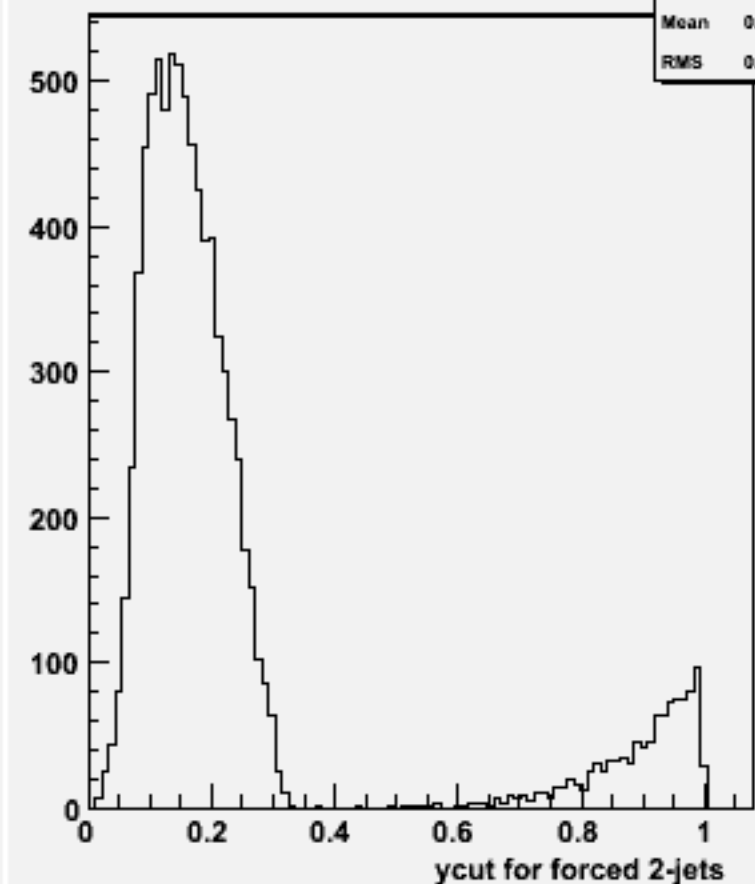
Ycut for 2-jets :w101176 sscse1n1_o
