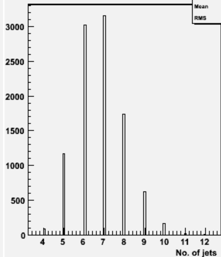
No. jets (ycut=0.001) : w101176 sscse1n1_o
