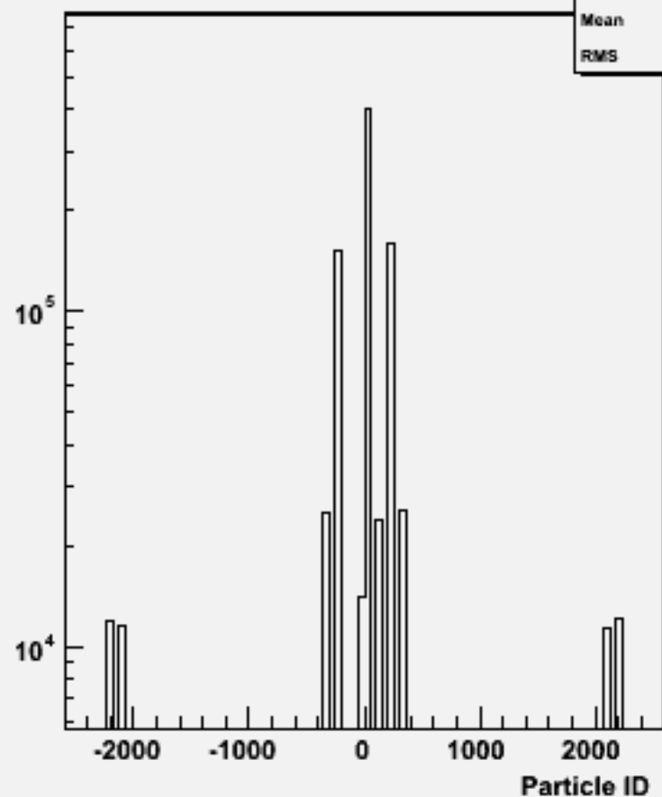
Particle ID : w101176 sscse1n1_o
