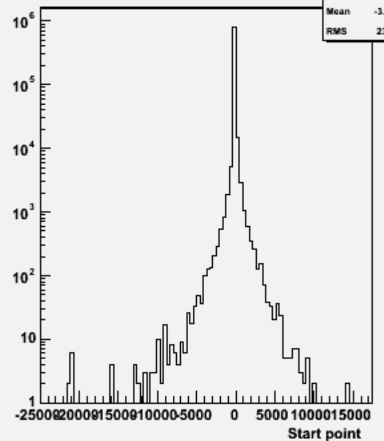
Start point Z : w101176 sscse1n1_o
