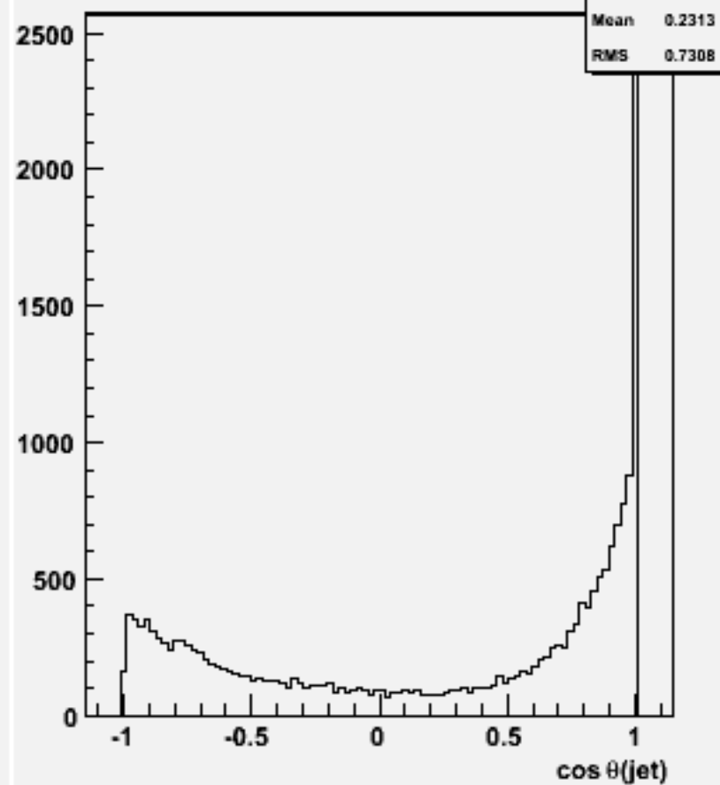
cos \theta for 2-jets :w101176 sscse1n1_o
