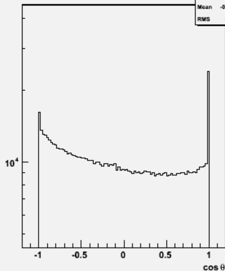
Particle cos \theta : w101176 sscse1n1_o
