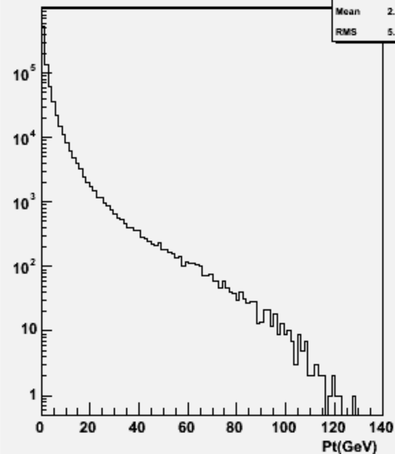
Particle Pt : w101176 sscse1n1_o
