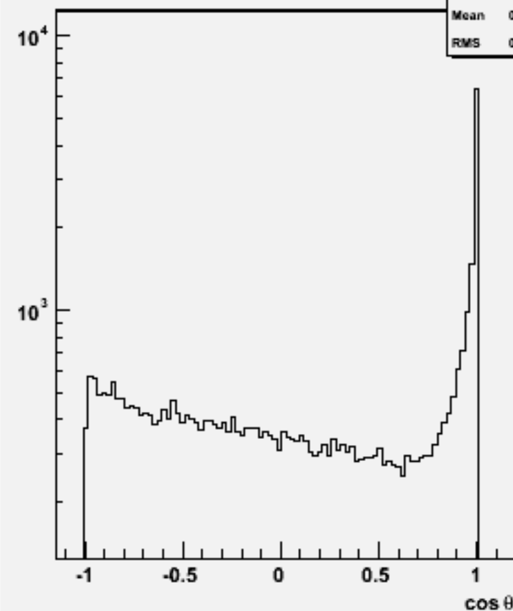
Jet cosθ (All jets)w101176 sscse1n1_o
