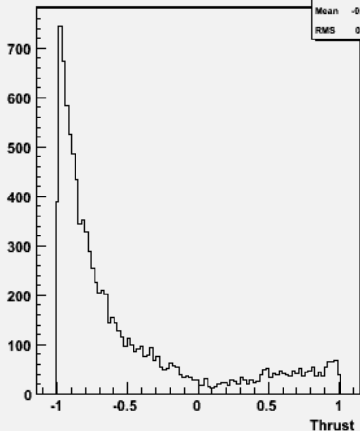
cos \Theta (thrust) w101176 sscse1n1_o
