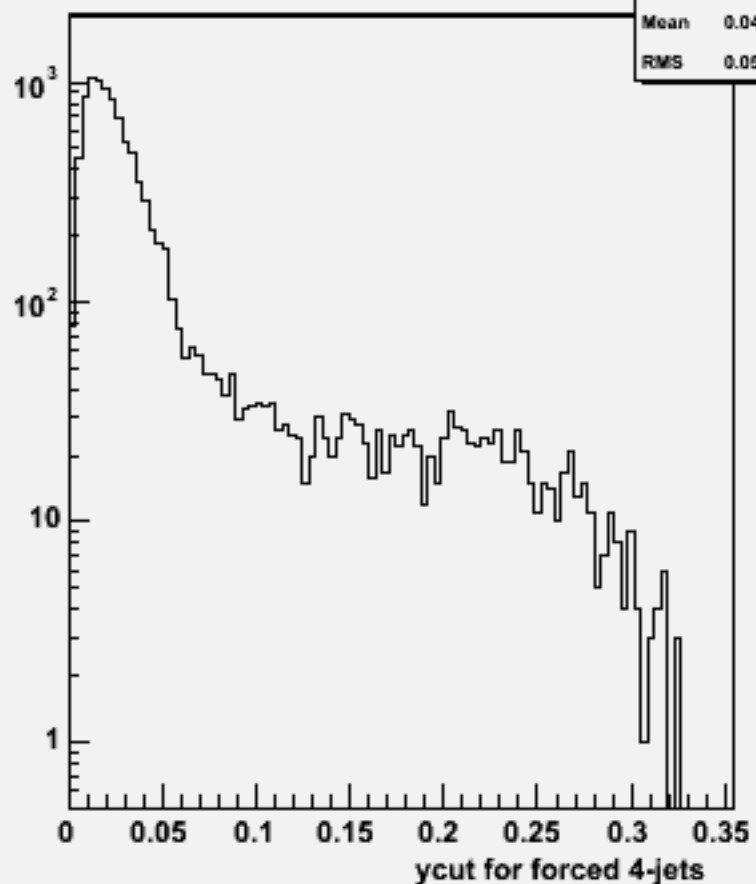
Ycut for 4-jets :w101172 ssudsc_o
