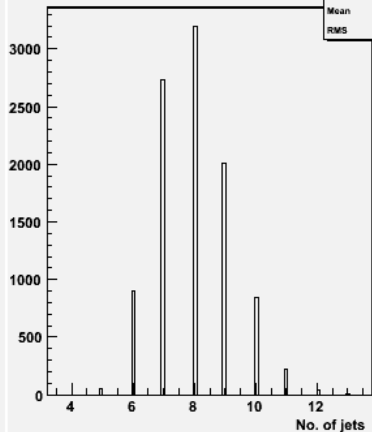
No. jets (ycut=0.001) : w101172 ssudsc_o
