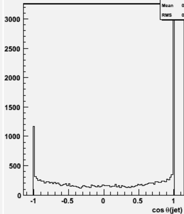
cos \theta for 2-jets :w101172 ssudsc_o
