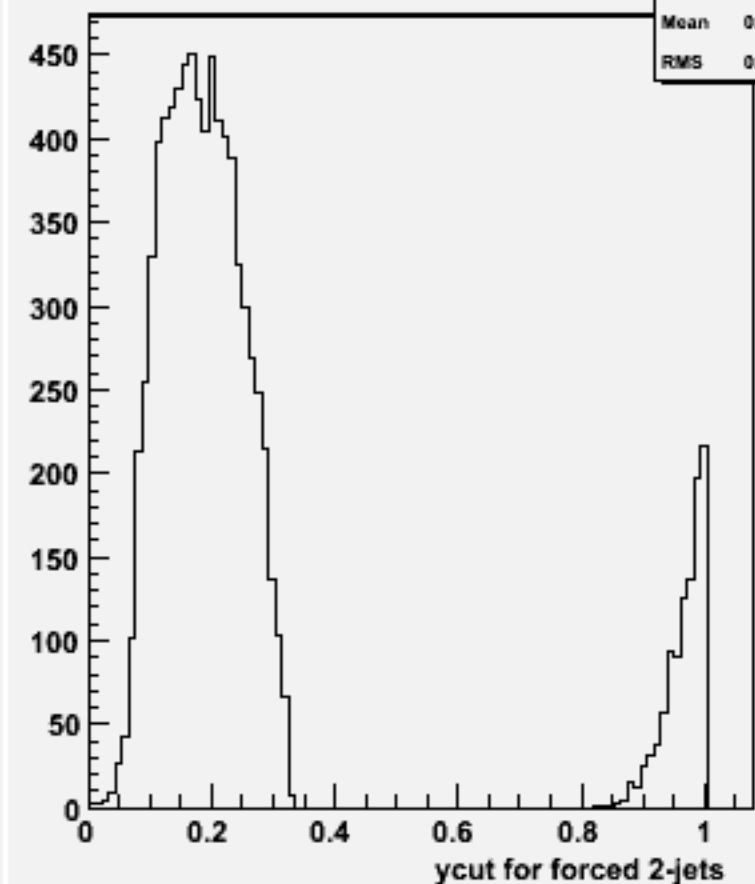
Ycut for 2-jets :w101172 ssudsc_o
