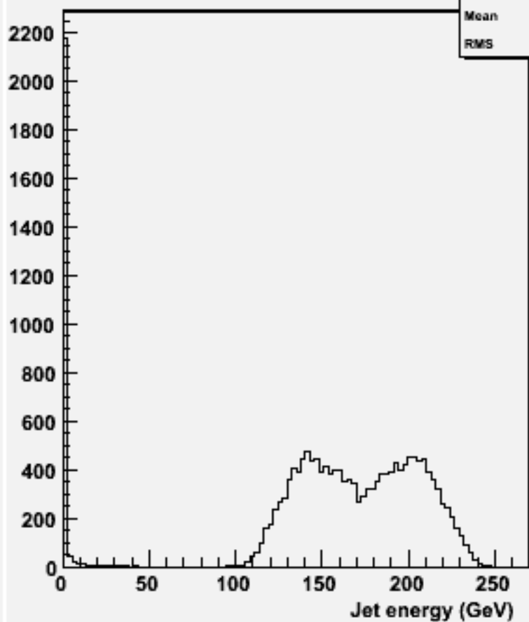
energy for 2-jets :w101172 ssudsc_o
