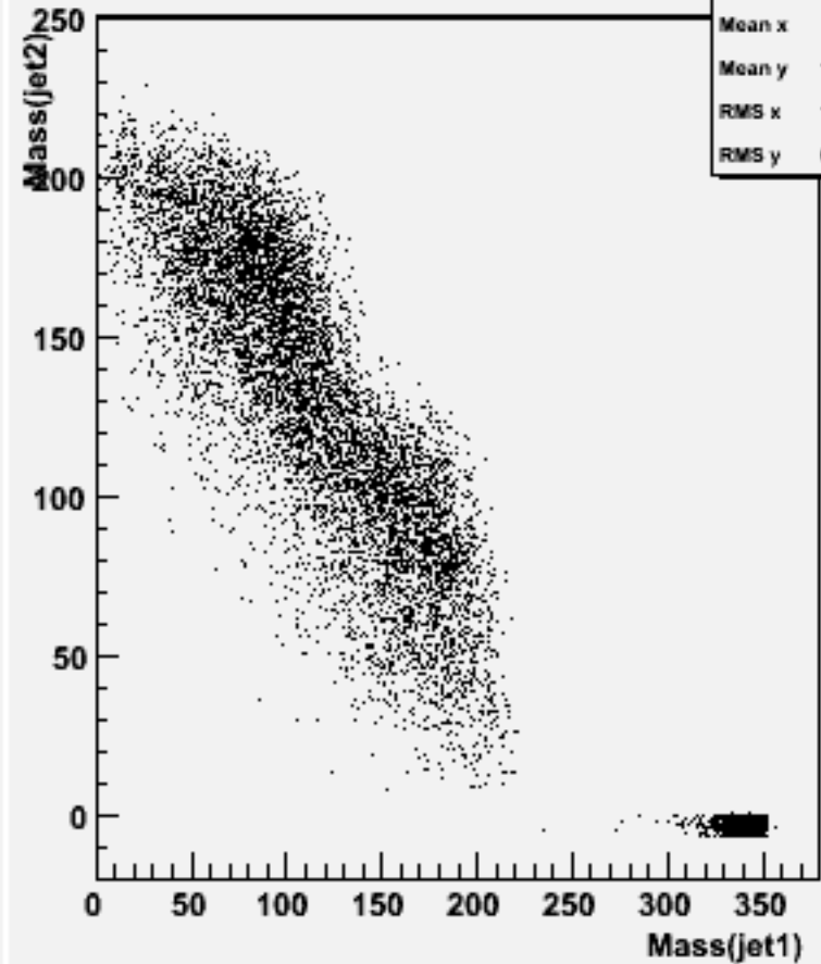
Jet mass for forced 2-jets : w101172 ssudsc_o
