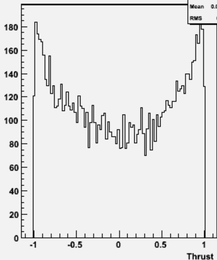
cos \Theta (thrust) w101172 ssudsc_o
