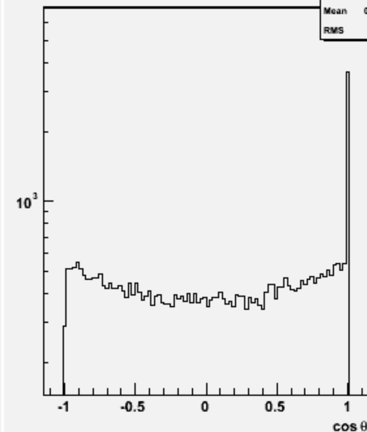
Jet cos \theta (All jets)w101172 ssudsc_o
