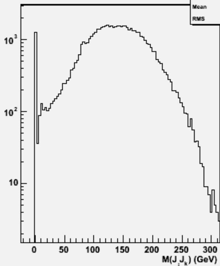
2jets mass(All comb)w101172 ssudsc_o
