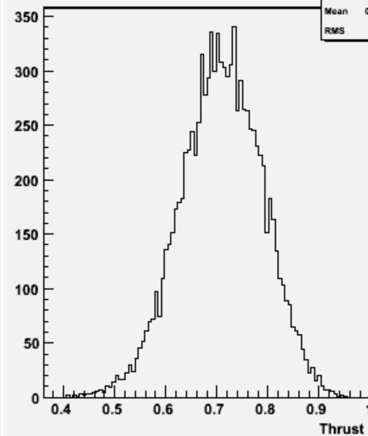
Thrust w101169 ssuddu_o
