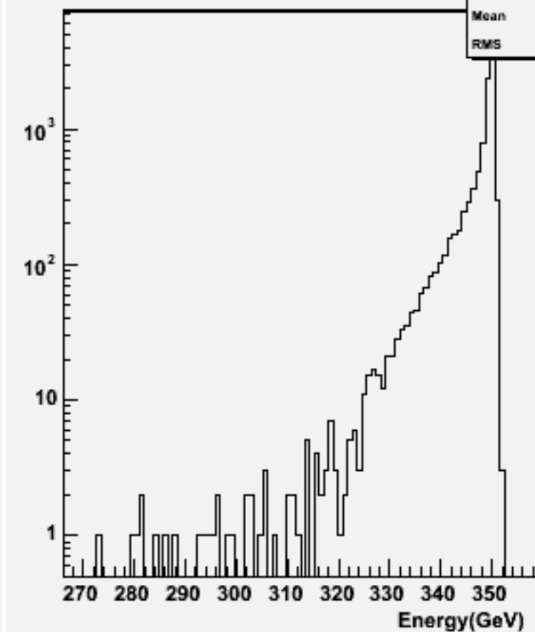
Total Energy (w/o \nu ): w101169 ssuddu_o
