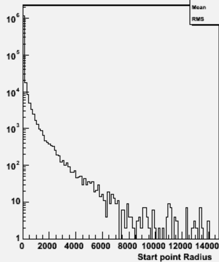
Start point R : w101169 ssuddu_o
