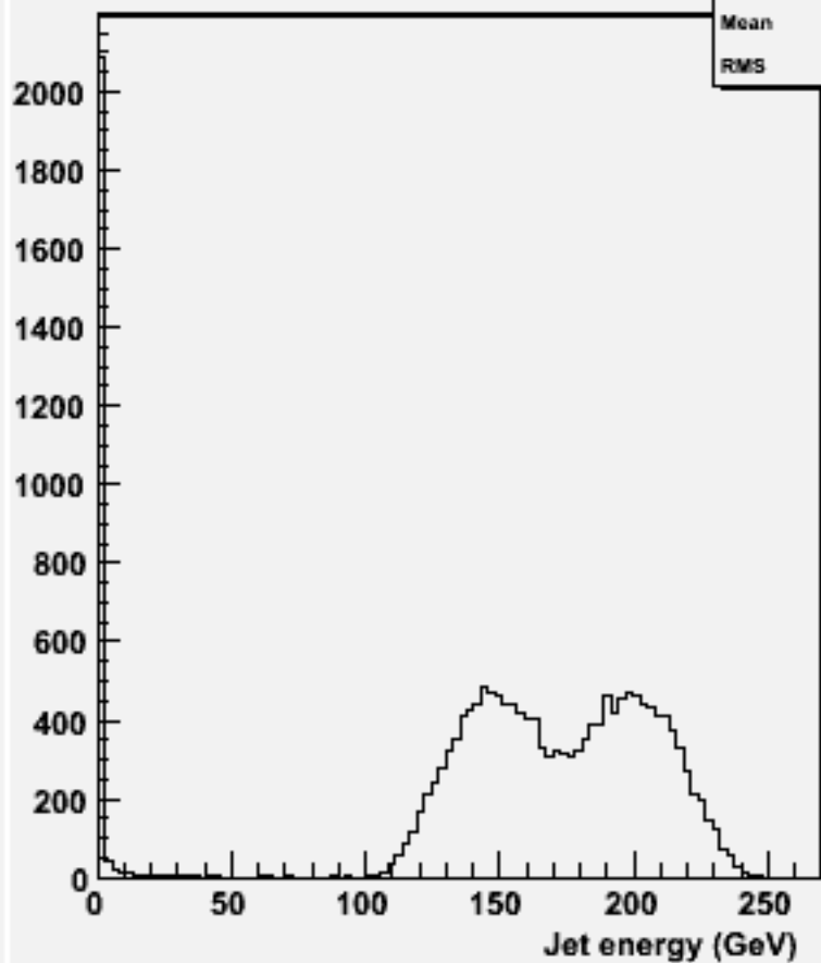
energy for 2-jets :w101169 ssuddu_o
