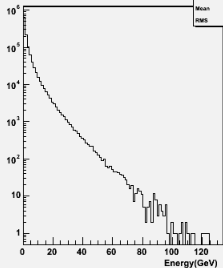
Particle Energy : w101169 ssuddu_o
