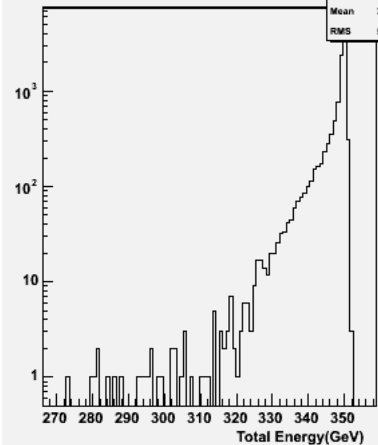
Total Energy (inc. \nu ): w101169 ssuddu_o
