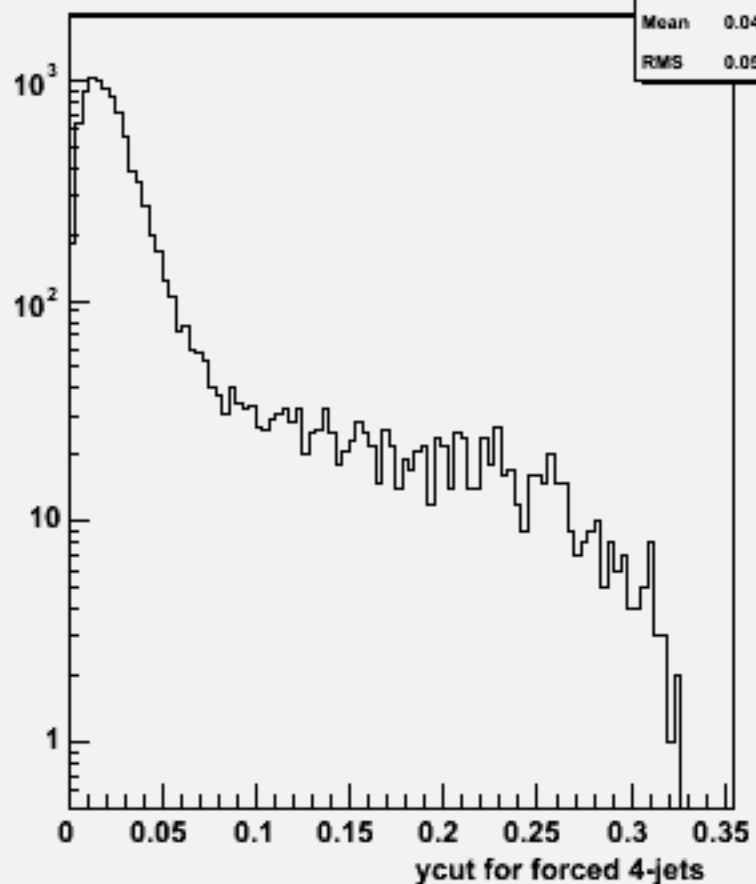
Ycut for 4-jets :w101169 ssuddu_o
