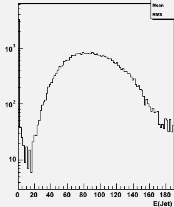
Jet energies(All jets)w101169 ssuddu_o
