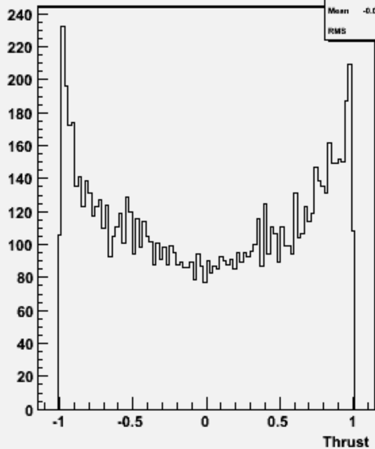
cos \Theta (thrust) w101169 ssuddu_o
