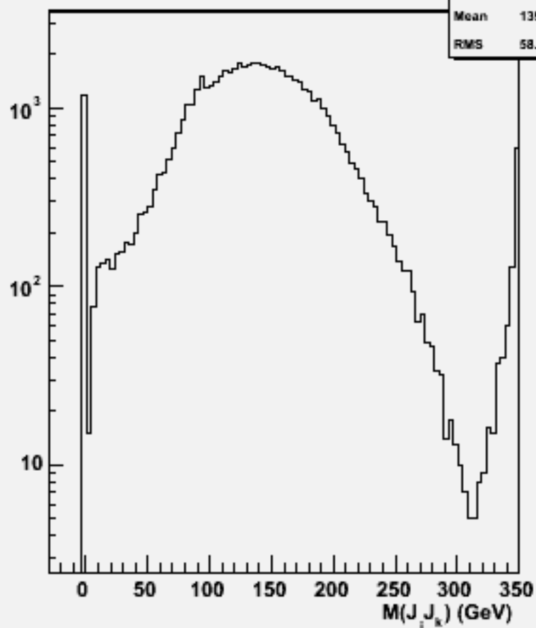
2jets mass(All comb)w101169 ssuddu_o
