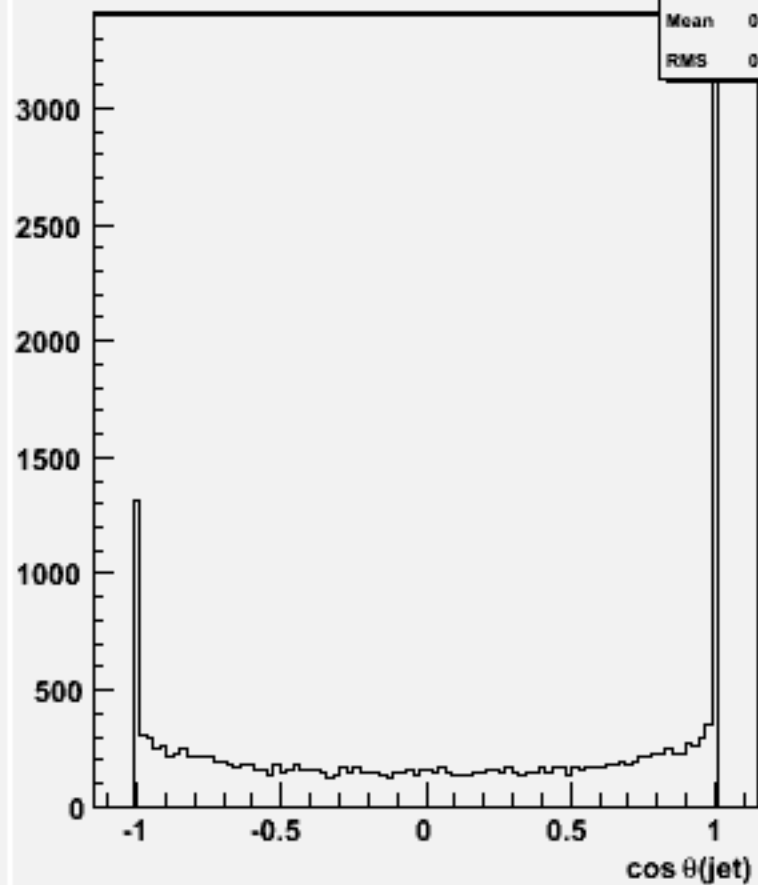
cos \theta for 2-jets :w101169 ssuddu_o
