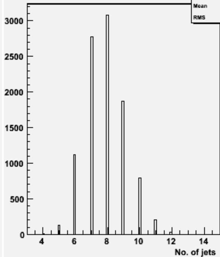
No. jets (ycut=0.001) : w101169 ssuddu_o
