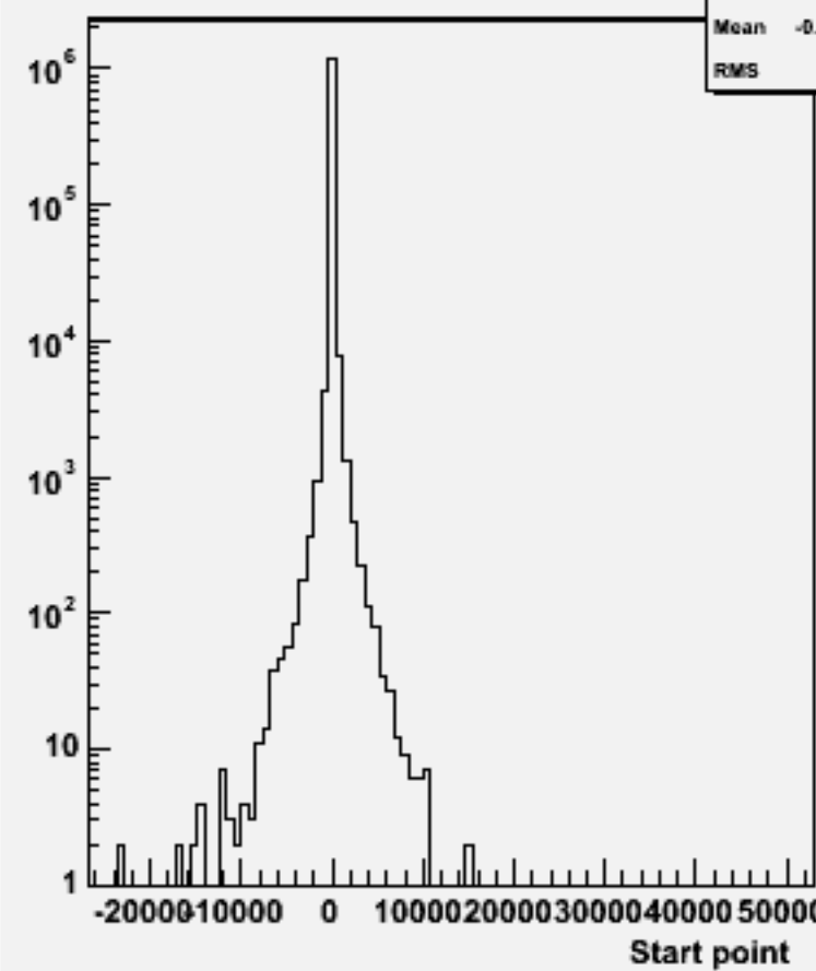
Start point Z : w101169 ssuddu_o
