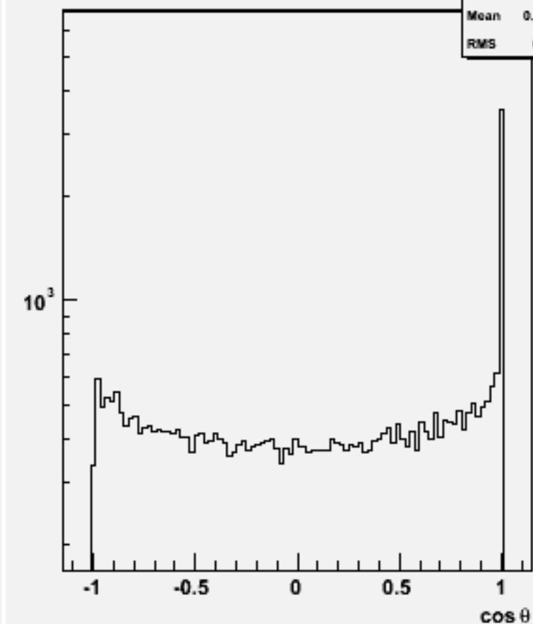
Jet cos \theta (All jets)w101169 ssuddu_o
