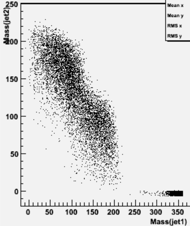
Jet mass for forced 2-jets : w101169 ssuddu_o
