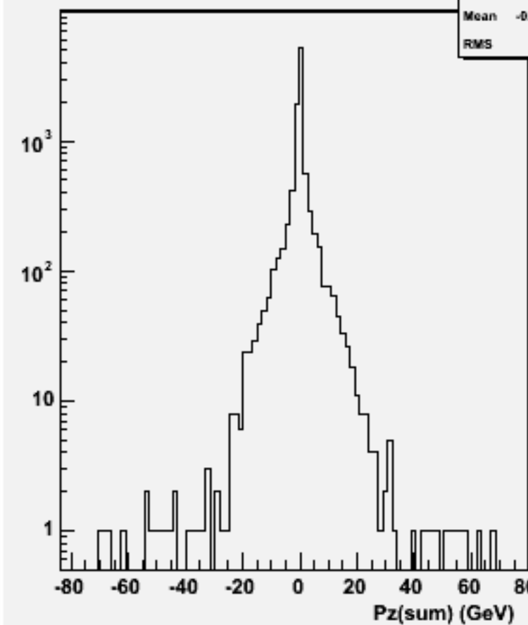
Pz Sum: w101169 ssuddu_o
