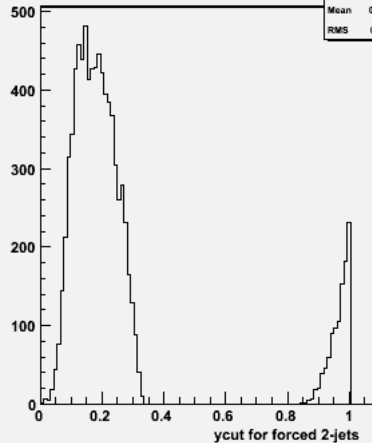
Ycut for 2-jets :w101169 ssuddu_o
