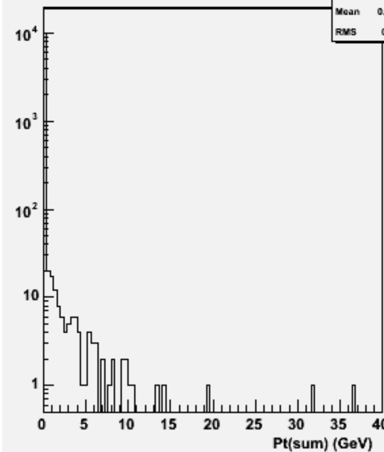
Pt Sum: w101169 ssuddu_o
