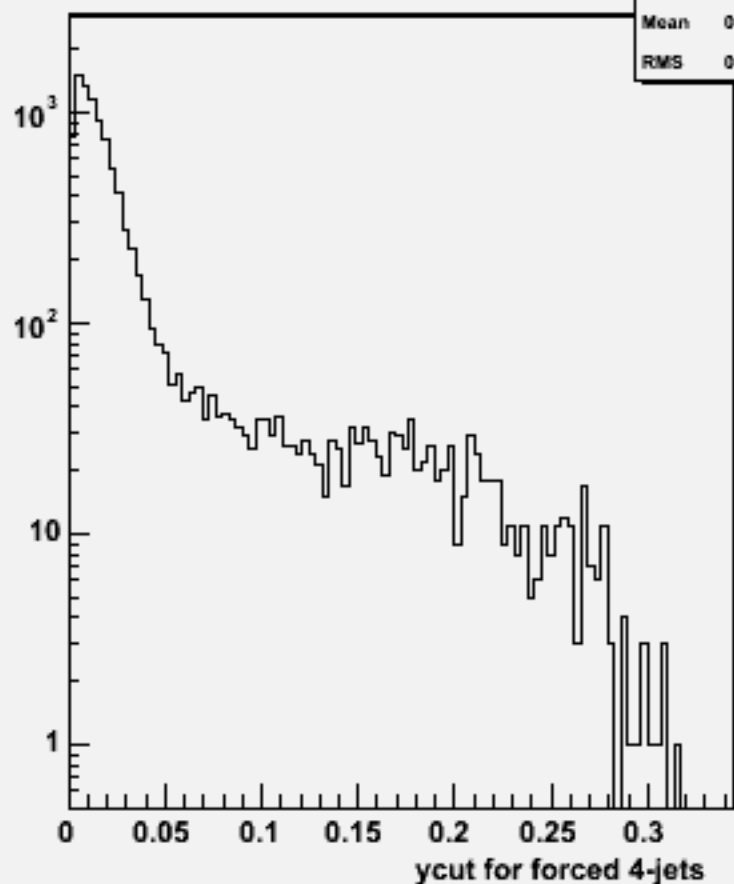
Ycut for 4-jets :w101165 ssude3n3_o
