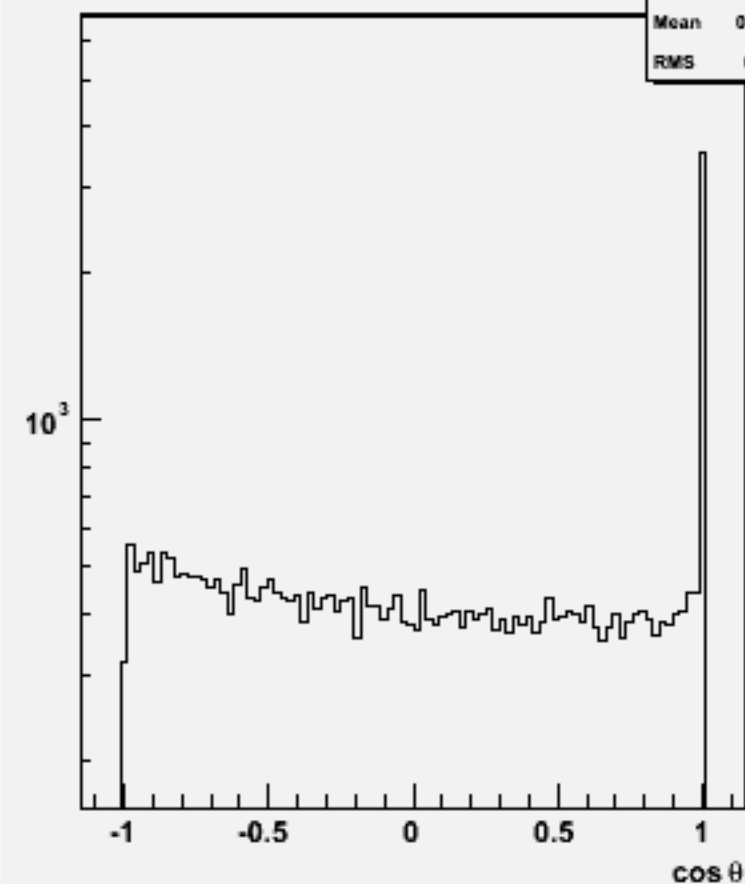
Jet cosθ (All jets)w101165 ssude3n3_o
