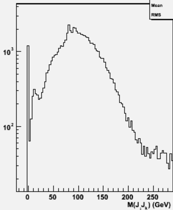
2jets mass(All comb)w101165 ssude3n3_o
