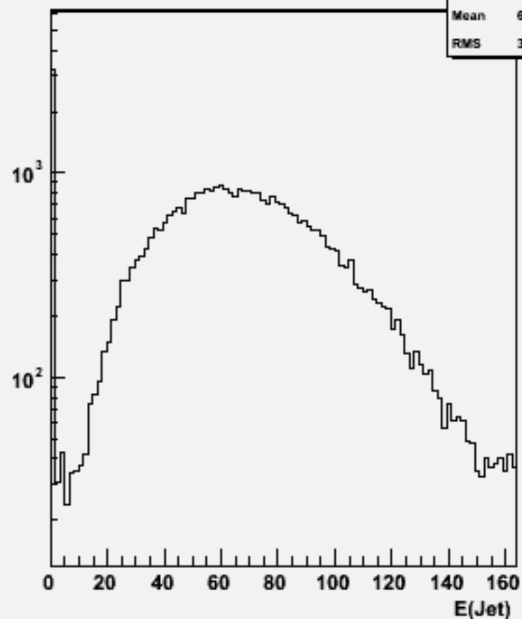
Jet energies(All jets)w101165 ssude3n3_o
