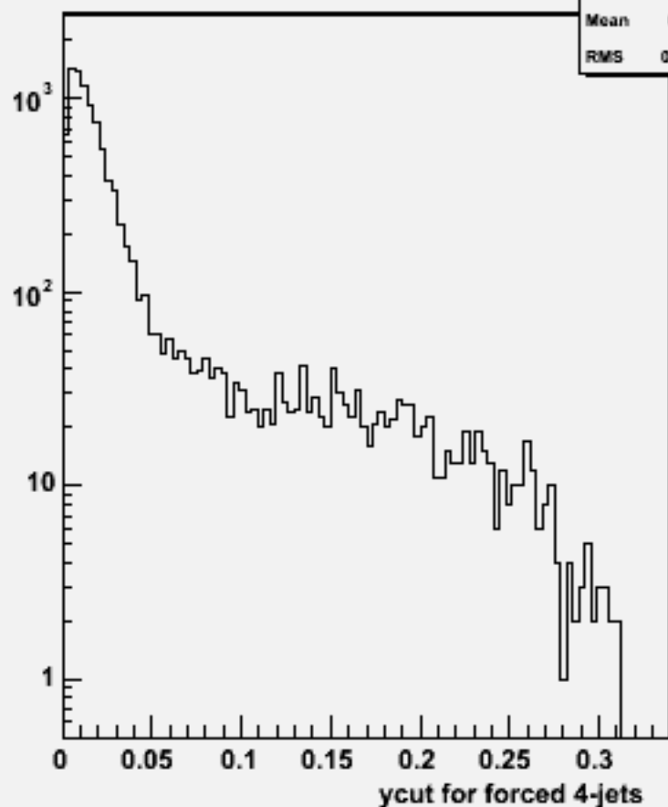
Ycut for 4-jets :w101164 ssude3n3_o
