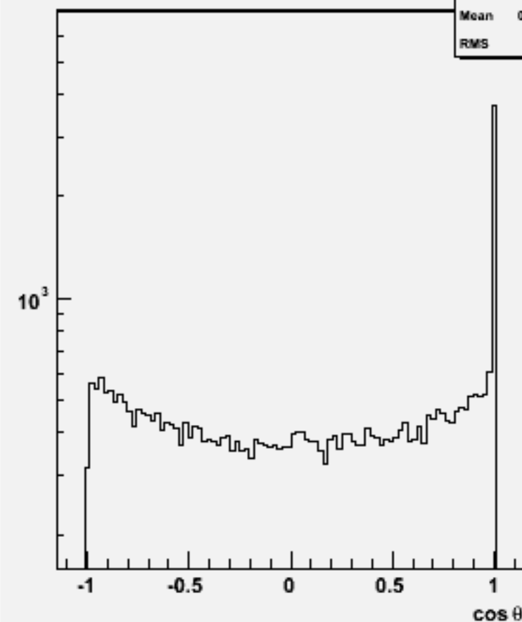
Jet cosθ (All jets)w101164 ssude3n3_o
