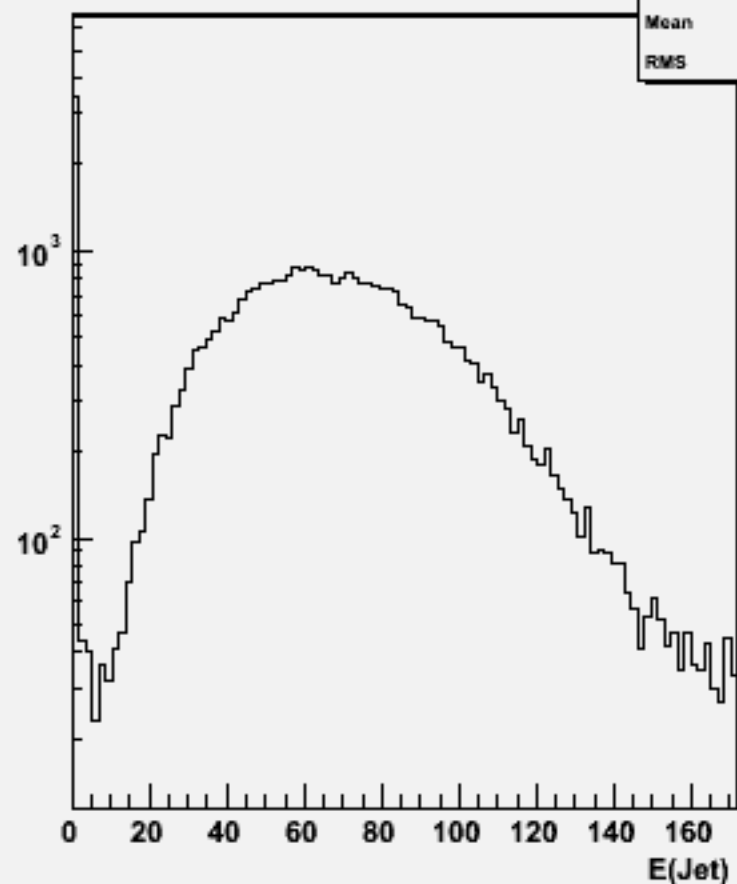
Jet energies(All jets)w101164 ssude3n3_o
