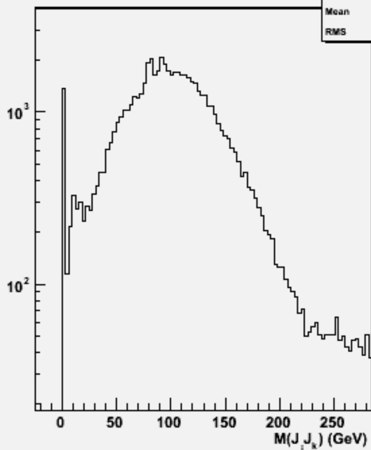
2jets mass(All comb)w101164 ssude3n3_o
