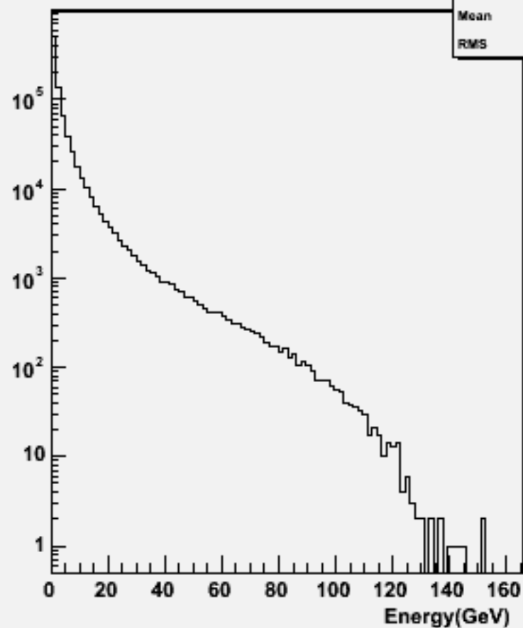
Particle Energy : w101164 ssude3n3_o
