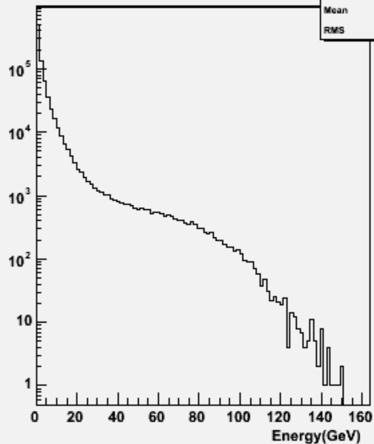
Particle Energy : w101161 ssude2n2_o
