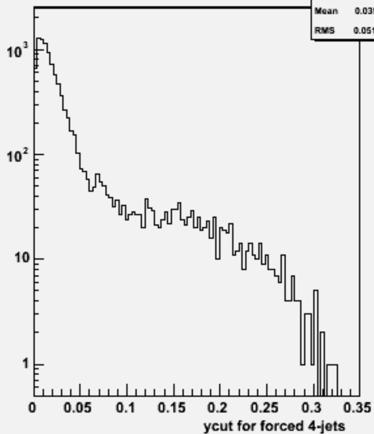
Ycut for 4-jets :w101161 ssude2n2_o
