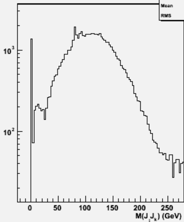
2jets mass(All comb)w101161 ssude2n2_o
