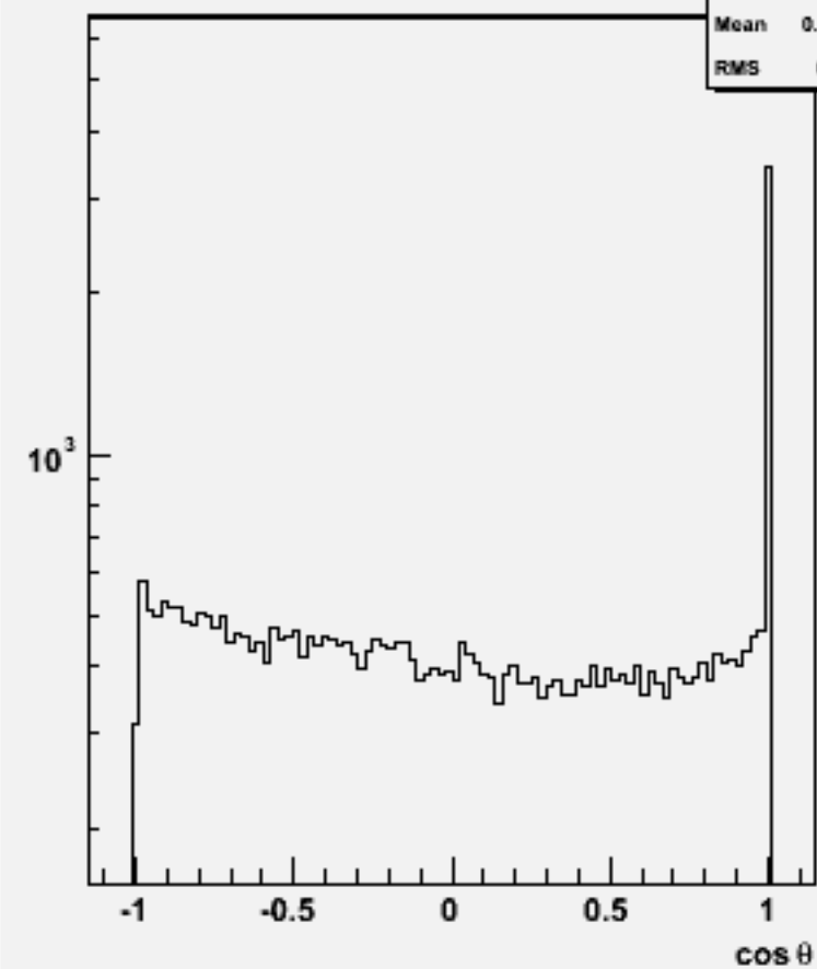
Jet cosθ (All jets)w101161 ssude2n2_o
