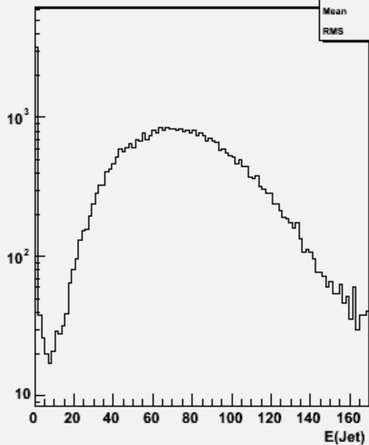
Jet energies(All jets)w101161 ssude2n2_o
