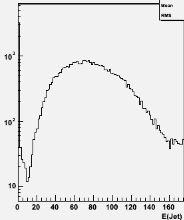
Jet energies(All jets)w101160 ssude2n2_o
