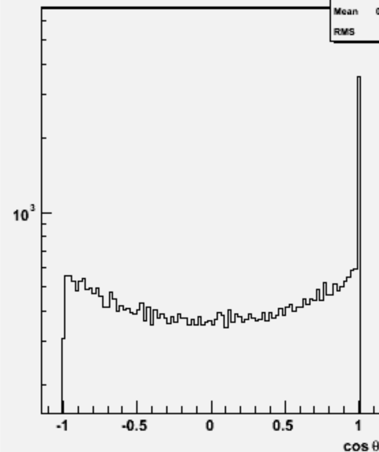
Jet cosθ (All jets)w101160 ssude2n2_o
