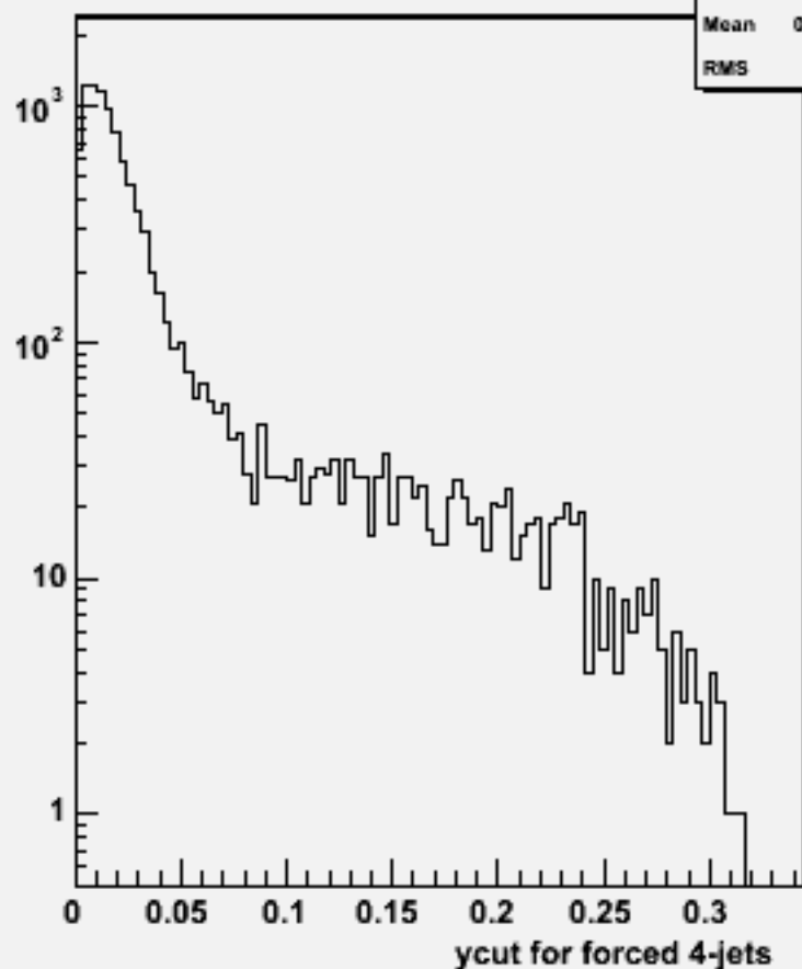
Ycut for 4-jets :w101160 ssude2n2_o
