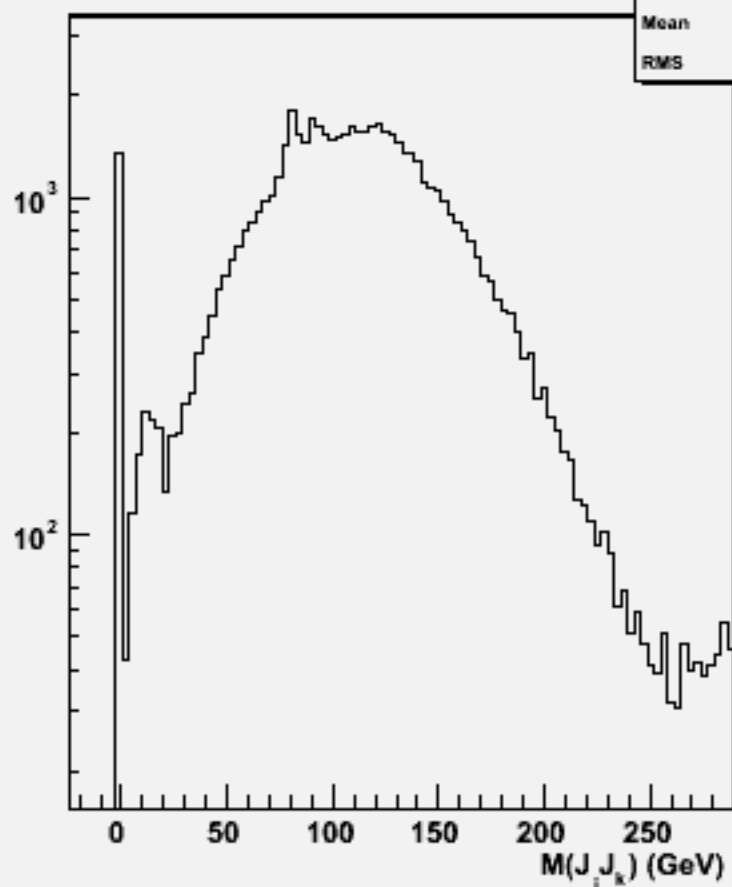
2jets mass(All comb)w101160 ssude2n2_o
