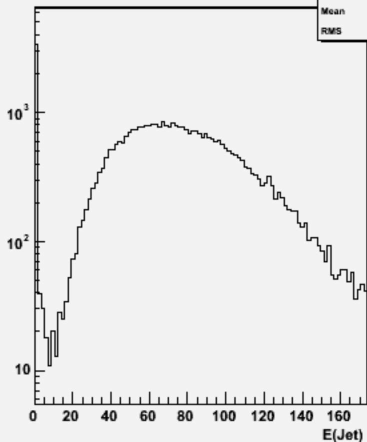
Jet energies(All jets)w101158 ssude1n1_o
