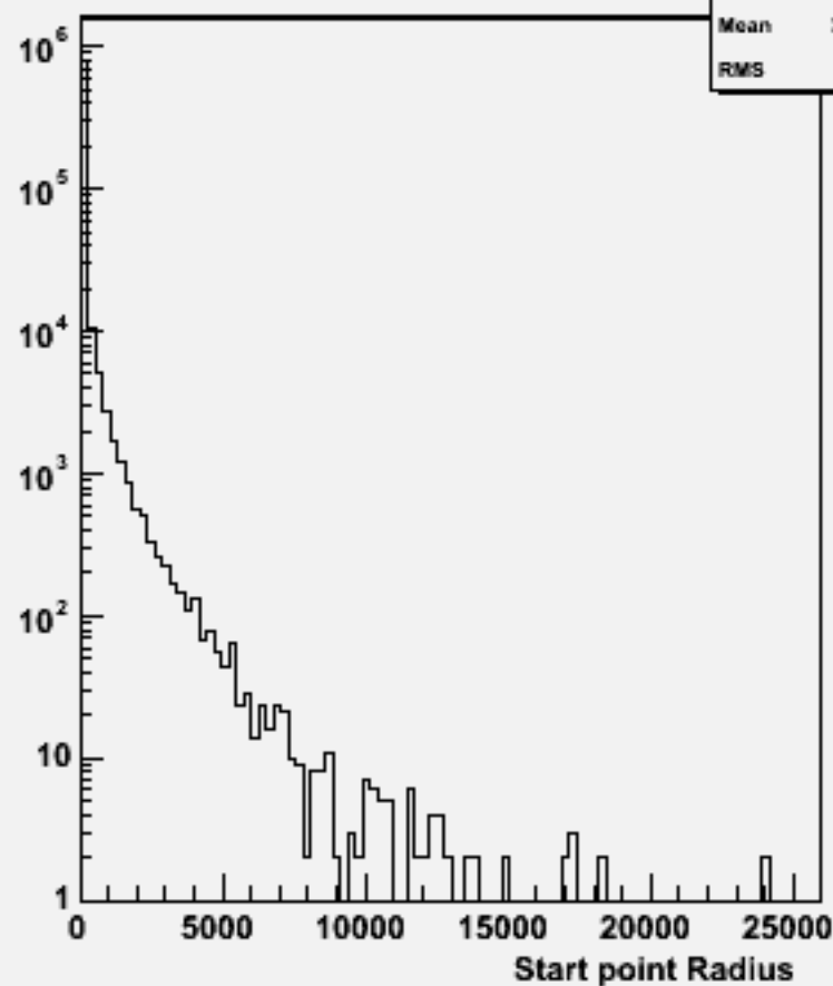
Start point R : w101158 ssude1n1_o
