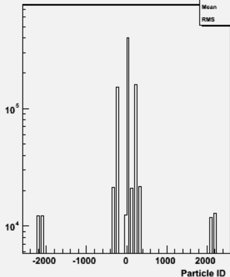
Particle ID : w101158 ssude1n1_o
