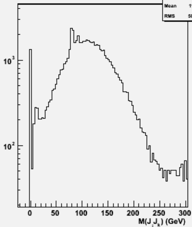
2jets mass(All comb)w101158 ssude1n1_o
