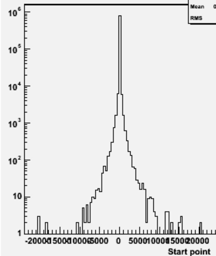
Start point Z : w101158 ssude1n1_o
