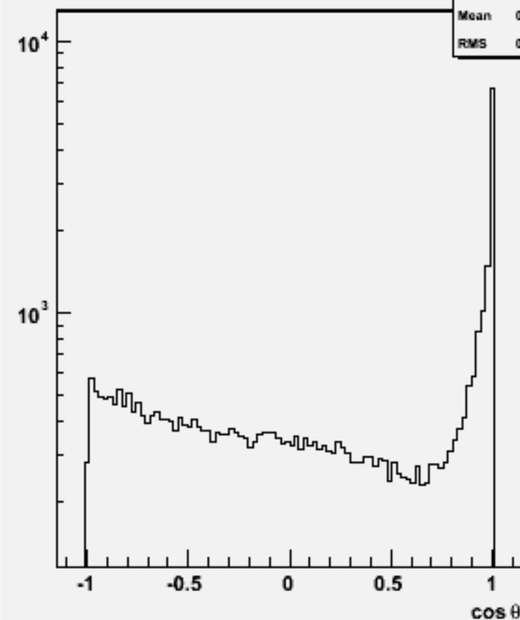
Jet cos \theta (All jets)w101158 ssude1n1_o
