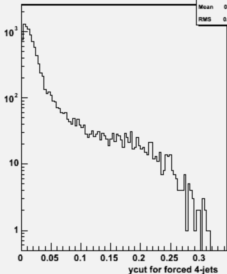
Ycut for 4-jets :w101158 ssude1n1_o
