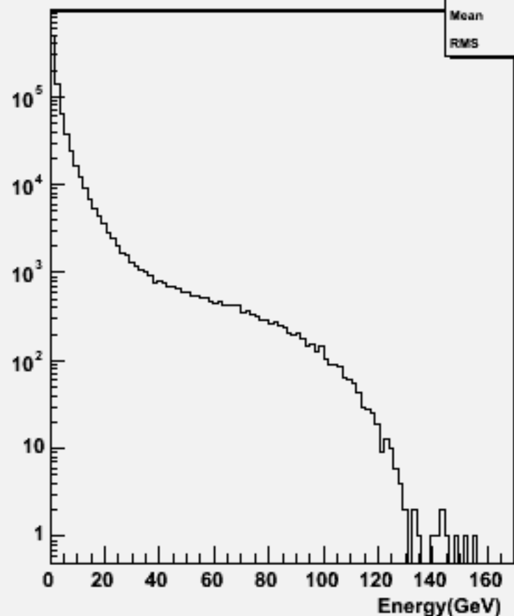
Particle Energy : w101158 ssude1n1_o
