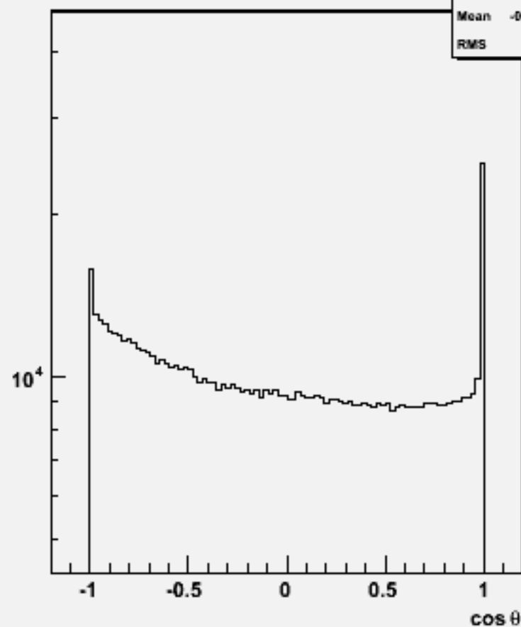
Particle cos \theta : w101158 ssude1n1_o
