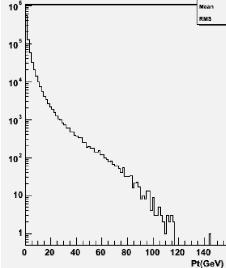
Particle Pt : w101158 ssude1n1_o
