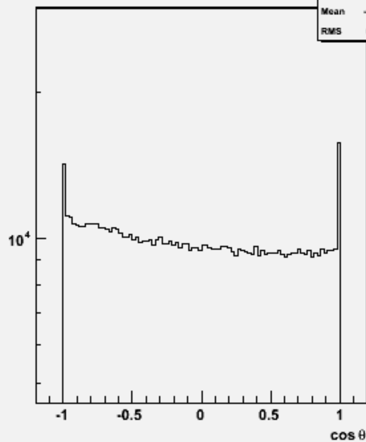
Particle cos \theta : w101157 ssude1n1_o
