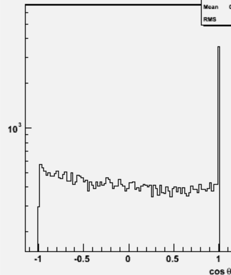
Jet cosθ (All jets)w101157 ssude1n1_o
