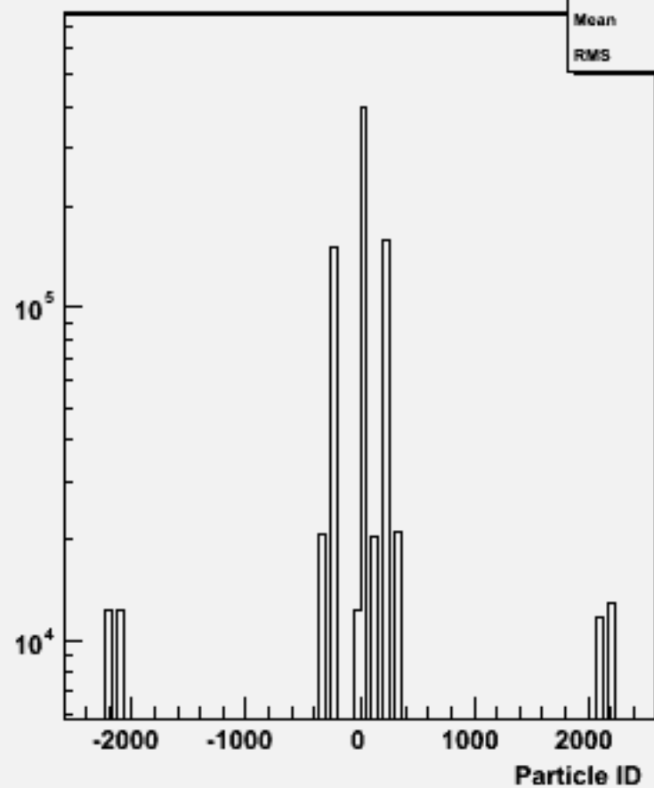
Particle ID : w101157 ssude1n1_o
