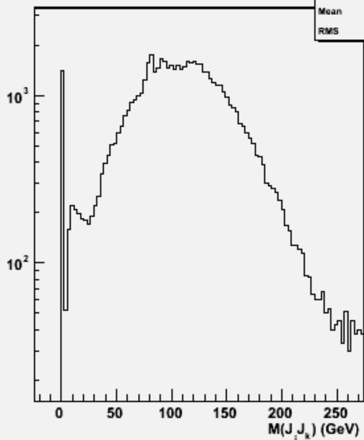
2jets mass(All comb)w101157 ssude1n1_o
