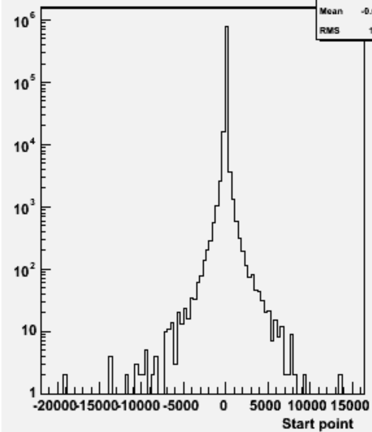
Start point Z : w101157 ssude1n1_o
