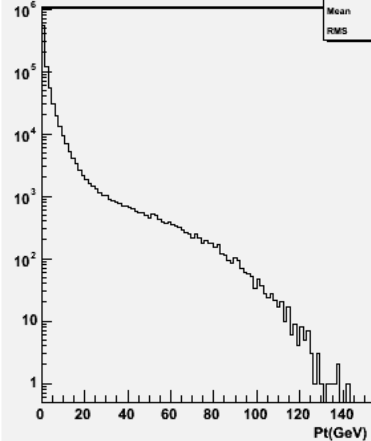
Particle Pt : w101157 ssude1n1_o
