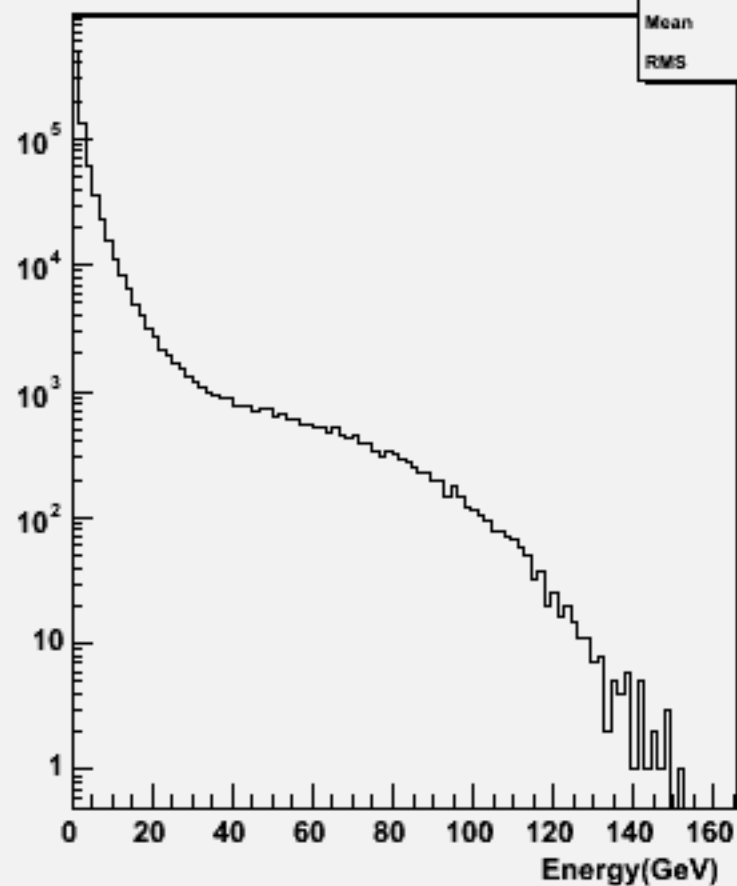
Particle Energy : w101157 ssude1n1_o
