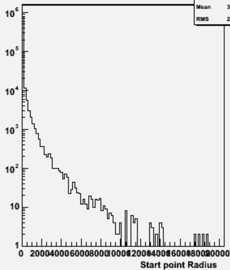
Start point R : w101157 ssude1n1_o
