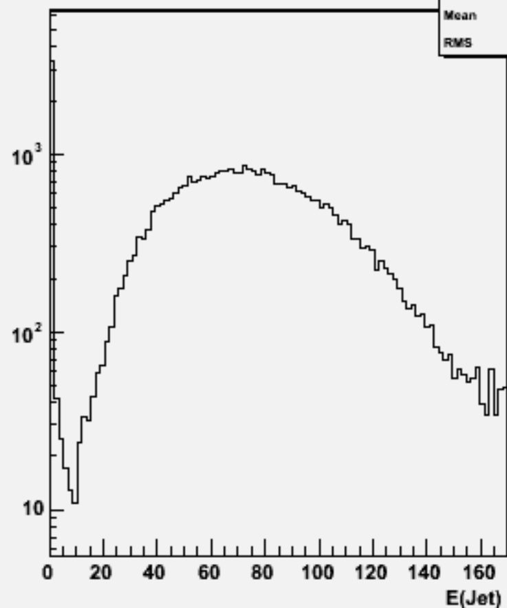
Jet energies(All jets)w101157 ssude1n1_o
