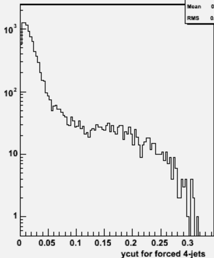
Ycut for 4-jets :w101157 ssude1n1_o
